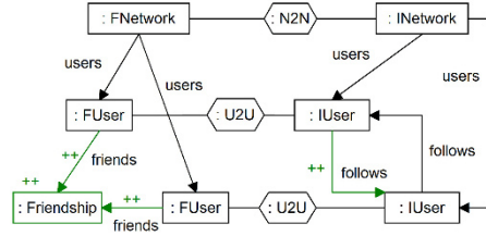
Fig. 7. Rule AcceptFriendship
