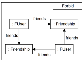
Fig. 2. NoDoubleFriendship
