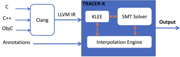
Fig. 1. TracerX Framework
