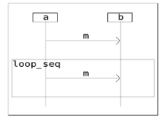
(b) i' = seq(i_{|_{11}}, i)
