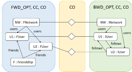
Fig. 11. Input models per operation
