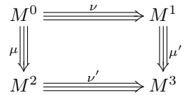
Fig. 7. Pushout in \mathbb{M}
