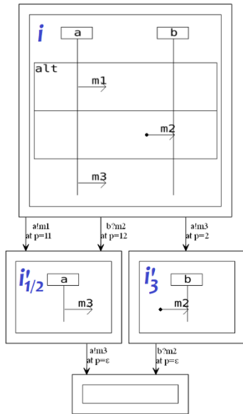
Fig. 5: Operational Semantics
