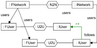
Fig. 6. Rule RequestFriendship
