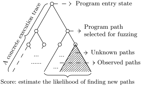
Fig. 2: MCTS-guided fuzzing in LEGION
