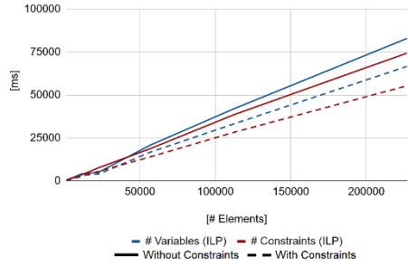
Fig. 10. #Variables and #Constraints
