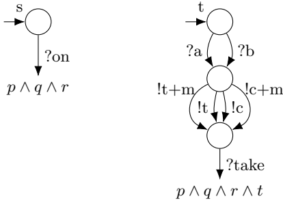
Fig. 2. Two specifications with transitions to a conjunction.
