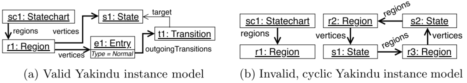
Fig. 2: Sample Yakindu Statechart instance models
