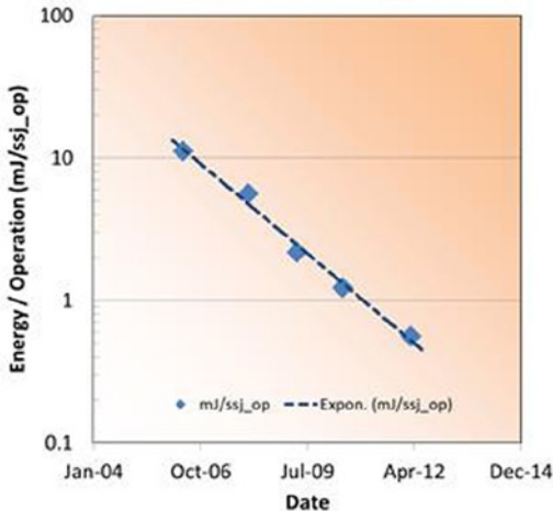
Figure 1-10. The SPECpower ssj_2008 trend of the energy per operation as a function of time shows an exponential trend that is consistent with an efficiency-doubling time of 0.9 years. This is much faster than the 1.5 years reported by Koomey, owing to additional efficiency gains from energy proportionality
