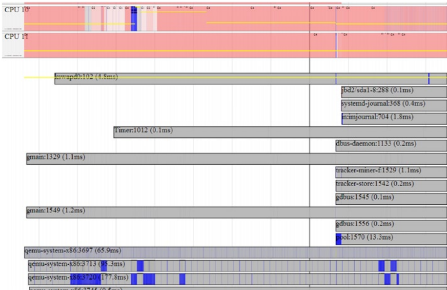
Figure 7-17. Timechart part 2: software thread activity
