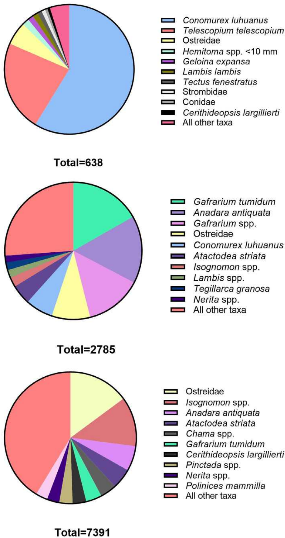
Figure 5.5. Percentage distributions of midden shell taxa in SU1 (top), SU3 (middle) and SU5 (bottom), as calculated from MNI values.
