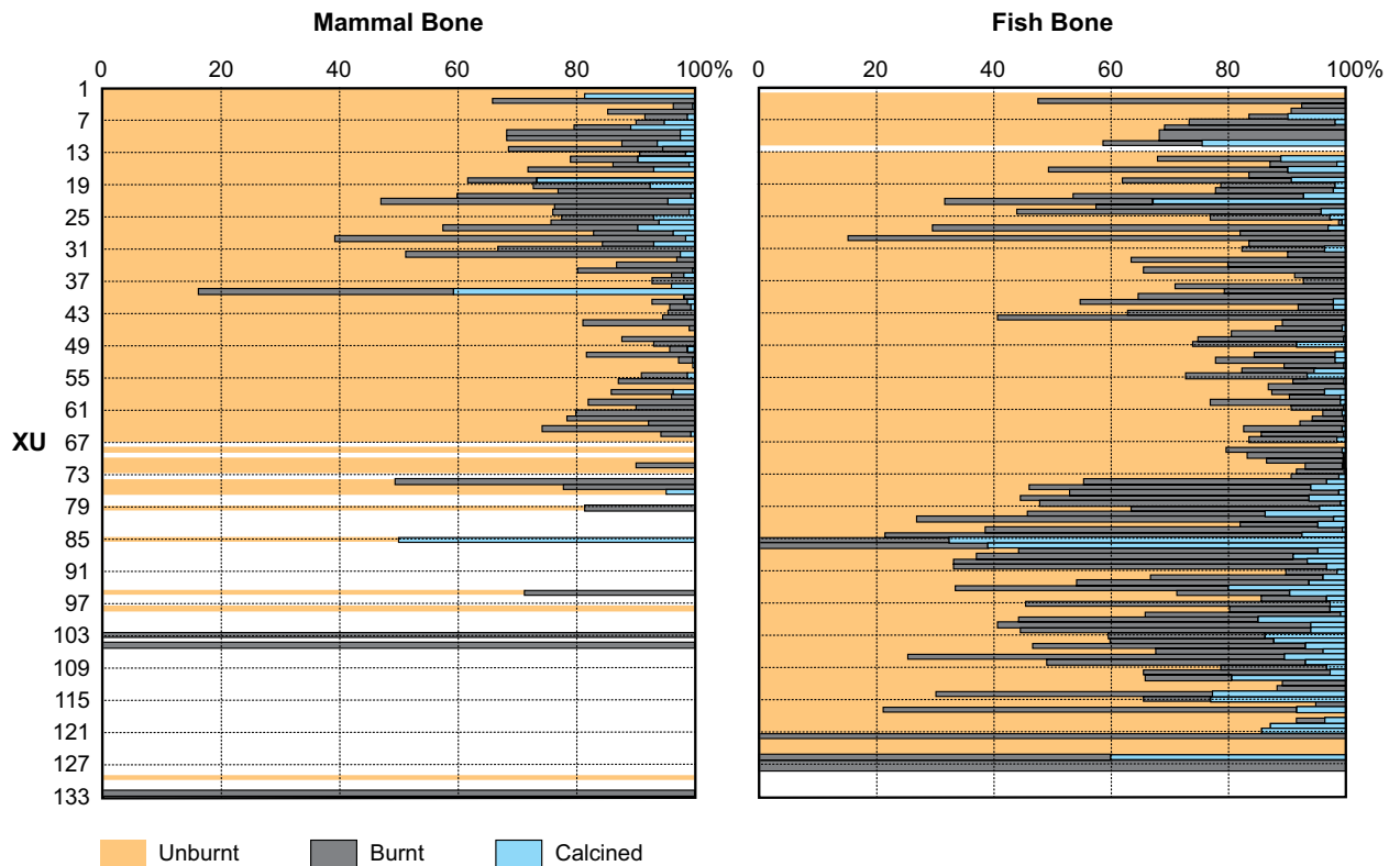
Figure 6.3. Distribution of unburnt, burnt (carbonised) and calcined mammal and fish bone by XU, Tanamu 1.
