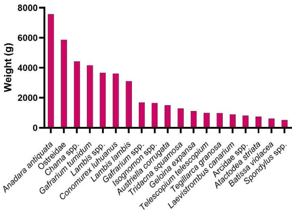
Figure 5.1. Molluscan taxa represented by >500g identified from Square A, Tanamu 1.
