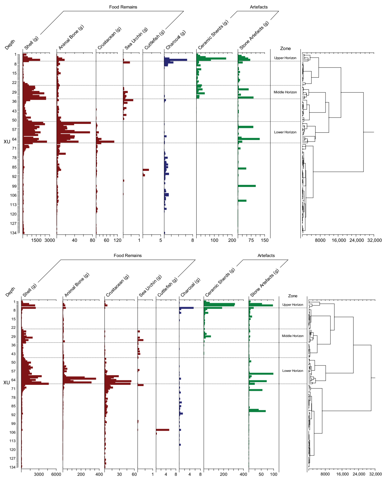
Figure 2.26. Distribution of cultural materials by XU, Tanamu 1 Squares A (top) and B (bottom).
