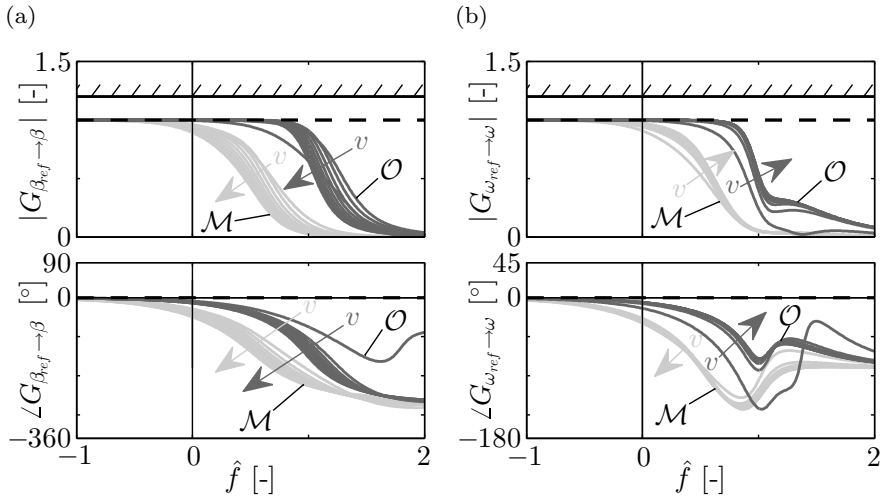
Figure 6.9: Comparison of manual design \mathcal{M} (light) with optimised design \mathcal{O} (dark) w.r.t. frequency responses of transfer functions (a) G_{\beta_{ref} \rightarrow \beta} and (b) G_{\omega_{ref} \rightarrow \omega} for vehicle speeds v = 10 \dots 100 km/h
