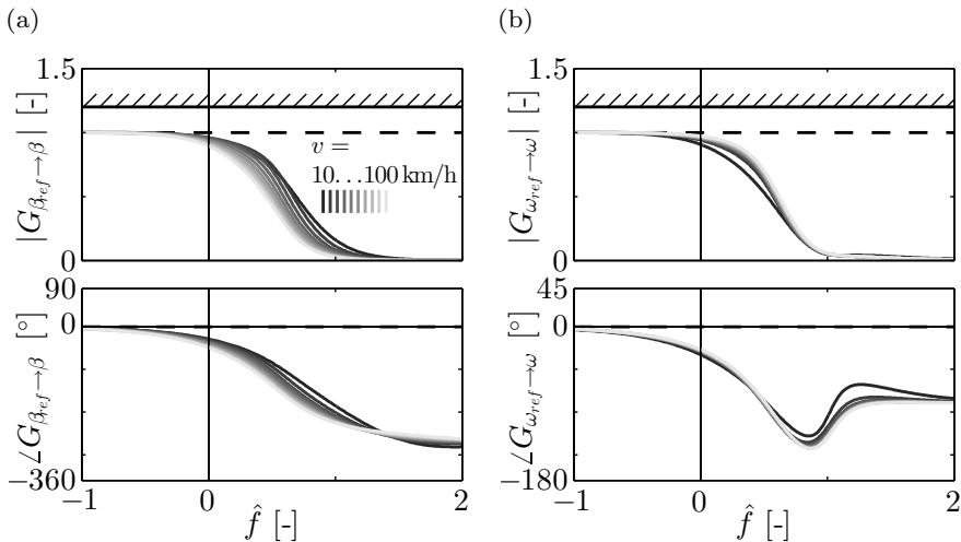
Figure 5.11: Dynamic performance criteria based on transfer functions (a) G_{\beta_{\text{ref}} \rightarrow \beta} and (b) G_{\omega_{\text{ref}} \rightarrow \omega} with desired characteristics (dashed) and upper bounds (hatched)
