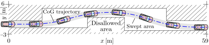
Figure 5.6: Double lane change test track and vehicle’s trajectory for v = 60 km/h
