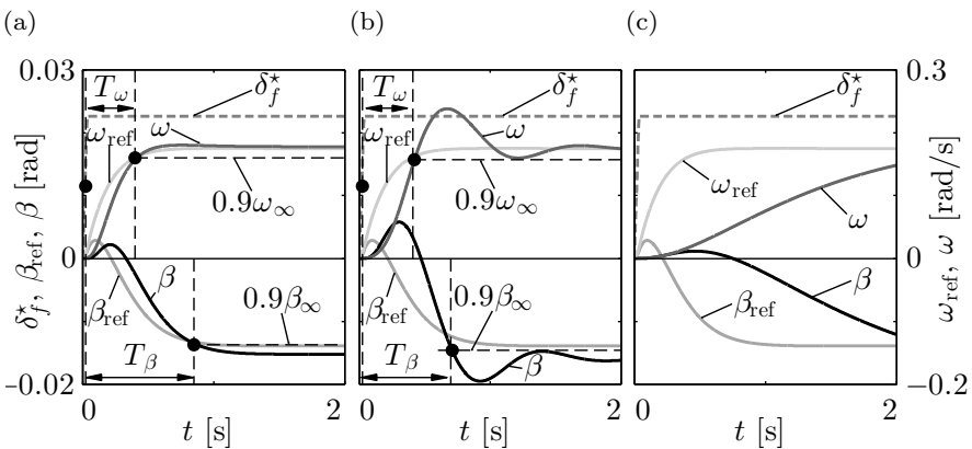
Figure 5.10: Step responses for different state weights \mathbf{Q} : (a) regular, (b) oscillatory and (c) slow behaviour (scale for \delta and \beta is shown on the left, that of \omega on the right)
