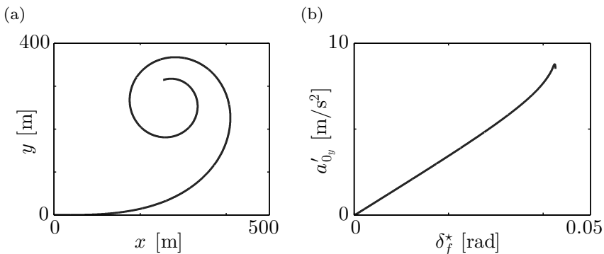
Figure 5.12: Quasi-steady cornering with constant speed v = 80 \text{ km/h} resulting in (a) spiral trajectory and (b) corresponding lateral acceleration
