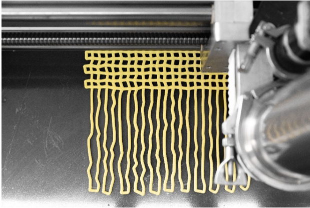
Fig. 3: Matteo Silverio, rehub, Proprietary 3d printer extruding revero (glass paste), 2024.
