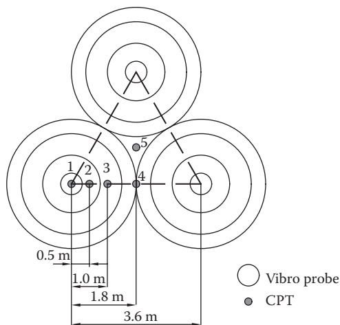
Figure 3.53 Post-CPT locations to establish acceptance criteria for vibro compaction.
