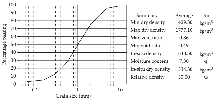
Figure 3.36 Typical grain size distribution and properties of sand.
