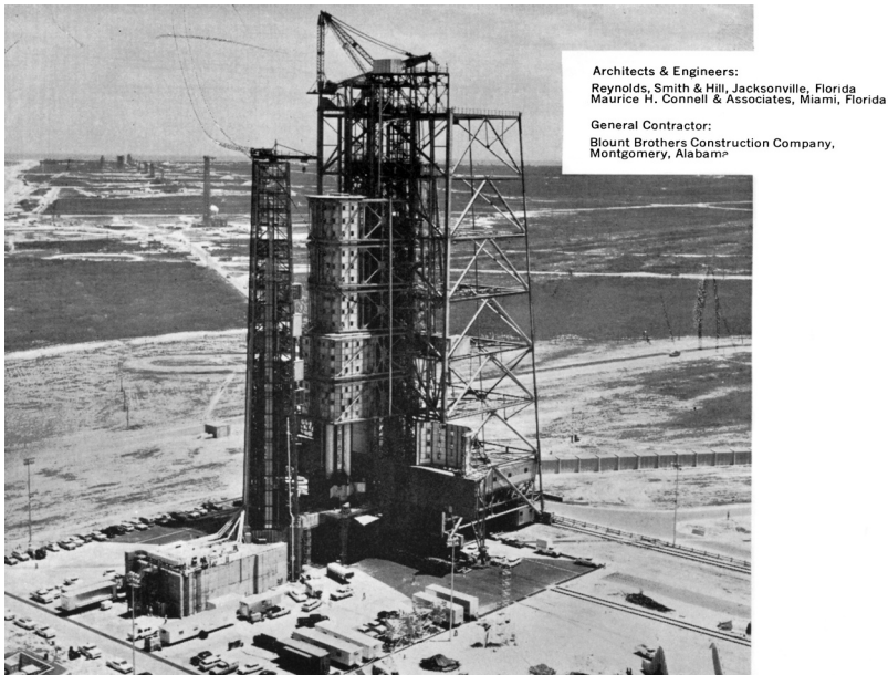
Figure 2.13 Saturn rocket launching facility at Florida. (Courtesy of Vibroflotation Foundation Company brochure.)
