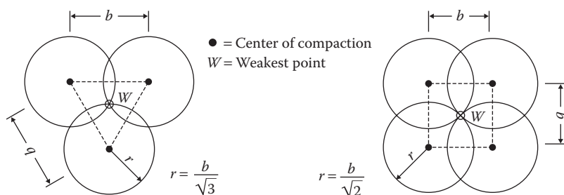
Figure 3.15 Triangular and square compaction patterns.
