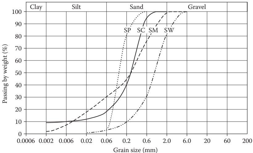
Figure 3.10 Grain size distribution curves of sands (SWV, well-graded, clean sand, fines content <5\% ), SP (poorly graded, clean sand, fines content <5\% ), SM (silty sand, fines content >12\% is mainly silt), and SC (clayey sand, fines content >12\% is mainly clay).
