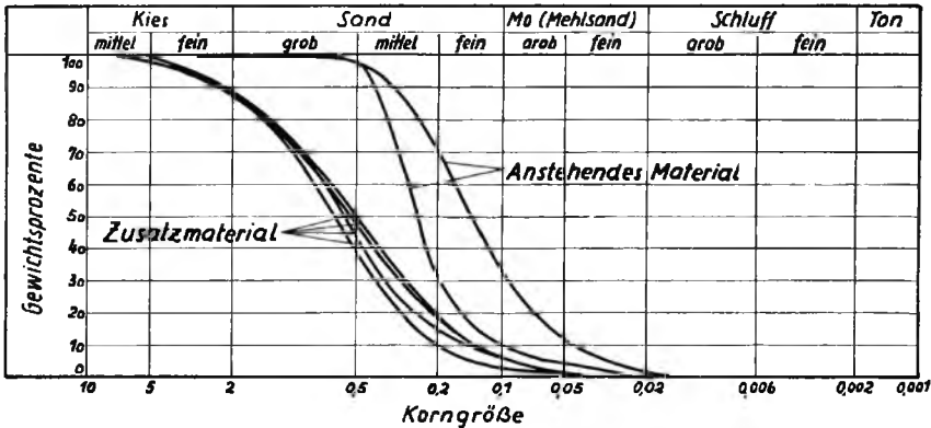
Figure 2.9 Grain size distribution curves for vibro compaction work at Rilinghетен, Norway. Note: Gewichtsprozente—percent by weight, Korngröße—grain size in mm, Zusatzmaterial—added material, Anstehendes Material—in-situ material. (Courtesy of Keller Group plc, London, UK.)
