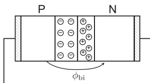
FIGURE 6.11 Short-circuited p-n junction.
