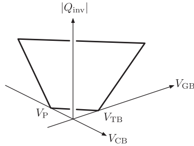
FIGURE 7.23 Dependence of the absolute value of inversion charge, |Q_{\text{inv}}| , on V_{\text{GB}} and V_{\text{CB}} .
