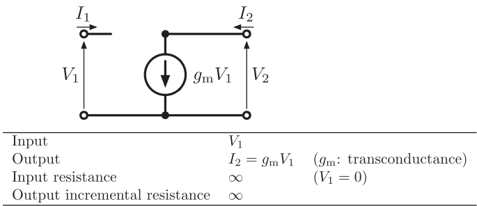
FIGURE 2.15 Voltage-controlled current source.
