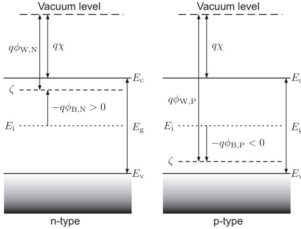
FIGURE 6.5 The work function and electron affinity of a semiconductor.
