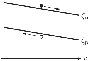
FIGURE 5.3 Directions of movement of electrons and holes with respect to quasi-Fermi level gradients.
