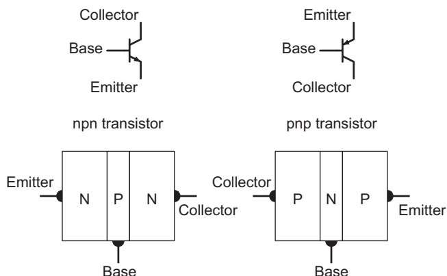
FIGURE 2.19 Schematic symbols and structures of npn and pnp bipolar transistors.
