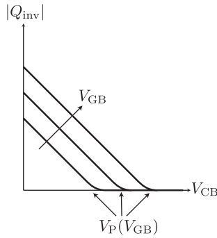
FIGURE 7.22 Controlling the inversion charge Q_{\text{inv}} by the channel potential V_{\text{CB}} .
