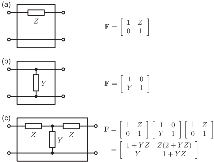
FIGURE A.3 Examples of ABCD matrices. Z is impedance. Y is admittance. (a) Series impedance. (b) Parallel admittance. (c) T-network.
