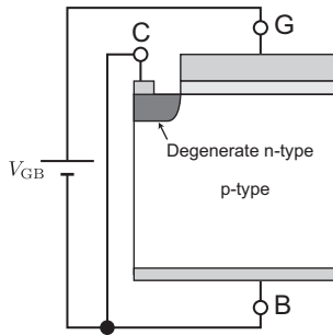
FIGURE 7.18 Three-terminal MOS structure.
