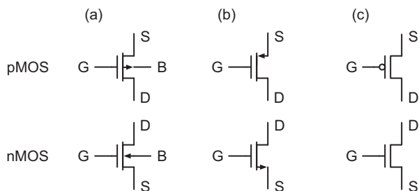
FIGURE 7.2 Schematic symbols of pMOSFET and nMOSFET. (a) Often used by analog circuit designers. (b) The back gate terminal is not drawn. (c) Often used by digital circuit designers.
