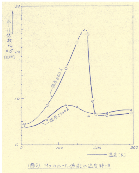
FIGURE 5.9 Temperature dependence of the Hall coefficient of molybdenum films of different thicknesses [38].
