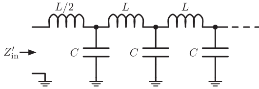
FIGURE 3.8 Infinitely long LC ladder.
