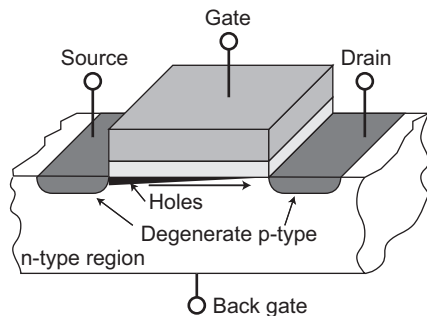
FIGURE 7.4 Structure of a pMOSFET.
