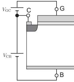
FIGURE 7.24 Channel-terminal-referenced three-terminal MOS structure.
