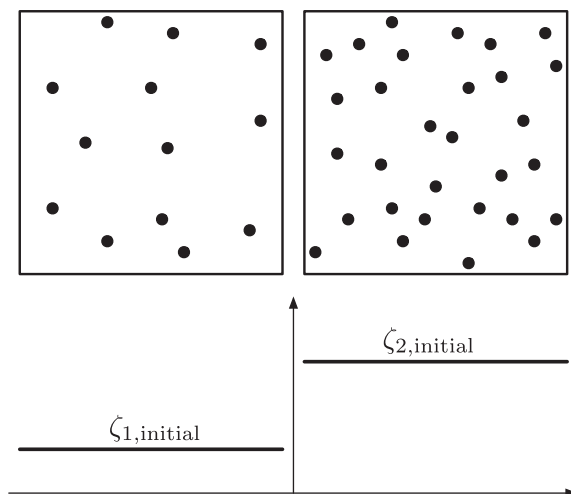
FIGURE 4.10 Two dissimilar metal pieces with electrons.
