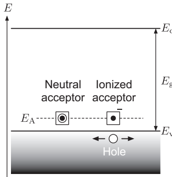
FIGURE 1.18 Acceptor levels in the forbidden band.
