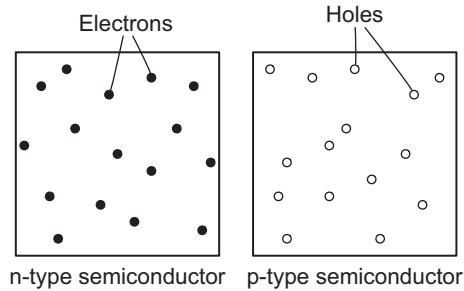
FIGURE 1.1 n-Type and p-type semiconductors. Black-filled circles ( \bullet ) represent electrons. Open circles ( \circ ) represent holes.
