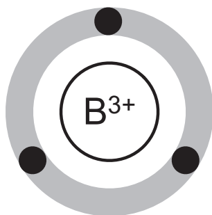
FIGURE 1.14 A model of a boron atom.
