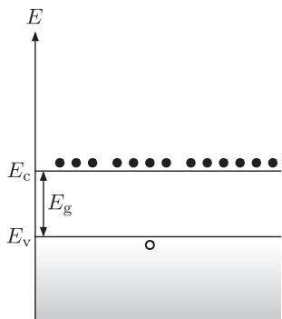
FIGURE 1.11 Carriers in conduction and valence bands of n-type semiconductor.
