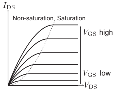
FIGURE 7.6 I_{DS} - V_{DS} characteristics of nMOSFETs.
