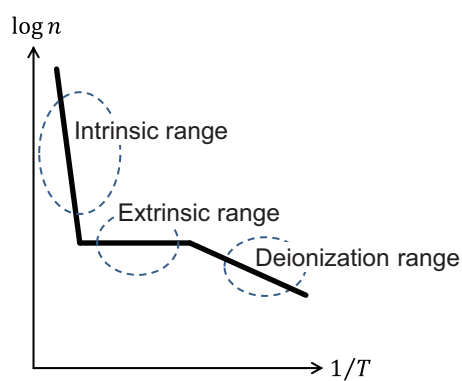
FIGURE 4.14 Approximate log carrier density versus inverse temperature. Three temperature ranges can be identified: intrinsic temperature range, extrinsic temperature range (also known as saturation range), and deionization temperature range (also known as freeze-out range).
