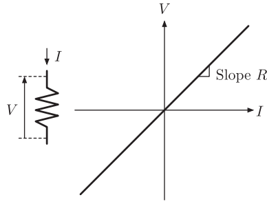
FIGURE 2.1 An element whose characteristics are given by a single straight line passing through the origin in the I - V plane is a linear resistor.
