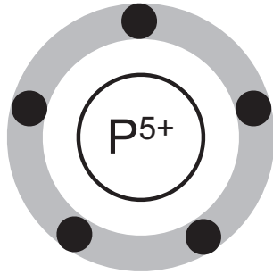
FIGURE 1.9 A model of a phosphorus atom.
