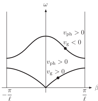
FIGURE 3.17 Example of a dispersion relation of a dispersive medium.
