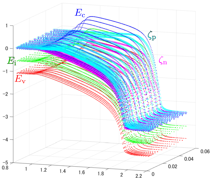
FIGURE 7.32 A TCAD-drawn 3D energy band diagram of an nMOSFET biased into the saturation region. Channel length is 1\text{ }\mu\text{m} . The channel is formed on the near side. The source is on the left-hand side and the drain is on the right-hand side.
