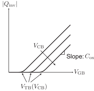
FIGURE 7.21 Controlling the inversion charge Q_{\text{inv}} by the gate voltage V_{\text{GB}} .
