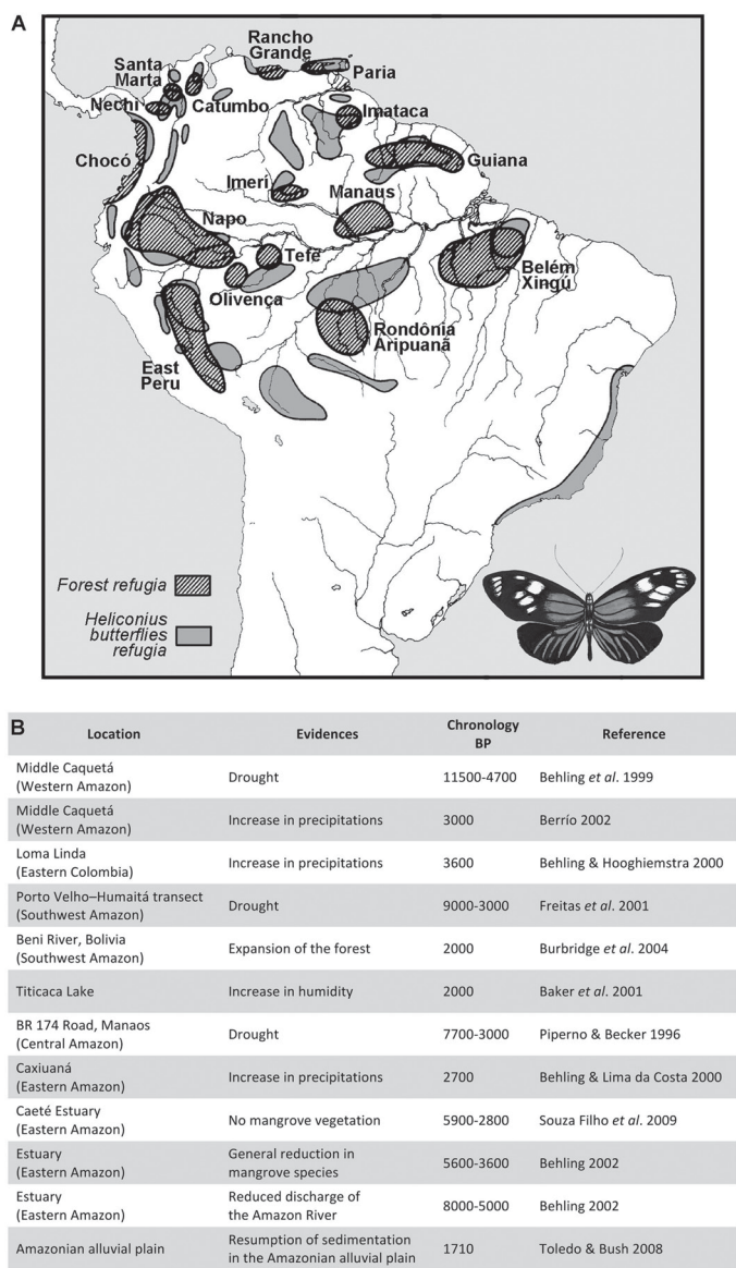
Figure 1.1A–B Part A: Refugia map in Amazonia reconstructed from the modern distributions of plants and Heliconius butterflies suggesting biogeographical probability for fragmentation of the humid forest several times during the Quaternary Period (redrawn from Prance 1973: fig. 24; Brown et al. 1974: fig. 3; Meggers 1979: fig. 1; water painting butterfly, Rostain). Part B: Compilation of some paleoecological studies that indicate climatic changes that occurred during the Middle Holocene in the Amazon Basin (redrawn from Neves 2007: tabl. 1).
