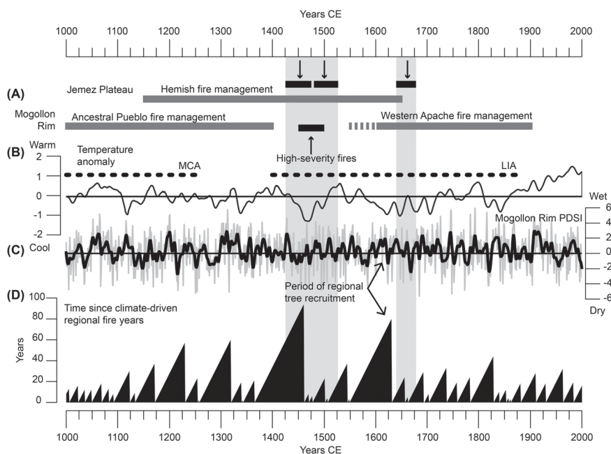
Figure 5.3A–D Synthesis of periods of Native American fire management (deliberate burning, wood harvesting; gray bars in Part A) and high severity fires (black bars in Part A indicated with arrows) in the Mogollon Rim (Roos et al. 2023) and Jemez Plateau areas (Roos et al. 2021) and temperature (Salzer et al. 2014) (Part B) and Palmer Drought Severity records (Cook et al. 2010; Williams et al. 2020) (Part C), and the cumulative duration since climate predicted fire years from Roos and Swetnam (2012) (Part D). Approximate boundaries for the Medieval Climate Anomaly (MCA) and the coldest period of the Little Ice Age (LIA) are marked (Part B). The early 17th century period of regional tree-recruitment associated with prolonged cool, wet conditions and longer fire-free periods is indicated (Part C) and (Part D).
