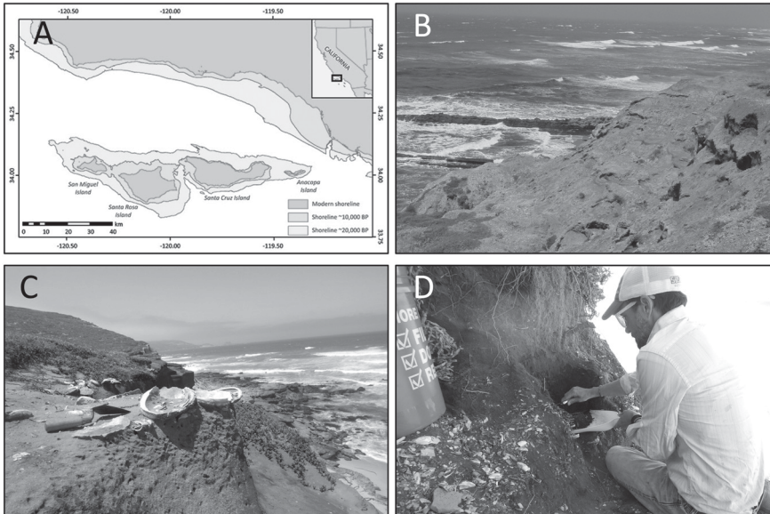
Figure 3.4 Part A: Map of Santa Barbara Channel shoreline changes from 20,000 years ago to present. Part B: Location of approximately 12,000-year-old site, CA-SRI-512. Part C: Red abalone shells at a 7,000-year-old site, CA-SRI-388. Part D: Excavation of a shell midden near Point Conception.
