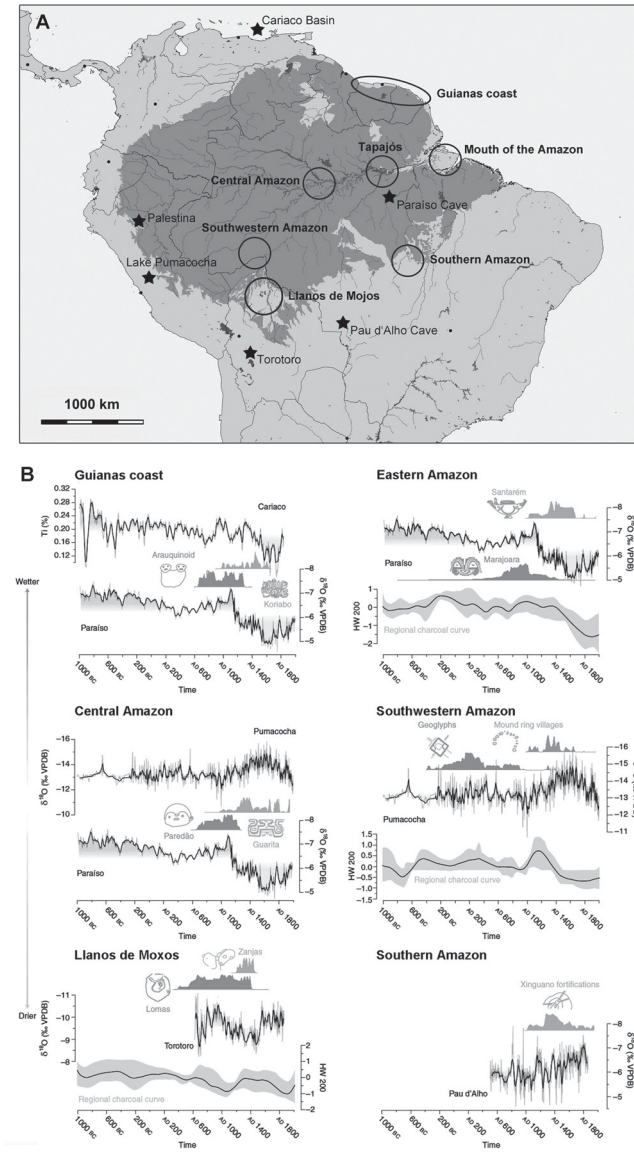
Figure 1.2A–B Part A: Map of the archaeological regions (circles) and paleoecological samples (stars) discussed in the Souza et al. (2019) study (drawing, Rostain). Part B: Periods of cultural change (graphics) and paleoclimate records (curves) for six regions of Amazonia, and regional charcoal curves from the best sampled regions. The duration of each archaeological culture is represented by summed calibrated probability distributions of the radiocarbon dates. The “wetter” and “drier” arrows refer to the interpretation of the paleoprecipitation records (Souza et al. 2019: fig. 3).
