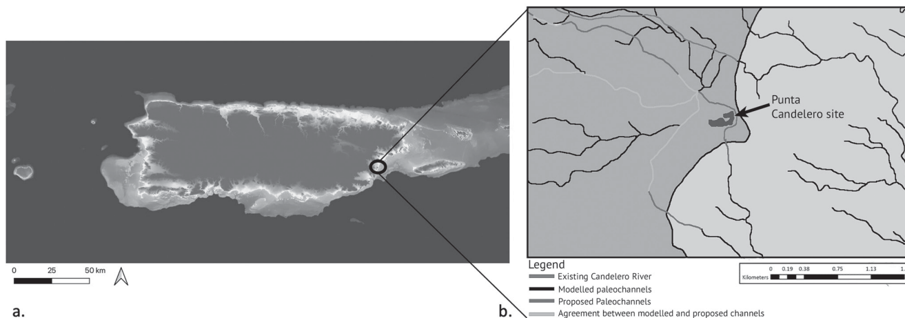
Figure 9.2A–B Landscape transformation after post-Pleistocene sea level rise. Part A: the archipelago of Puerto Rico showing in light blue the areas of the insular shelf that would have been dry land during times of lower sea level. Part B: the location of Punta Candelerio site on the east side of Borikén. The analysis of the local topography and bathymetry demonstrate the existence of paleochannels that extend under water and suggest that this landscape today is dramatically different from the one experienced by the inhabitants of Candelerio between 480 and 1100 AD.
