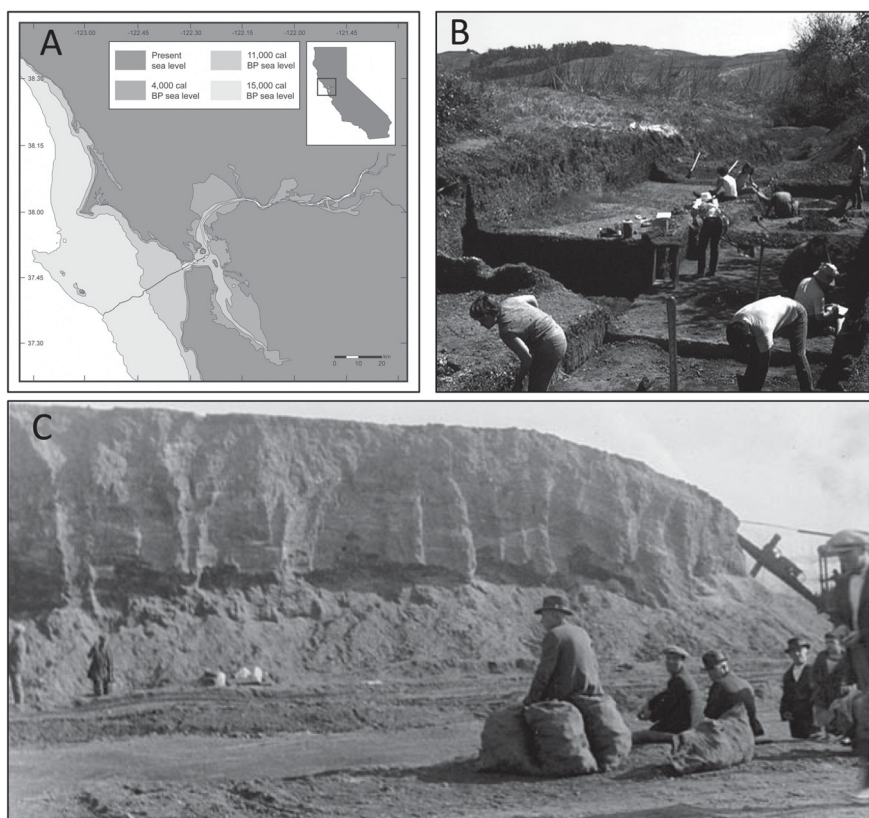
Figure 3.3 Part A: Map of sea level change in the San Francisco Bay Area from 15,000 years ago to modern times. Part B: Excavation of the Patterson Mound, CA-ALA-328. Part C: Destruction of the Emeryville shell mound (CA-ALA-309) in 1924.
