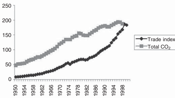
Figure 17.2 Relationship between increase in world trade and global carbon dioxide emission.
