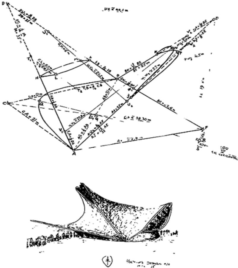
Figure 18. Le Diatope : Technical drawing and sketch of the architectural design.
