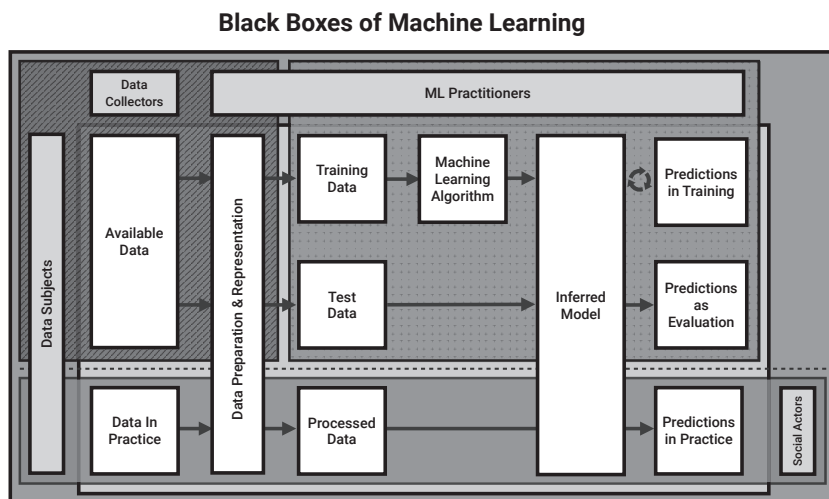
Figure 5.2. Three black boxes of machine learning, extending on ML models of Heuer (2020) and Veale (2019).
