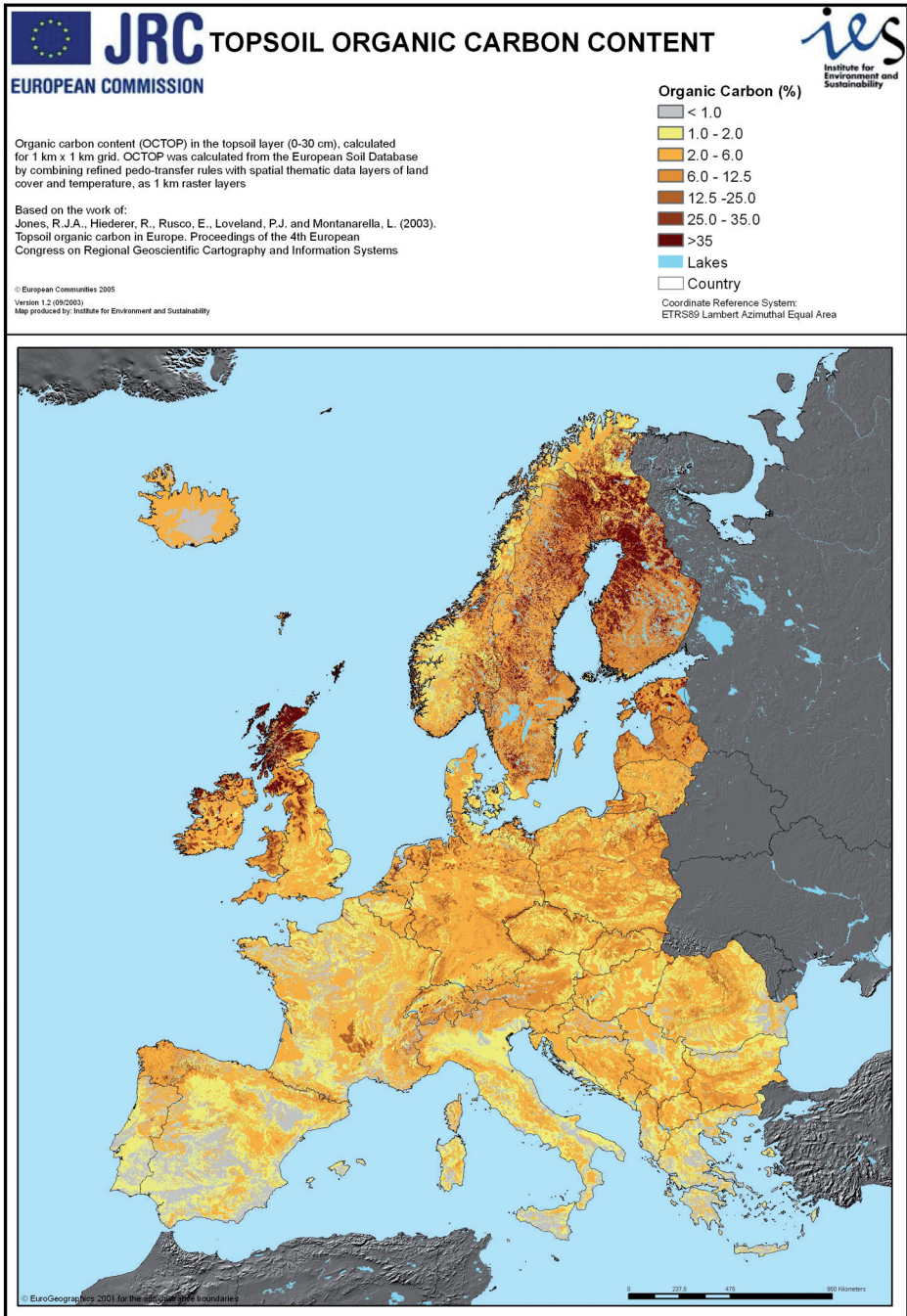
Figure 43. Organic carbon content (%) in the surface horizon of soils in Europe. Source: http://eussoils.jrc.ec.europa.eu/esdb_archive/octop/octop_download.html European Commission – Joint Research Centre, Institute for Environment and Sustainability. © European Union.
