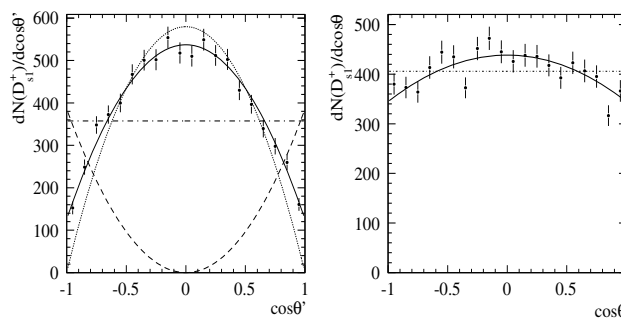
Figure 19.3.25. From (Lees, 2011d). Left: Efficiency-corrected D_{s1}(2536)^+ signal yield as function of D^{*+} decay angle \theta' . Lines correspond to the following hypotheses fitted to the data: J^P = 1^+, 2^-, 3^+, \dots with S - and D -wave (solid); 1^+, 2^-, 3^+, \dots with S -wave only (dash-dotted); 0^- (dashed); 1^-, 2^+, 3^-, \dots (dotted). 0^+ is forbidden. Right: Efficiency-corrected D_{s1}(2536)^+ signal yield as function of D_{s1}(2536)^+ decay angle \theta . Assuming J^P = 1^+ , the data are fitted with hypotheses of pure S -wave (dotted line); S - and D -wave (solid line) D_{s1}(2536)^+ decays.
