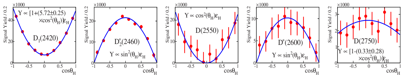
Figure 19.3.12. From (del Amo Sanchez, 2010i). Distribution in \cos \theta_H for each signal observed in the D^{*+}\pi^- final state. The error bars include statistical and correlated systematic uncertainties. The curve is a fit using the function Y shown in the plot; \epsilon_H is the efficiency as a function of \cos \theta_H .
