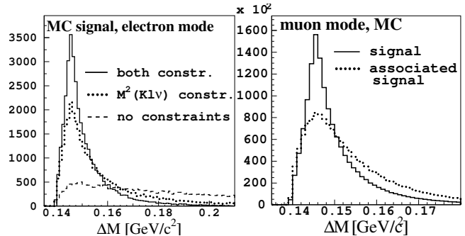
Figure 19.2.22. Left: The effect of the kinematic constraints on the \Delta M distribution of the simulated D^0 \rightarrow K^-\ell^+\nu_\ell decays. Right: \Delta M distribution for simulated associated signal events (see text for the explanation). From (Bitenc, 2008).
