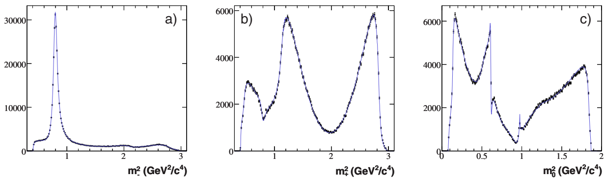
Figure 19.1.22. From (Aubert, 2008l). D^0 \rightarrow K_S^0 \pi^+ \pi^- Dalitz plot projections from D^{*+} \rightarrow D^0 \pi^+ events on (a) m_-^2 , (b) m_+^2 , and (c) m_0^2 . The curves are the reference model fit projections.
