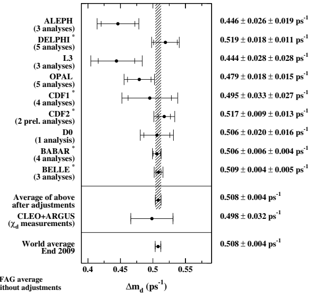
Figure 17.5.6. The B^0\bar{B}^0 oscillation frequency \Delta m_d as measured by the different experiments along with their average. Averages are also given separately for the time-dependent measurements by the B Factories and the LEP and Tevatron experiments, and the time-integrated measurements by CLEO and ARGUS (Asner et al., 2010).
