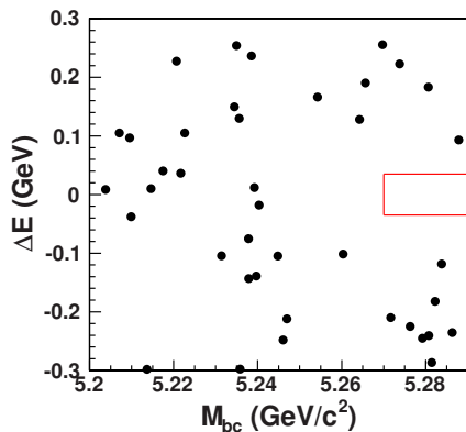
Figure 17.11.10. (\Delta E, m_{ES}) distribution of B^+ \rightarrow D^-\mu^+\mu^+ candidates from (Seon, 2011). The solid red line denotes the signal region.
