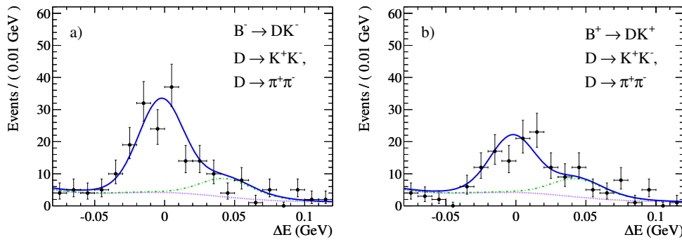
Figure 17.8.2. \Delta E projections of the fits to the B^\pm \rightarrow D_{CP}K^\pm candidates selected in the full BABAR data sample (Aubert, 2008o), split into subsets of definite charge of the B candidate: a) B^- \rightarrow D_{CP}K^- , and b) B^+ \rightarrow D_{CP}K^+ . The curves are the full probability density function (solid, blue), and B^\pm \rightarrow D\pi^\pm (dash-dotted, green) stacked on the remaining backgrounds (dotted, purple). The region between the solid and the dash-dotted lines represents the B^\pm \rightarrow DK^\pm contribution. We show the subset of the data sample in which the track from the B decay is identified as a kaon and a signal-enriching selection is applied to the other variables used in the fit ( m_{ES} and \mathcal{F} ).
