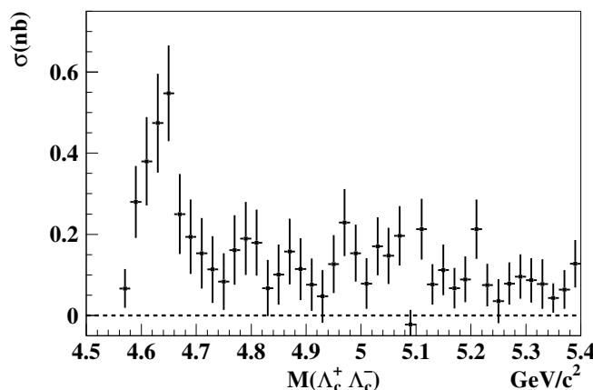
Figure 21.4.10. The exclusive cross section for e^+e^- \rightarrow \Lambda_c^+\Lambda_c^- measured by Belle (Pakhlova, 2008b).
