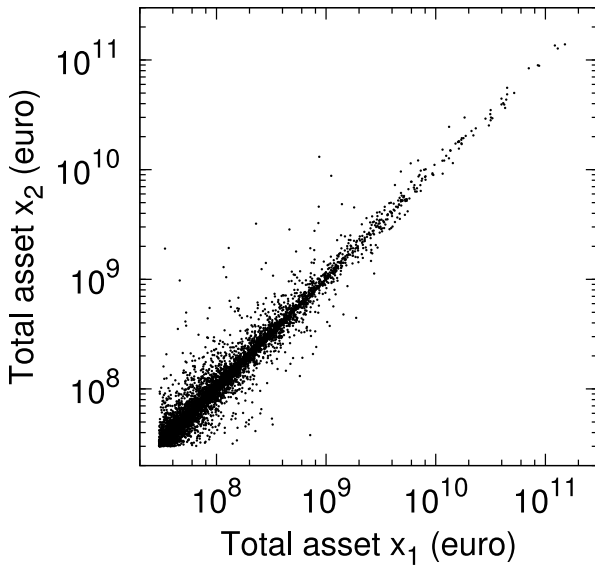
Fig. 4. Scatter-plot of the firms in France whose firm size (total-assets) exceeds a certain threshold in both 2000 and 2001
