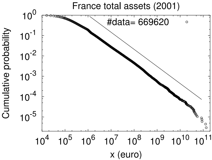
Fig. 2. Cumulative probability distribution of firm size (total-assets) in France in the year 2001. Data consist of 669,620 firms, which are exhaustive in the sense that firms exceeding a threshold are all listed. The line corresponds to \mu = 0.84 in (1). Reproduced from [1].
