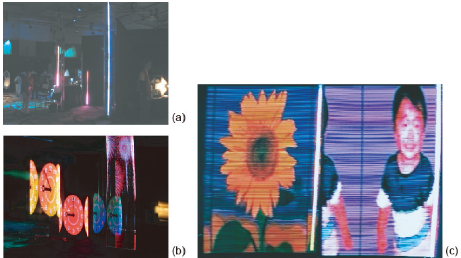
Fig. 2. Perceived image with observer's eyes static (a). Two LED columns 1.8 m in height and one LED column 4 m in height are shown in this photo. An example of perceived images displayed with Saccade-based Display (b). Life-size photographic images can be presented (c). The images are 128 pixels in vertical and horizontal resolutions with 4-bit color depth. Images (b) and (c) were taken with a slow-shutter rotating camera.
