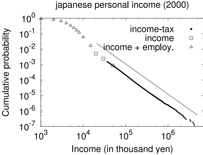
Fig. 1. Cumulative probability distribution of Japanese personal income in the year 2000. The line is simply a guide for eyes with \mu = 1.96 in (1). Note that the dots are income tax data of about 80,000 taxpayers. Reproduced from [1].
