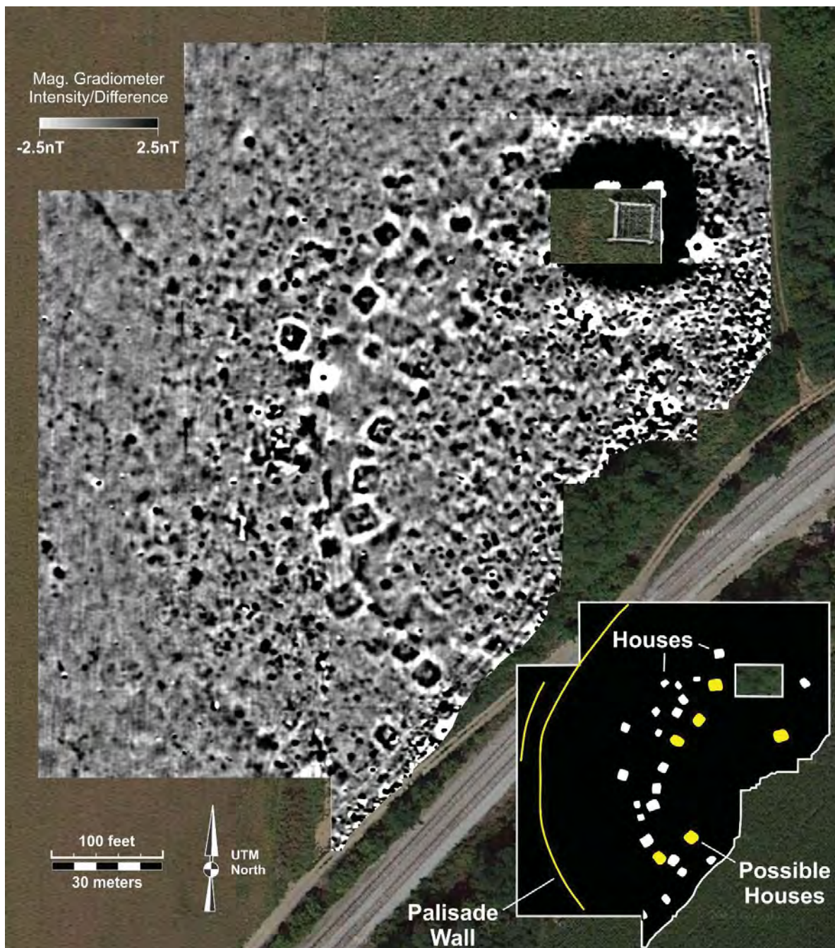
Fig. 3. Magnetic gradiometer data from the Guard site, in southeast Indiana near Lawrenceburg.
