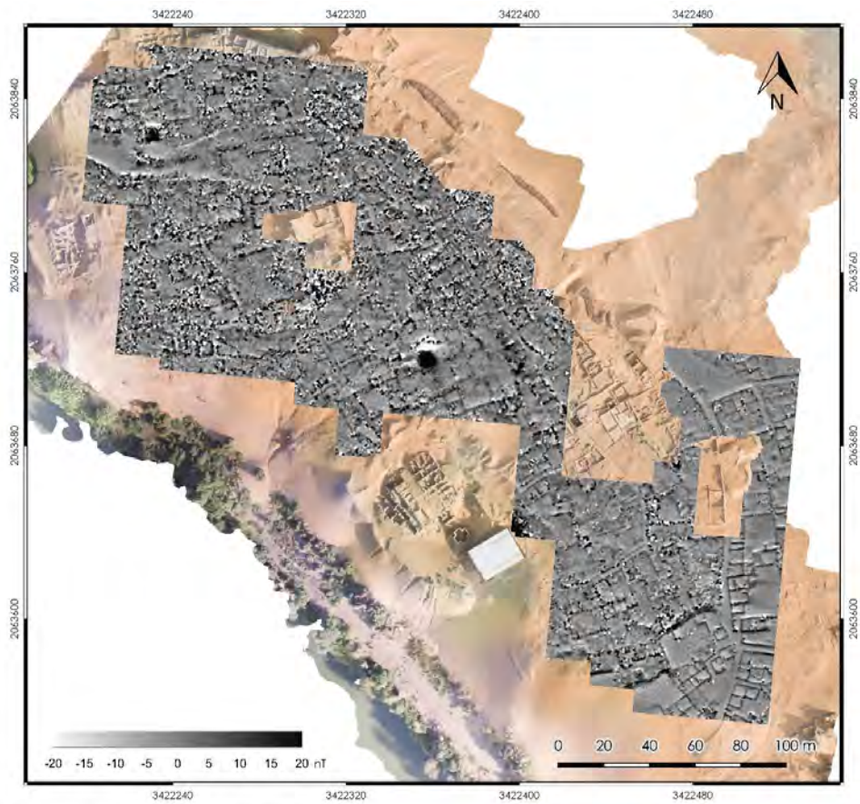
Fig. 3. Old Dongola, citadel. Magnetic map on a vertical aerial photograph of the citadel.
