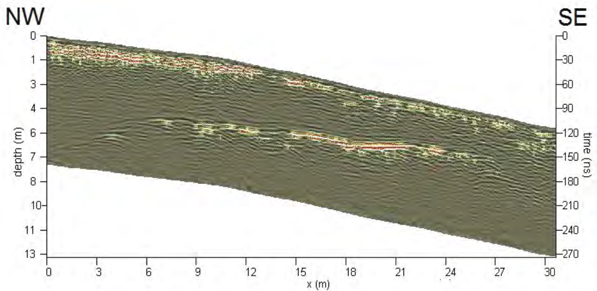
Fig. 2. GPR profile showing a high amplitude reflection that corresponds to the ceiling of an air-filled cave.
