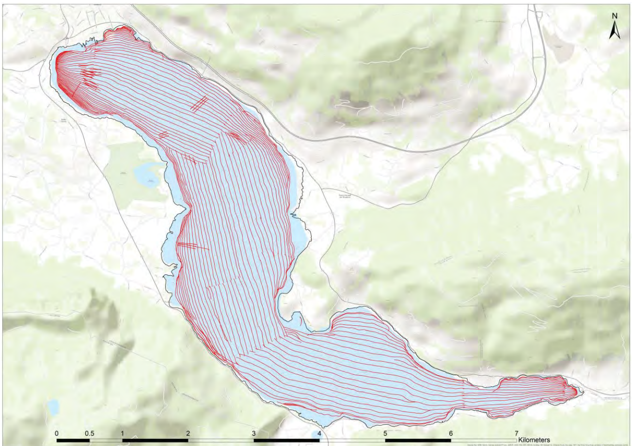
Fig. 1. Position and distribution of survey swaths of the multi-beam sonar measurements on Lake Mondsee (total length 304km).
