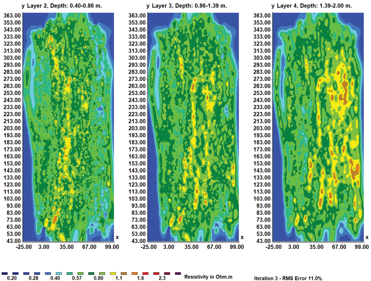
Fig. 3. Area covered with 3-D electrical resistivity tomography (red polygon) and the individual dynamic ERT lines during 2018 field season in Lambayanna (top). Horizontal depth slices extracted from the 3-D robust resistivity inversion model from Lambayanna using the dynamic dipole-dipole measurements (bottom).
