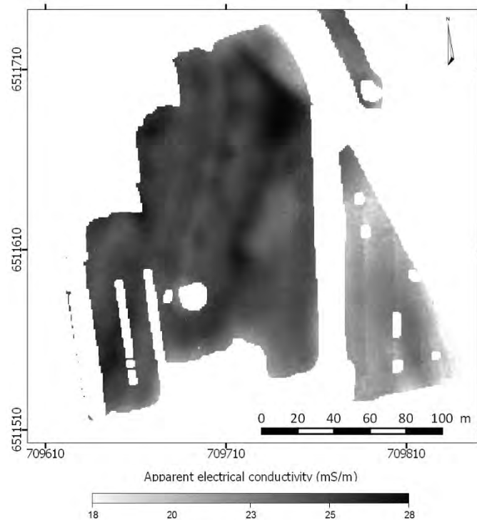
Fig. 3. Apparent electrical conductivity map of the central area of the site.
