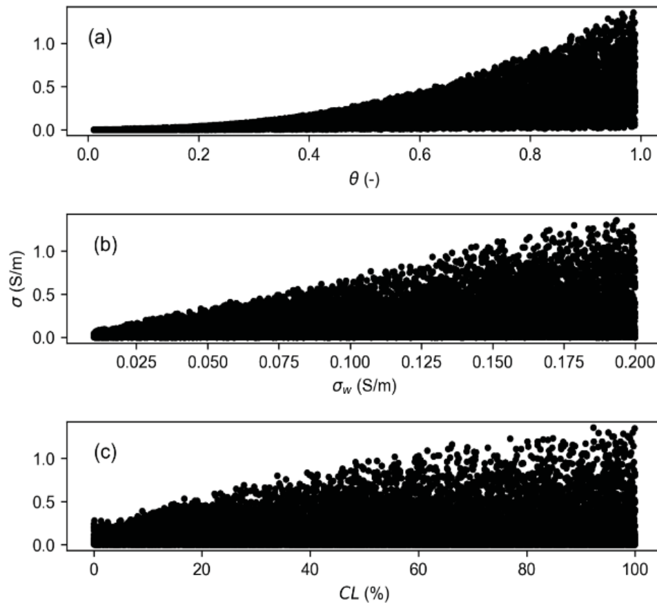
Fig. 1. Monte-Carlo (random uniform) sampling (15,000 samples) of the Generalized Archie's Law (Eq. 1). The soil's bulk electrical conductivity \sigma (S/m) is expressed in function of (a) the volumetric moisture content \theta (-), (b) the electrical conductivity of the pore solution \sigma_w (S/m) and (c) the clay content CL (%).
