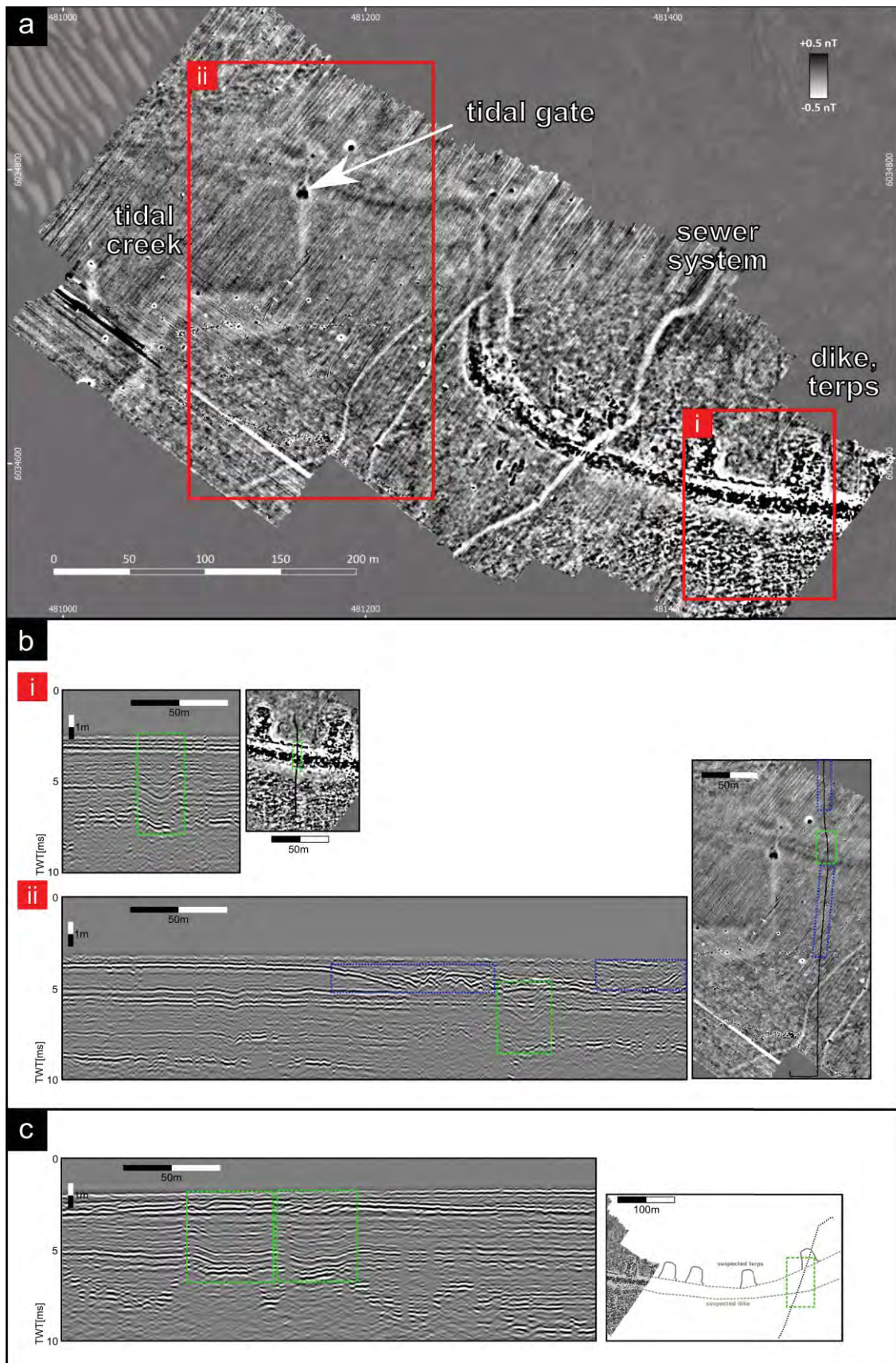
Fig.2. (a) Magnetic anomaly map of study area 1. Several features like the dike, terps, the tidal gate and sewer systems can be identified. (b) Close-up of two selected areas and comparison with seismic profiles. In close-up (i) the imprint of the former dike is seen as trough-shaped reflector, marked in green. In close-up (ii) the seismic profile shows the former tidal creek (blue) and the dike's imprint. (c) A seismic profile further to the east crossing a dike and terp, characterized again as trough shaped reflectors.
