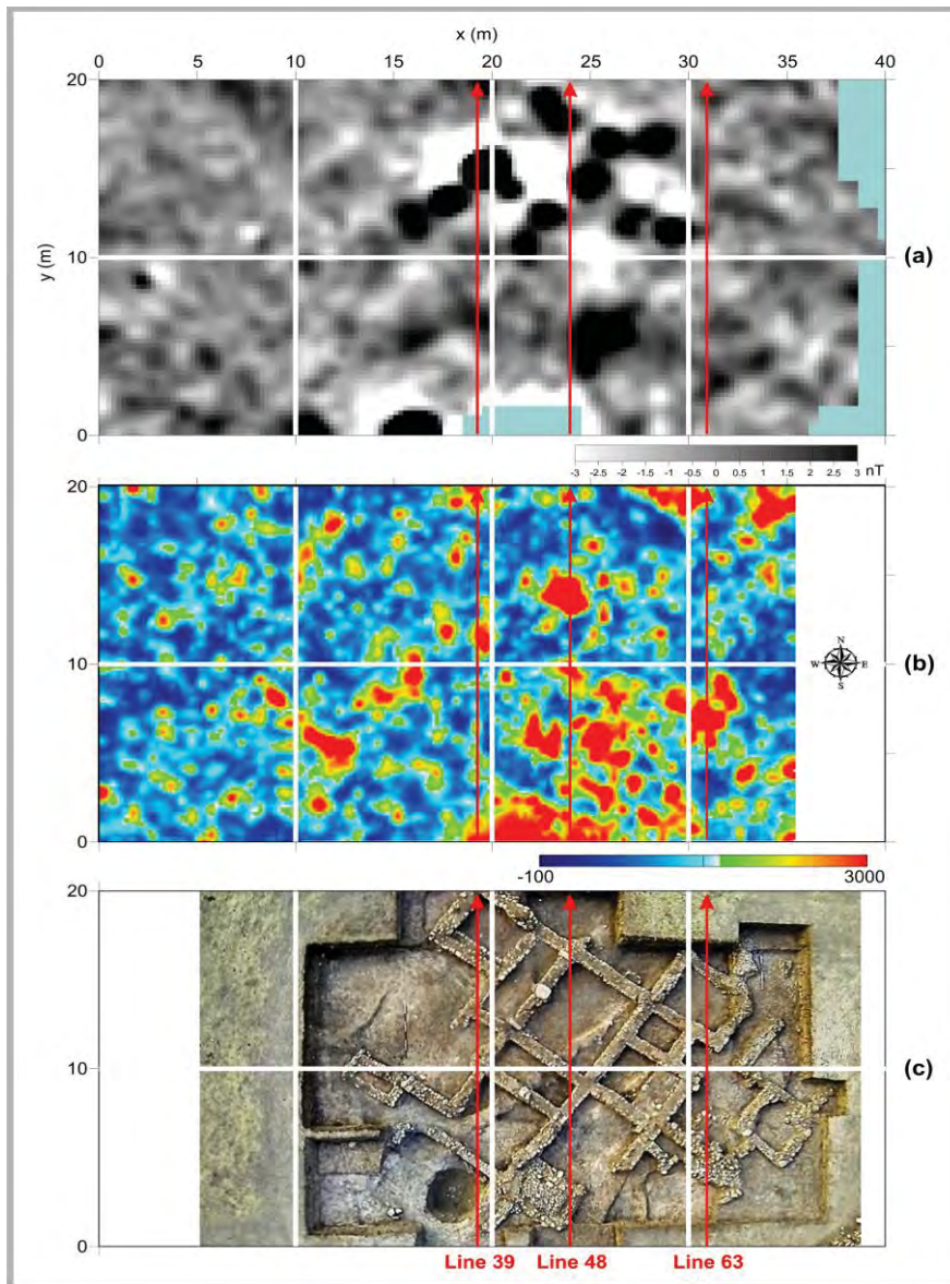
Fig. 1. (a) Magnetic gradiometry image, (b) GPR depth slice of 0m-2m and (c) aerial photo of excavated part of the workshop area.
