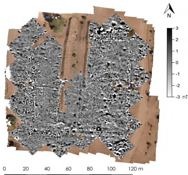
Fig. 2. Hosh el-Kab magnetometry results. Data collected with a Geoscan Research FM256. Sampling grid 0.25m x 0.5m. (Data processing by Robert Ryndziewicz; orthophotomosaic by Mariusz Drzewiecki).
