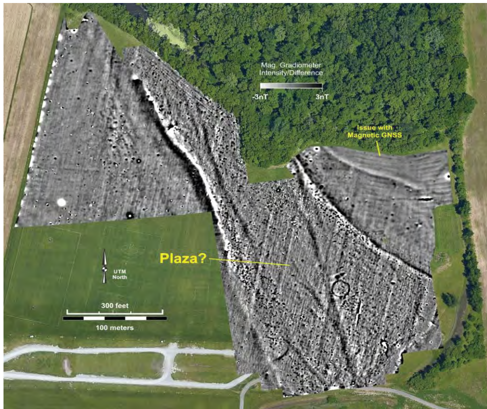
Fig. 1. Magnetic gradiometer data from the Hahn Village site, near Cincinnati, Ohio.
