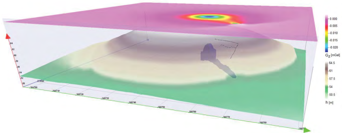
Fig. 1. Results from the synthetic density modelling - a 3D view of the Newgrange passage tomb together with the modelled passageway/chamber structure and its simulated gravitational anomaly for measurements that would be made on the top surface of the mound.
