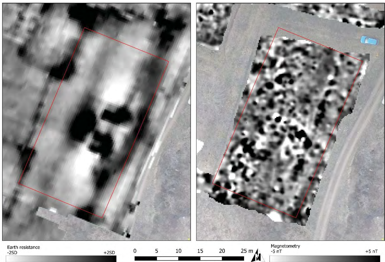
Fig. 2. Polygon 1 (marked with red line) over visualisations of the earth resistance (left) and magnetometry (right).
