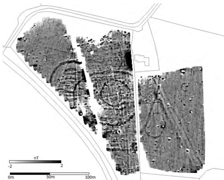
Fig. 2. Magnetometer data of the enclosure at Ranelagh along the N61 Coolteige Road Project, County Roscommon.
