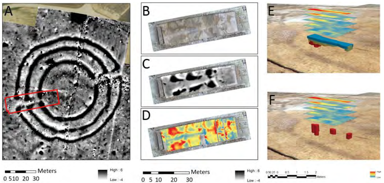
Fig. 2. Topsoil magnetometry survey (A), and surveys after the removal of the topsoil: aerial photo (B), magnetometry (C), magnetic susceptibility (D), and detailed magnetic susceptibility survey of the palisade showing the outline (E), and postholes (F).
