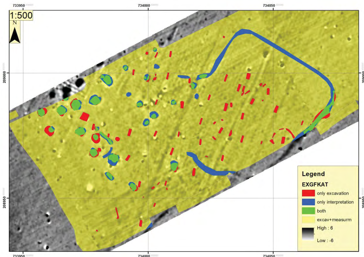
Fig. 2. Results of overlapping interpretation and excavation feature polygons.
