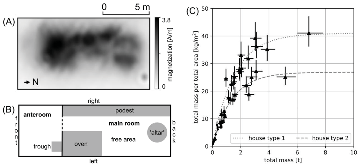
Fig. 3. Example results of the interpretation scheme. (A) Magnetization distribution for one unexcavated building in comparison to the schematic floor plan (B) (after Chernovol 2012). Note that areas of increased magnetization can match to the location of the immovable inventory. (C) Estimated masses of unexcavated buildings with a tentative interpretation of two different types of houses.
