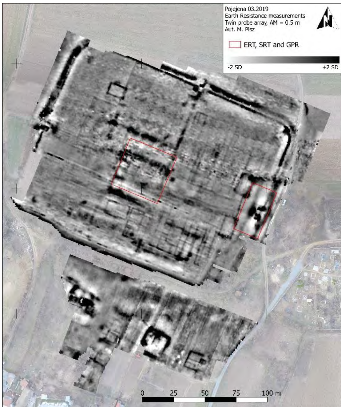
Fig. 1. Earth resistance results. Twin probe array, AM = 0.5m. Polygon 1 and Polygon 2 are outlined with red line.
