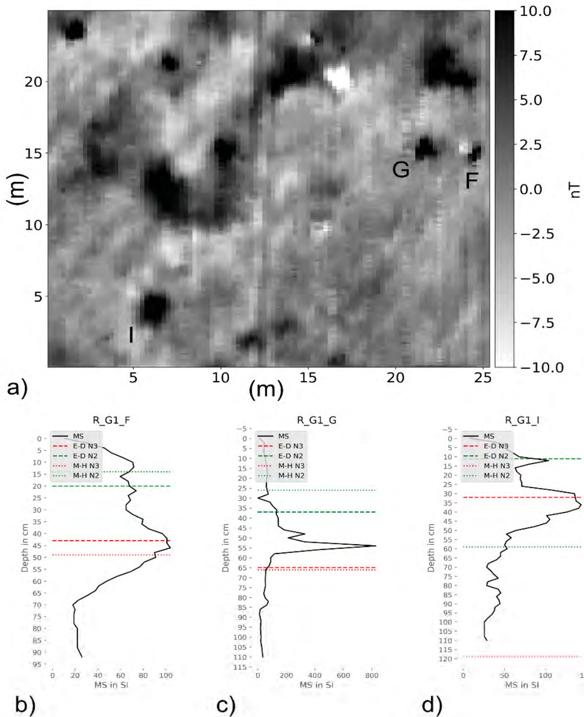
Fig. 1. (a) Shows a subset of the lower sensor survey at Runion, Tennessee with three features indicated G, F, and I. (b), (c), and (d) Black line shows the down-hole magnetic susceptibility compared to Multi-height (short dash) and Euler deconvolution (long dash) depth estimates using a structural index of two (green) and three (red), for features F, G, and I respectively.
