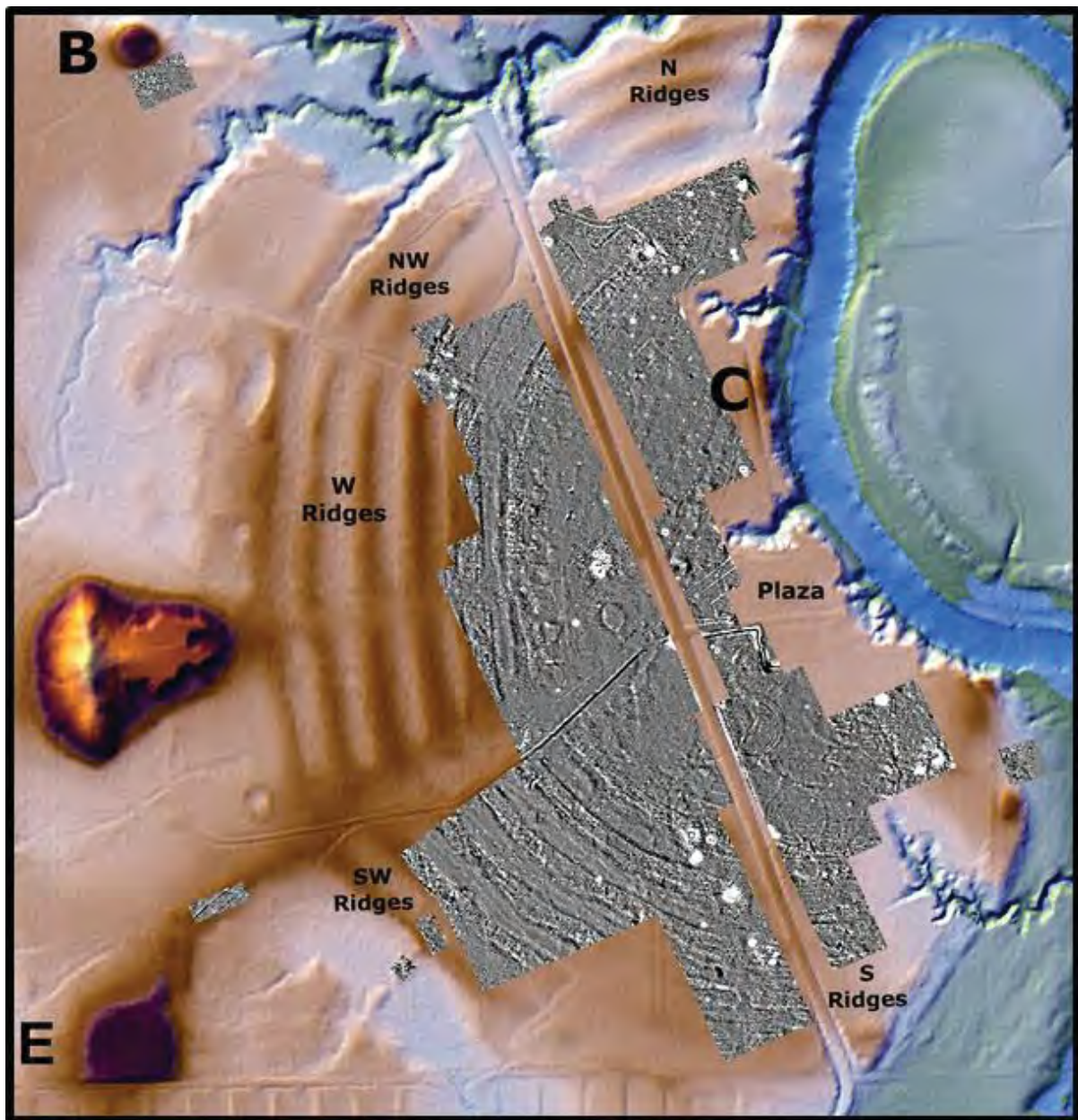
Fig. 2. Results of the magnetic gradient survey at Poverty Point. Note circles in and near the plaza and negative and positive linear anomalies associated with each concentric ridge.
