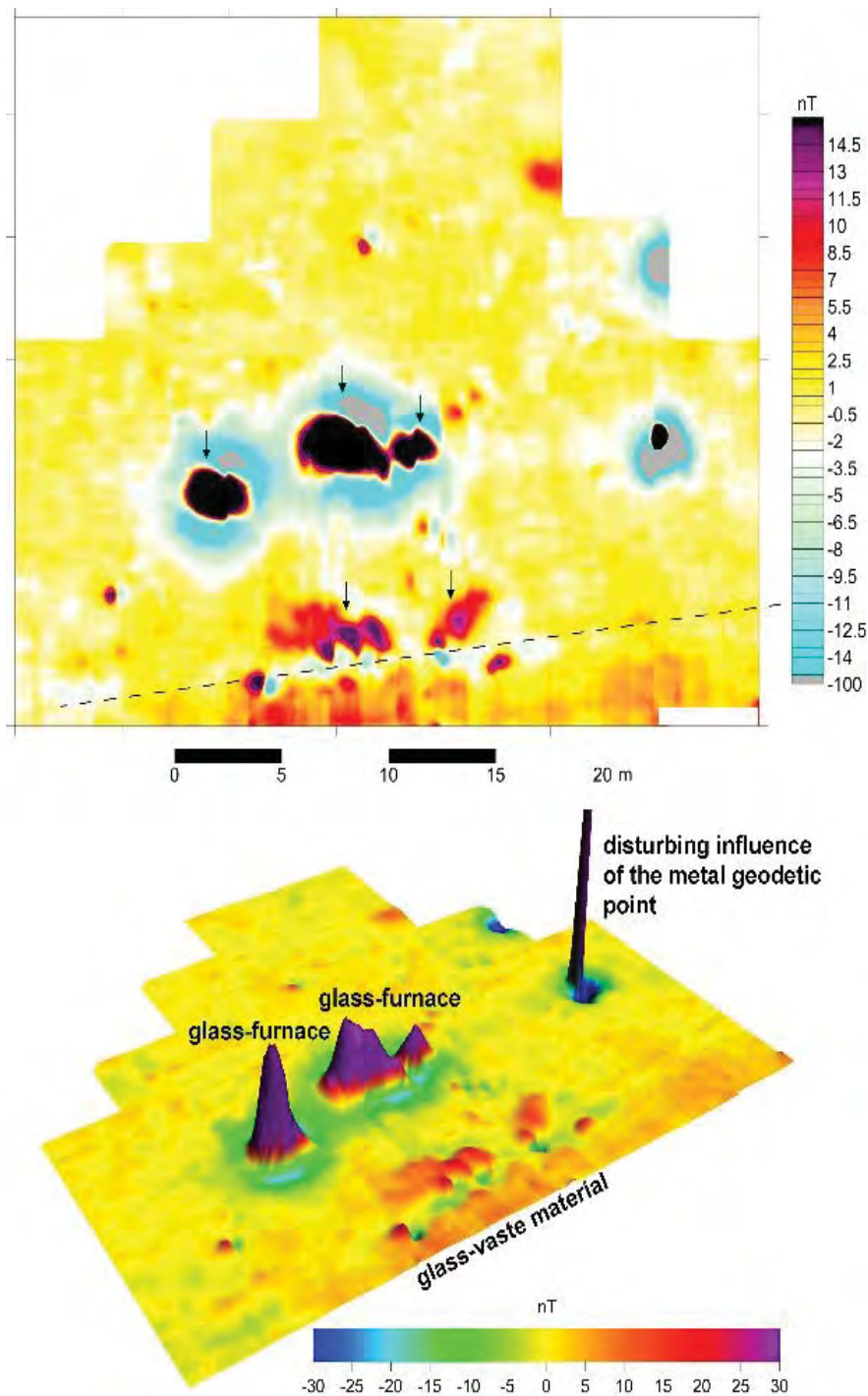
Fig. 2. Boč, Karlovy Vary district. The separation of two glass furnaces and the remains of a destroyed glass waste heap at the abandoned medieval glass-working site (dotted line – the edge of the deserted ravine road; survey: Křivánek 2017; surveyed area: approx. 25m x 20m).
