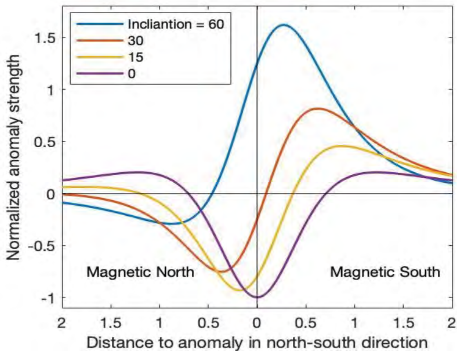
Fig. 2. Anomaly strength of the total field intensity as north-south traverse through the anomaly's centre for different inclinations. Horizontal and vertical component in units of burial depth. After Mike Tite (1966: 26).
