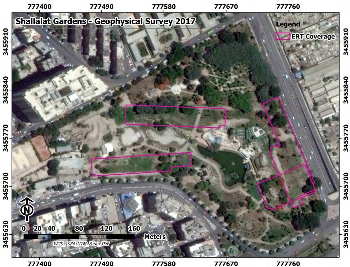
Fig. 1. Area coverage with ERT in Shallalat Gardens during the 2017 field campaign.
