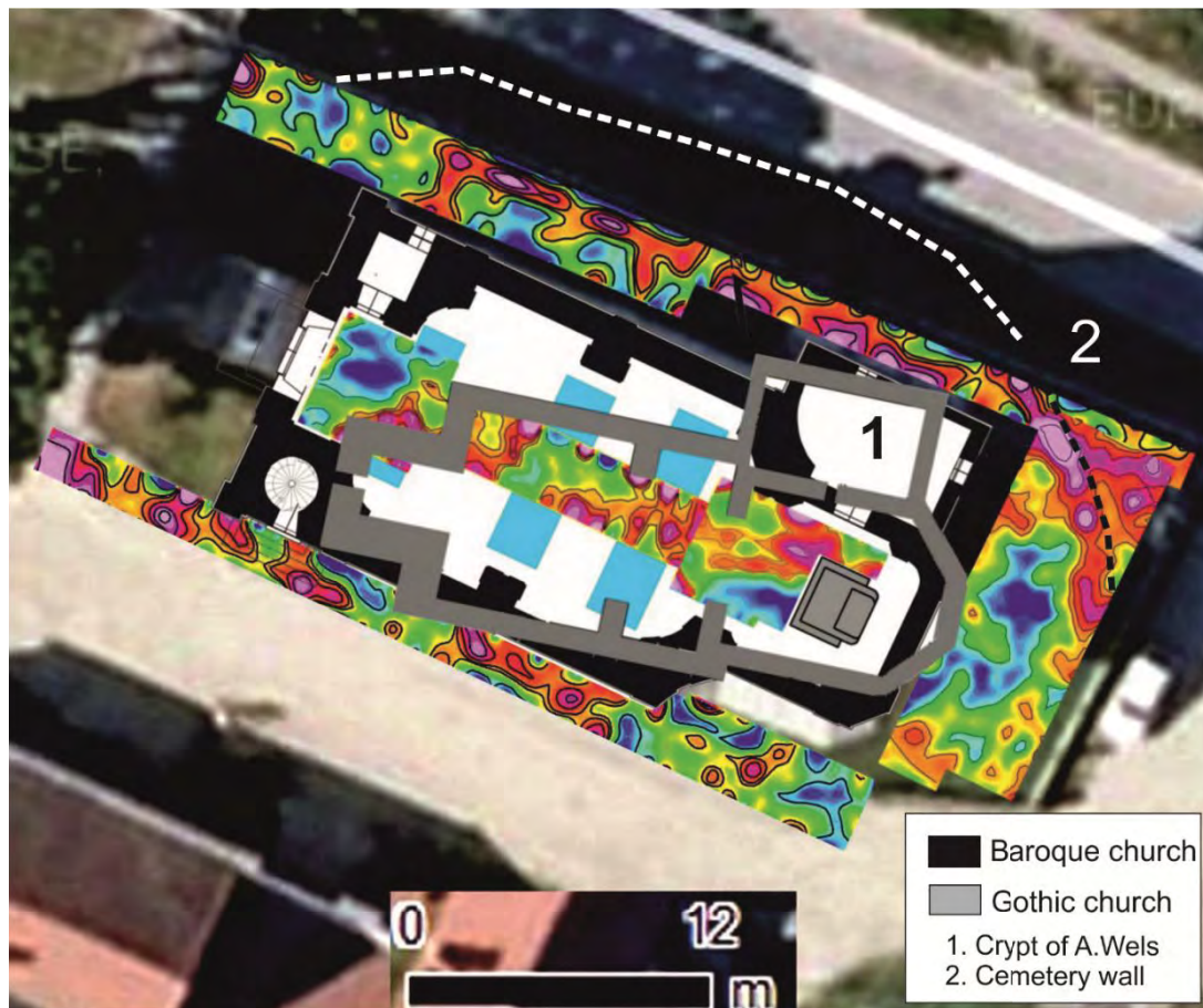
Fig. 1. Kovarce, St. Nicolas Church. The results of geophysical measurement - horizontal slides, depth 80-120cm. The Baroque church (black) and the foundations of the Gothic church (grey).
