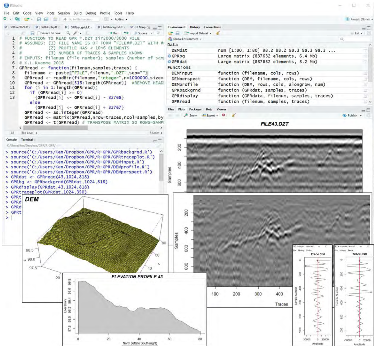
Fig. 2. Screen shot from RStudio showing various windows with R language code, command lines, defined functions, and output graphics depicting GPR and DEM findings.
