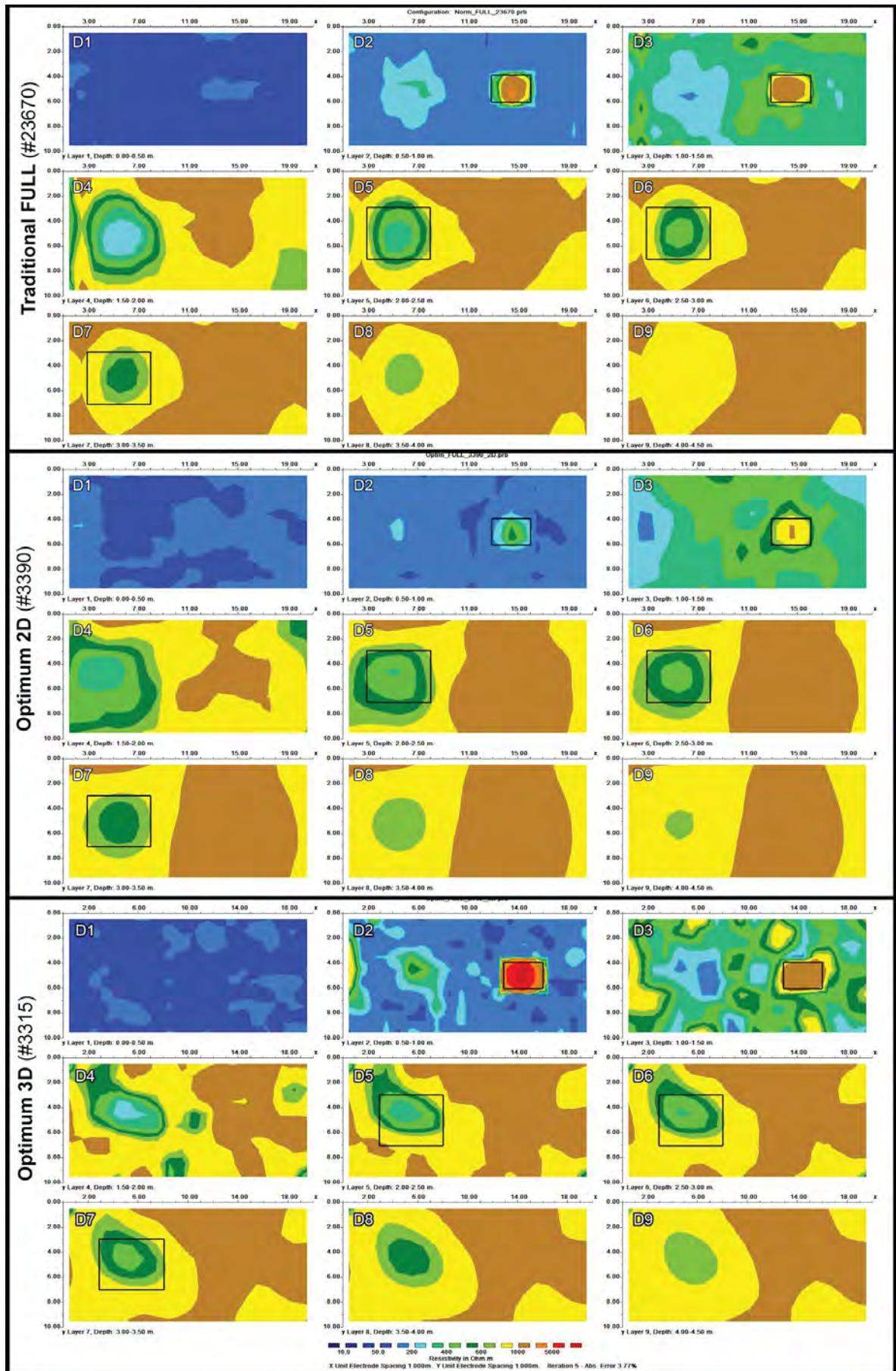
Fig. 2. Inversion results with Traditional dataset, Optimum 2-D and Optimum 3-D.
