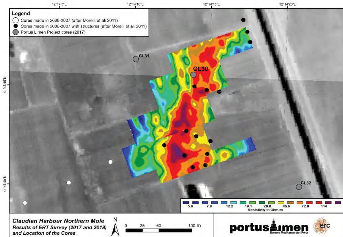
Fig. 3. Results of the ERT survey, the location of the 2006-2007 cores and the new 2017 cores.
