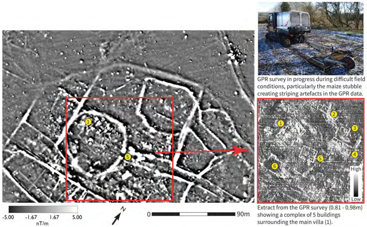
Fig. 2. Extract from the magnetic survey showing a complex multi-phase landscape including two IA banjo enclosures. The scheduled villa (1) is located within the larger banjo enclosure and one building (5) appears to be built over the entrance to the enclosure on the alignment of the approach ditches. Additional building remains were revealed by the targeted GPR survey (inset bottom right).
