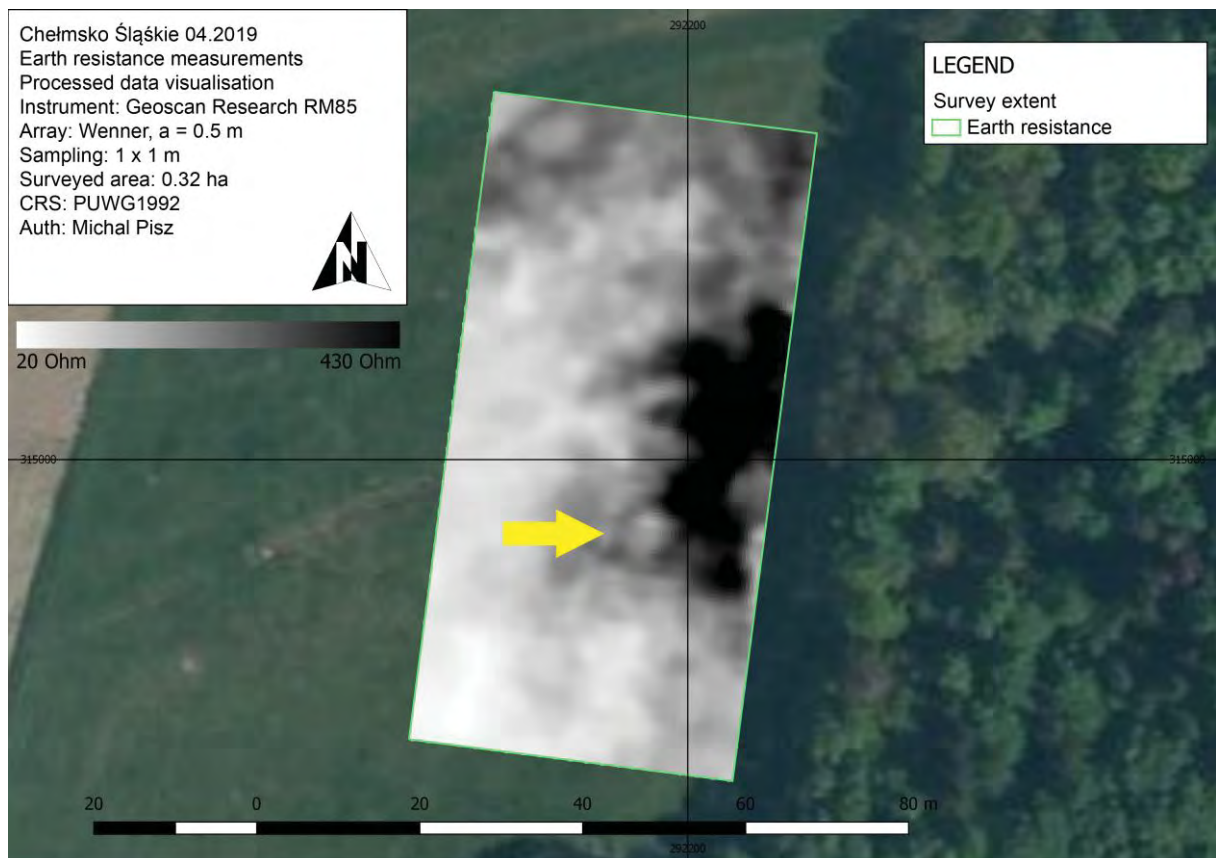
Fig. 2. Earth resistance survey. A round high resistance anomaly (marked by a yellow arrow) was initially interpreted as the possible remains of a gallows.
