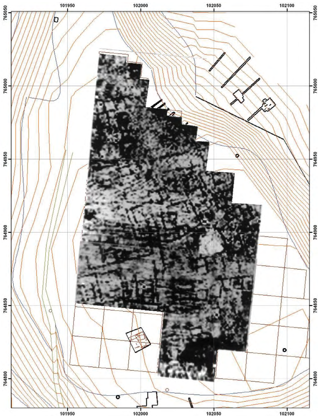
Fig. 1. The ancient ruins comprise resistive structures buried in a relatively conductive environment, creating high resistance anomalies which are mapped by geophysical prospecting. The subsurface resistance has been mapped and its distribution is depicted in a greyscale. The darker tones indicate areas of high resistance which are presumably caused by the concealed ancient ruins. The example has been drawn from the exploration of the site hosting the ruins of the ancient city “Europos” in northern Greece (Tsokas et al. 1994). The closed rectangular anomalies, reflecting the presence of remnants of foundation walls, form a plan view showing the shape of the ancient urban complex.
