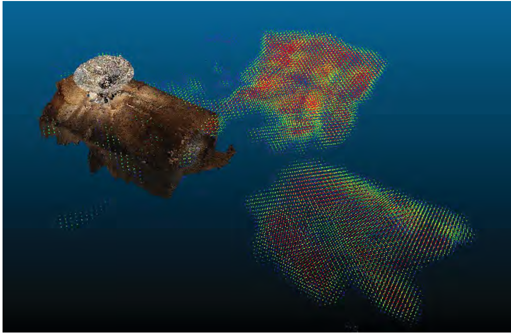
Fig. 2. Combined visualisation of the 3D point-clouds derived from IBM and GPR data, with the GPR reflection amplitude expressed by different colours (blue=25, red=78).
