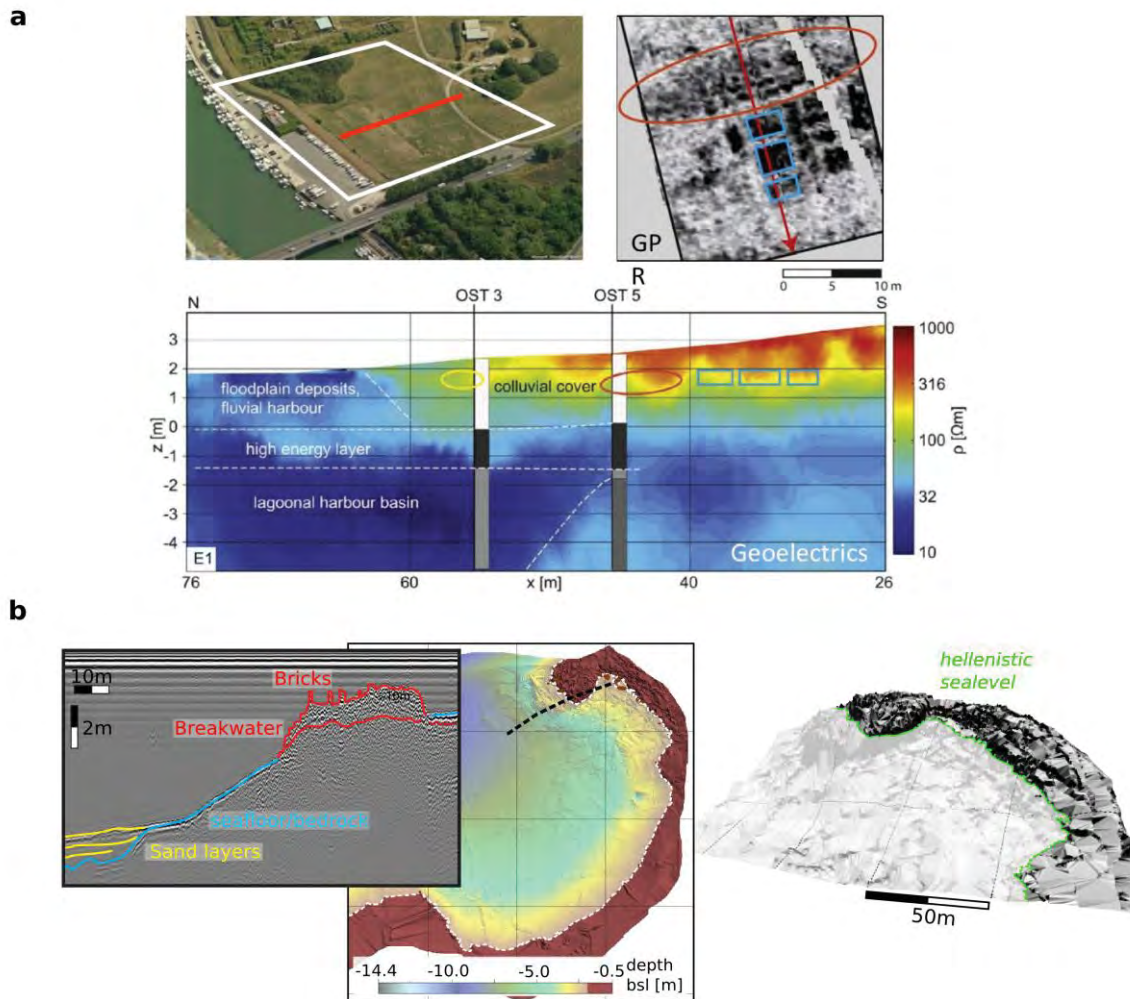
Fig. 2. Examples of the prospection of ancient harbours. (a) Fluvial harbour of Ostia Antica: Aerial view of the harbour and location of ERT profile (top left); ERT combined with drilling (bottom figure of a) revealed the two-phase nature of the harbour basin; GPR mapping shows the remains of houses and harbour construction (top right) (after Wunderlich et al. 2018). (b) Visualization of a Hellenistic/Roman sea harbour basin (right) on the Kane peninsula (western Turkey) based on seismic (left) and bathymetry (middle) data (after Fediuk et al. 2018).
