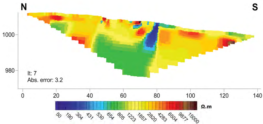
Fig. 1. ERT profile showing a silted-up entrance and a small sediment-filled cave. Note that the values for sediments are estimated to be < 400 \Omega.m .
