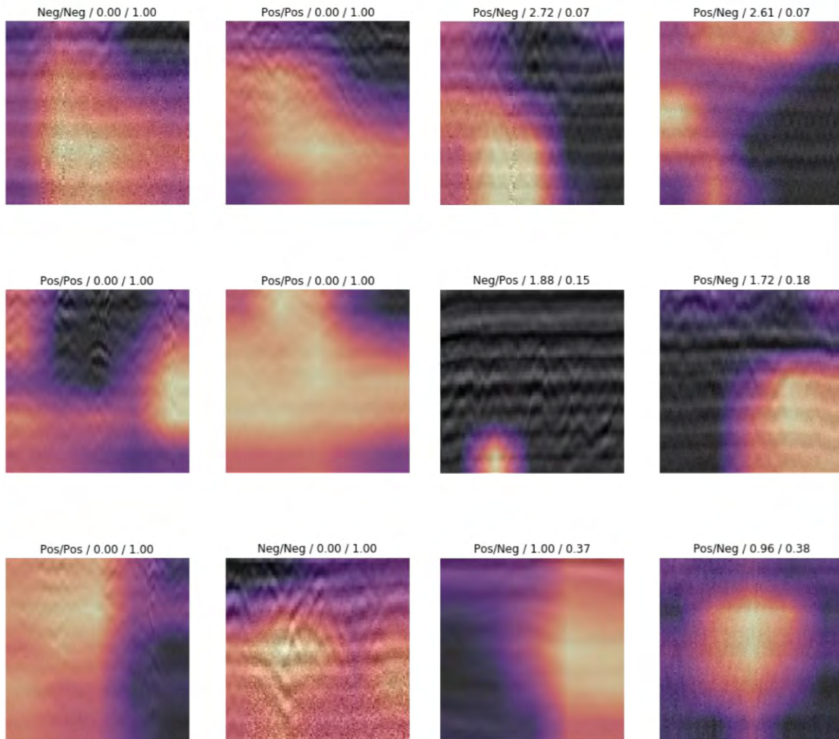
Fig. 3. Heatmaps indicating the areas of interest identified using the retrained ResNet152 model and their predictions and probability score.
