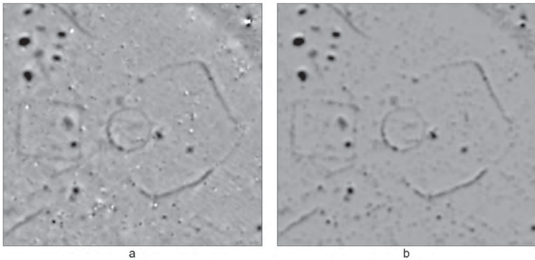
Fig. 2. a) Magnetic anomalies minus the modelled near-surface iron parts. b) Magnetic anomalies of the modelled susceptibility distribution. Visualization [white ... black]: [-2 ... +3nT].
