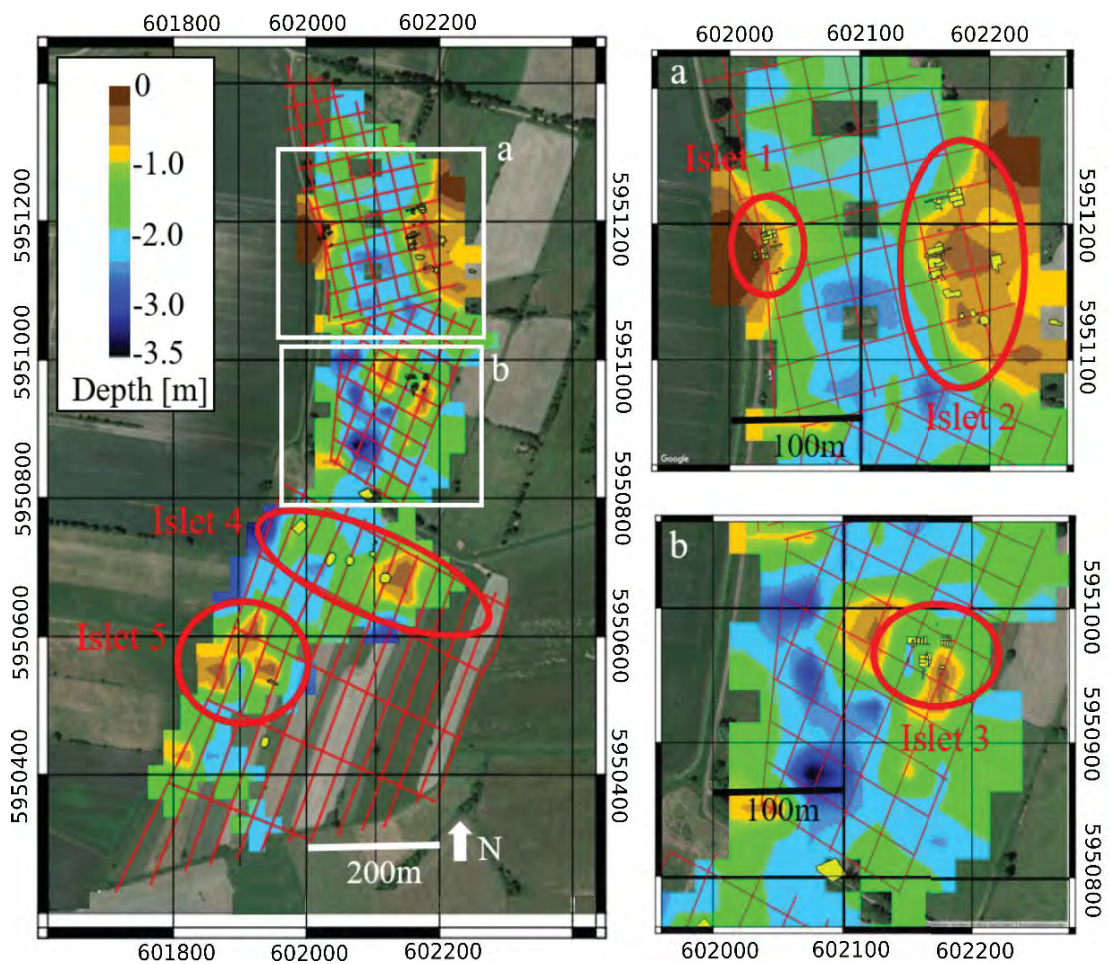
Fig. 2. The map of the surface related to the bottom of the lake. This illustrates a match between the brown areas (elevated palaeosurfaces, associated with the islets) and the Mesolithic camps (the yellow squares).
