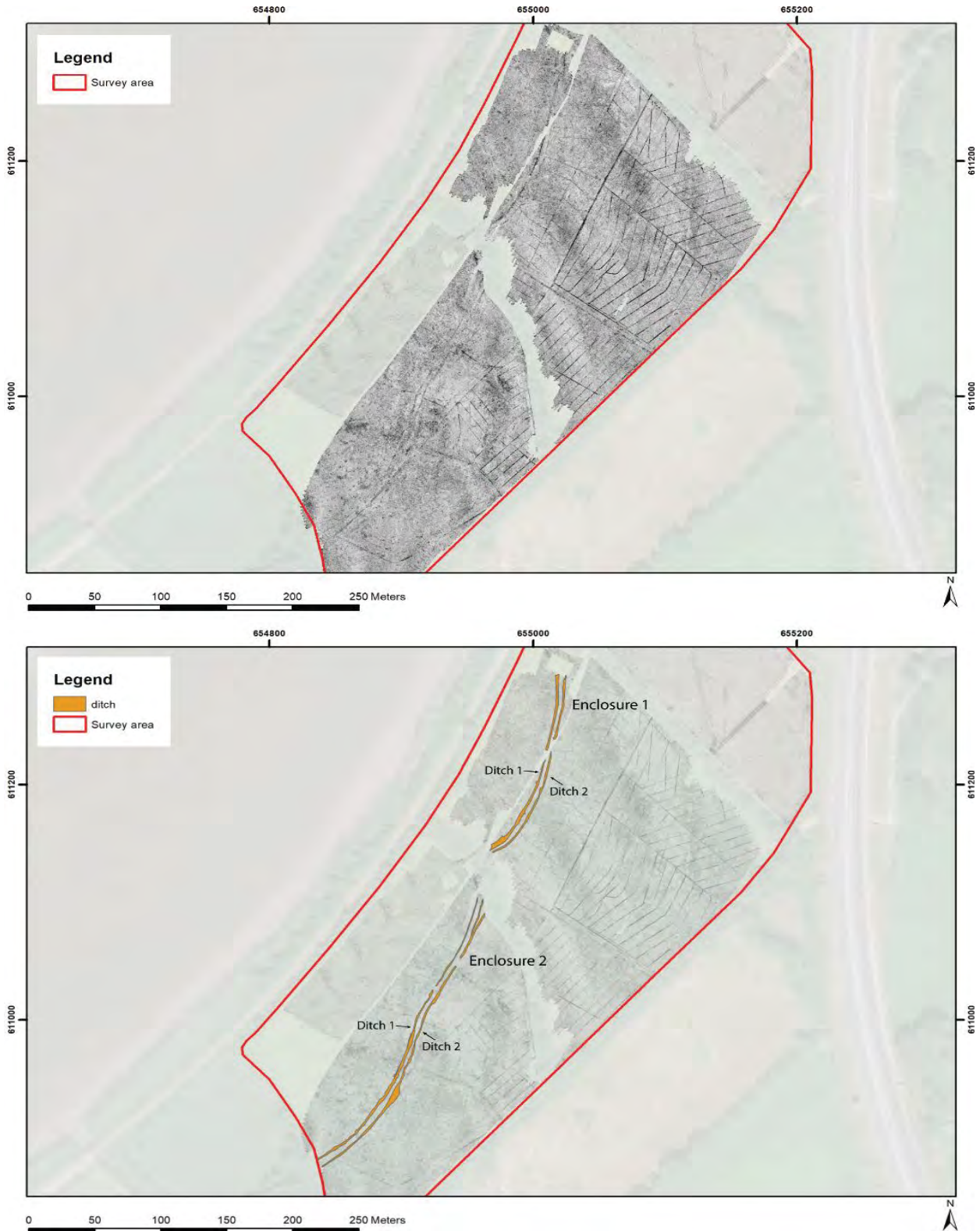
Fig. 2. (Upper) The double ditches of Enclosures 1 and 2 were discovered in the GPR data of fields C, E and F and are here visualised between 30cm and 200cm BGS. (Lower) Interpretative mapping of Enclosure 1 and 2.
