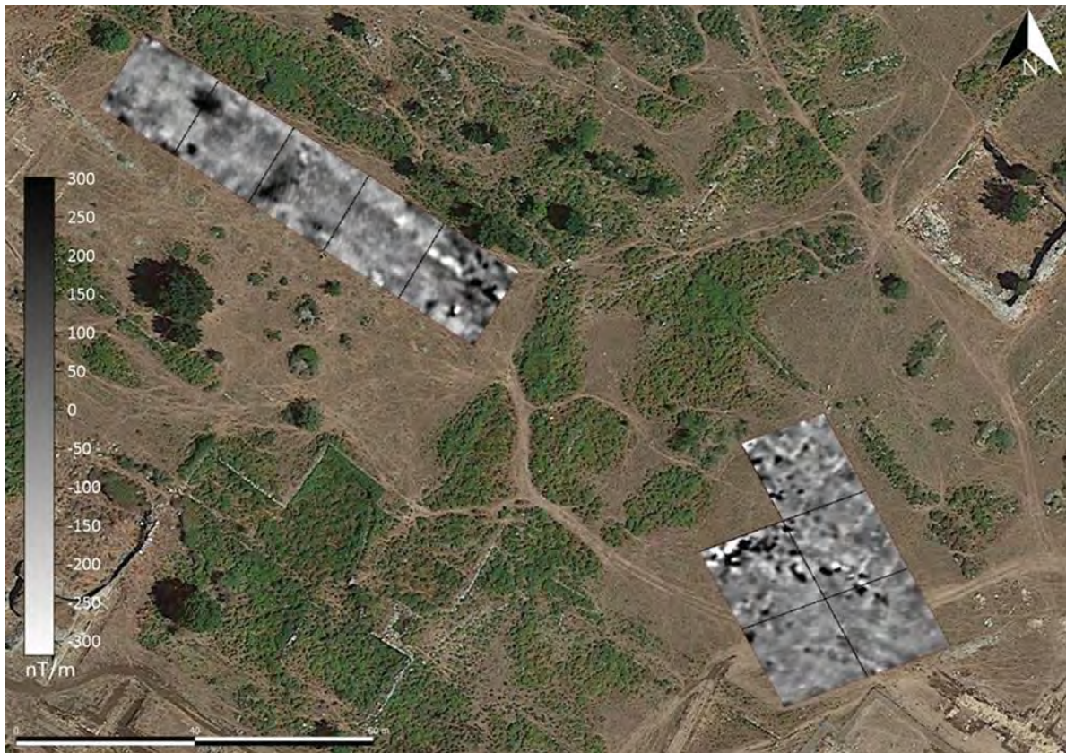
Fig. 2. Gradiometric contour map of the investigated area. Range -300 to +300nT/m.
