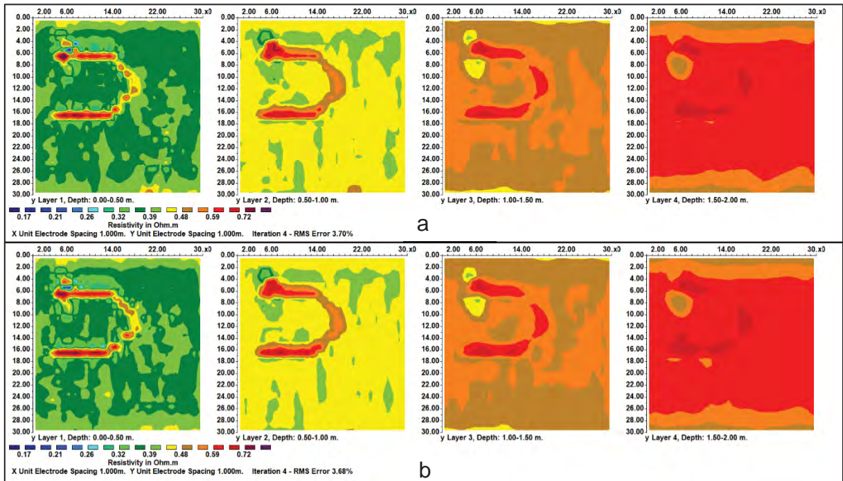
Fig. 2. a) Inverted section with electrodes at their actual position. b) Inverted section with electrodes moved to fit in a regular grid of 1m.
