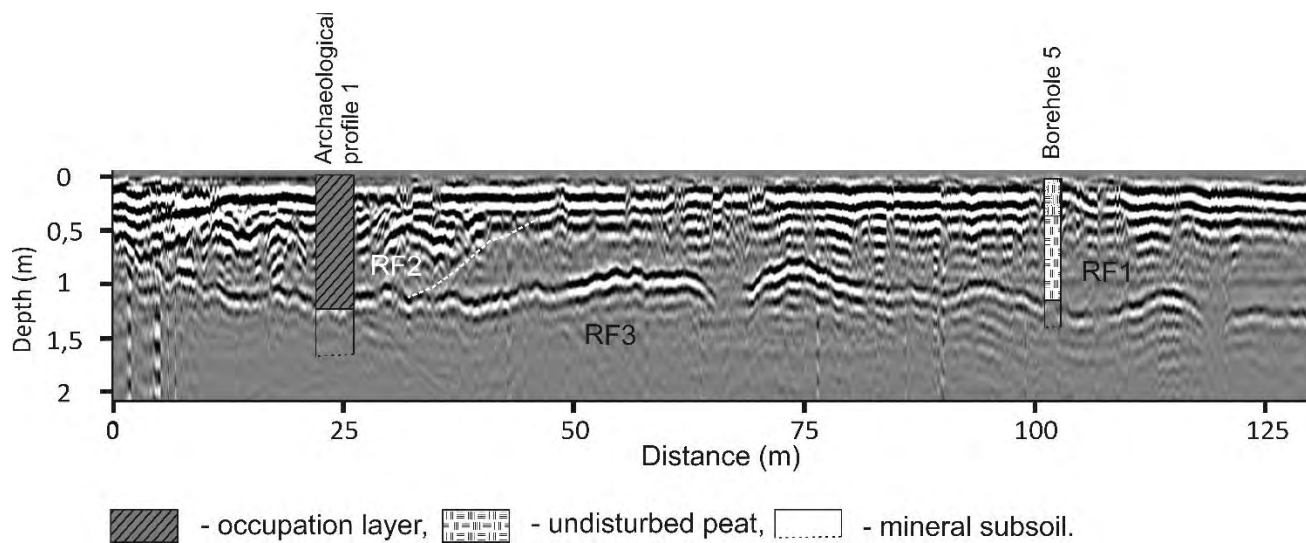
Fig. 1. Ground-penetrating radar image (with 300MHz centre frequency), demonstrating three characteristic radar facies: RF1 – long horizontal reflections corresponding to the undisturbed peat layer, RF2 – tilted chaotic reflections corresponding to the occupation layer, RF3 is separated from RF1 and RF2 by strong continuous reflector and corresponds to the mineral subsoil.
