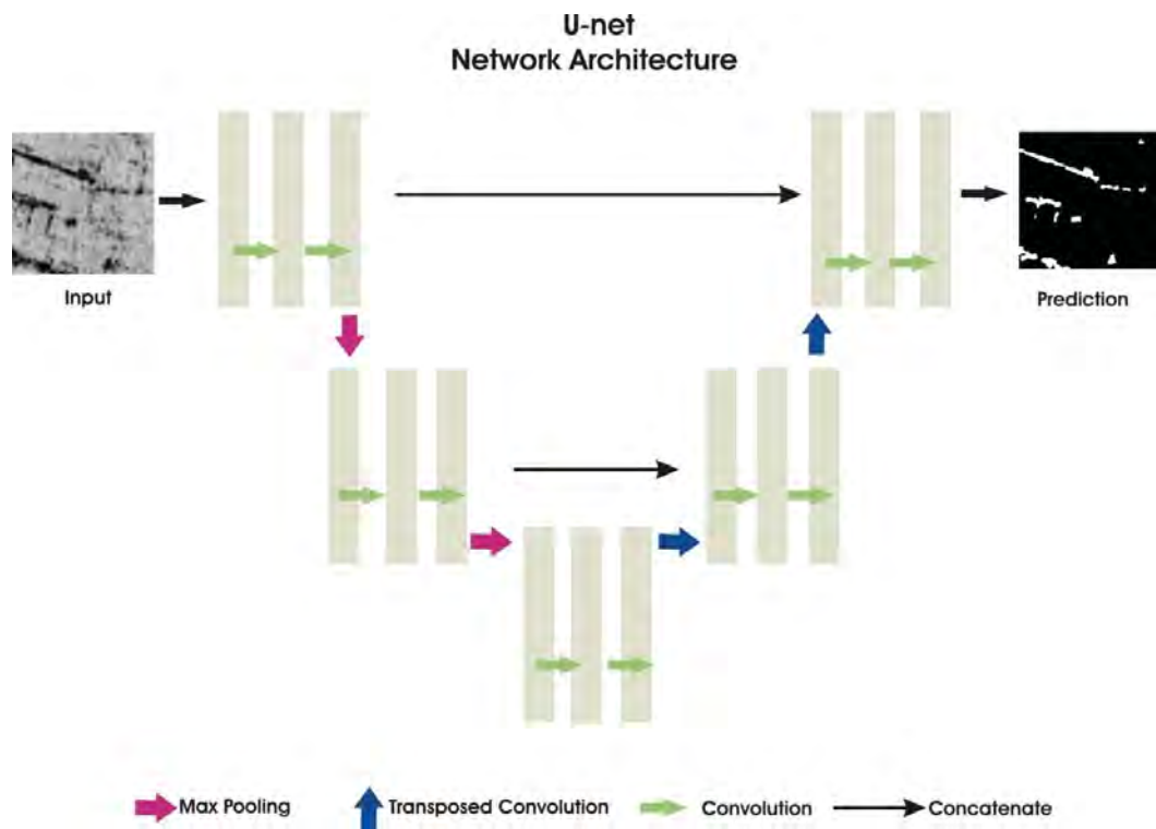
Fig. 1. Block diagram of U-net Architecture
