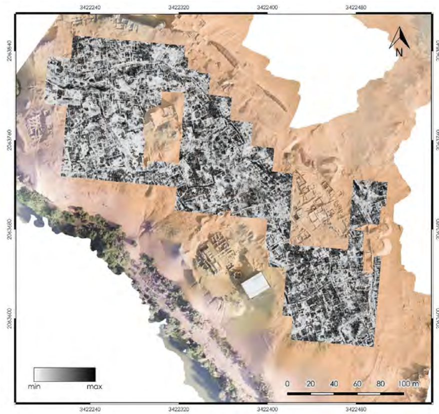
Fig. 2. Old Dongola, citadel. GPR survey. Timeslice 12sn to 14ns (approximate depth 0.6m–0.7m) on a vertical aerial photograph of the citadel
