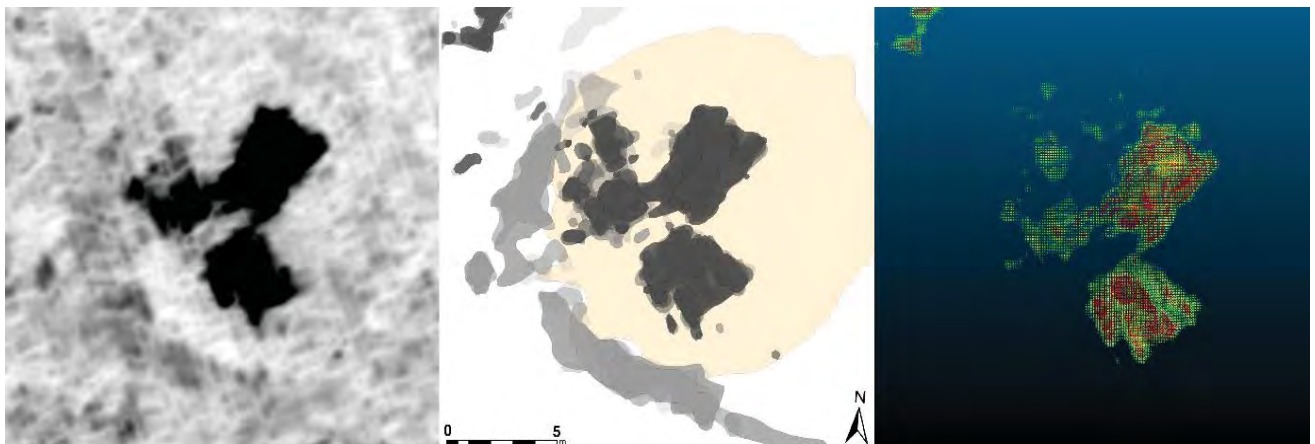
Fig. 1. Left: 160MHz GPR depth-slice 40cm to 250cm. Centre: interpretative mapping of GPR data (grey=path, black=burial chamber, ochre=tumuli). Right: 3D point-cloud amplitude rendering derived from the GPR dataset.
