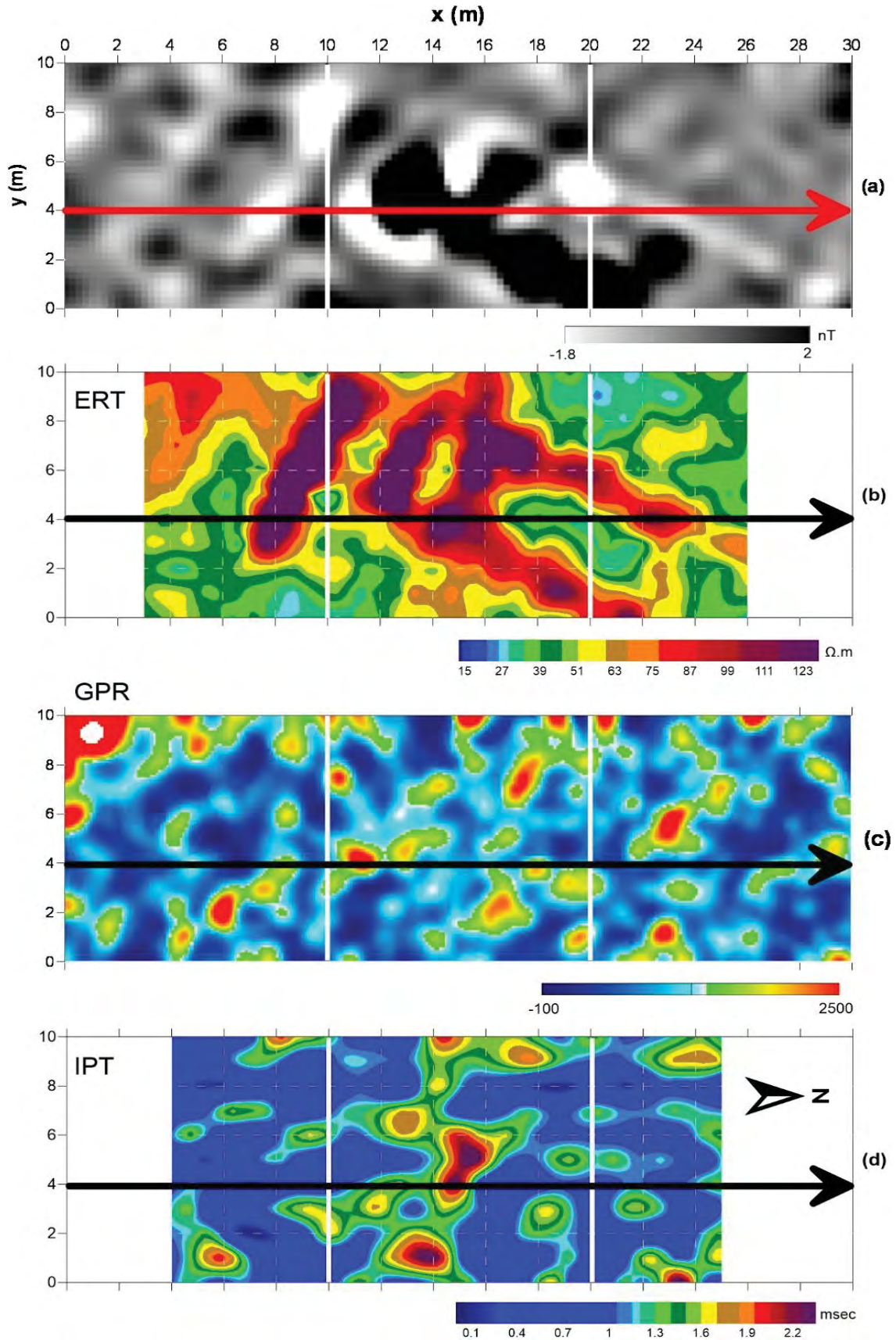
Fig. 1. Magnetic gradiometry image (a) and depth slices of ERT (b), GPR (c) and IPT (d) obtained from the test site. The arrows on these images indicate the example profile given in Fig. 2.
