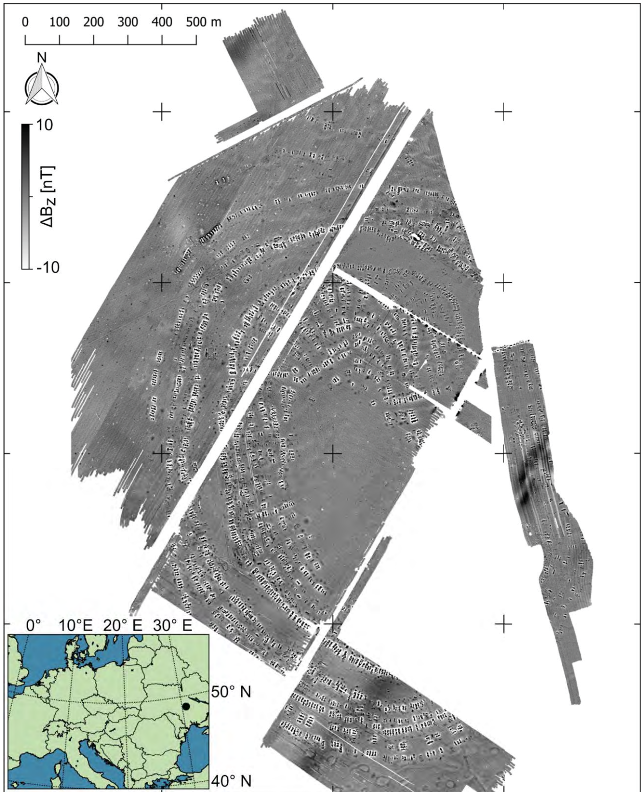
Fig. 1. Magnetic map of the site Maidanetske (after Rassmann et al. 2014) with the location of the site in Ukraine.
