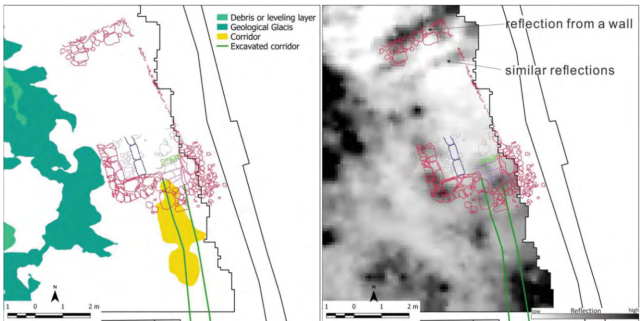
Fig. 3. Excavation results over the interpretation scheme based on GPR survey, and over the amplitude map corresponding to a depth between 0.80-1.05m.
