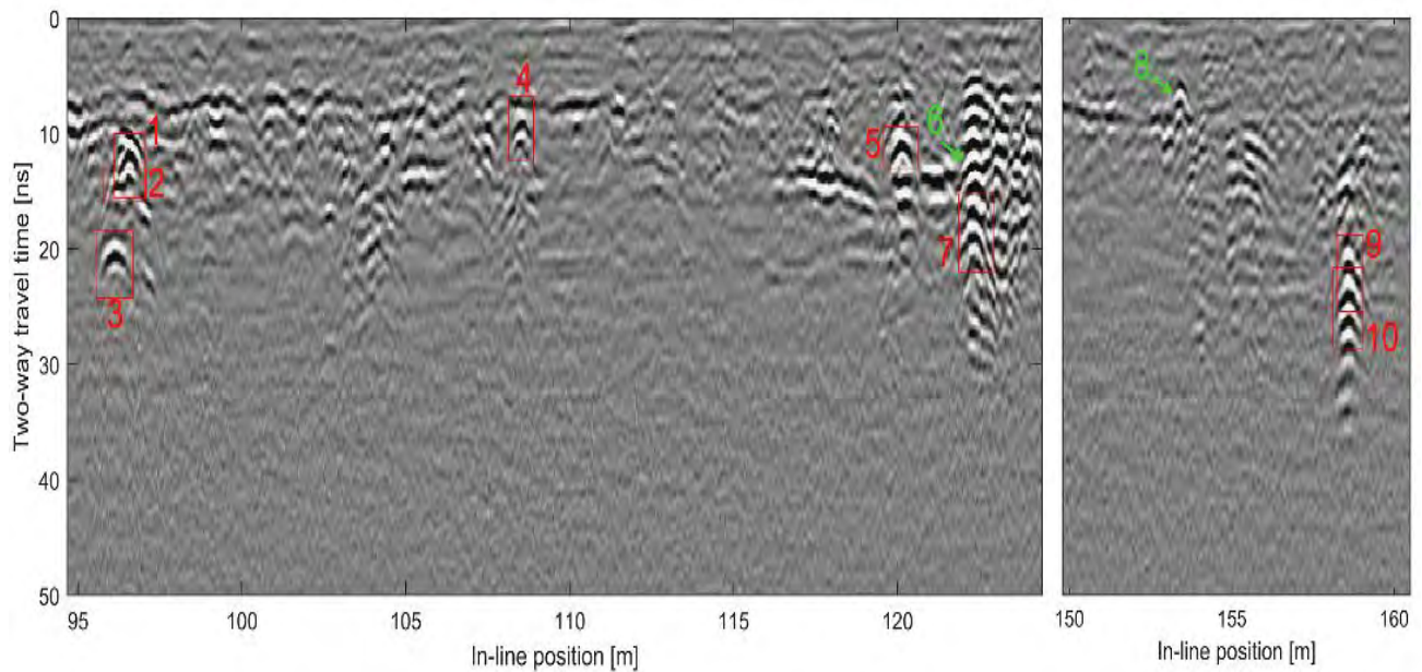
Fig. 2. Two parts of a GPR profile from Falerii Novi. The automatically detected hyperbolae are indicated in red, the ones used for the manual velocity analysis but not detected automatically are indicated in green. The numbers correspond to the ones in Table 1, and are explained in the text.
