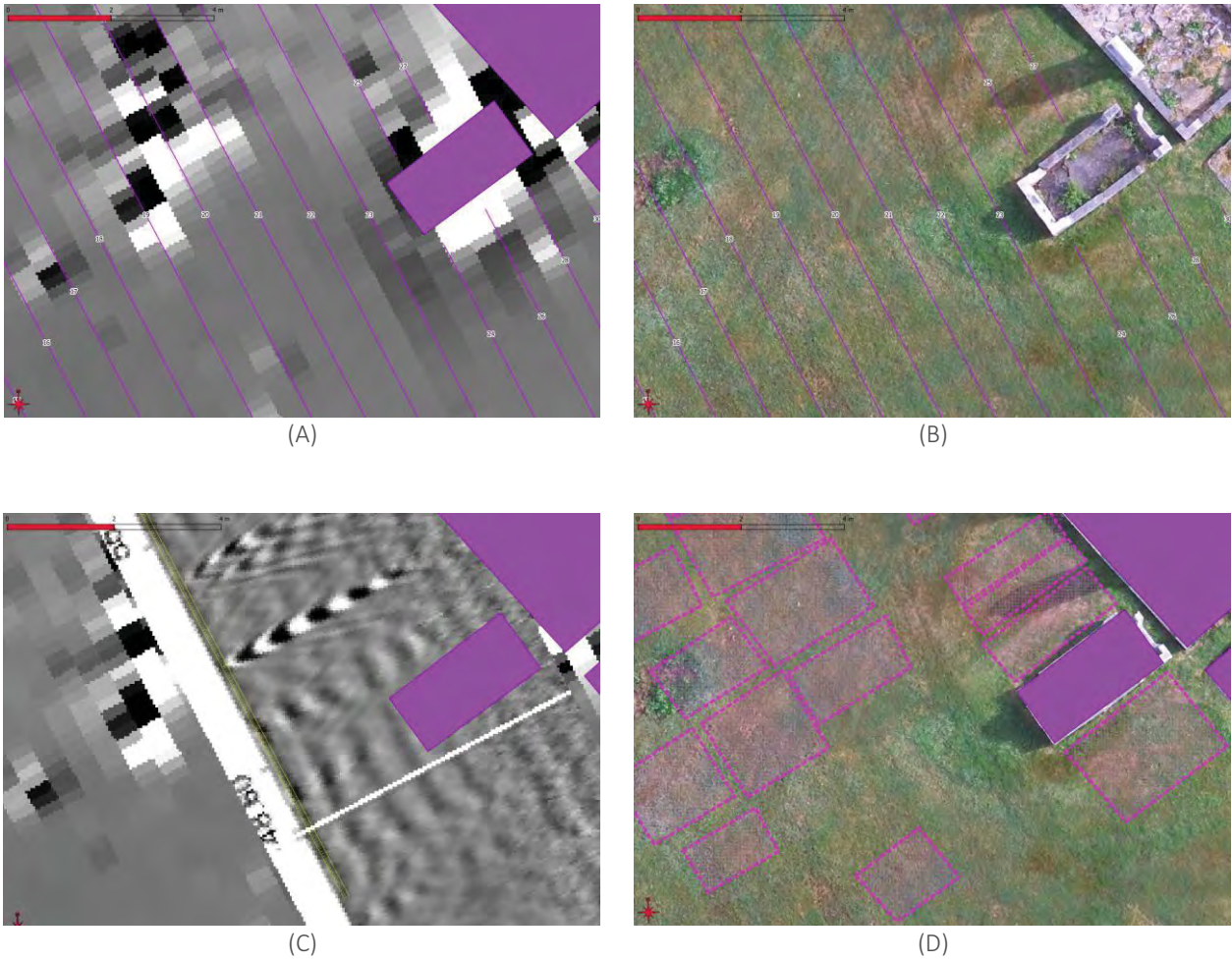
Fig. 1. (A) Geomagnetic survey around and over marked graves. (B) Ground-penetrating radar lines around the marked graves. (C) Marking "disturbed" areas on radar profile and comparing it with geomagnetic data. (D) Plan of marked graves and possible, unmarked graves.
