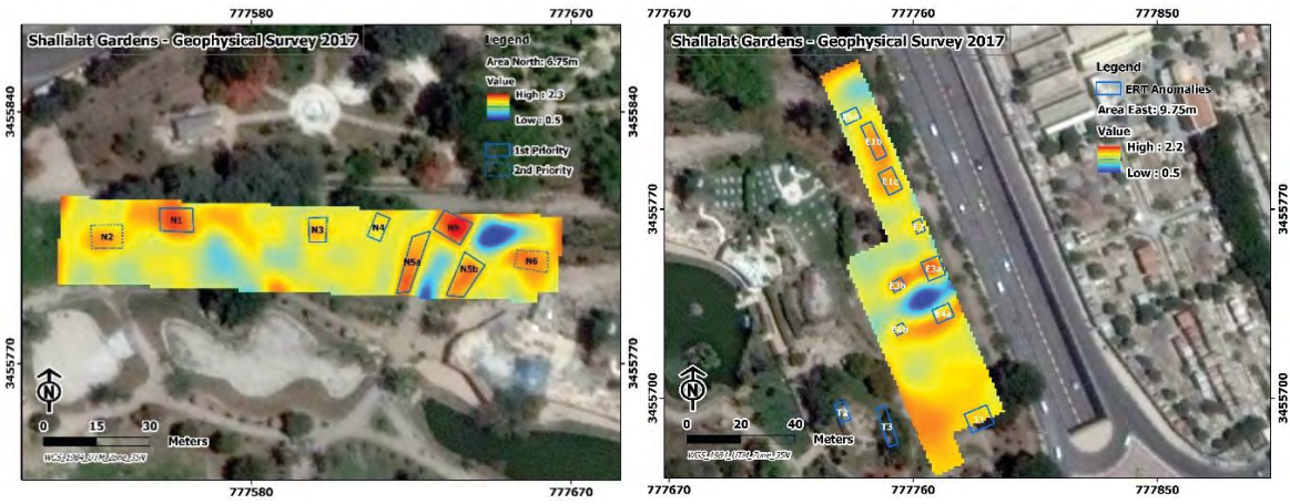
Fig. 2. Resistivity depth slice of 6.75m and 9.75m of the northern and eastern area respectively in Shallalat gardens. The axis units in metres and the resistivity is in Ohm.m.
