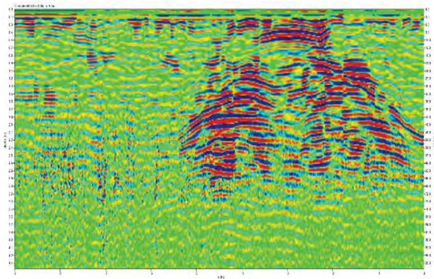
Fig. 2. GPR section profile of the stone chamber (6.5m line from the chamber entrance).
