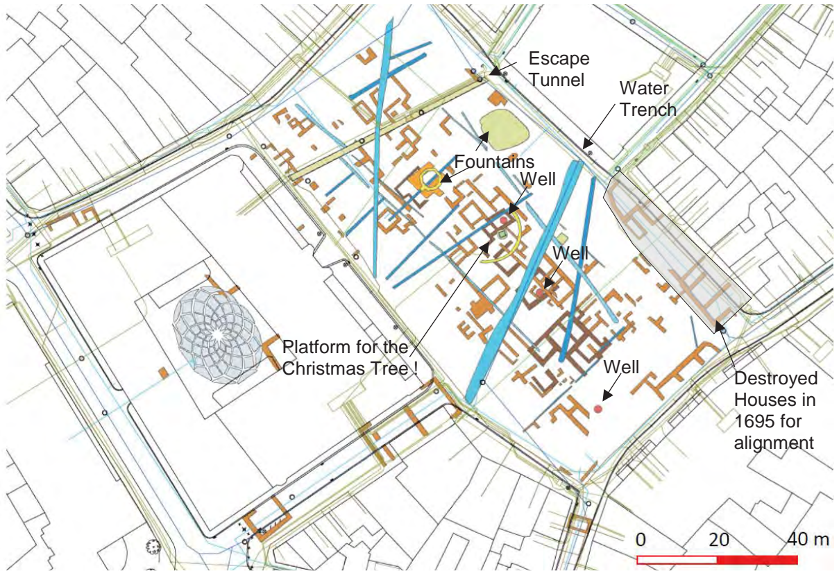
Fig. 4. First joint interpretation of resistivity maps and GPR time-lapse maps (March 2019 – F. Blary).
