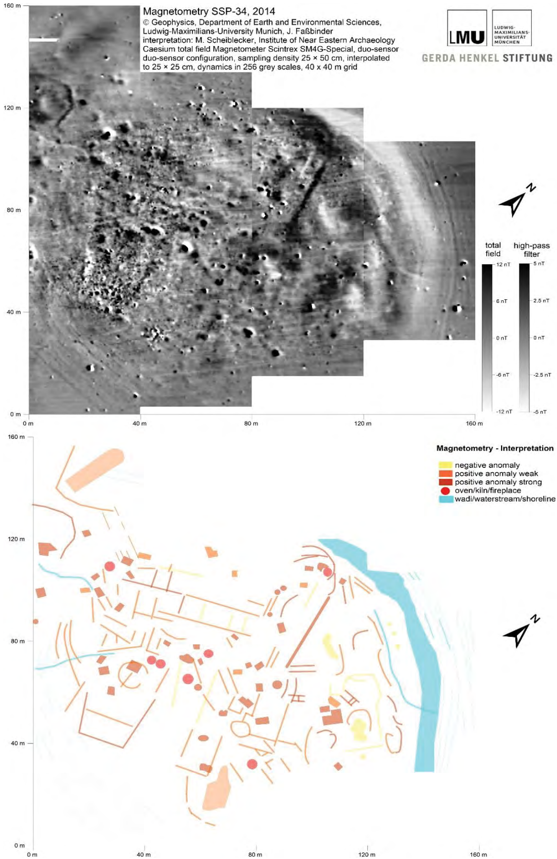
Fig. 3. Magnetogram and interpretation of SSP-34.
