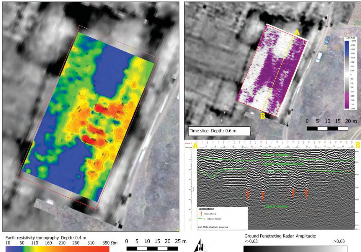
Fig. 3. Left: ERT results – a slice at 0.4m depth. Right: GPR time-slice and a profile from Polygon 1 (marked A-B).
