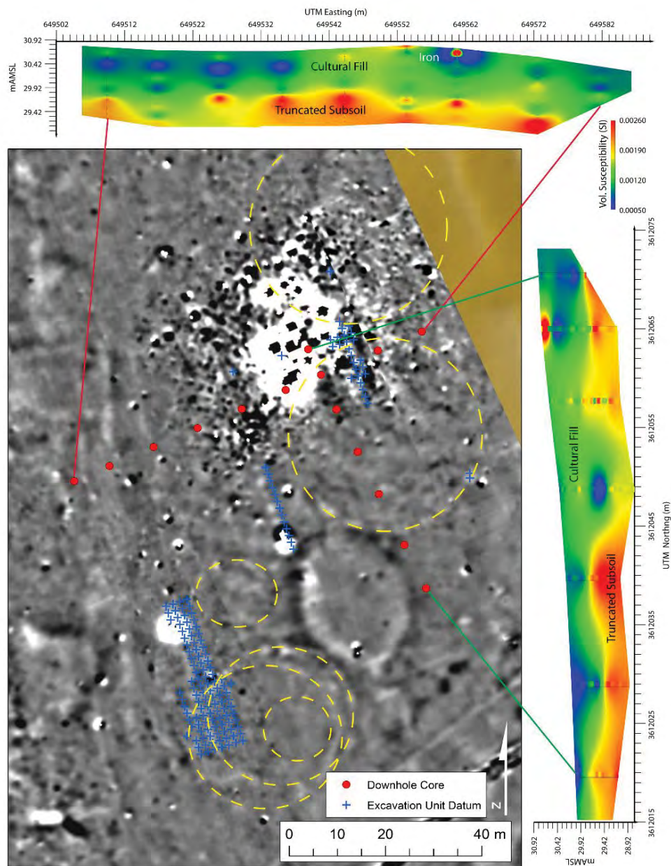
Fig. 2. Magnetic gradient basemap ( \pm 4nT ) of the WPR area, with locations of downhole transects, previous excavations, and circular magnetic anomalies. Magnetic susceptibility curtains at top and right correspond to west-east and north-south transects, respectively.
