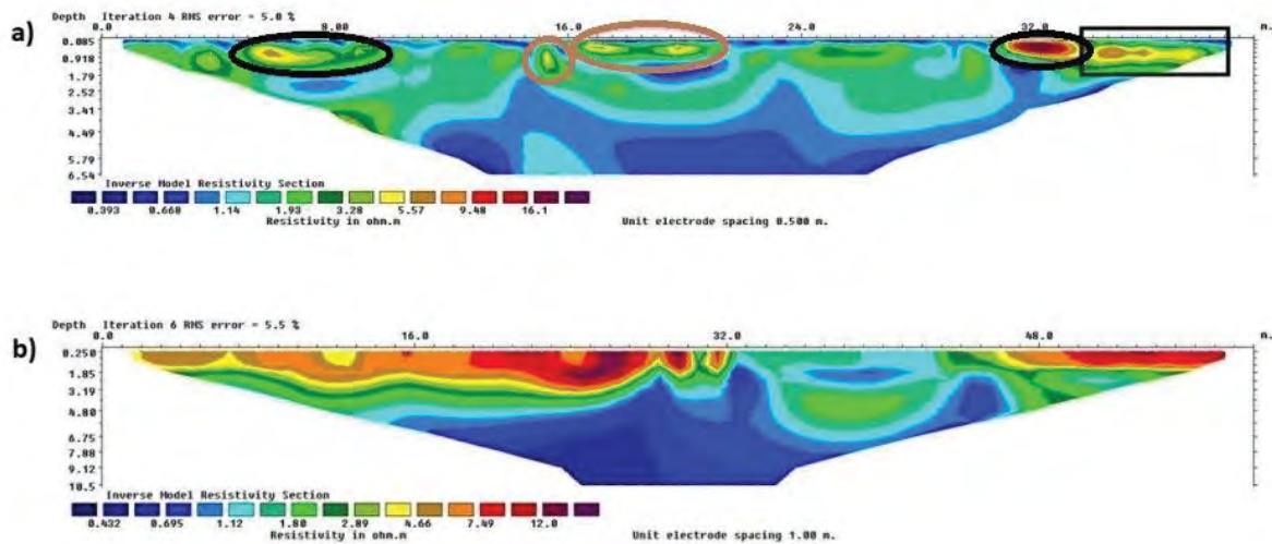
Fig. 3. (a) ERT profile over the city wall in Ur (electrode spacing 0.5m, dipole-dipole configuration). The black circles indicate inner and outer wall, the pink circles show the walls in between and the black rectangle indicates Woolley's excavation, which was refilled afterwards. (b) 2-D map of the harbour (1m electrode spacing, Wenner configuration).
