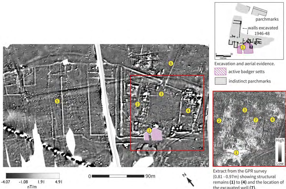
Fig.1. Extract from the magnetic survey showing the previously excavated west wing (1) of the scheduled villa and damage from an active badger sett threatening the survival of the remains. Additional building ranges (2), (3) and (4), only partially recognised from parchmarks, have been better defined in both the magnetometer survey and GPR data (inset bottom right). A much wider landscape of ditched enclosures (5) and an avenue (6) heading towards the river from the villa compound are also evident.
