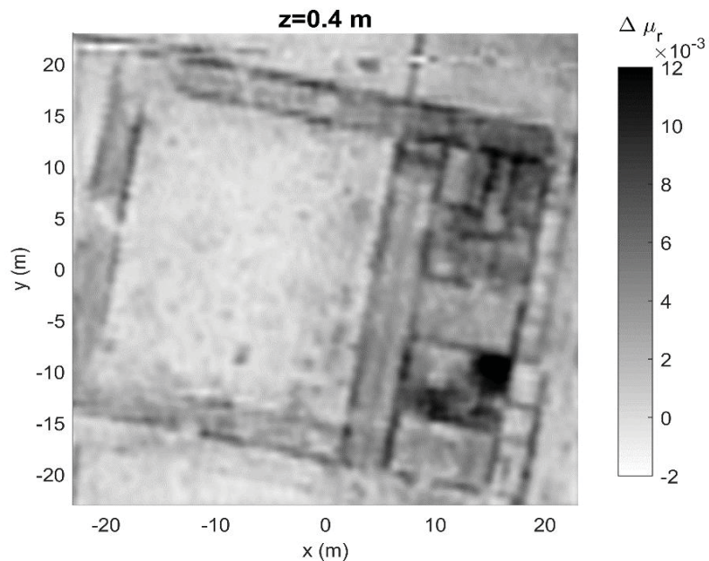
Fig. 3. Horizontal slice, at z=0.4\text{m} below ground surface, of the 3D model of magnetic permeability contrast resulting from the 3D MCD imaging approach.
