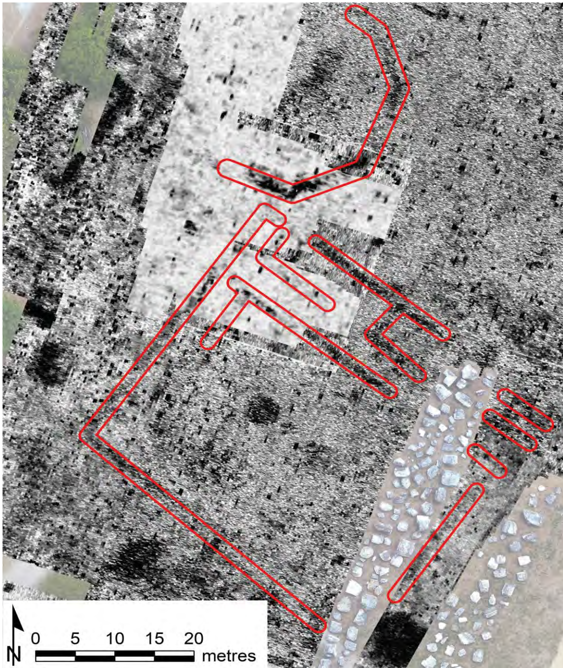
Fig. 2. GPR timeslice of central area (estimated depth 0.8m) with major anomalies outlined in red. Southern anomalies relate to the Portuguese church, northern anomalies to the octagonal Dutch building.
