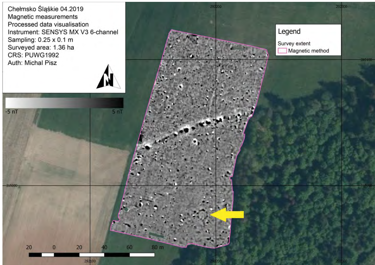
Fig. 1. Magnetic measurements. Magnetic anomaly interpreted as the remains of gallows is marked by a yellow arrow.
