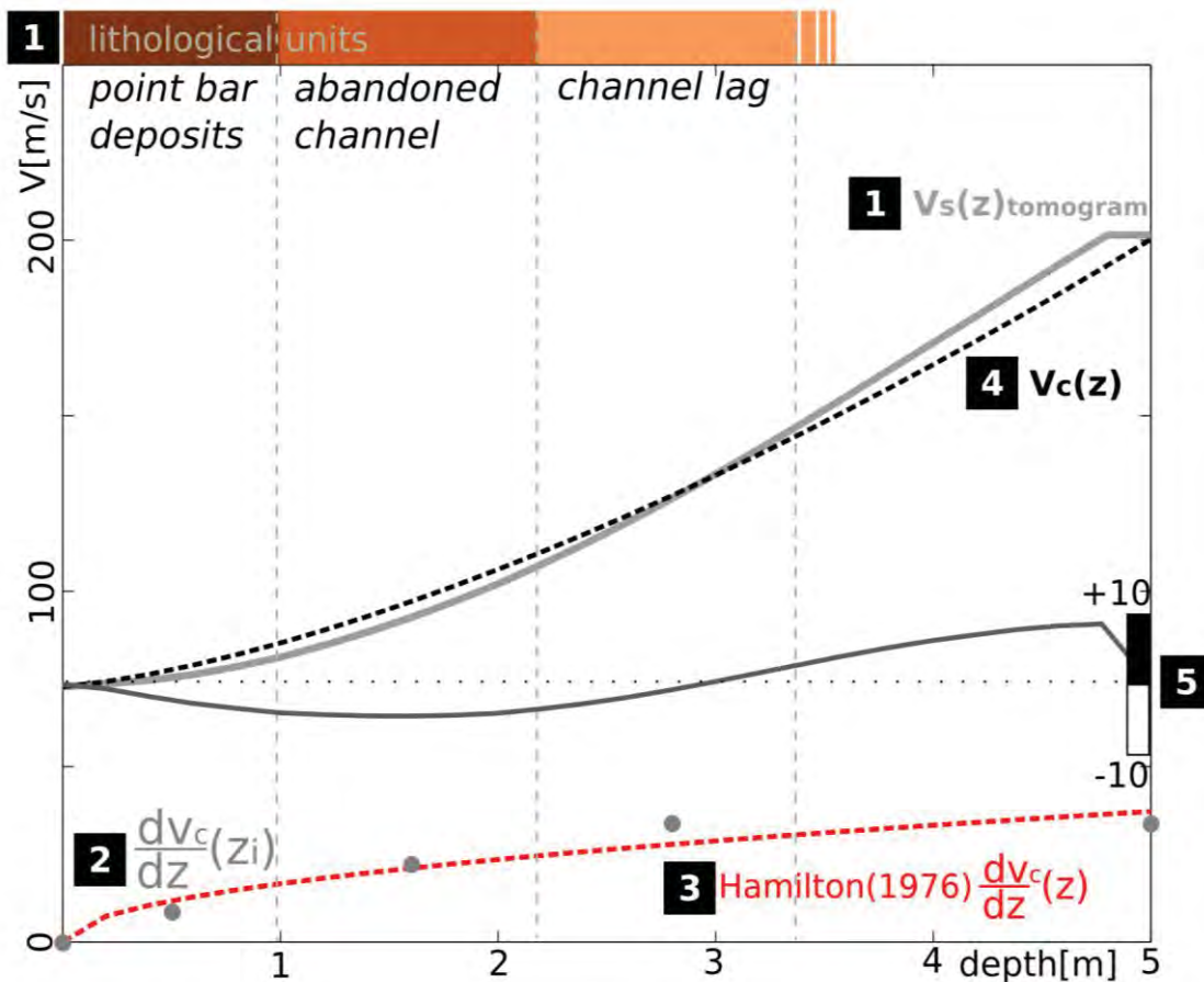
Fig. 2. Steps involved in the pressure correction methodology, using the velocity depth curve example located at the position of the reference core (numbers refer to the steps detailed in the text).
