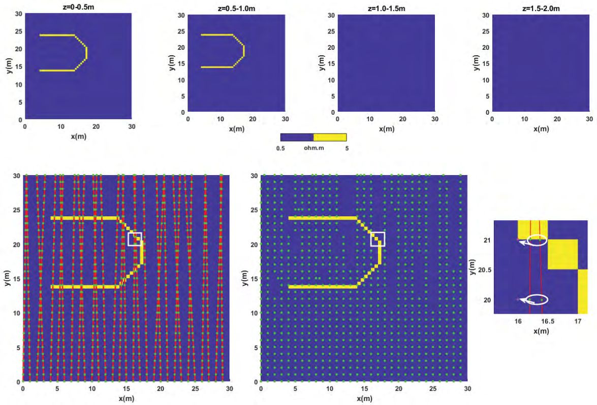
Fig. 1. Model that describes a U-shape wall buried below the sea bottom (top). Dynamic ERT lines (red lines) and electrodes (green dots) in their correct position (bottom-left). Electrodes moved in regular grid of 1m (bottom-centre) and schematic representation of this movement (bottom-right).
