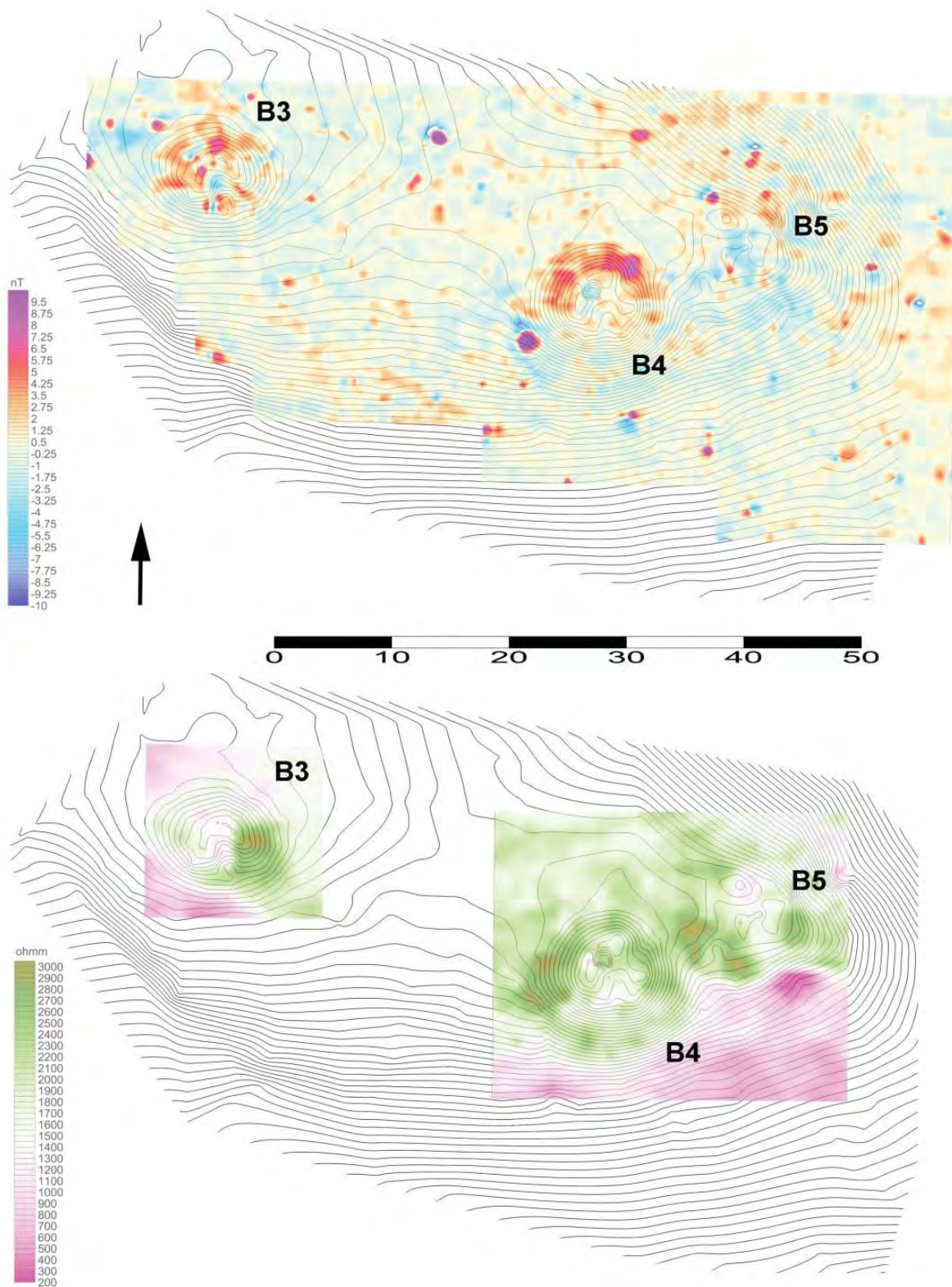
Fig. 1. Plav, České Budějovice district. Combination of magnetometer (top) and resistivity (bottom) surveys, overlain by a detailed contour line plan of area surveyed, forming part of a barrow cemetery (source of plan: South Bohemian University in Č. Budějovice; survey: Křivánek 2017; surveyed area: 0.237ha).
