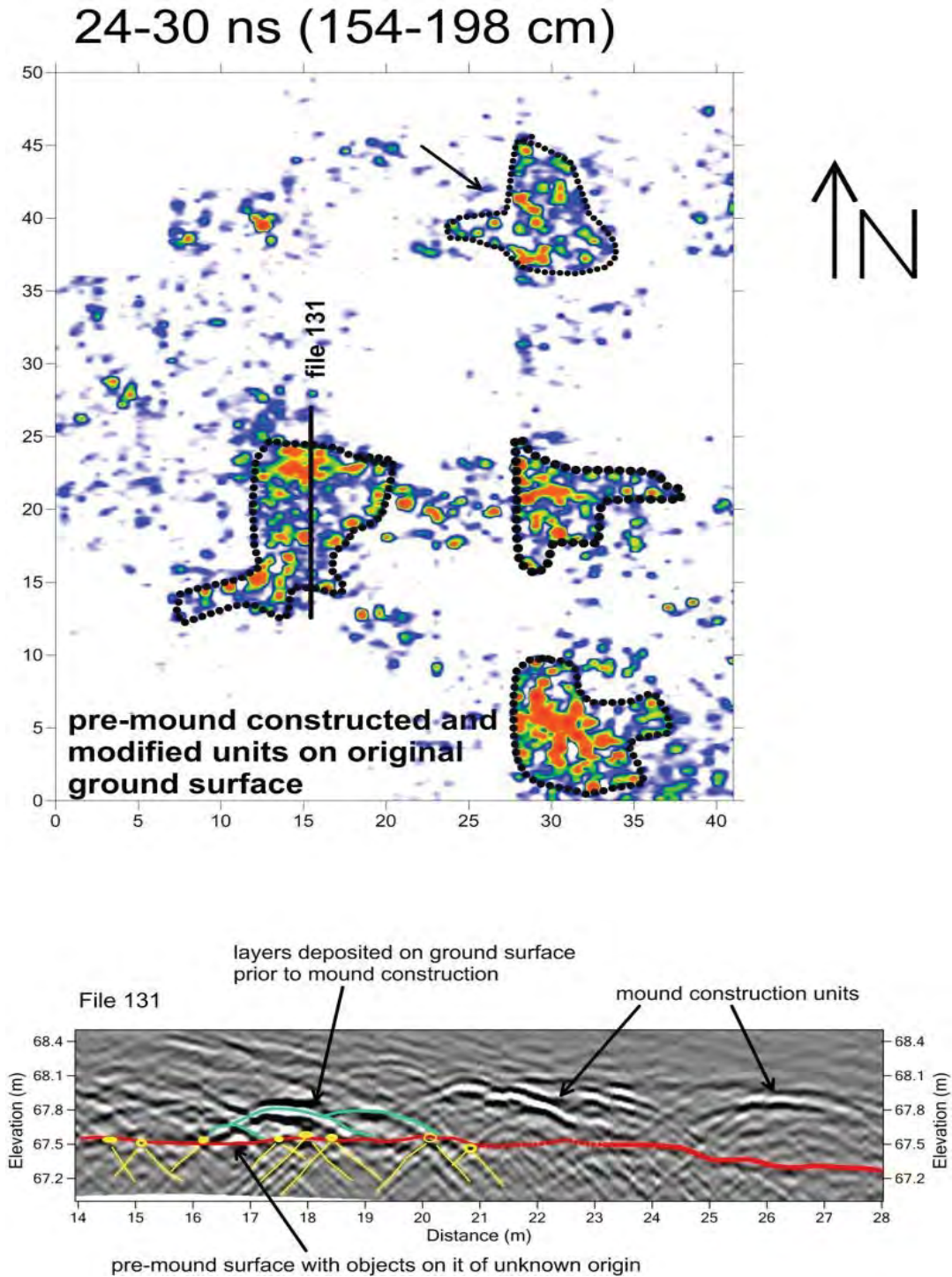
Fig. 3. Amplitude slice map of the deepest slice showing the concentrations of high amplitude reflections on the pre-mound surface that are concentrations of stones. A reflection profile produced after the reflections were frequency filtered to include only those between 400MHz and 600MHz shows the point-source reflection hyperbolae (axes of which are shown in yellow) from the stones on the original ground surface.
