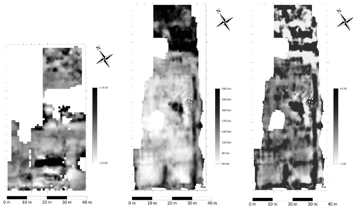
Fig. 1. Earth resistance results from Gračine. From the left: results from 2016 with despike, low pass and high pass filters applied; results from 2016 with despike and low pass filters applied; the same results with added high pass filter. All data are interpolated to 0.25\text{m} \times 0.25\text{m} .
