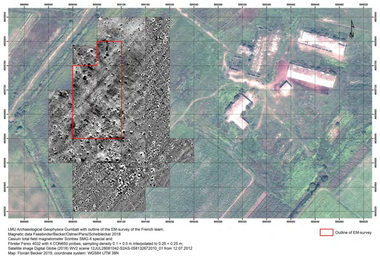
Fig. 1. Results of the magnetic prospection on Gumbati (scale: white/-10nT to black/+10nT).
