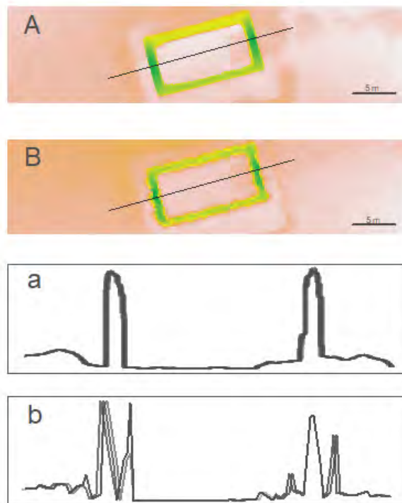
Fig. 2. An example of profile comparisons. Upper: Comparison of (A) photogrammetry and (B) LiDAR of St. Leo's Church, Inishark, Co. Galway, Ireland. Lower: west-east cross section profile of St. Leo's Church developed with (a) photogrammetry and (b) LiDAR.
