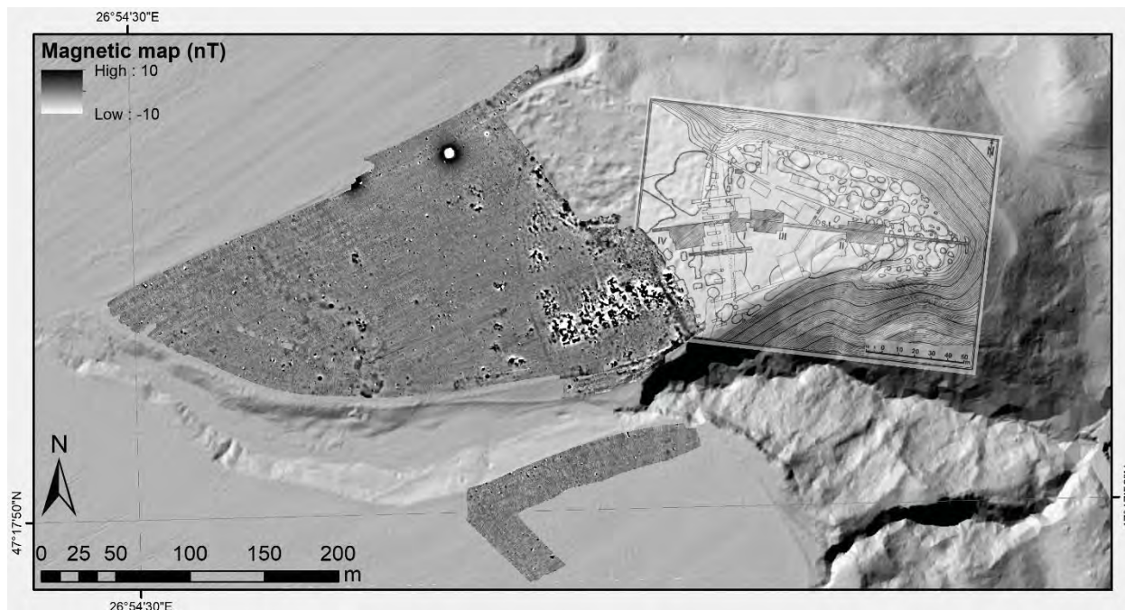
Fig. 3. Magnetic map (-10+10nT / white-black) and old excavation plan overlaid on Lidar DEM.
