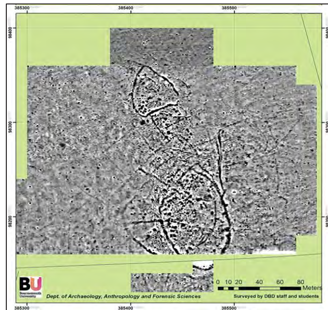
Fig. 2. Example magnetometry results from a site that is within the multiperiod landscape at Winterborne Kingston, Dorset, UK. Bartington 601-2 fluxgate gradiometry at 0.125m x 1m plotted -5 to +5nT (white to black).
