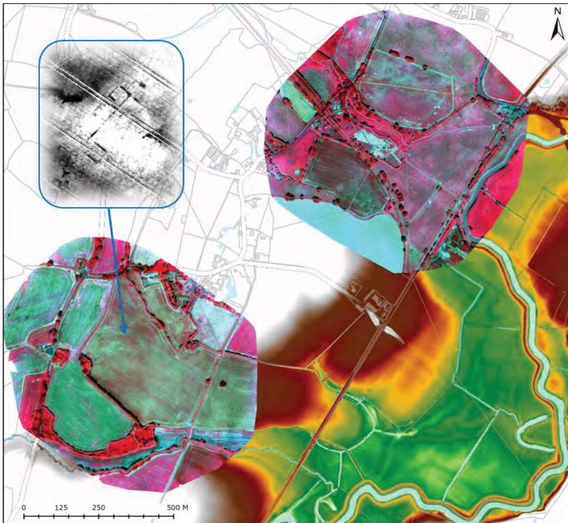
Fig. 1. LiDAR DTM constrained to 2m-9m (aOD), with false colour composite imagery overlain (R=NIR, G=Red, B=Green) and a detailed view of a Romano-British Villa (inset; greyscale NDVI).
