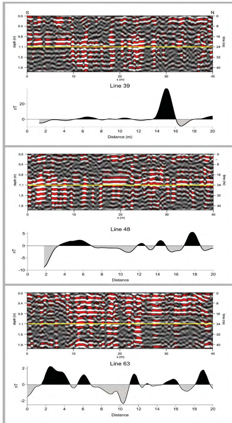
Fig. 3. Radargrams and magnetic gradiometry data of three selected lines. Yellow lines on radargrams show the general structure base
