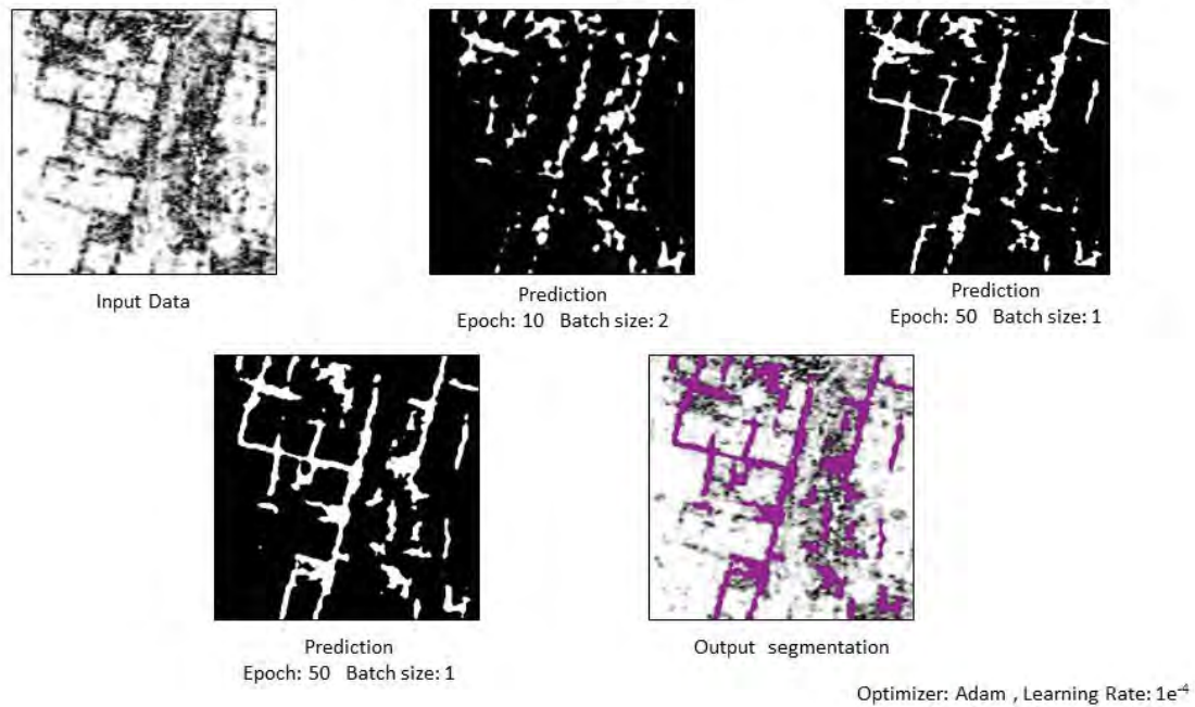
Fig. 2. The results of prediction process on a sample image created from a GPR (Sensors & Software, Nogin Plus, 250MHz antenna) depth slice from the archaeological site of Demetrias, close to Volos, Greece.
