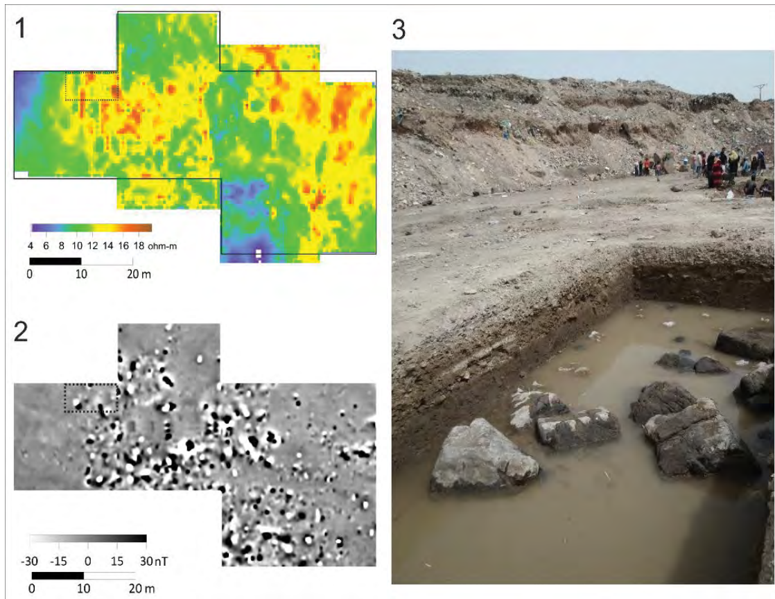
Fig. 1. Heliopolis / Matariya, temple of Nektanebo I. 1: resistivity map (Schlumberger asymmetrical array, AM=3.5m; MN=1m); trench in dotted outline, solid line marks the extent of the magnetic survey; 2: magnetic map; 3: stone blocks found in the trench.
