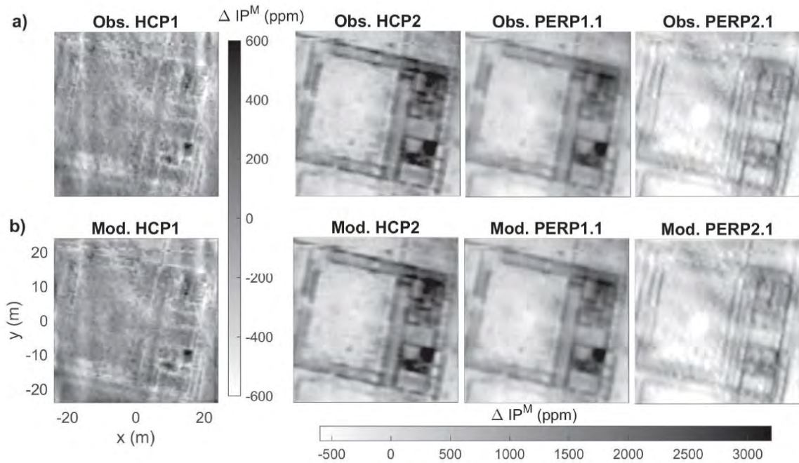
Fig. 2. Comparison between (a) the observed field data and (b) the modelled data computed after the 3D MCD imaging approach. The global RMS error including the four channels is 59 ppm.
