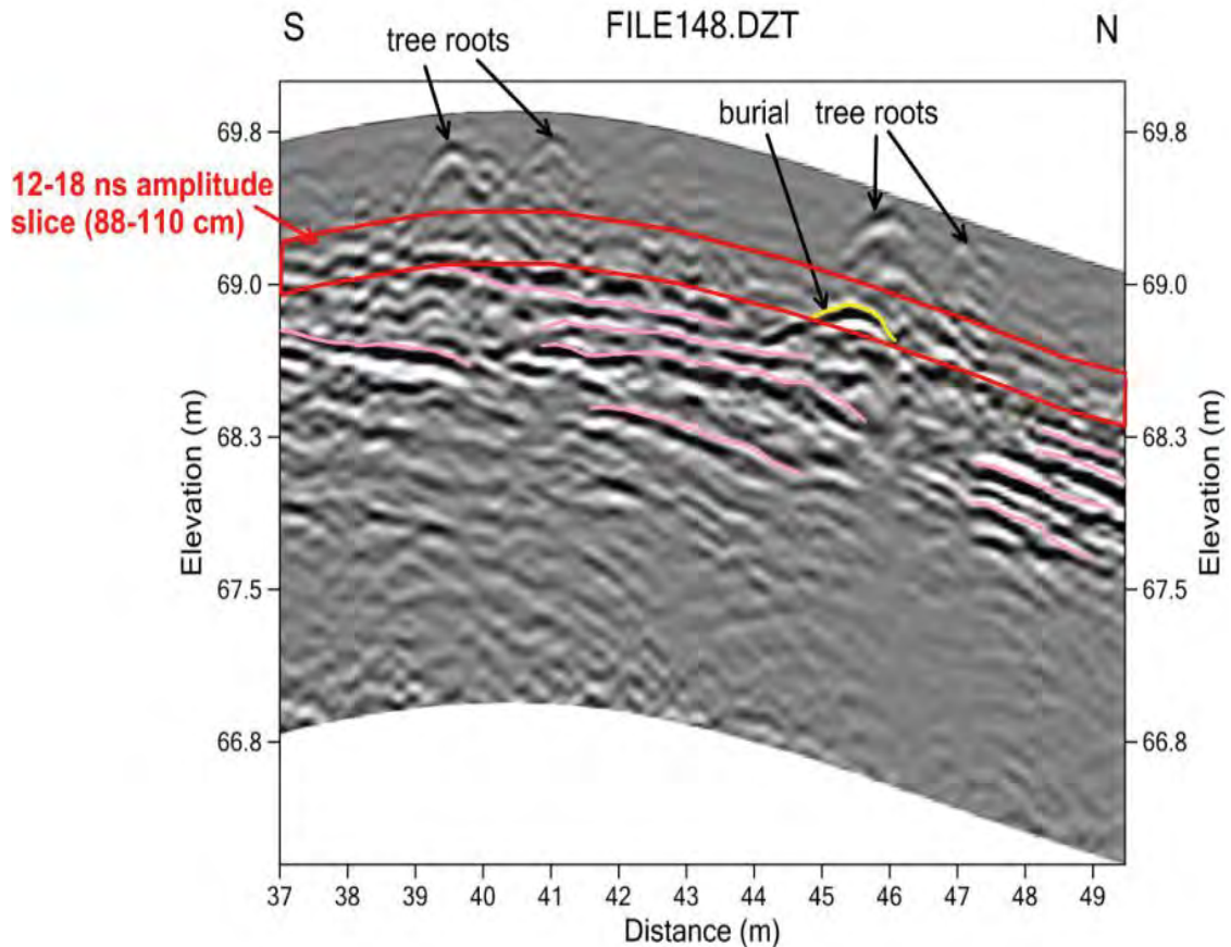
Fig. 2. Reflection profile corrected for topography, showing the reflection hyperbola produced by a human burial below the tree-root reflection. Mound fill units are shown in pink.
