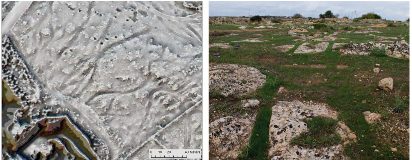
Fig. 2. Relict vehicle track networks in the project area. Left: Track outlines visible in ALS-derived relief model visualization. Right: Representative image of a relict track set.
