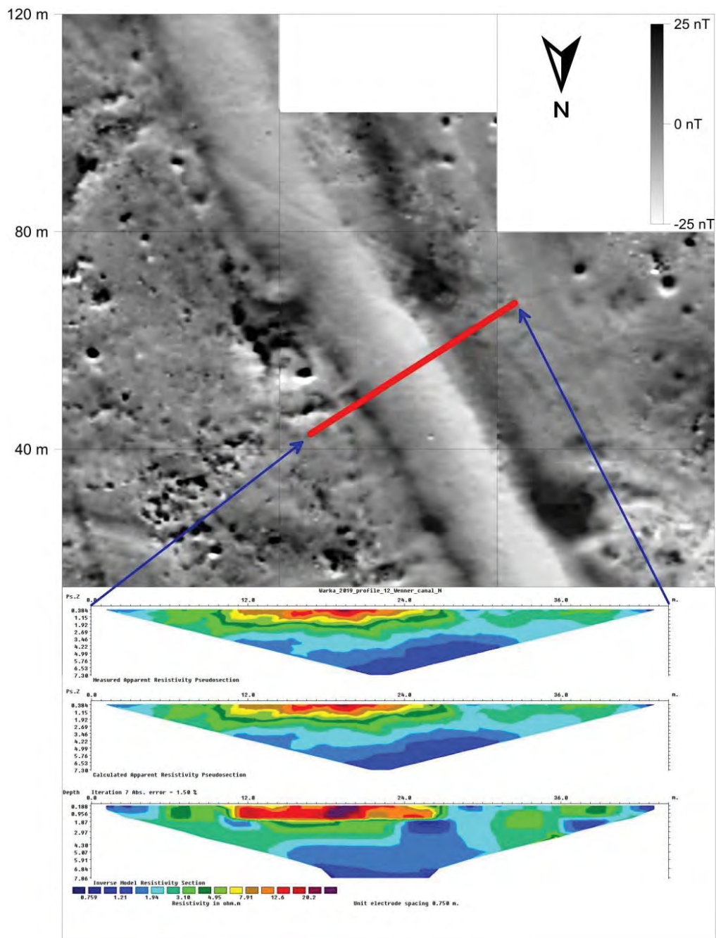
Fig. 3. At the top: Magnetogram extract of the main canal near the “Sinkashid” palace, the location of the 45m ERT-profile is marked in red. Below: ERT profile across the canal (0.75m electrode spacing, Wenner configuration).
