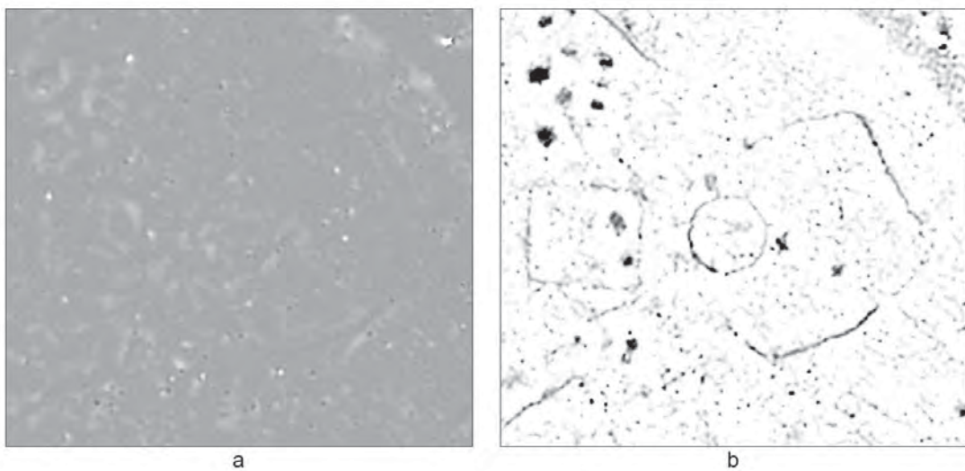
Fig. 3. a) Magnetic data without the modelled magnetic anomalies. Visualization [white ... black]: [-2 ... +3nT]. b) Relative susceptibility distribution. Visualization [white ... black]: [0 ... 3].
