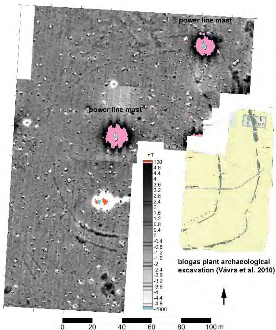
Fig. 2. Chrášťany, Kolín district. The result of the magnetometer survey combined with previous rescue archaeological investigation (source: plan from report of archaeological investigation by Vávra-Šťastný in 2010; survey: Křivánek 2018; surveyed area: approx. 2ha; Sensys 5-channel push-cart fluxgate gradiometer system; sampling interval: 0.5m x 0.2m).
