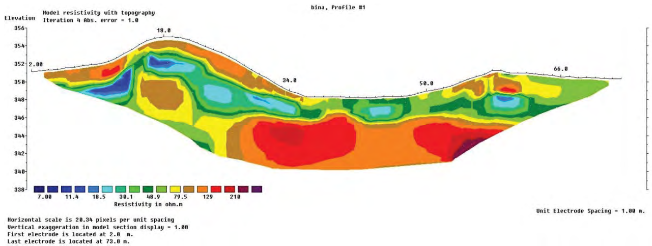
Fig. 1. Case study of ERT survey (Schlumberger configuration) on the early medieval hillfort Bina, located in the south-west region of Slovakia. The rampart has higher values of electrical resistivity in the lower central part covered by a layer of lower values above it.
