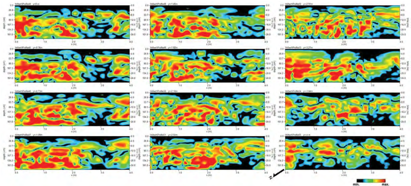
Fig. 2. Kovarce, St. Nicolas Church. Vertical slides from GPR measurement of crypt.
