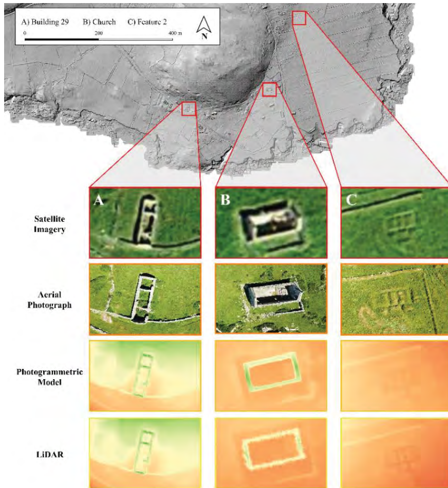
Fig. 1. An example of plan view comparisons of Building 29, the Church, and Feature 2 via satellite imagery, aerial photography, photogrammetry and LiDAR.
