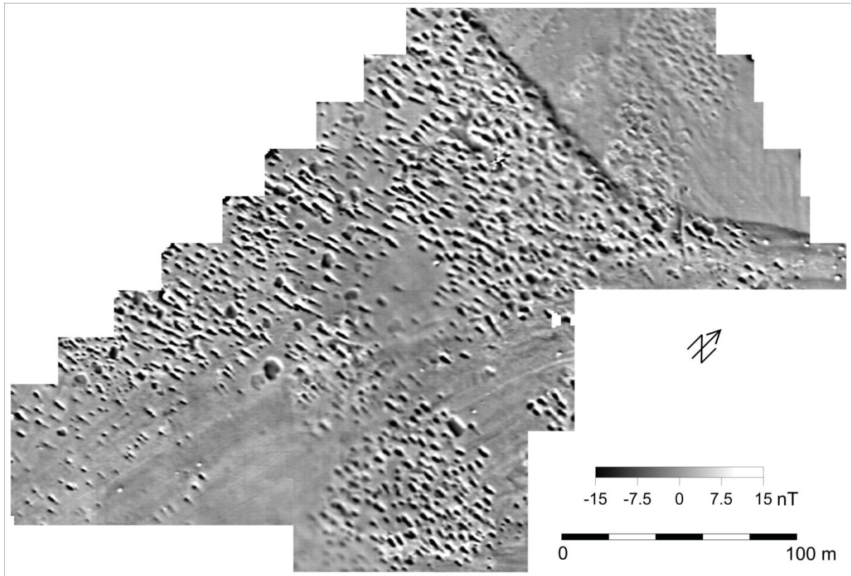
Fig. 3. Kawa, eastern cemetery. Magnetic map.
