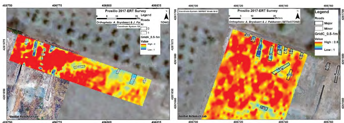
Fig. 2. Resistivity depth slice of 0.5-1.0m from Grid A (left) and the northern part of Grid C (right). Axes units in metres and resistivity in Ohm.m.
