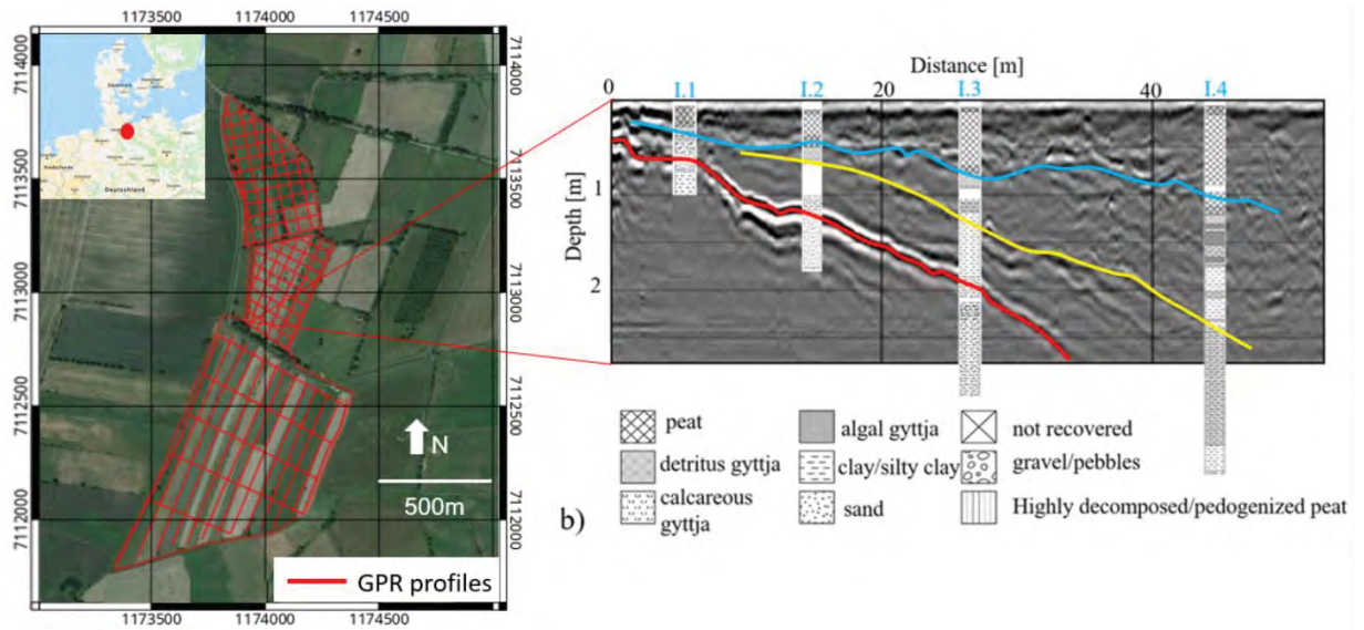
Fig. 1. (a) The investigated area of Duvenese with red lines indicating the GPR profiles. (b) Comparison between a radargram and the stratigraphy from the corings I.1, I.2, I.3 and I.4. The red line indicates the reflection coming from the bottom of the lake visible in the cores with the transition between clay and sand, yellow and blue lines indicate the clay layer and the peat on top.
