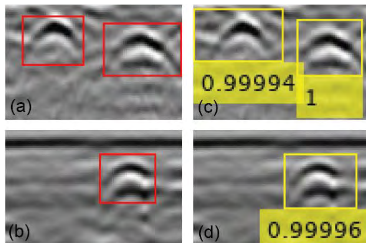
Fig. 1. Sample images used to test the Faster R-CNN detector after it had been trained. (a-b) Rectangles defining hyperbolae, marked manually. (c-d) Hyperbolae extracted by the Faster R-CNN detector, with the confidence score indicated.
