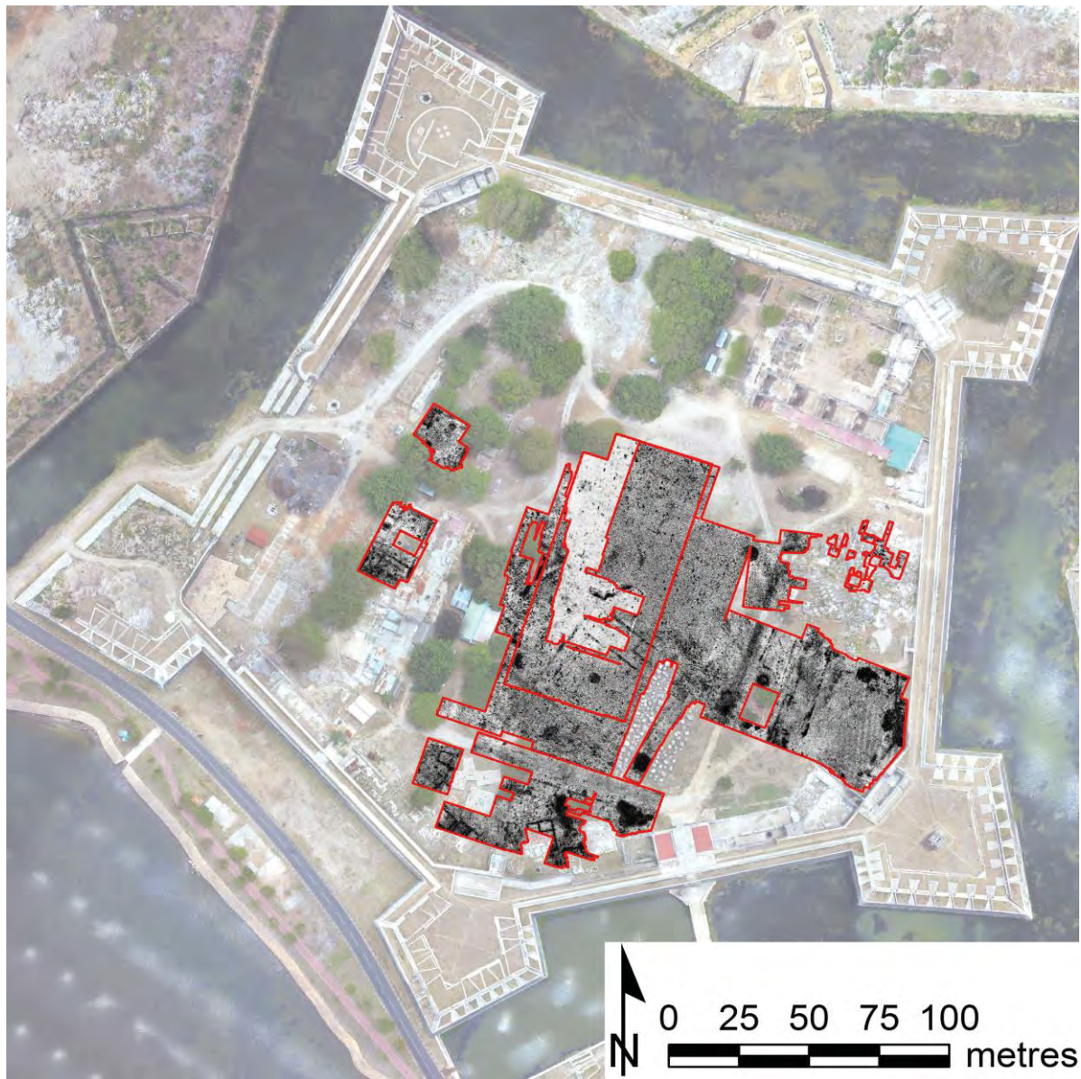
Fig. 1. UAV orthophoto of Jaffna Fort with GPR data outlined in red.
