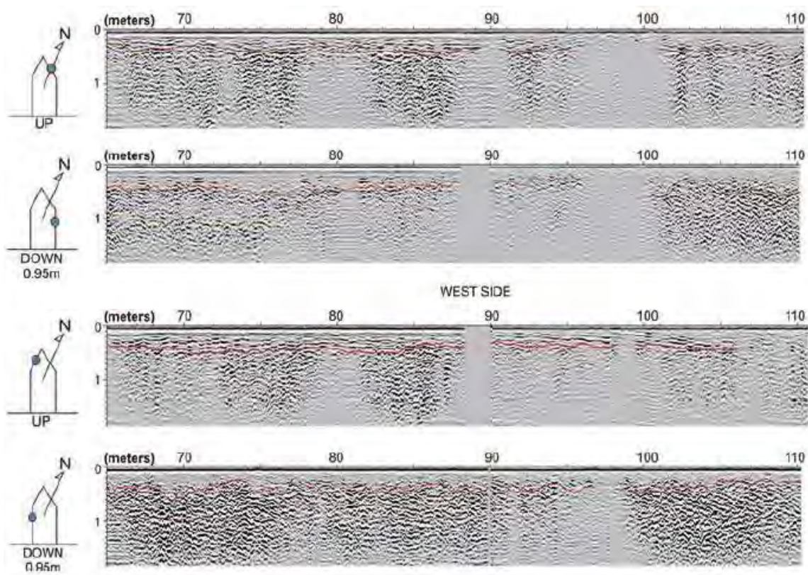
Fig. 2. Processed GPR sections on the sidewalls of the lining of Roman age. The small sketches on the left depict the direction of the profiles, and the dots mark the levels where they were carried out. The red line annotates a clear continuous reflection very close to the wall's surface at a distance varying \sim 0.3\text{ m} - 0.5\text{ m} . This reflection corresponds to the interface between the lining's building stones and the backfill material.
