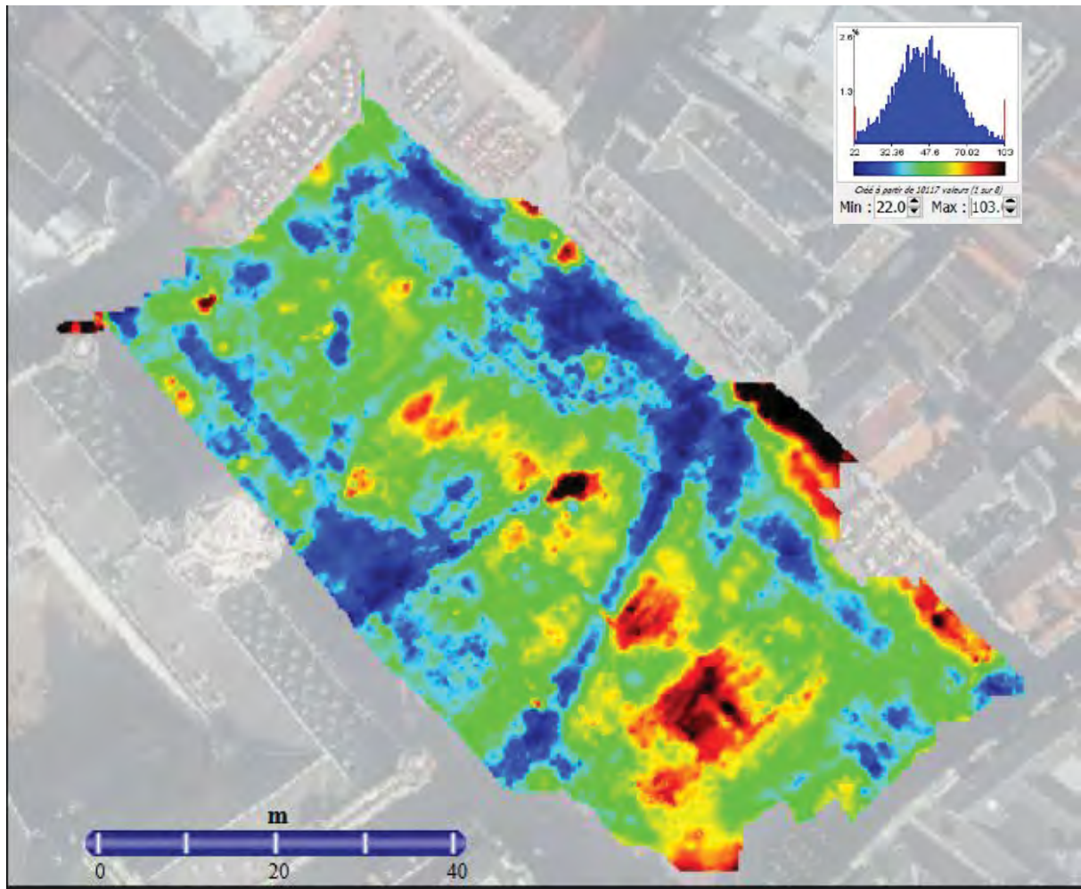
Fig. 2. Apparent resistivity data obtained with channel2 (0m to 1m) of the MP3 prototype (charge coupled resistivitimeter) overlaid on orthoimagery (June 2016, source: cirb.brussels, Open licence).
