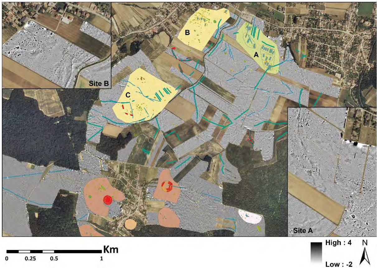
Fig. 1. Magnetometry data overlain with the aerial and magnetic interpretation and the three sites (A, B & C) used in the study.
