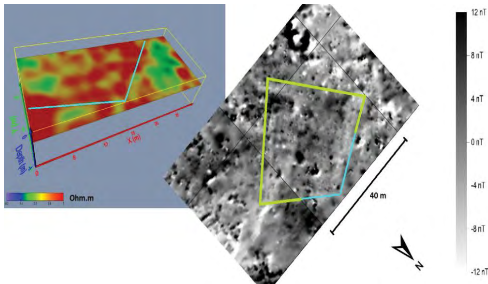
Fig.2. The left picture shows a 3-D model of the house. The light blue lines indicate the outer walls of the house (ERT instrument 4point light 10W, electrode spacing 0.5m x 0.5m).
