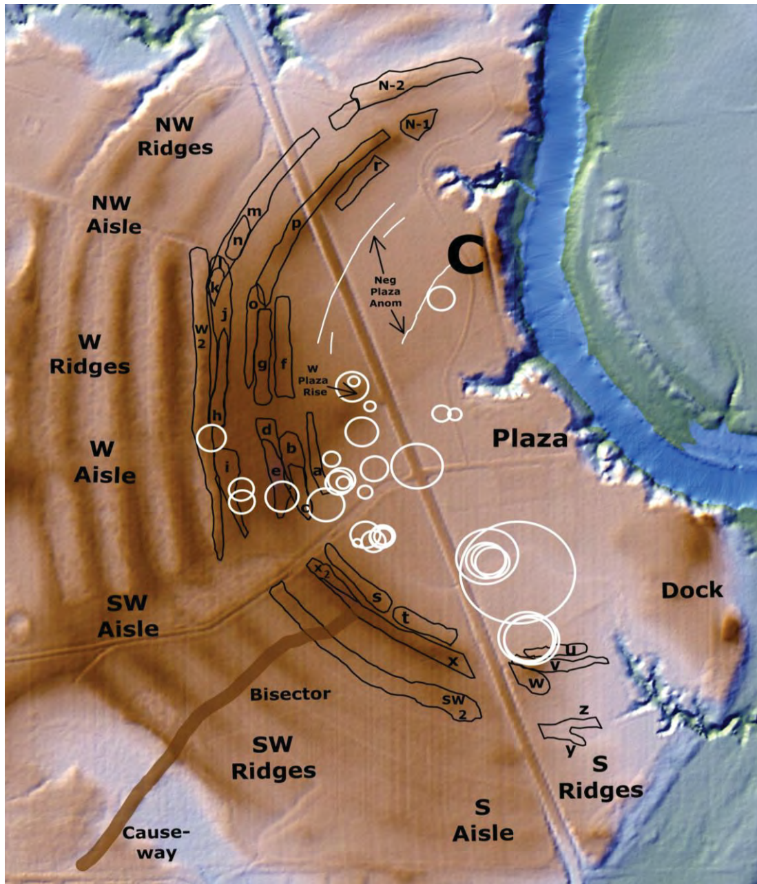
Fig. 3. Location of ridge components and post circles based on interpretation of the magnetic data. Traces of the Bisector ridge are seen in the magnetic data and early aerial photographs.
