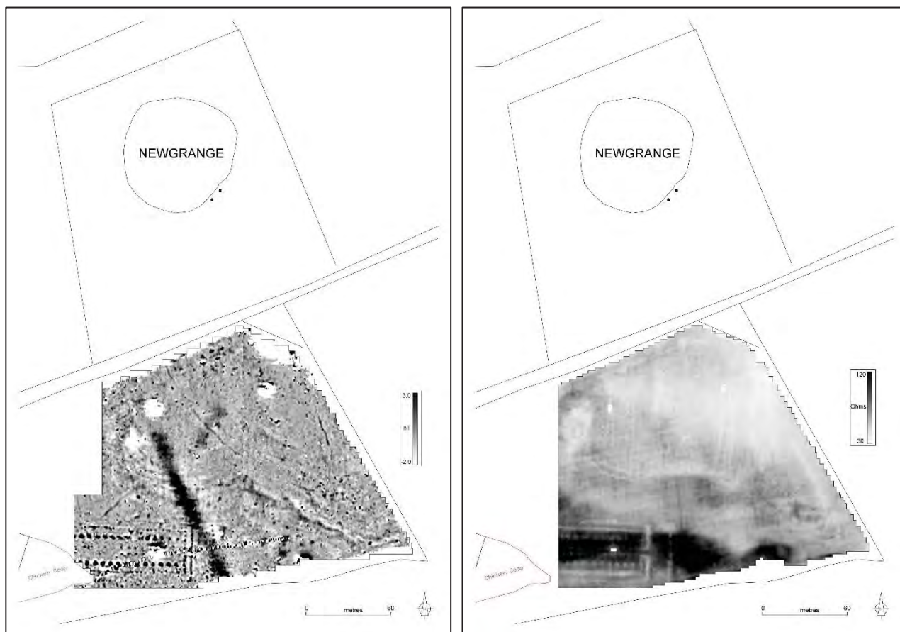
Fig. 1. (left) Magnetometer data and (right) earth resistance data, south of Newgrange passage tomb.
