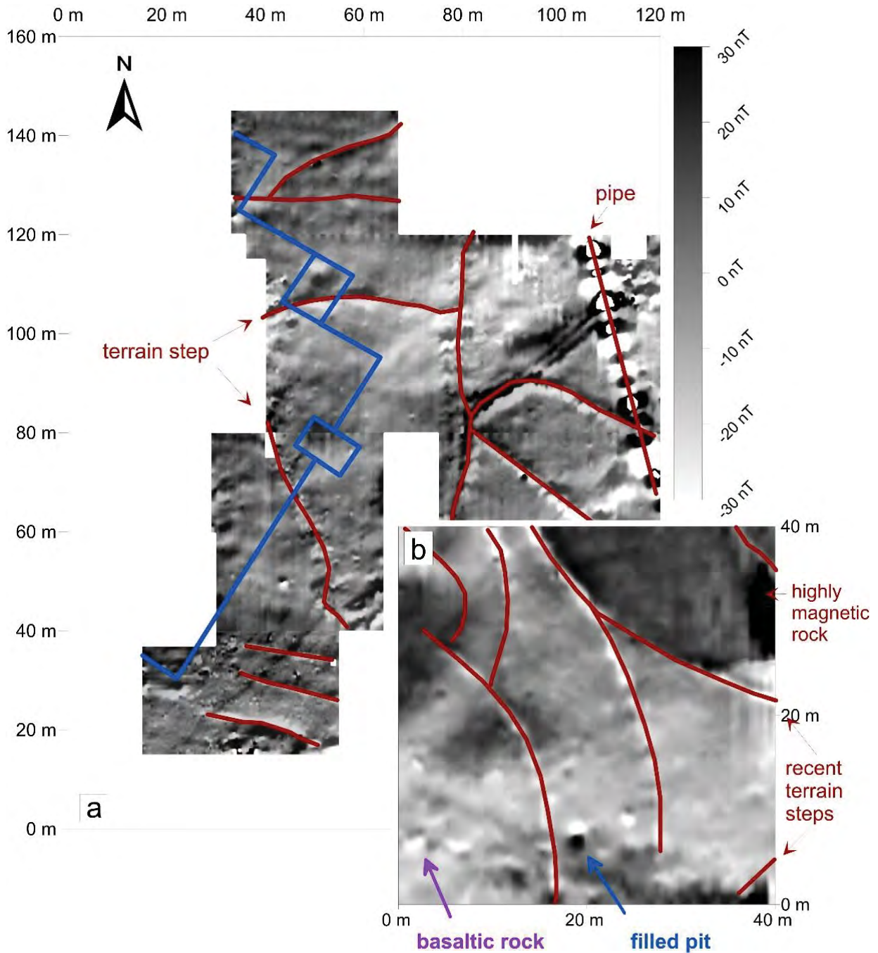
Fig. 3. a) Magnetogram of the survey area in the south of the Grat Be'al Gebri. Caesium Magnetometer, Scintrex SM4G-Special and Geometrics 858 in duo-sensor configuration, sensitivity \pm 0.01 nT, sampling interval 25cm x 50cm, total field in Yeha 11/2019 c. 37,500 \pm 100 nT. Magnetic inclination of around 15°. Geological structures and recent field boundaries are marked red. In blue, the detected archaeological feature with similarities to the monumental buildings of Yeha.
