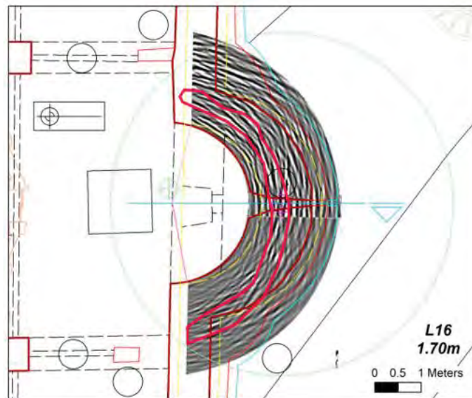
Fig. 3. GPR cross section on a semi-circular church wall at a height equal to 1.70m above the church floor. The red rectangle annotates a reflection possibly caused by a vertical internal surface within the wall structure. This reflection is seen in all the cross sectional GPR images collected on this wall.
