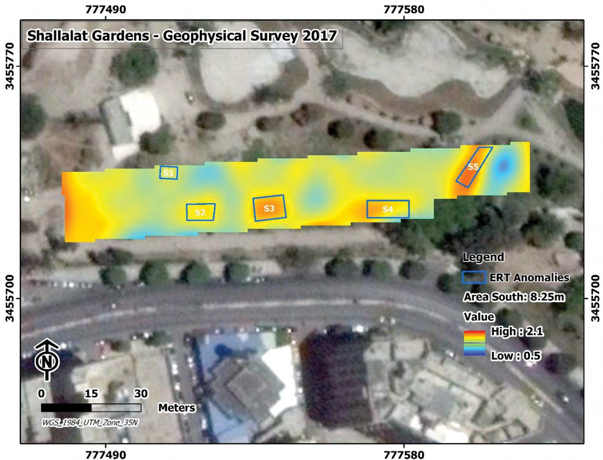
Fig. 3. Resistivity depth slice of 8.25m of the southern area in Shallalat gardens. The axis units in metres and the resistivity is in Ohm.m.
