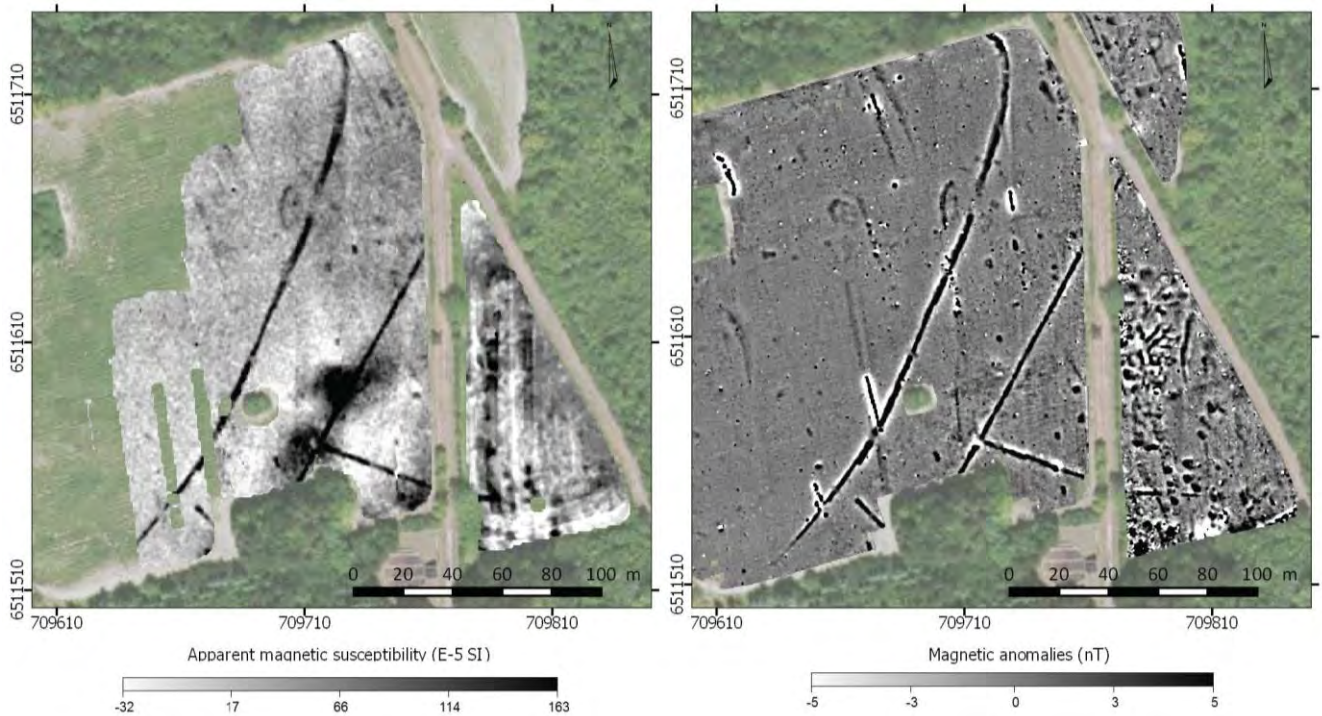
Fig. 2. Apparent magnetic susceptibility (left) and magnetic data (right) map of the central area of the site.
