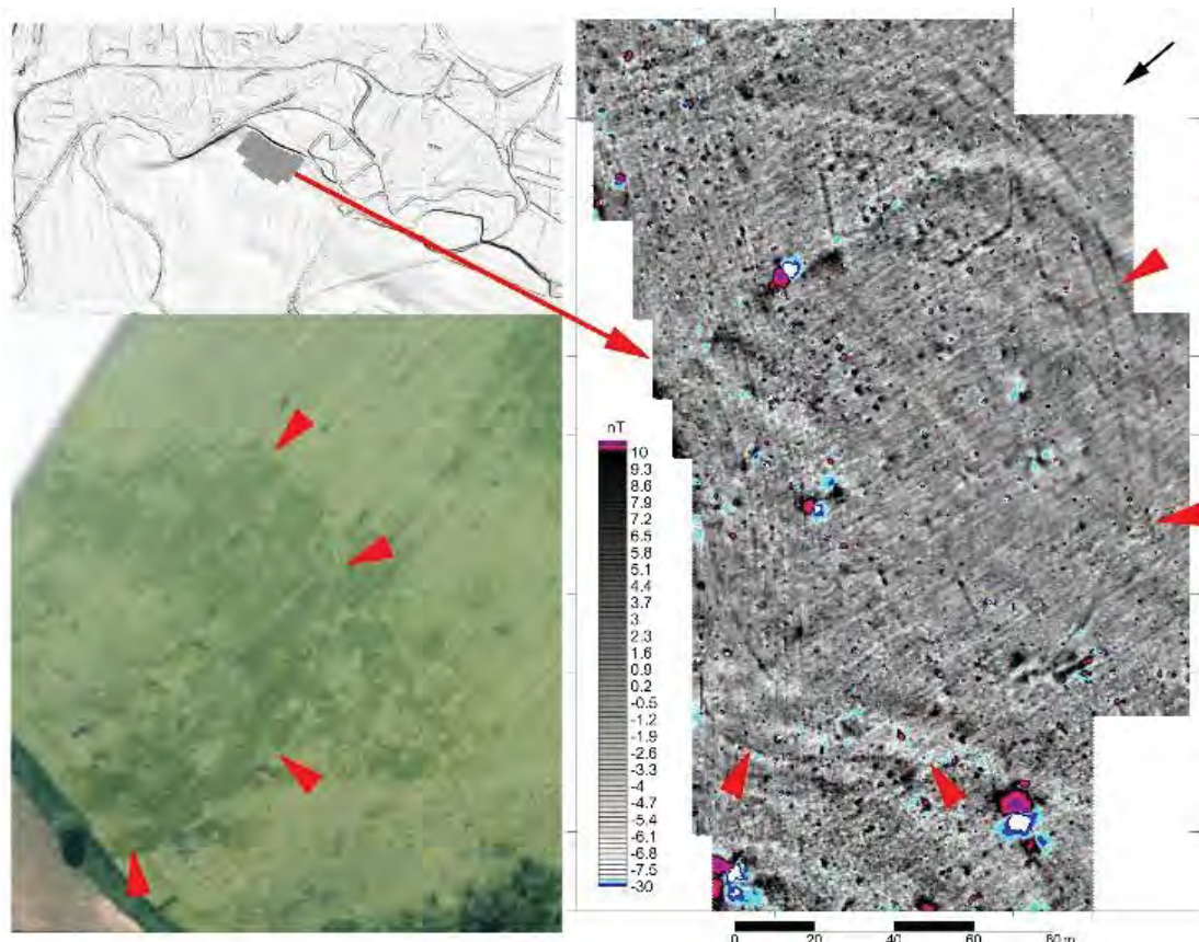
Fig. 1. Budyně n. O., Litoměřice district. Comparison of magnetometer survey and older aerial prospection of the polycultural site with Eneolithic enclosure and abandoned remains of the medieval village of Mileticko (source: Smrž; lidar: www.cuzk.cz ; survey: Křivánek 2016; surveyed area: approx. 2.7ha; Sensys 5-channel push-cart fluxgate gradiometer system; sampling interval: 0.5m x 0.2m).
