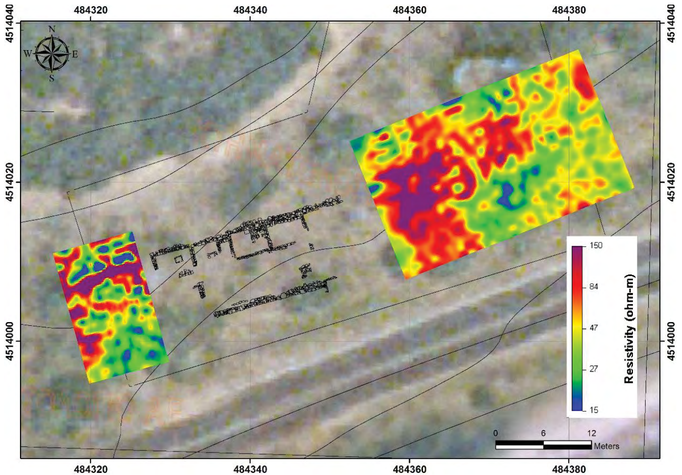
Fig. 2. Resistivity distribution (slice) at the depth of about 1.0m in ancient Argilos (Bonias et al. 2017).
