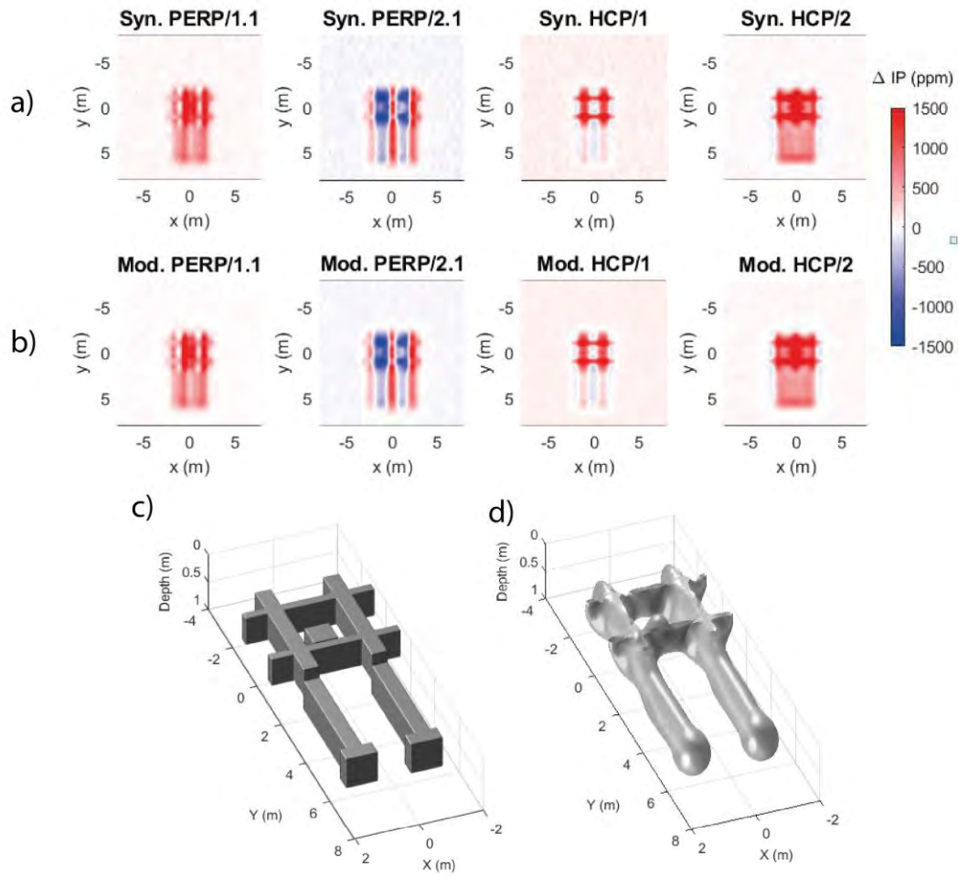
Fig. 1. Synthetic test with noisy EMI four-configuration in-phase data modelled at a height of 0.2m above ground. The data are interpreted in terms of an anomalous in-phase field. a) Synthetic dataset with an added 50 ppm random noise. b) Modelled data after 3D MCD imaging. c) True structure, which served to generate the synthetic dataset, with a relative magnetic permeability contrast of the background. d) Reconstructed subsurface model shown with an iso-surface representation.
