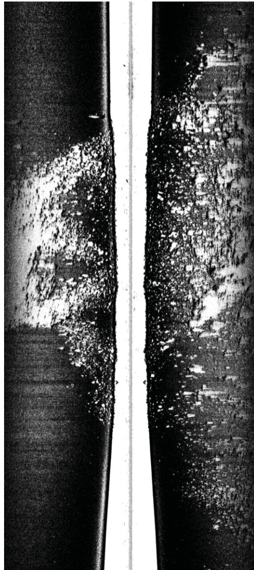
Fig. 5. Sonar data of a section across the site. The white / grey areas represent features standing proud of the seabed, in this case stone material, with the natural (flat profile) seabed being dark coloured / black. This demonstrates the distinct unusual aspect of the material, and shows a clear delimitation of the site. The perimeter of the sites may represent a collapsed wall, with a small structure attached to the enclosure wall at the top centre of the scan. The central white band of the image highlights where no data has been captured as this is directly below the sonar unit. (Image source: authors).
