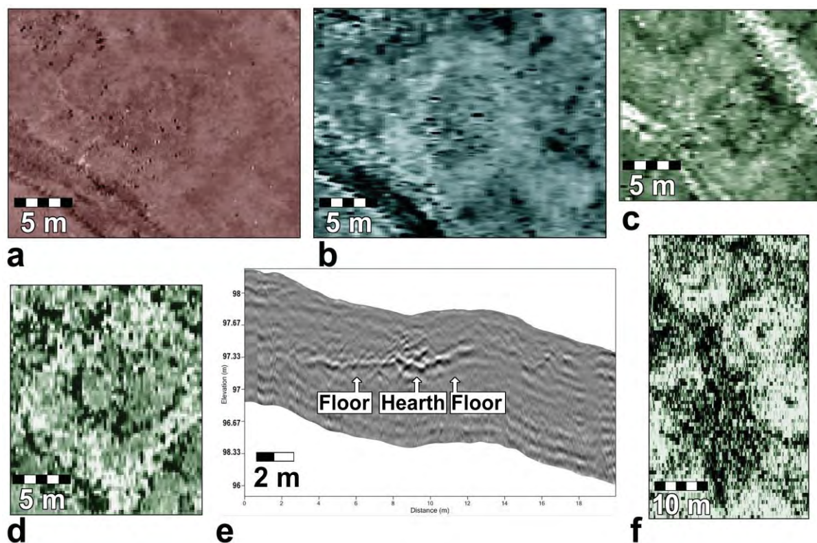
Fig. 1. Time-slice and GPR profile indications of lodges: a) shallow time-slice in a normal-moisture year, b) same area as (a) with identical settings but shortly after a very moist spring (note keyhole entryway, lower right), c) rectangular lodge extending under footpath (white line, upper right), d) small circular lodge atop larger rectangular one, e) terrain-corrected profile through lodge centre, f) segment through village showing multiple lodges and well-indicated central hearths.
