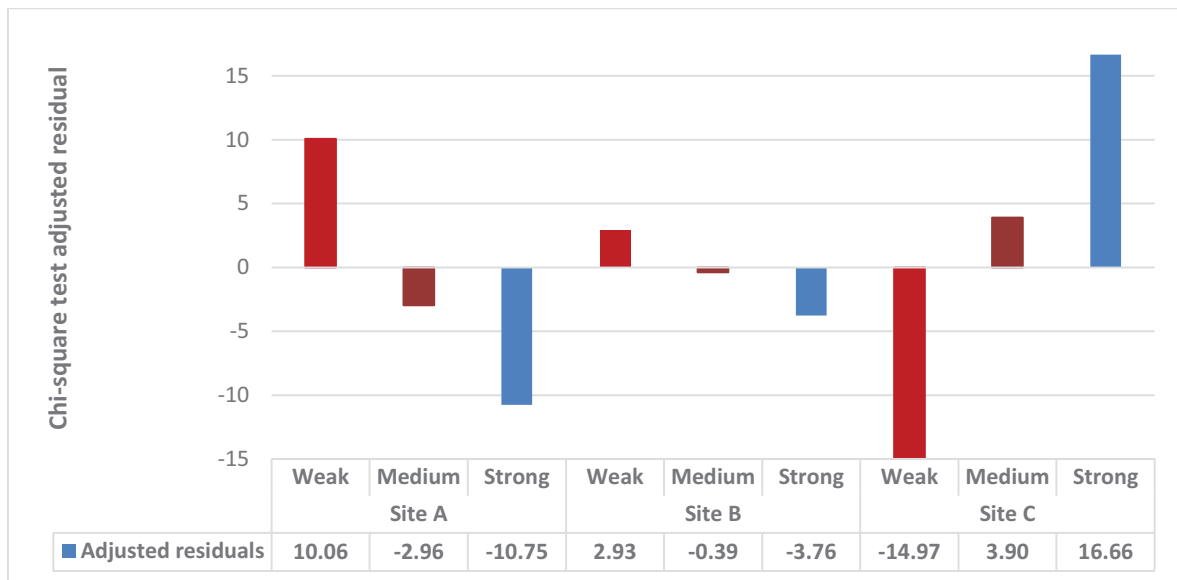
Fig. 3. The chi-square adjusted residuals for the frequencies of weak (<5nT), medium (5-10nT) and strong (>10nT) magnetic anomalies at sites A, B and C showing the different magnetic characteristics for these, with a trend for weak anomalies at site's A and B and medium and strong anomalies at site C.
