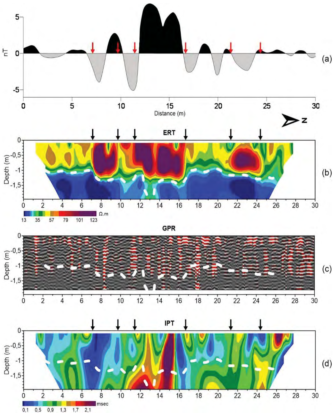
Fig. 2. Geophysical results obtained from the example profile shown in Fig. 1, (a) magnetic gradiometry, (b) ERT, (c) GPR and (d) IPT. Arrows indicate the boundaries of particular magnetic anomalies and resistive structures. White dashed lines show the transition between archaeological context and bedrock according to the ERT result.
