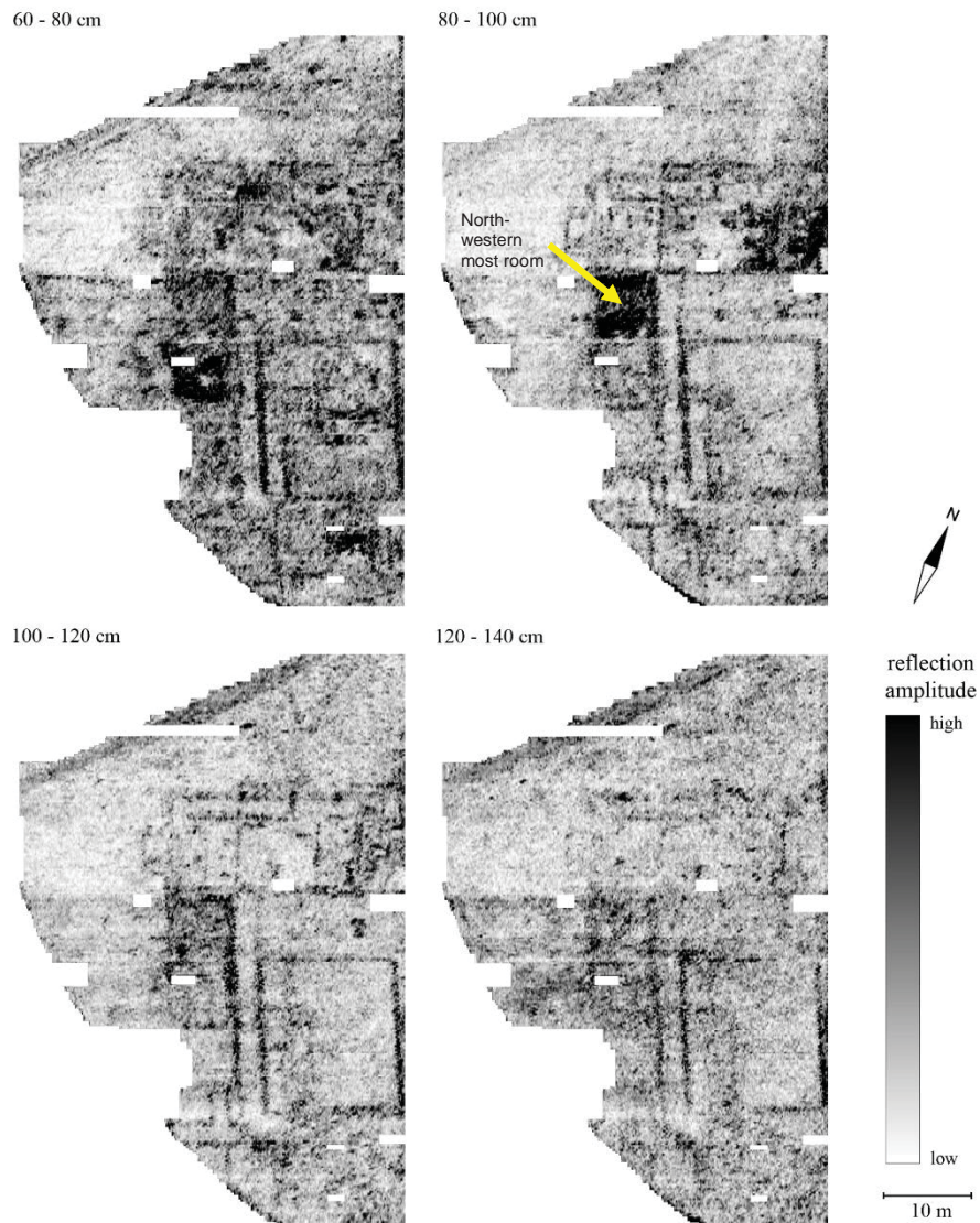
Fig. 1. Selection of depth slices of the GPR survey. GSSI SIR-3000 with 400MHz antenna, sample density: 2cm x 25cm, grid size: 67m x 46 m. The gaps in the depth slices are caused by trees.
