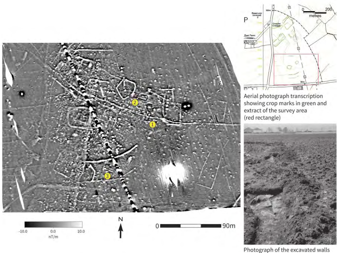
Fig. 3. Extract from the magnetic survey over the scheduled area which reveals a complex of pits and intercutting enclosures. Rectilinear negative anomalies at (1), (2) and (3) suggest buried wall footings. From its position the building anomaly at (1) is likely to be that excavated by Charles Bean in the 1950s (inset bottom right).
