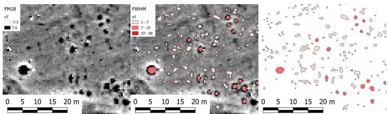
Fig. 1. (left) Fluxgate gradiometer data (FM18) from Guiting Power, (centre) overlaid with amplitude classified FWHM polygons and (right) the polygons on their own.
