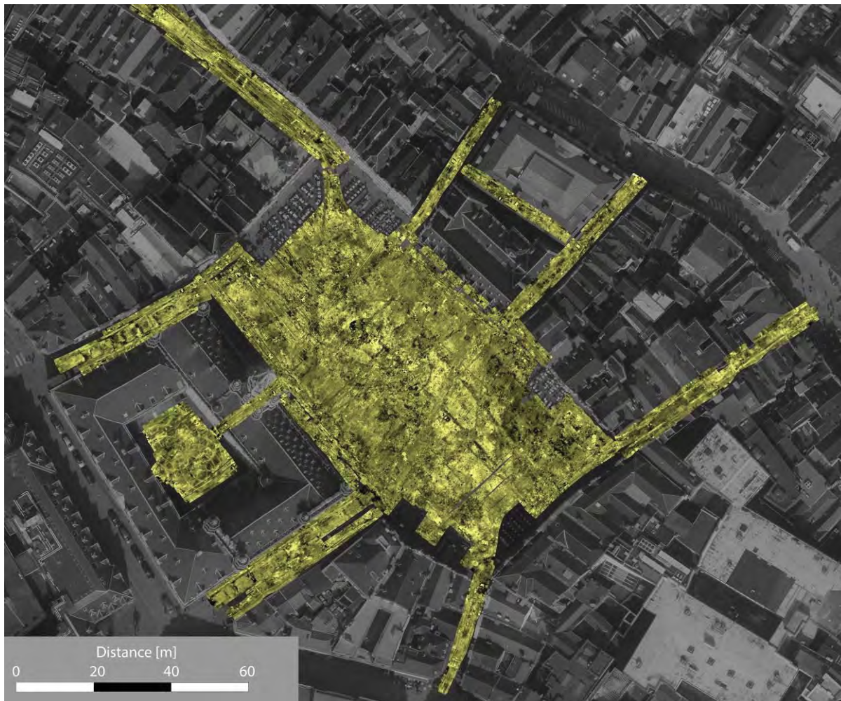
Fig. 3. 600MHz GPR phase time-slice centered on 0.25m overlaid on ortho-imagery (June 2016, source: cirb.brussels, Open licence).
