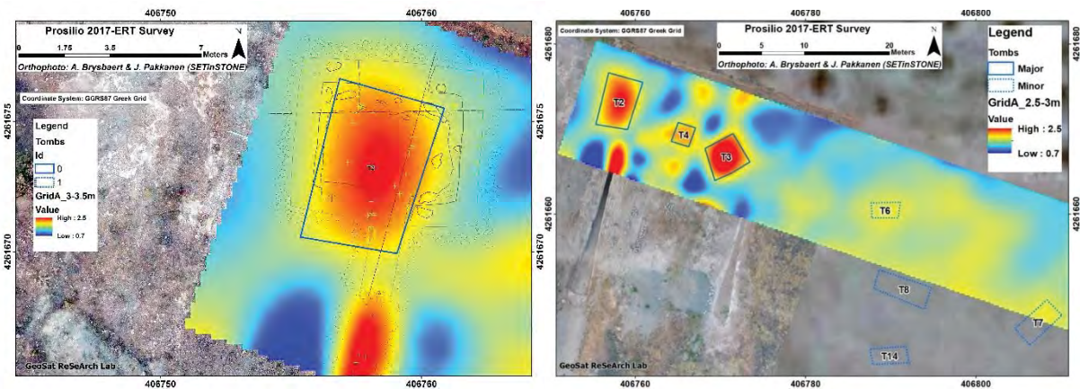
Fig. 3. (left) Resistivity depth slice of 3-3.5m over the known excavated tomb T2. (right) Resistivity depth slice of 2.5-3m from Grid A. Axes units in metres and resistivity in Ohm.m.
