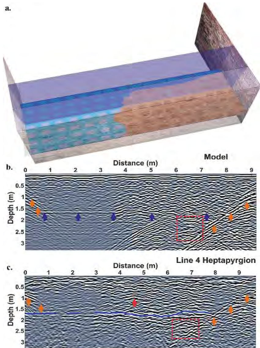
Fig. 5. a) A simulated 2D wall model fused with a 3D representation of the surveyed wall. b) Processed synthetic cross section of the wall model. Blue and orange arrows and the red rectangle indicate the different construction wall phases, lateral air reflections and distorted areas, respectively. c) Processed GPR cross section collected on one of the Heptapyrgion walls. Indicated are: the second construction phase of the wall (blue line), possible voids (red arrow), distorted region (red rectangle), lateral air reflections (orange arrows).
