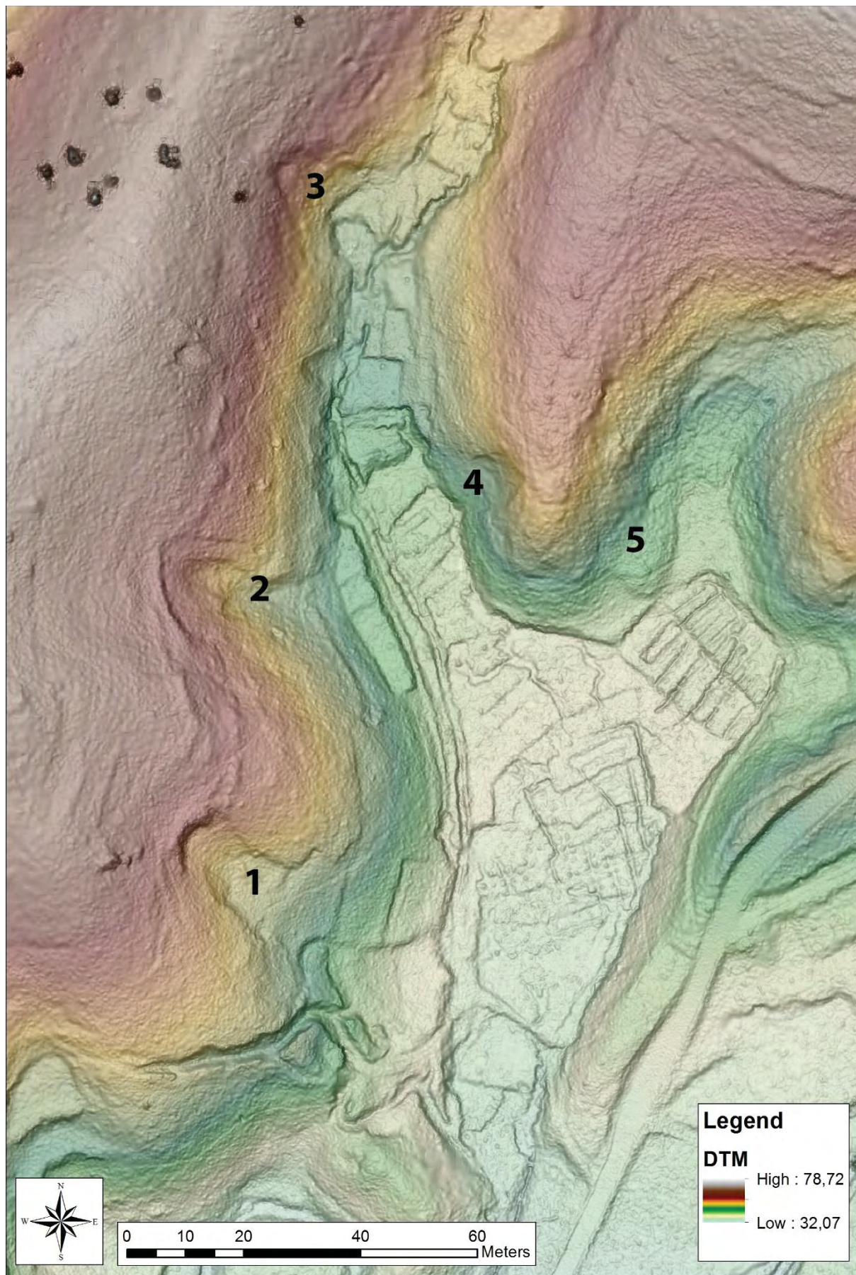
Fig. 3. Height-coded combination of slope and hillshade displaying a small valley with at least 5 potential Sue pottery kiln sites (1-5).
