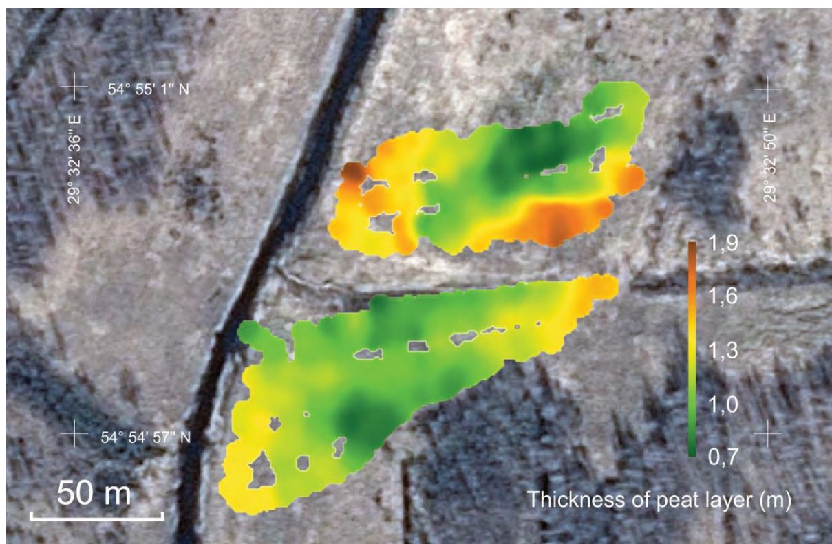
Fig. 2. Map of the peat layer's thickness.
