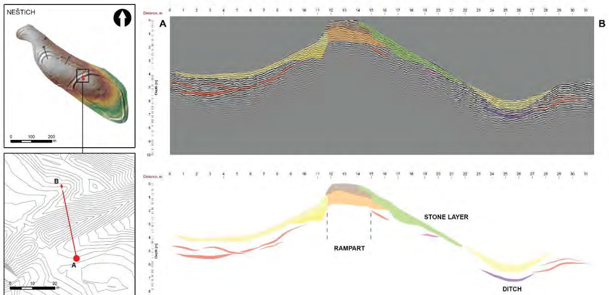
Fig. 2. GPR survey on early medieval hillfort Neštich, located in the south-west region of Slovakia. Results shows the inner structure of the rampart with the remnants of stone destruction and the original bottom of the filled outer ditch in front of the rampart.
