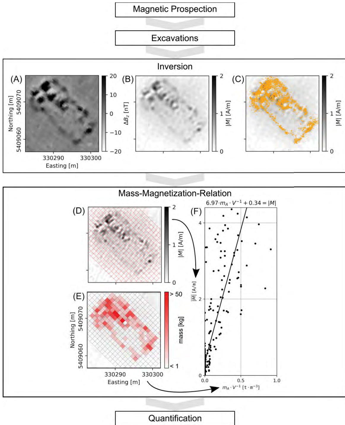
Fig. 2. Novel scheme for quantitative interpretation of magnetic prospection data with example data of the excavated megastructure. (A) Magnetic map, (B) calculated magnetization, (C) magnetization distribution overlaid with documented daub in the excavation (orange). Note that areas of increased magnetization overlap with the documented daub. (D) Magnetization distribution with excavation squares, (E) documented mass of daub and pottery per excavation square, (F) orthogonal distance regression of mass and mean magnetization per excavation square.
