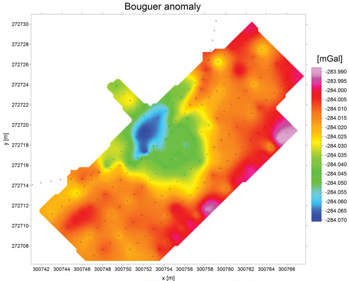
Fig. 3. Main result of microgravity data acquisition – the Bouguer anomaly map (correction density: 2200\text{kg}\cdot\text{m}^{-3} ) on the surface of the mound. Dots represent positions of measured gravity points. Units: milliGals ( 1\text{ milliGal} = 10^{-5}\text{ m}\cdot\text{s}^{-2} ).
