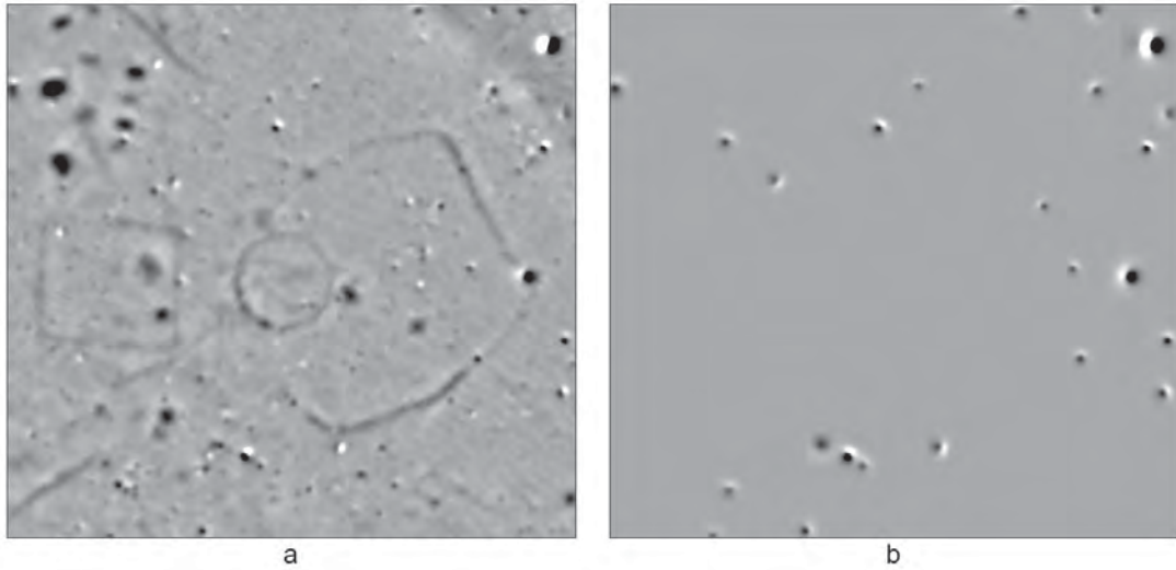
Fig. 1. a) Part of the magnetic prospecting of Podersdorf. b) Magnetic anomalies of the modelled near-surface dipoles. Visualization [white ... black]: [-2 ... +3nT].
