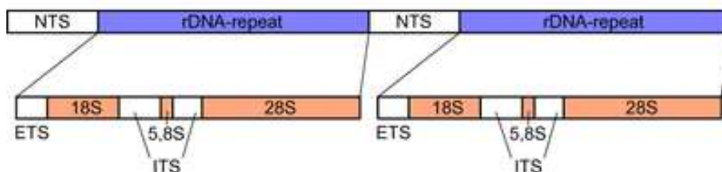
Fig. 2. Structure of eukaryote rDNA genes (18S, 5,8S, 28S) in tandem clusters with internal (ITS 1 and ITS2) and external (ETS) transcribed spacers and nontranscribed spacers (NTS). ( http://www.absoluteastronomy.com/topics/Ribosomal_DNA ).
