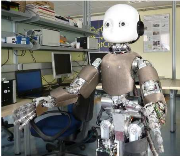
Figure 5. The iCub covered with artificial skin
