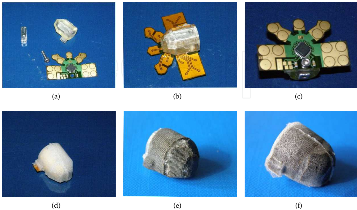
Figure 7. The production steps for the fingertip iCub
