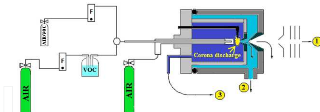
Figure 3. Schematics of APCI ion source and gas inlet system (1) quadrupole analyzer, (2) rotary pump, (3) diaphragm pump.
