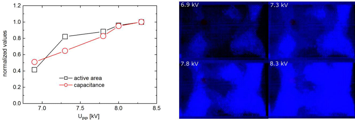
Figure 13. Left: Increase in active plasma area and increase in capacitance with respect to the operating voltage. Right: Photographs of the plasma operated at different voltages.
