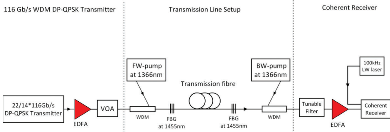
Figure 16. A schematic diagram of random fiber laser-based amplification scheme in unrepeated transmission.
