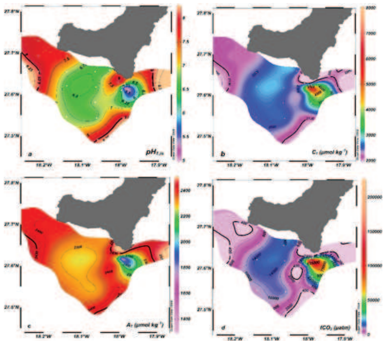
Figure 4. Distributions of the carbonate system variables at 5 m depth around the volcanic area. (a) \text{pH}_{T,\text{is}} in total scale at in situ conditions. (b) Total dissolved inorganic carbon ( C_T , \mu\text{mol kg}^{-1} ). (c) Total alkalinity ( A_T , \mu\text{mol kg}^{-1} ) (d) f\text{CO}_2 ( \mu\text{atm} ).
