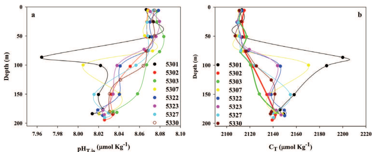
Figure 9. Yo-yo study for the carbonate variables (a) \text{pH}_{\text{T,is}} and (b) C_{\text{T}} ( \mu\text{mol kg}^{-1} ) at the station 53, during VULCANO cruise March 2013.
