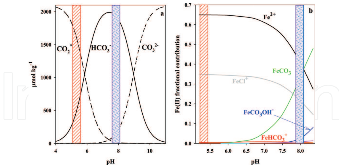
Figure 6. Chemical speciation of the (a) carbonate system and (b) Fe(II) in seawater as a function of the pH.
