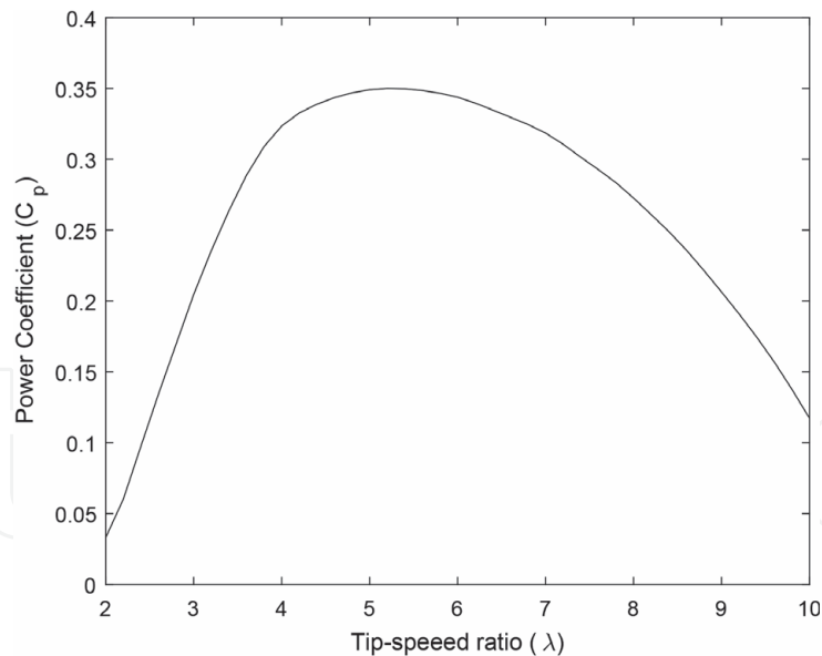
Figure 4. A typical C_p - \lambda for a tidal turbine [4]. Only indicative values are shown here; these values do not reflect the maximum C_p in a tidal turbine.
