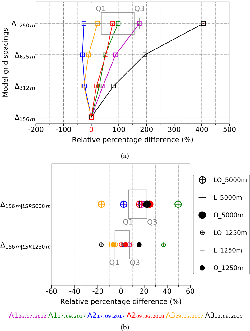
Figure 6.9.: RPD of areal mean daily total accumulated precipitation amount across LES model grid spacings ( \Delta_{1250m} , \Delta_{625m} , \Delta_{312m} , \Delta_{156m} ) of the control runs (□) (a) and in \Delta_{156m} of LO_1250 m run (⊕), L_1250 m run (+), O_1250 m run (●), LO_5000 m run (⊕), L_5000 m run (+), and O_5000 m run (○) (b) for the six simulated cases. Q1 and Q3 represent the first (25th) and third quartiles (75th percentiles).
