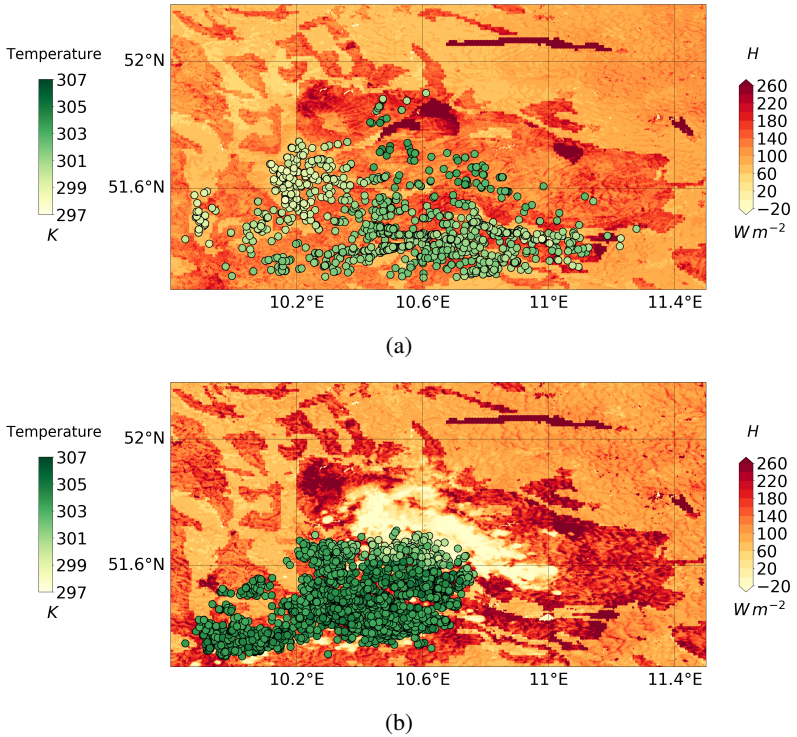
Figure 7.18.: Surface sensible heat flux (colour shaded) and the trajectory points (circles with air temperature in the colour shade) at 0900 UTC (a) and 1200 UTC (b) in \Delta_{156m} of case over A2, dated 09 June 2018.
