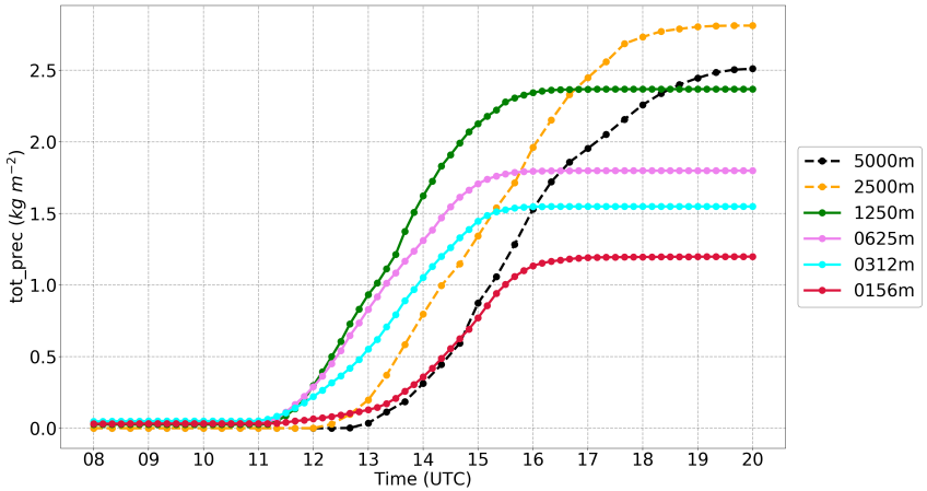
Figure B.9.: Time series of total accumulated precipitation for NWP ( \Delta_{5000m} , \Delta_{2500m} ), dashed lines, and LES model grid spacings ( \Delta_{1250m} , \Delta_{625m} , \Delta_{312m} , \Delta_{156m} ), solid lines, over A1, case: 17 Sept 2017.
