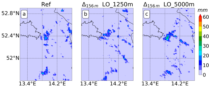
Figure 6.7.: Total accumulated precipitation from reference run ( \Delta_{156m} - control run) (a), \Delta_{156m} - LO_1250 m run (b) and \Delta_{156m} -LO_5000 m run (c) at 2000 UTC over A1, case: 26 July 2012.
