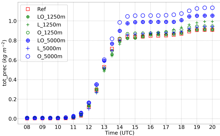
Figure B.16.: Time series of total accumulated precipitation from \Delta_{156m} - control run ( \square ), \Delta_{156m} -LO_1250 m run ( \oplus ), \Delta_{156m} -L_1250 m run ( + ), \Delta_{156m} -O_1250 m run ( \odot ), \Delta_{156m} -LO_5000 m run ( \oplus ), \Delta_{156m} -L_5000 m run ( + ), and \Delta_{156m} -O_5000 m run ( \odot ) over A2, case: 09 June 2018.
