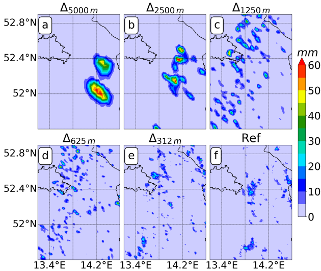
Figure 6.3.: Total accumulated precipitation patterns (colour coded) across the six model grid spacings ( \Delta_{5000m} , \Delta_{2500m} , \Delta_{1250m} , \Delta_{625m} , \Delta_{312m} and \Delta_{156m} ) at 2000 UTC over A1, case: 26 July 2012
