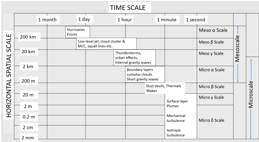
Figure 2.1.: Scale definition and the characteristic time and horizontal scales of different processes (adapted after Orlanski (1975))
