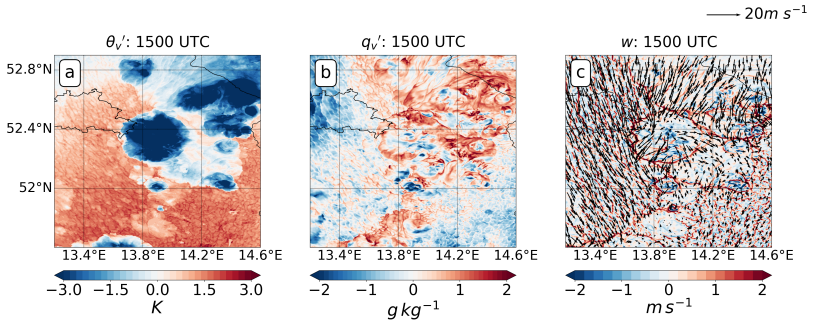
Figure 7.14.: Spatial pattern of virtual potential temperature anomaly \theta_v' at 10 m (a), specific humidity anomaly q_v' at 10 m, and vertical velocity at \approx 1 km (c) at 1500 UTC in \Delta_{156m} of case over A1, dated 26 July 2012.
