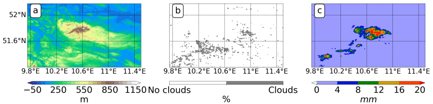
Figure 7.15.: Orography (a), cloud cover at 1250 UTC (b) and the resulting accumulated precipitation at 1500 UTC (c) in \Delta_{156m} of case over A2, dated 09 June 2018.
