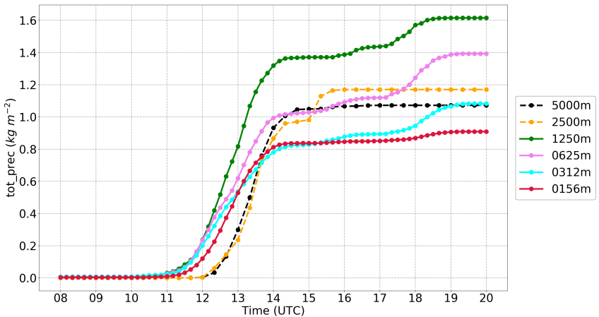
Figure B.10.: Time series of total accumulated precipitation for NWP ( \Delta_{5000m} , \Delta_{2500m} ), dashed lines, and LES model grid spacings ( \Delta_{1250m} , \Delta_{625m} , \Delta_{312m} , \Delta_{156m} ), solid lines, over A2, case: 09 June 2018.
