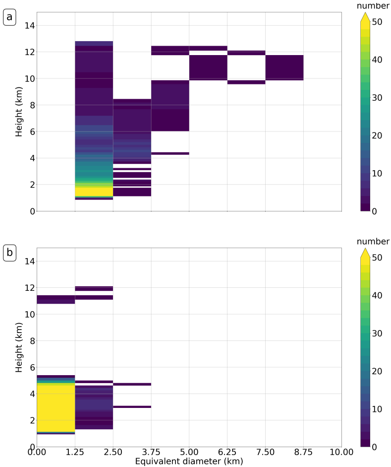
Figure 6.26.: Vertical distribution of equivalent diameter of clouds and number of clouds (colour coded) in \Delta_{1250m} (a) and \Delta_{156m} (b), respectively at 1200 UTC for case over A1, dated 26 July 2012.
