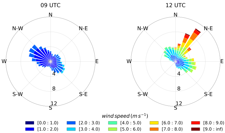
Figure 7.19.: Wind rose diagram for wind speed and direction over a region of convergence zone in the south west of Harz in \Delta_{156m} of case over A2, dated 09 June 2018.
