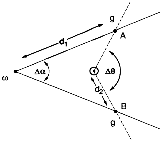
Figure 3.5. Double image of a galaxy behind a cosmic string. \odot is the axis of the string, \omega is the observer and g is the galaxy.
