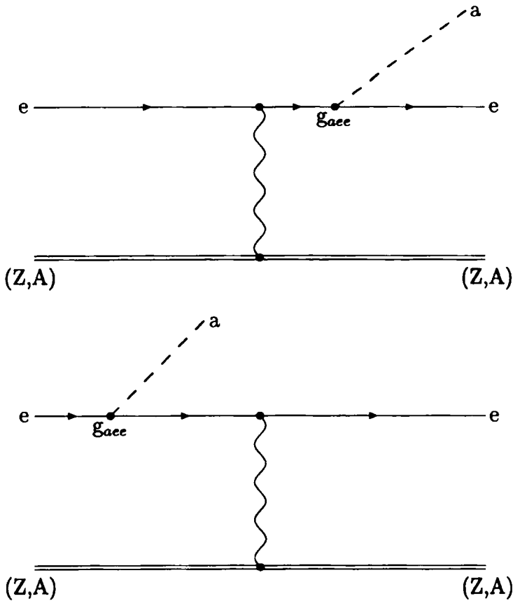
Figure 5.2. Axion bremsstrahlung.
