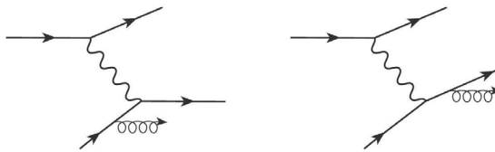
FIGURE 15.8 Electron-quark scattering with single-gluon emission
