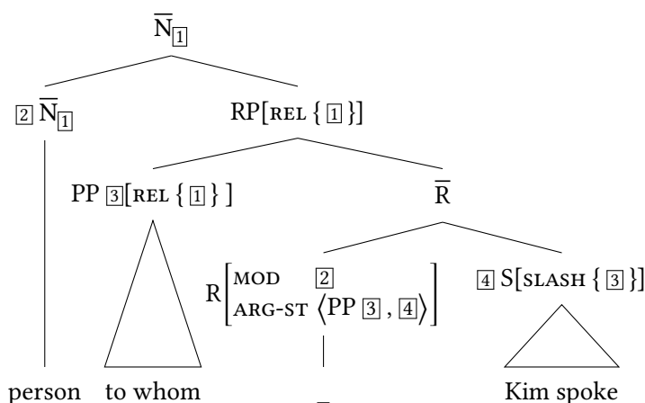
Figure 3: A Pollard & Sag (1994)-style structure involving a finite wh -relative clause
