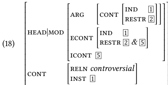
Figure 2: Kasper’s analysis of potentially controversial
