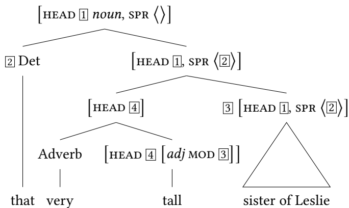
Figure 4: Adnominal modifiers
