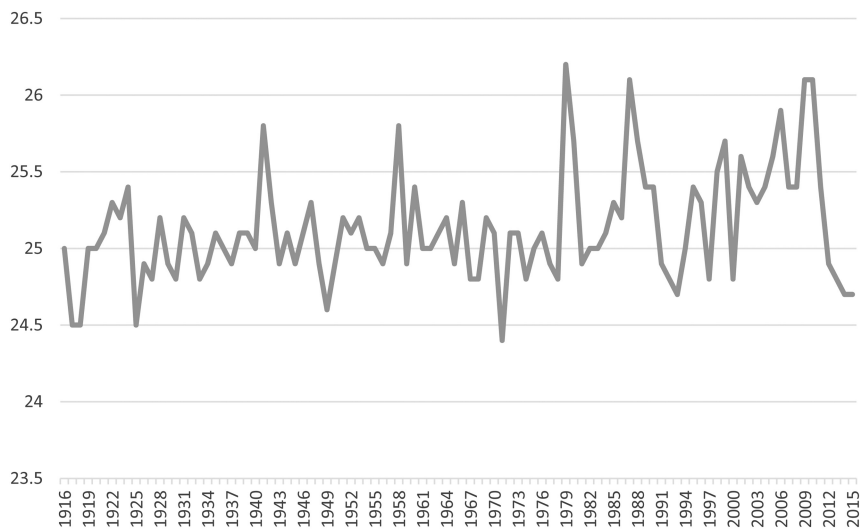
Figure 4.3 Average temperature (°C) from 1916 to 2015. Source: The World Bank's Climate Change Knowledge Portal.
