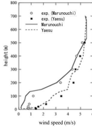
Figure 4: Mean velocity profiles at Marunouchi area and Yaesu area.
