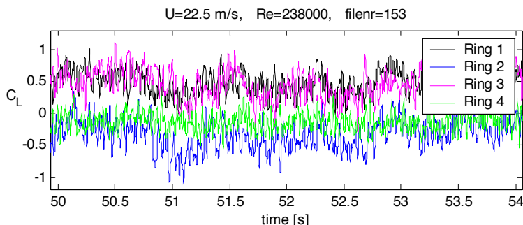
Figure 35: Time histories of lift coefficient at Re=238000 , fixed cylinder inclined at 59.3^\circ to the approaching flow
