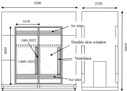
Fig.1 Model with four double skin windows
