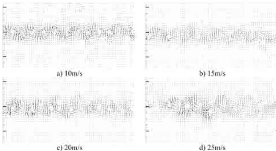
Figure 6: Wake flow field of thin plate section
