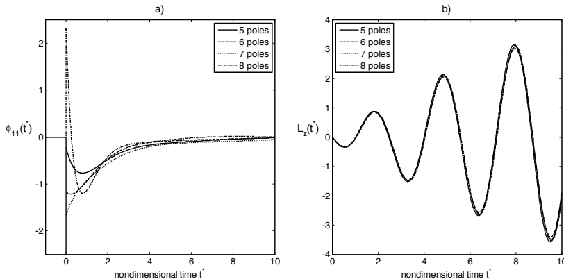
Figure 1: (a) Step response functions \Phi_{11} (amplitude cutoff at zero t^* ) (b) Reference forces L_z
