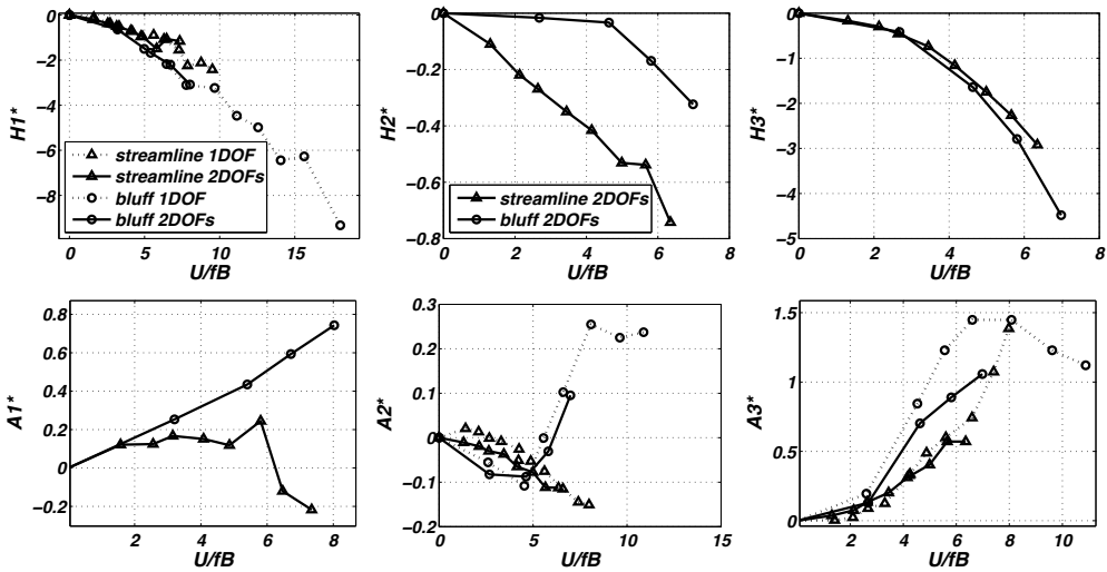
Figure 1: Aerodynamic derivatives of the tested sections obtained by modified method; pictures including four graphs represent the cases, where both single and coupled system measurements have been performed; rectangular body: \circ , bridge-like deck: \triangle .
