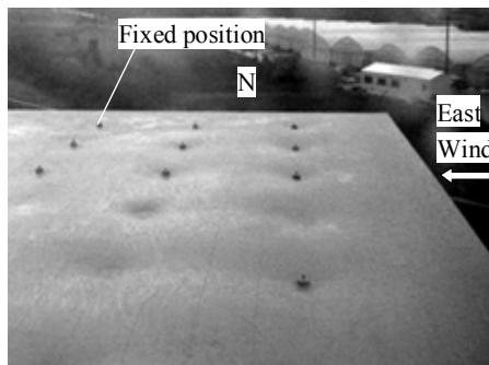
Figure 1: billowing condition of waterproofing membrane on roof during Typhoon No.12 in Japan
