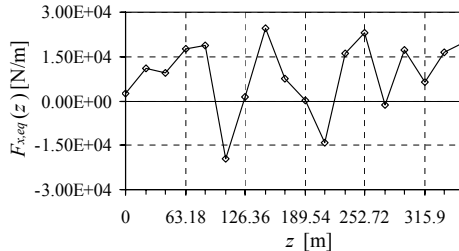
Figure 2: ESF F_{x,eq}(z) obtained by using spectral eigenfunctions and imposing 14 conditions.
