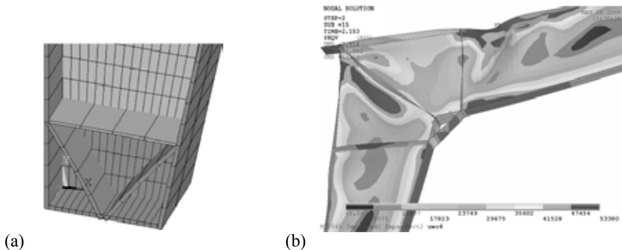
Figure 3: (a) Triangular stiffener at column support; (b) left haunch, von Mises stresses in psi (1 psi= 0.006895 MPa) (Duthinh et al., 2008).
