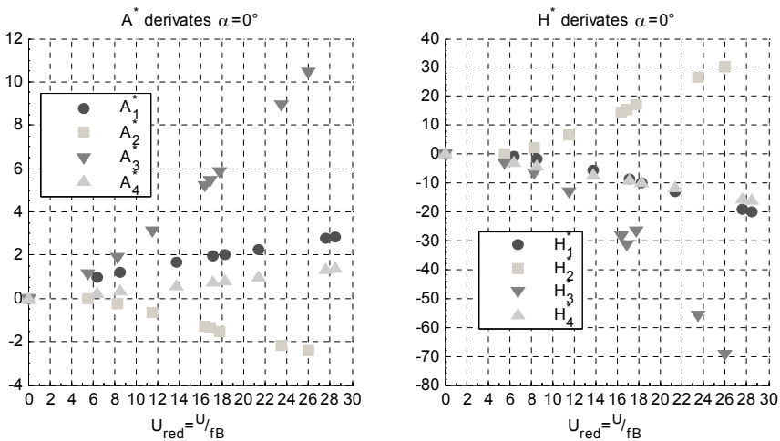
Figure 2: Flutter derivatives at 0^\circ angle of attack plotted versus reduced velocity.
