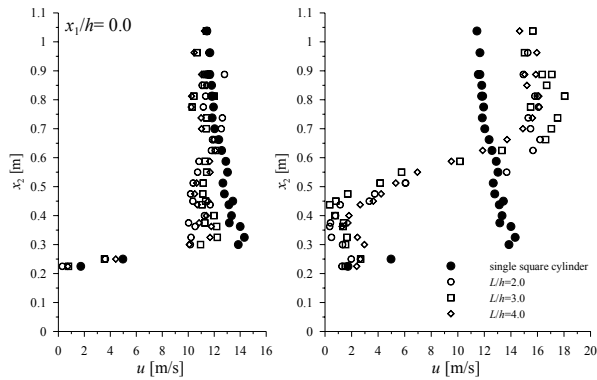
Figure 4: The graphs of velocities in vertical cross-section under square cylinder which is: a) the upstream model; b) the downstream model.
