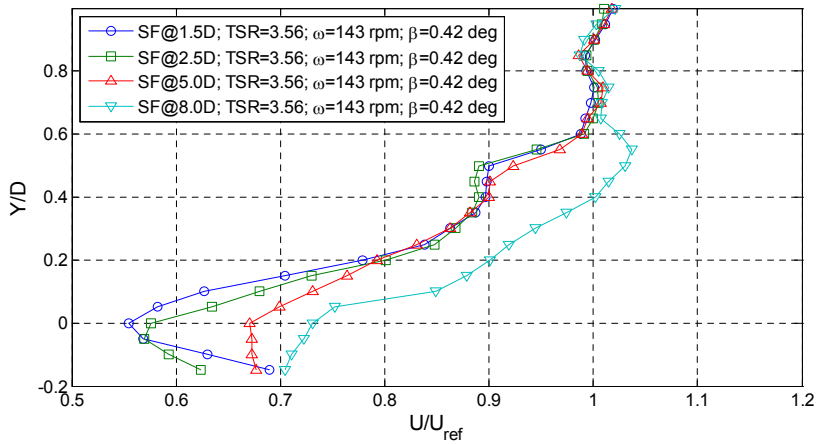
Figure 2: Horizontal velocity profiles at different distances from the wind turbine.
