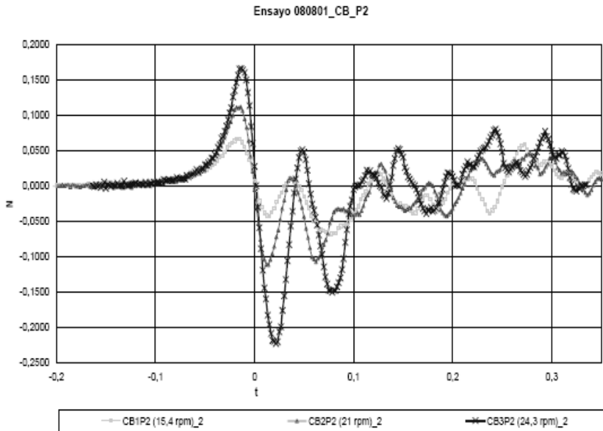
Figure 3: Variation of the transversal force acting on the plate N [N] with the time [s]. The legend indicates the angular rotation speed of the centrifuge arm. The plate is placed parallel to the motion direction.
