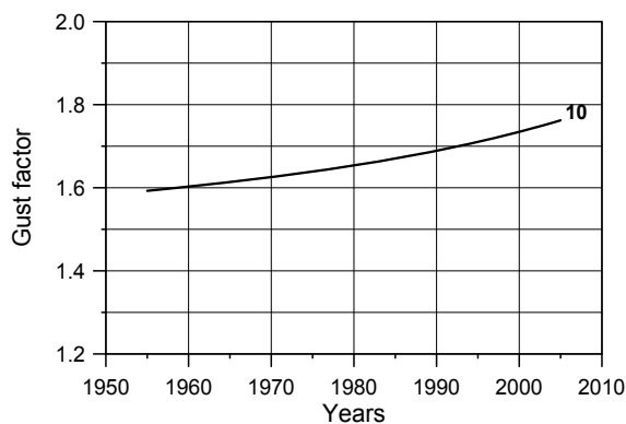
Figure 2. Annual maximum gust factor as a function of years of measurements; meteorological station in Wroclaw, sector 10
