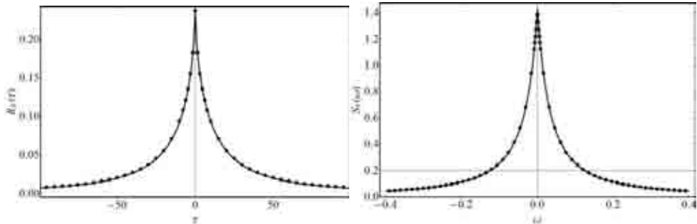
Figure 2: Comparison between the exact (continuous line) and the approximated (dotted line) Kaimal's correlation function (left panel) and PSD (right panel).
