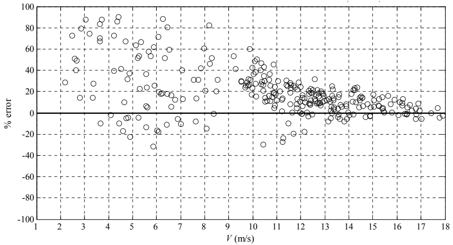
Figure 2. Relative error in the 30-minutes-ahead forecast (non-exceedance probability 95%).
