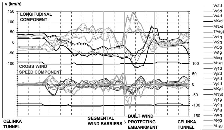
Figure 1: Measured three-second wind speed obtained during four measurement series
