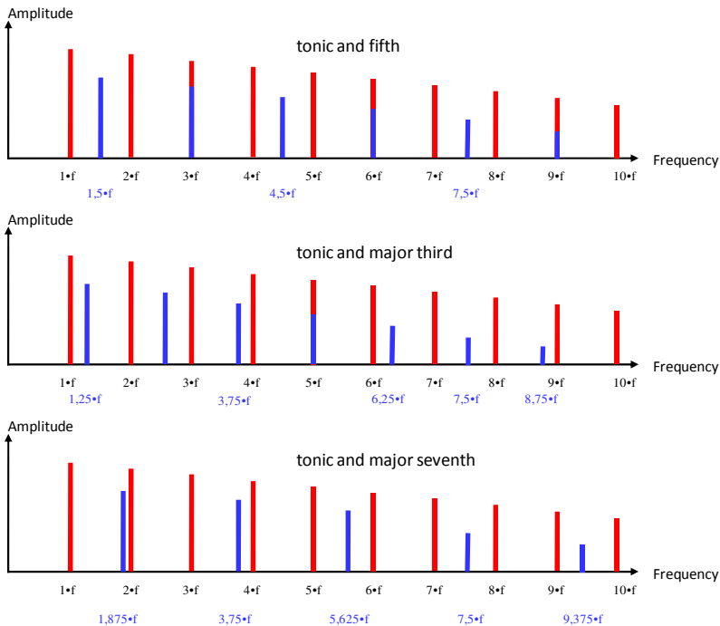
Figure 12: Overtone relations for different intervals, Spitzer (2008)
