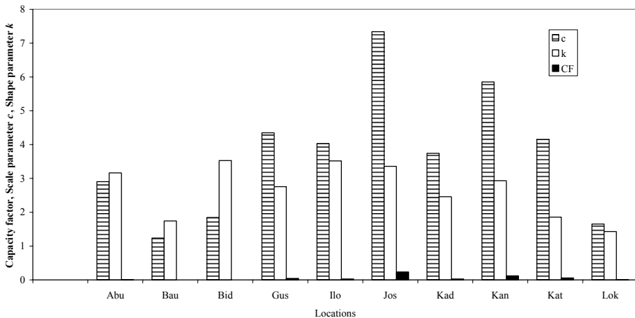
Figure 1: Annual scale and shape parameters, annual capacity factors at a height of 50 m for Abuja, Bauchi, Bida, Gusau, Ilorin, Jos Kaduna, Kano, Katsina and Lokoja.
