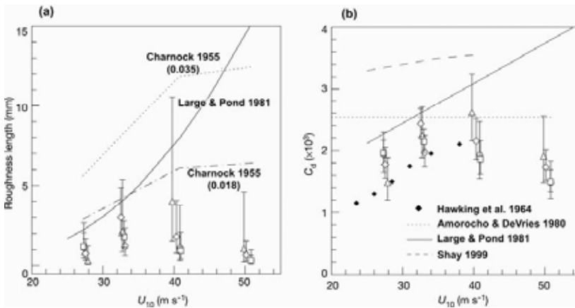
FIG. 4. Momentum exchange quantities as a function of U_{10} . Vertical bars represent the range of estimates based on 95% confidence limits and the symbols represent the different layer depths used in the profile method: \circ 10–100, \_ 10–150, \Delta 20–100, \diamond 20–150 m. (a) z_0 from GPS sonde profiles (symbols) and Large and Pond (1981) relationship (solid line) and Charnock (1955) relationships for comparison (dotted line, \lambda = 0.035 ; dashed-dot line, \lambda = 0.018 ) and (b) C_D with relationships and values from tropical cyclone budget studies. Adapted from Powell et al. (2003).
