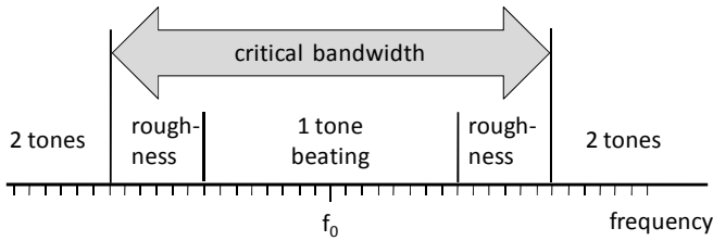
Figure 11: Critical bandwidth, Pierce (1998)
