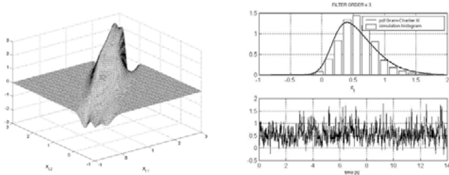
Figure 1: on the left, the function h(\mathbf{y}) obtained for an order 3 autoregressive filter; on the right, above the target distribution with the histogram of a realization and below a window of the realization itself.
