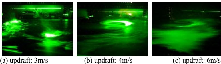
Figure 3: Flow visualization of vortices with horizontal shear flow for various updraft speeds
