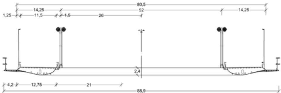
Figure 3: Cross-section of the deck with main suspension cables spaced apart of 52 m.
