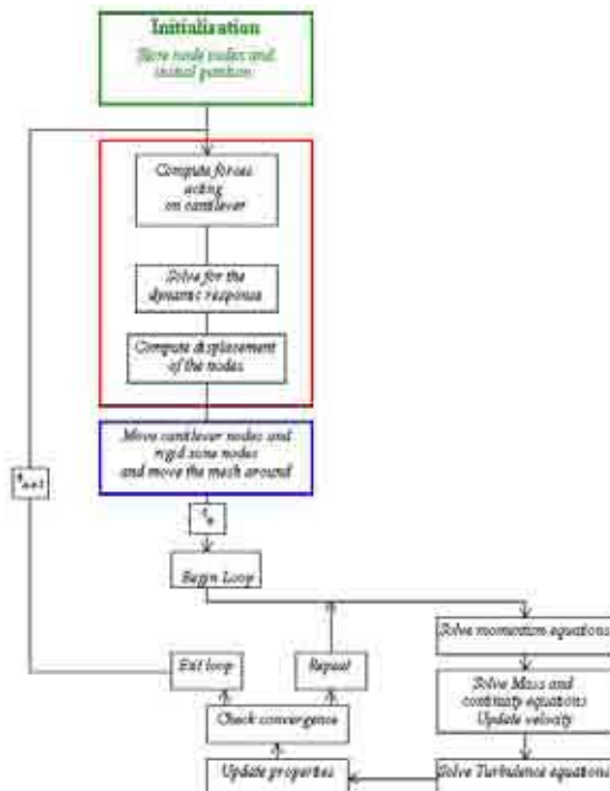
Figure 1: Diagram of the sequential fluid-structure coupling
