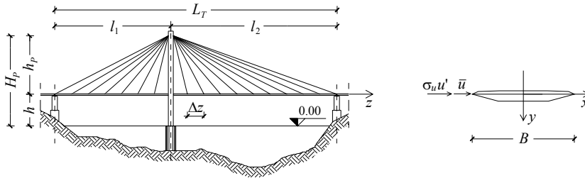
Figure1: Cable-stayed bridge under examination.
