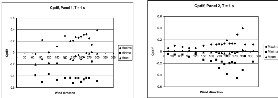
Figure 4: Differential pressures over both panels; negative values represent uplift loads; positive values represent forces directed to the roof.
