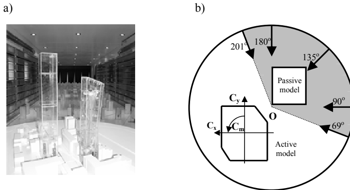
Figure 2: a) Model of the building in the working section of the wind tunnel- case of two high-rise buildings, b) wind attack directions during experiments.
