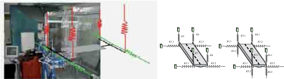
Figure 3: Spring support system of a sectional model deck in wind tunnel.
