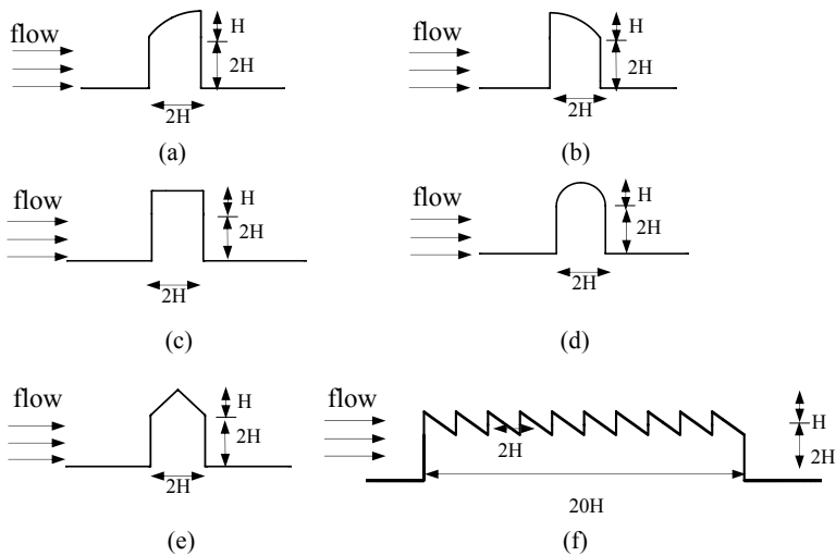
Figure 2: shapes of higher roofs and the computational zone
