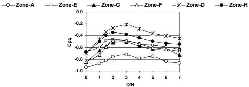
Figure 3. Variation of C_{pq} on roof surface in presence of boundary-wall
