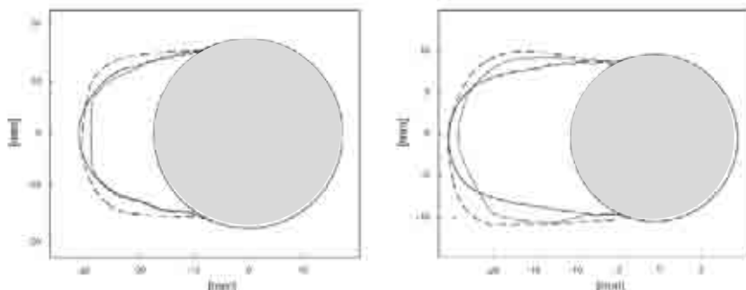
Figure 28: Ice accretion on single cables with different diameter
