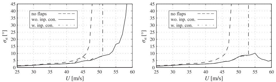
Figure 3: System response to a gust disturbance; for kinematically coupled flaps that are moved in the same direction on the left, for separately driven flaps on the right. (abbr.: w. / wo. inp. con.: with / without input constraints)
