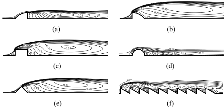
Figure4: Distribution of \sqrt{k}/U_0 around the roofs lower greenhouses
