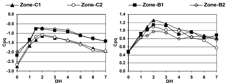
Figure 4. Variation of Net C_{pq} of overhang in presence of boundary-wall a) - C_{pq} b) + C_{pq}
