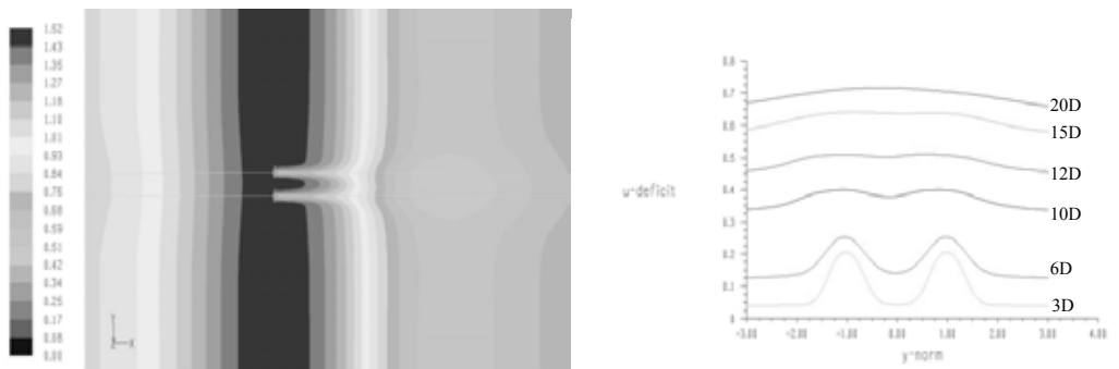
Figure 4: normalized x-velocity contours and velocity deficit – RSM
