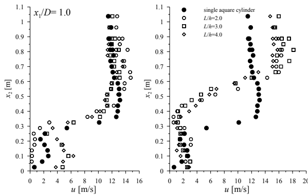
Figure 5: The graphs of velocities in vertical cross-section behind square cylinder (at x_1/h=1.0 ) which is: a) the upstream model; b) the downstream model.
