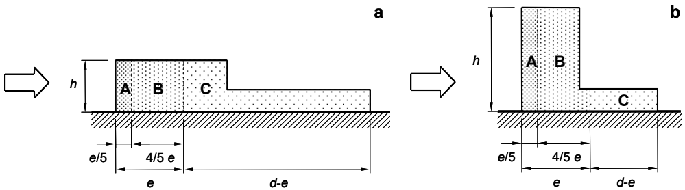
Figure 2: different pressure zones for buildings with non uniform heights (Fig. H.14 from CNR-DT 207/2008)
