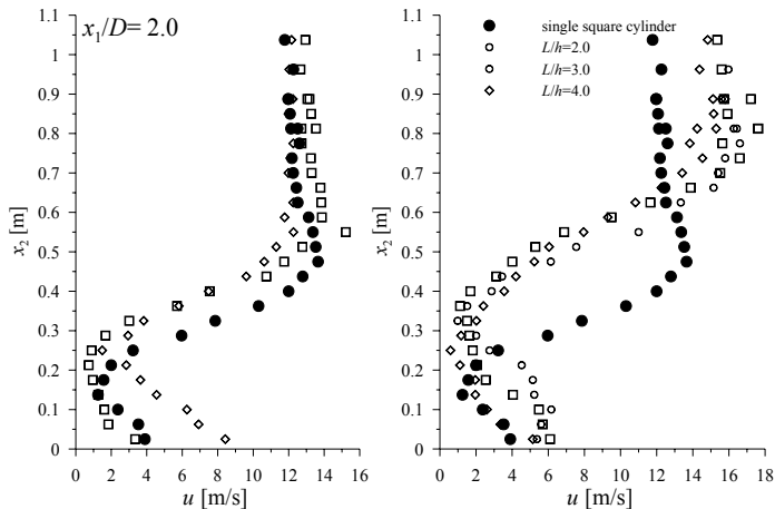
Figure 6: The graphs of velocities in vertical cross-section behind of square cylinder (at x_1/h=2.0 ) which is: a) the upstream model; b) the downstream model.
