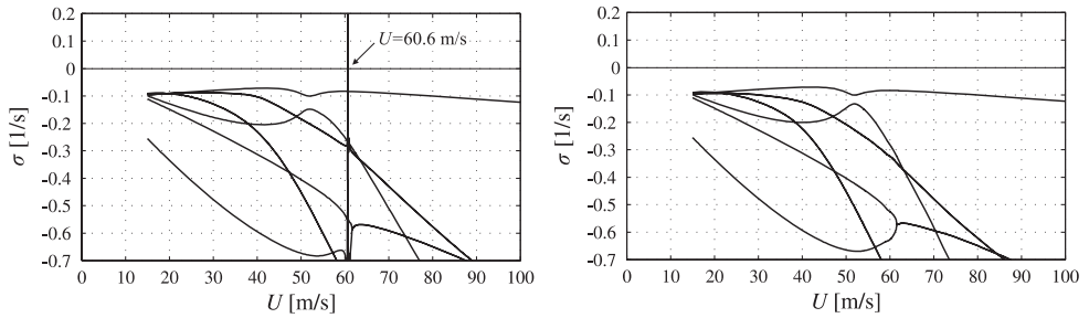
Figure 2: Eigenvalues of the aeroelastic system; controlled with kinematically coupled flaps that are moved in the same direction on the left, controlled with separately driven flaps on the right.
