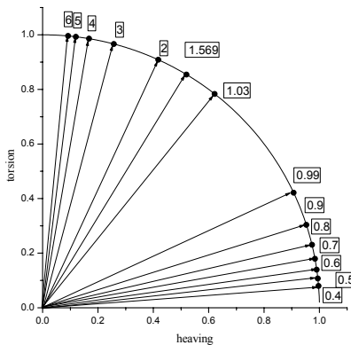
Figure 4: Flutter modality vectors
