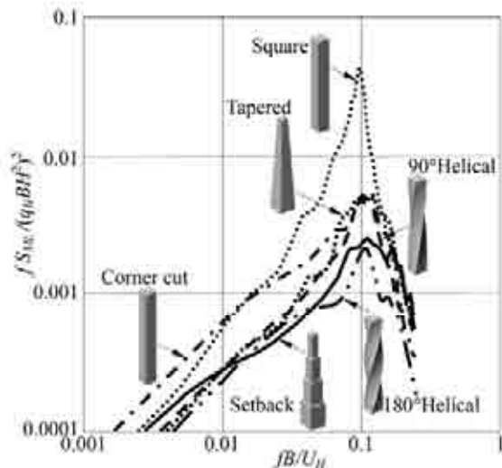
Figure 9: Crosswind overturning moment spectra for tall building models with various configurations (Tanaka et al., 2009)
