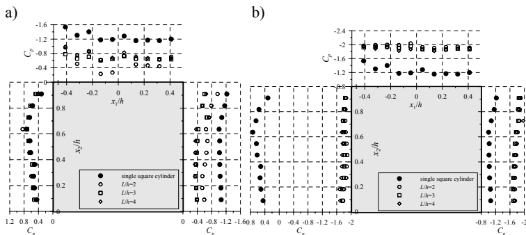
Figure 2: The distribution of the aerodynamic coefficient C_p on the square cylinder at different distance between models for a) the set with square cylinder as the upstream model; b) the set with square cylinder as the downstream model.
