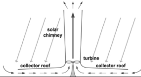
Figure 1: Building components of an SCP: The central solar chimney and the collector roof
