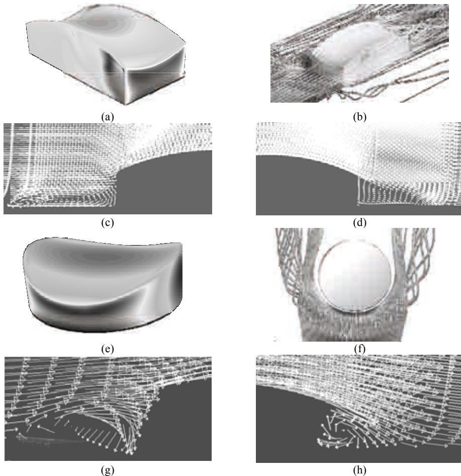
Figure 1: Examples of CFD analyses data: pressure coefficients variation of structures with rectangular (a) an circular (e) plain, streamlines of structures with rectangular (b) an circular (f) and vortex shading in the middle section of building with wind direction angle equal to 0^\circ , rectangular (c,d) and circular (g, h).
