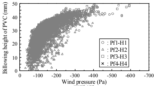
Figure 4: relationship between wind pressure and the billowing height of PVC
