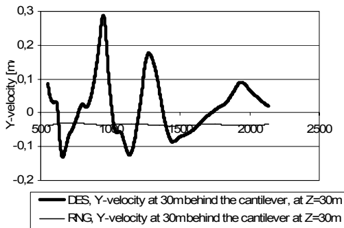
Figure 2: Time history of the Y velocity in the wake, comparison of DES and RNG k- \epsilon model
