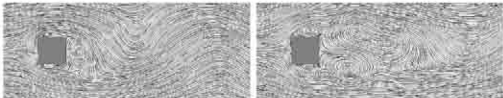
Figure 4: The different flow pattern at f_v = 26\text{Hz} and f_v = 35\text{Hz} .
