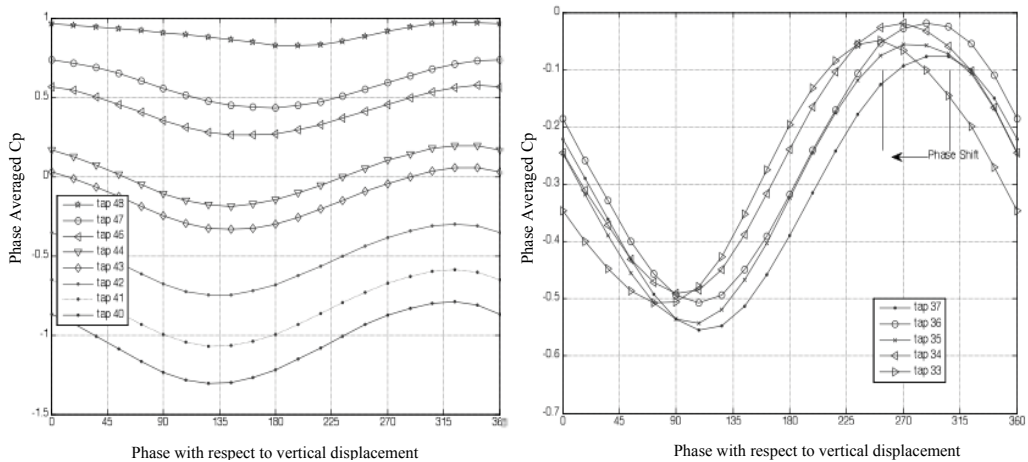
Figure 4: Left, pressure coefficients at maximum amplitude oscillation on the lower flange of the leading edge with approximately constant phase equal to 0^\circ . Right, pressure coefficients at maximum amplitude oscillations along the bottom flange, progressive phase shift up to 90^\circ near the trailing edge corner.
