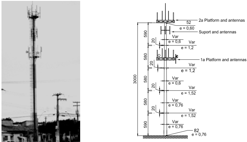
Figure 1: the mobile phone antennas support pole (centimetres).
