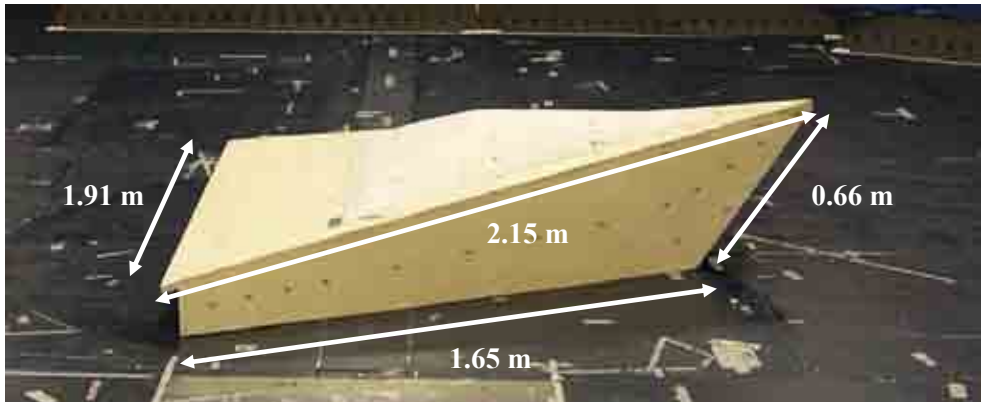
Figure 1: Geometry of the Cultural Centre (CC) building: 1:100 scaled model used for wind tunnel tests. Dimensions in model scale.
