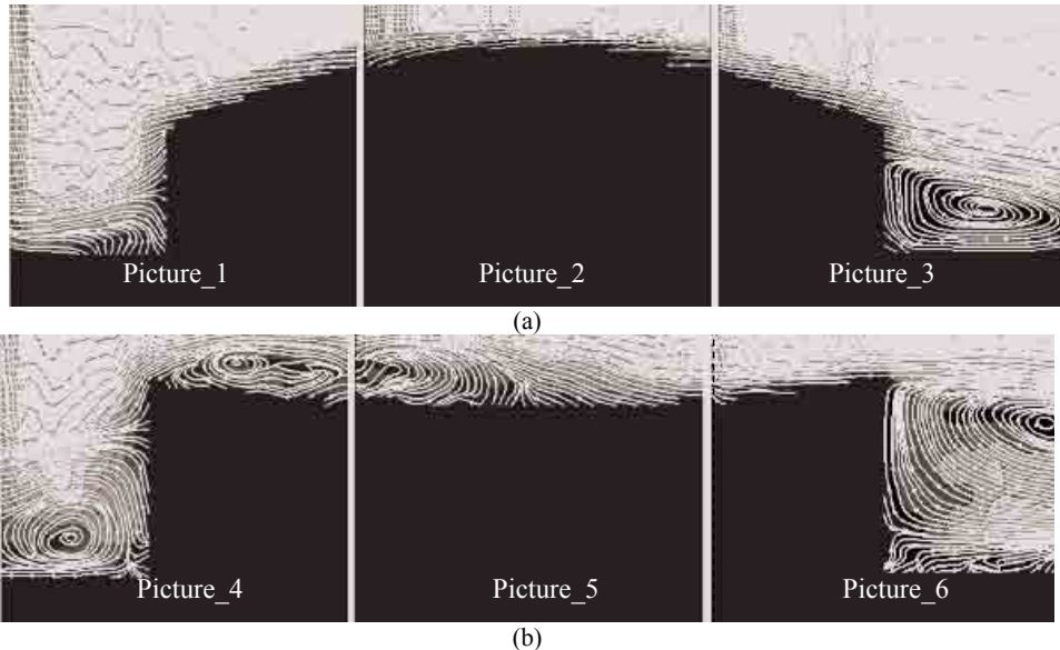
Figure 3: Wind tunnel tests: P.I.V. analysis. 0° (a) and 90° (b) Streamlines – three pictures for each wind direction angle
