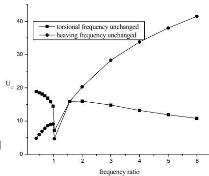
Figure 5: Flutter critical velocities
