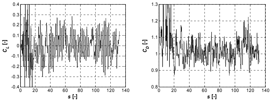
Figure 2: computed lift and drag coefficients ( C_L and C_D are normalized respectively referring to the cylinder chord length B and height H ).
