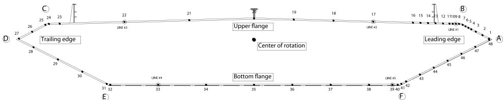
Figure 2: Pressure measurement distribution of a typical ring. Three rings of taps distributed along the span were used. Another set of taps is distributed in five lines along the span (line #1-5). Wind is from right to left.
