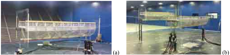
Figure 3: Sectional model in the wind tunnel: (a) test on a single deck (b) Wake effect tests.
