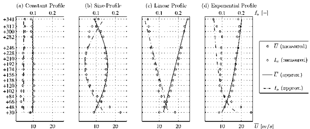
Figure 1: Measured wind profiles at the 344m data acquisition tower Gartow.
