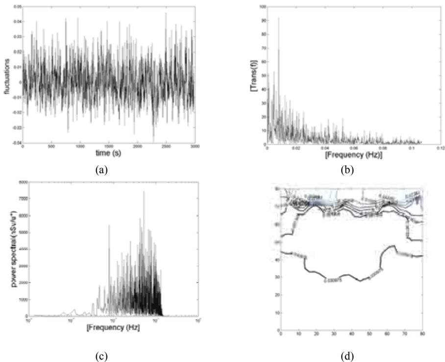
Figure 2: Referring to mode 1, wind direction angle equal to 0^\circ and square plan structure (test p.2) – wind pressure fields calculated with POD. technique: fluctuations of pressure fields with (a), Fourier transform of the frequency (b), Power spectral densities (c), 1st mode shape (d).
