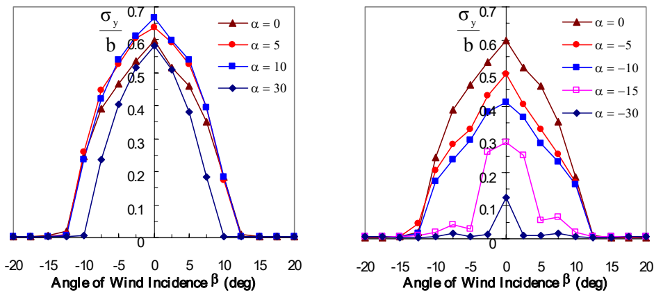
Figure 2: Normalized transverse response of square tower model as a function of angle of incidence of mean wind for various angles of inclination angle
