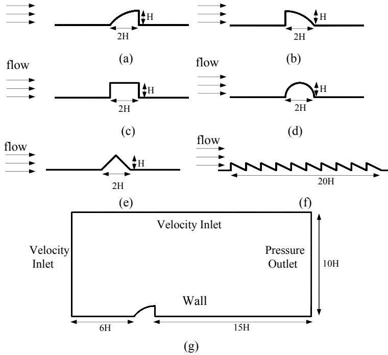
Figure 1: shapes of lower roofs and the computational zone
