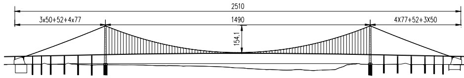
Figure 1: Elevation of Runyang Bridge (Unit: m)
