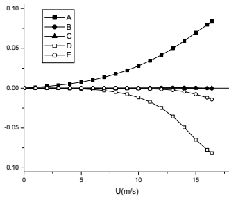
Figure 3: Aerodynamic damping of the systematic torsional motion
