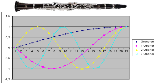
Figure 7: Harmonics of a closed cylindrical pipe (clarinet for instance)
