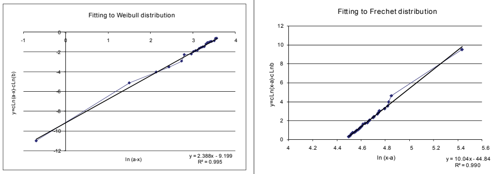
Figure 2.: Fitting of monthly maximum wind speed
