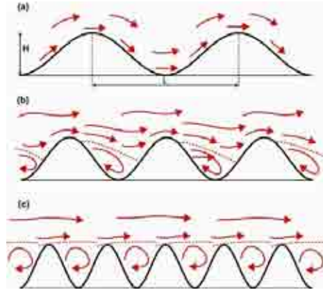
FIG. 1. Schematic diagram of the flow regimes over waves: (a) isolated roughness flow, (b) wake interference flow, (c) and skimming flow.
