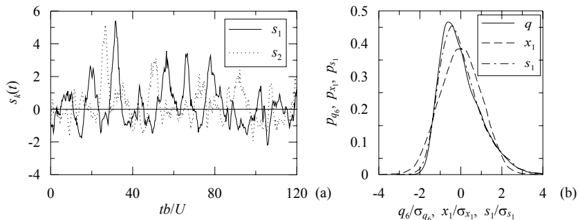
Figure 3: a – First two ICs; b – pdf of local pressure after a windward corner (solid line), pdf first PC (dashed line), pdf first IC (dash-dot line).
