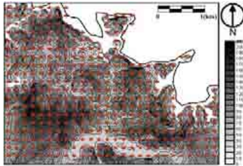
Figure 1: Tuft observation for flow direction of easterly wind over the coastal complex terrain at z/h=1.87
