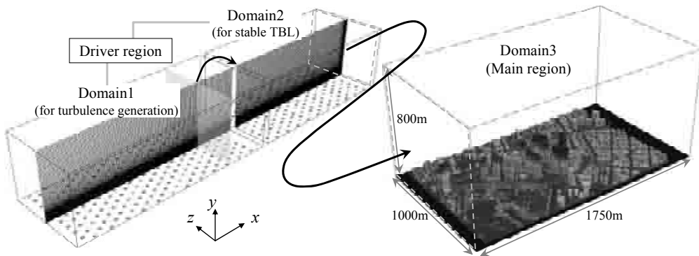
Figure 1: Schematic of the computational model for hybrid method of LES and meso-scale meteorology model concerning urban heat island.
