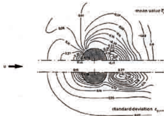
Figure 6: Pressure distribution on ground level for a boundary layer flow around a cylinder, Hölscher (1993)
