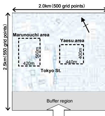
Figure 2: Computational region and spatially averaging area for Marunouchi and Yaesu.
