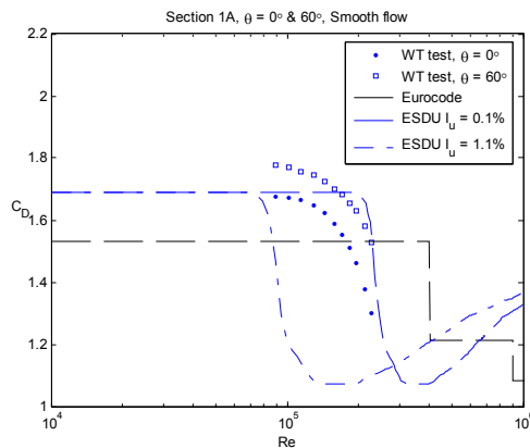
Figure 4: Reynolds-dependant force coefficients in smooth flow for configuration 1A, 0 and 60 degrees angle of attack.
