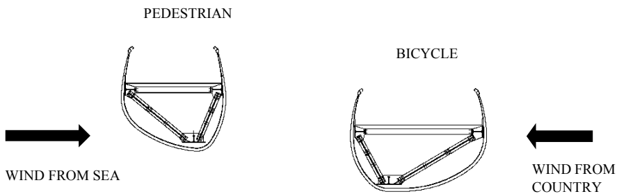
Figure 2: Pedestrian and bicycle deck sections: geometry of the models and wind direction
