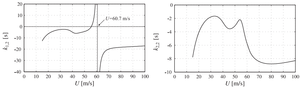
Figure 1: Typical controller gains; for kinematically coupled flaps that are moved in the same direction on the left, for separately driven flaps on the right.
