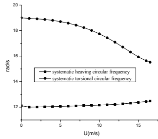
Figure 2: Oscillation frequencies
