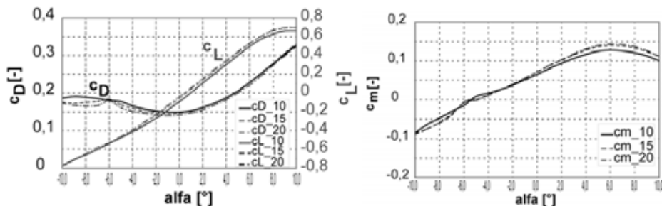
Figure 1: Drag, lift and moment coefficient in function of angle of attack at different wind speeds.
