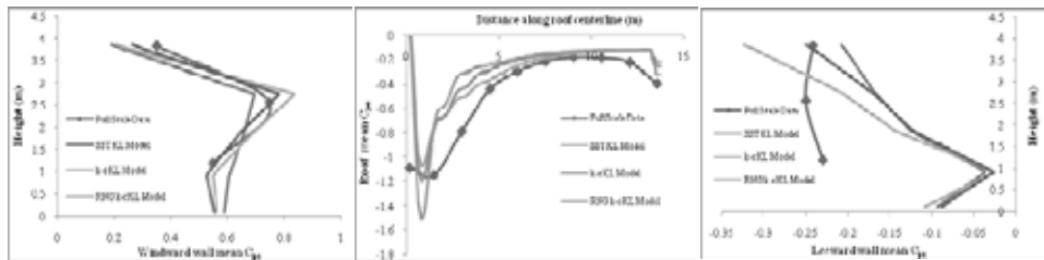
Figure 1: (a) Windward wall (b) Roof and (c) Leeward wall centre-line mean pressure coefficient for mesh setup 1
