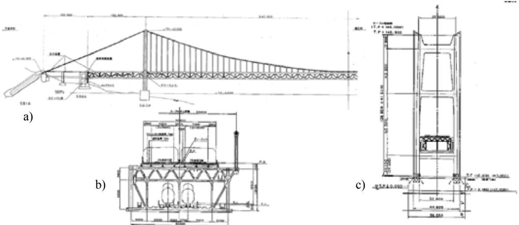
Figure 1: Bridge geometry (Courtesy of Dr. M. Nishitani HBSE-JP): (a) longitudinal profile, (b) deck section, (c) tower.
