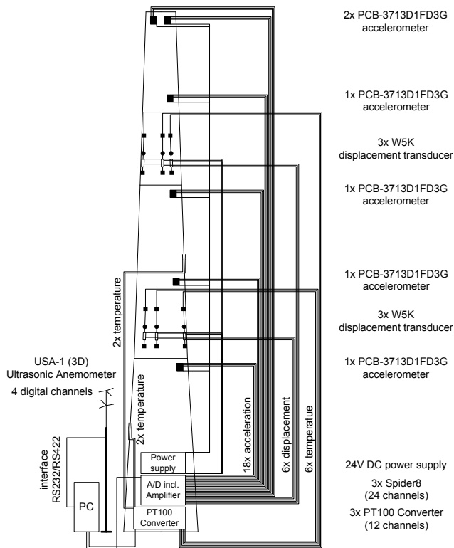
Figure 2: Overview of the planned measurement setup in natural scale
