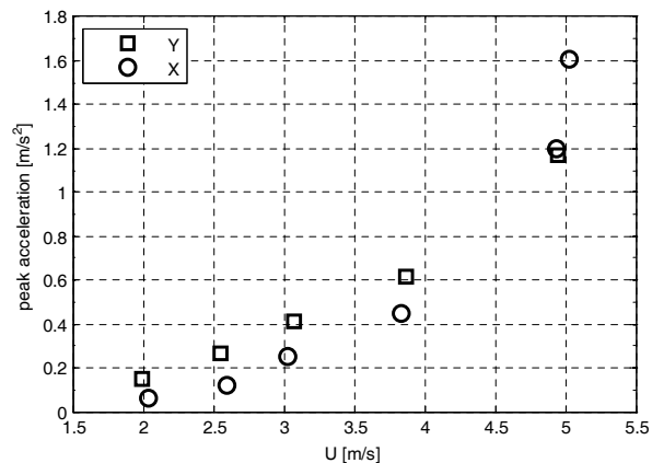
Figure 3: Cross wind peak acceleration in turbulent flow conditions. X: wind perpendicular to the long side of the rectangular section; Y: wind perpendicular to the short side.
