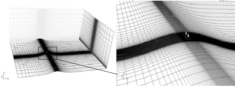
Figure 1: The quasi-2D Gaussian hill with 2 wind turbines on the top.
