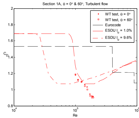
Figure 5: Reynolds-dependant force coefficients in turbulent flow for configuration 1A, 0 and 60 degrees angle of attack.
