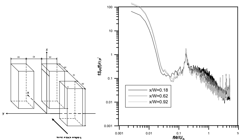
Fig.5 Wind pressure spectrum variations along downstream distance for inner face of building 2 at z/H=0.888
