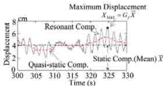
Figure 2: Wind-induced response of a 108m-high tower by GPS (Tamura et al., 2002a)
