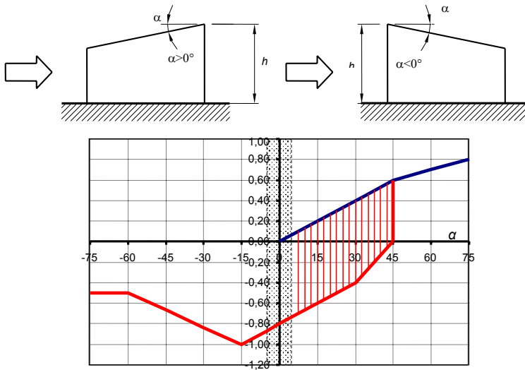
Figure 1: simplified pressure coefficient (constant on the whole surface) for a monopitch roof (Fig. G.7 from CNR-DT 207/2008)
