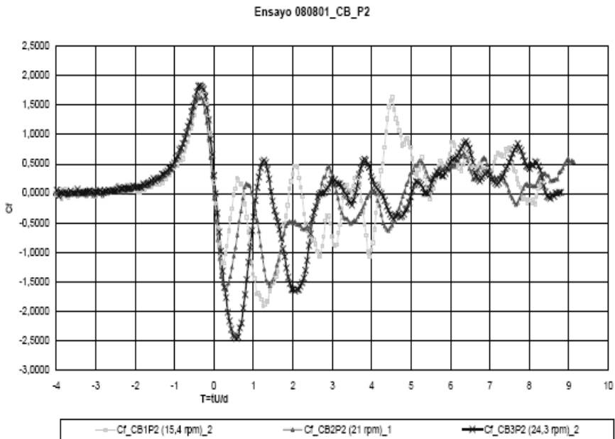
Figure 4: Variation of the transversal force coefficient C_f with the dimensionless time T = tU/d . The legend indicates the angular rotation speed of the centrifuge arm. The plate is placed parallel to the motion direction.
