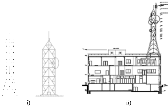
Figure 1: Steel lattice telecommunication masts i) on the ground ii) on buildings
