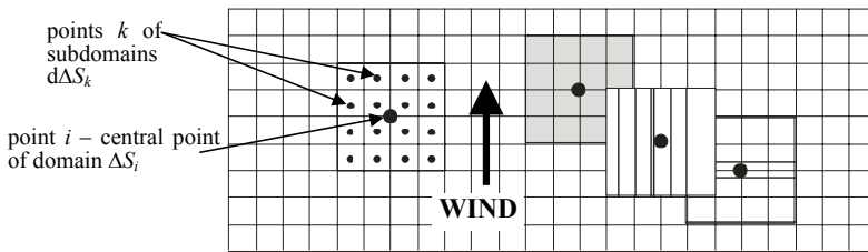
Figure 3: Plane view of domains \Delta S_i in front of the structure corresponding to the roof surface point i .
