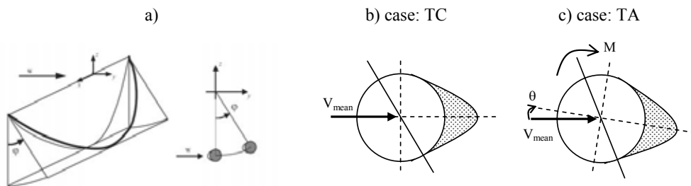
Figure 3. a) Geometric configuration of the cable; b) U-shape aerodynamic cable section for twist-constrained case, TC; c) U-shape aerodynamic cable section for twist-allowed case, TA
