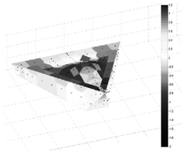
Figure 2: contour plot of the mean pressure coefficient for an incoming wind direction of 0 deg.
