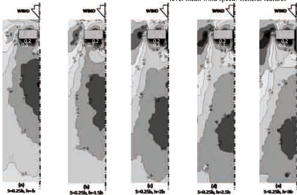
Figure 4: Distribution of the normalized mean wind speed with varying building height and fixed building spacing ( b = 50 m)
