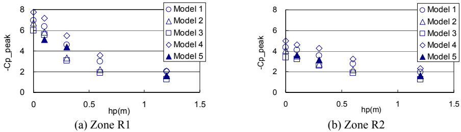
Figure 2: Effect of parapet height h_p and thickness t_p on C_{p\_peak} in Zones R1 and R2.
