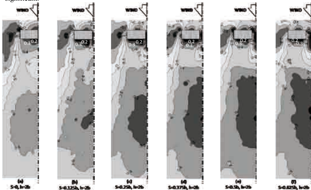
Figure 5: Distribution of the normalized mean wind speed: with varying building spacing and fixed building height ( b = 50 m)
