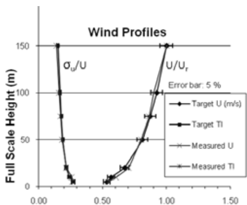
Figure 1: Profiles of mean wind speed and turbulence intensity
