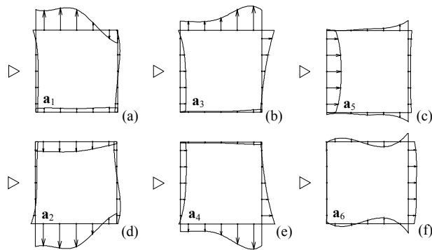
Figure 2: ICA spanning the space defined by the first six PCA modes (Fig. 1).
