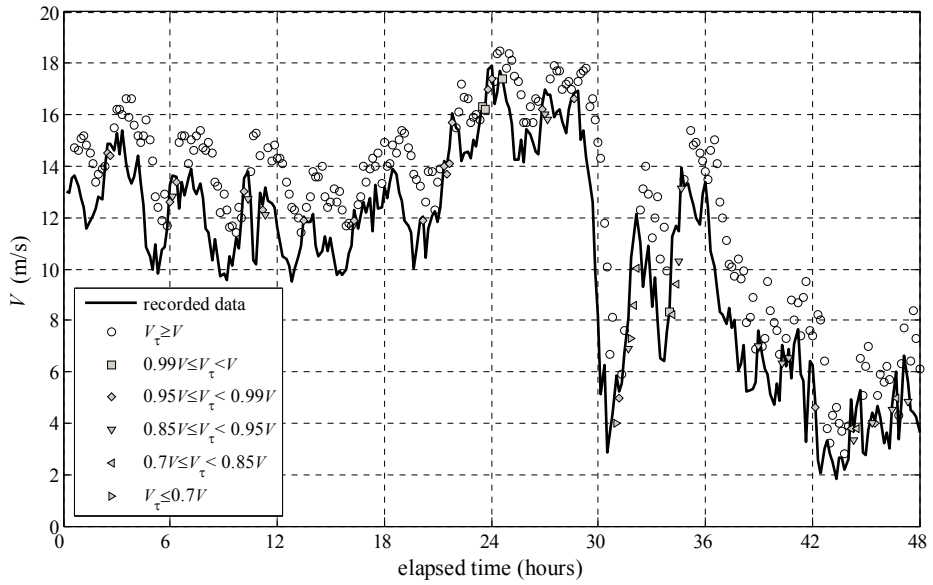
Figure 1. Wind time series (solid line) and 30-minutes-ahead forecast evaluated for non-exceedance probability 95% (symbols).
