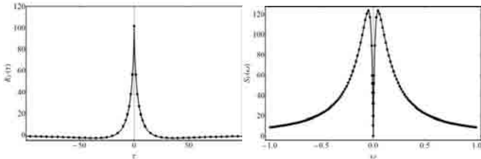
Figure 1: Comparison between the exact (continuous line) and the approximated (dotted line) Davenport's correlation function (left panel) and PSD (right panel).
