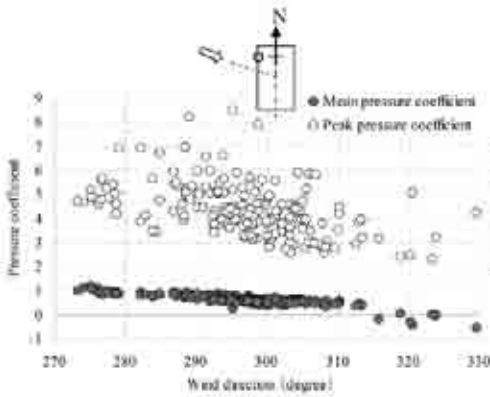
Fig.5 Mean and peak pressure coefficients on the west side outer skin normalized by the 10 minute mean velocity pressure.
