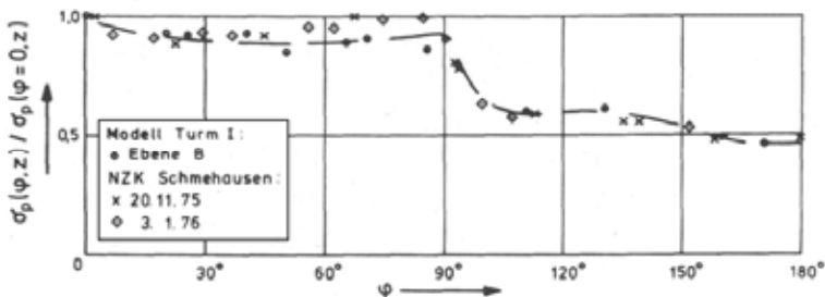
Figure 3: Rms. Pressure distribution at level z
