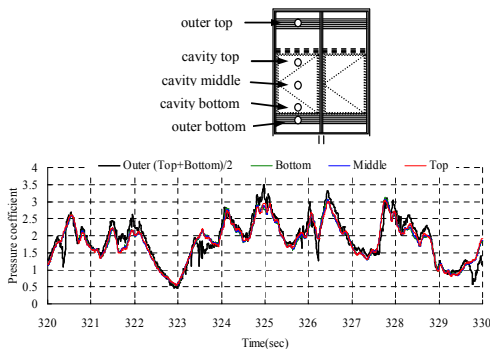
Fig.7 Pressure fluctuations on the cavity side of the inner skin.
