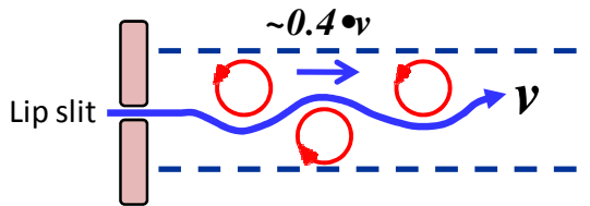
Figure 14: Basic mechanism of whistling
