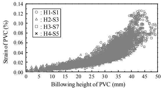
Figure 5: relationship between billowing height of PVC and strain of PVC
