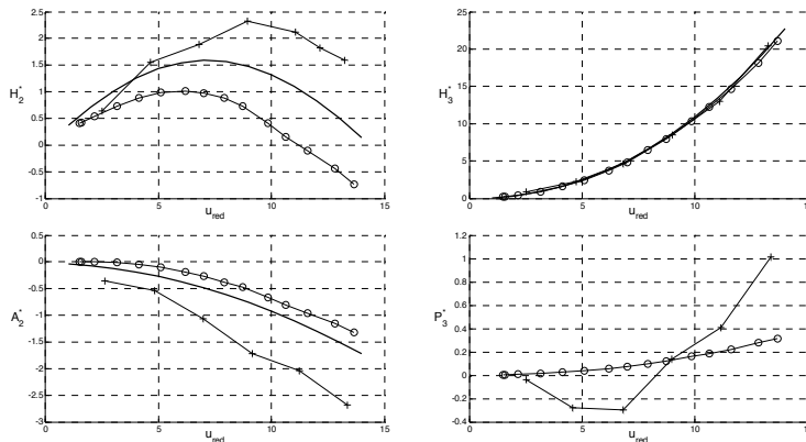
Figure 4: Examples of aerodynamic derivatives for a NACA 0020 airfoil (“-“ Theodorsen’s analytical solution, “+” free vibration measurement of Chowdhury and Sarkar (2003), “o” forced vibration measurement results)
