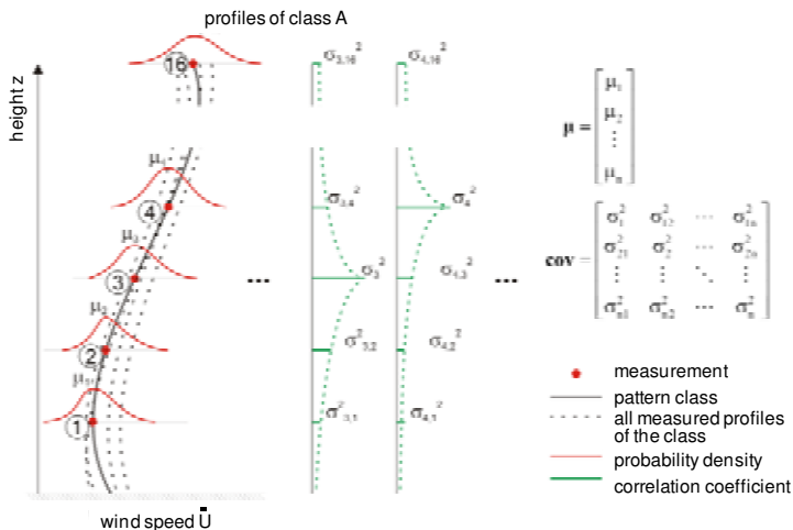
Figure 24: Statistical classification of wind profiles
