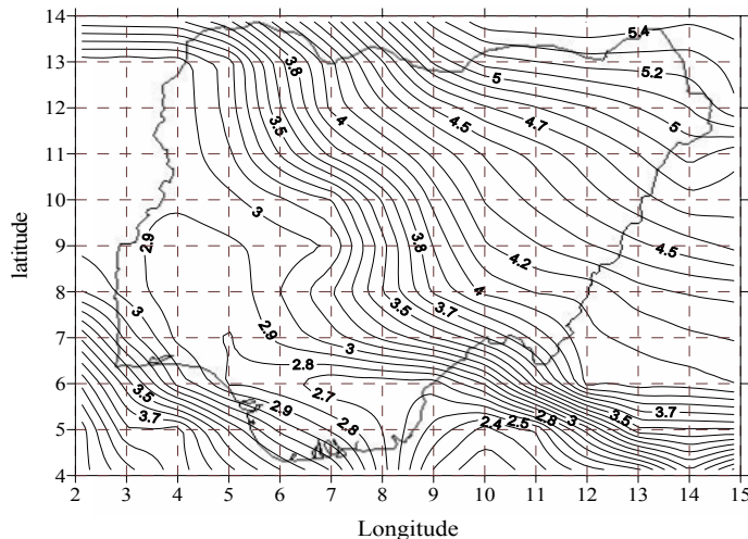
Figure 1: Isovents of Average Daily Wind Speed at 50 m of Height above Earth Surface across Nigeria.
