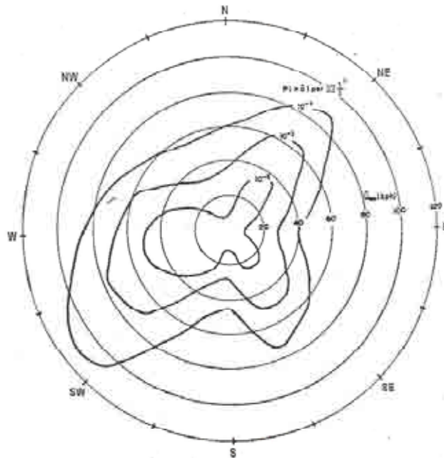
Figure 3: probability distributions of hourly mean wind speed at 300 m over Montreal for daylight hours during the winter (derived from 10 year record of wind data obtained at a height of 10 m at Trudeau Airport).
