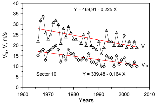
Figure 1. Many year change of the annual maxima of wind speed V (gusts) and V_m (10 min mean) at the meteorological station in Wroclaw, sector 10 (central direction of the sector 10 is 270^0 - western).
