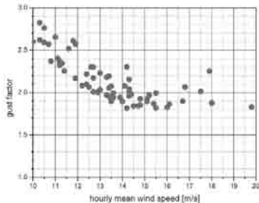
Figure 1: Observed gust factors, Düsseldorf airport 1952 - 2007
