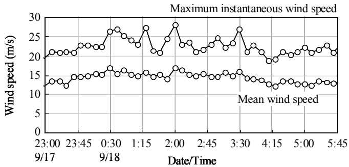
Figure 3: the mean wind speed and the maximum instantaneous wind speed for ten minutes in Typhoon No.12 in Japan
