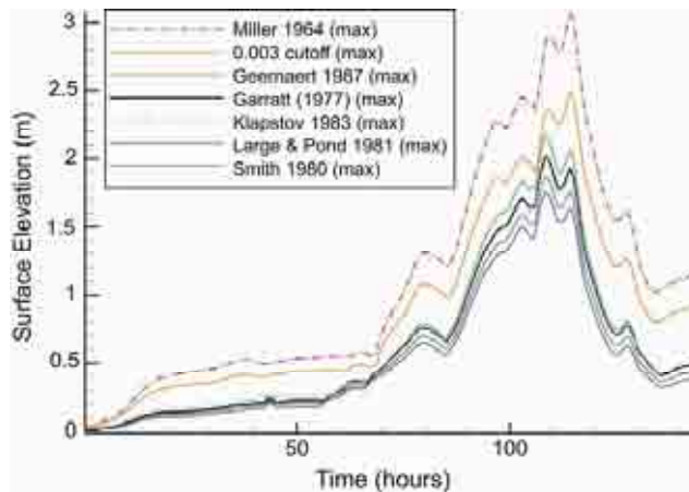
FIG. 10. Peak storm surge generated (ADCIRC) for Hurricane Georges (1998) using the maximum value of the drag coefficient formulations. Adapted from Weaver (2004).
