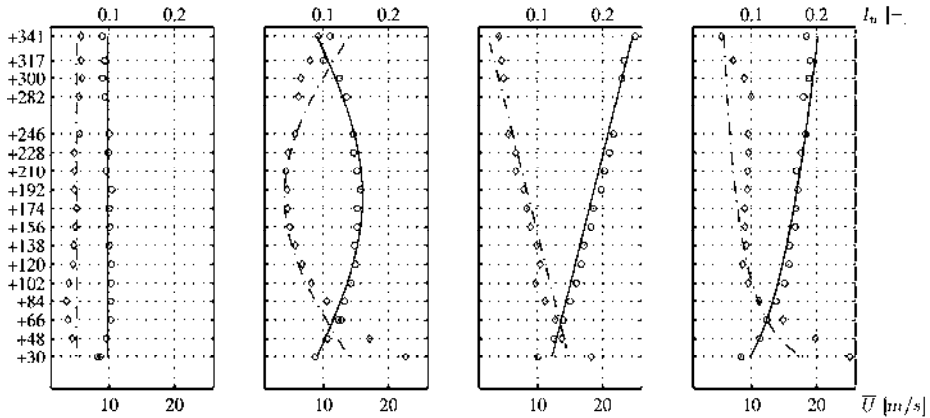
Figure 23: Typical wind profile classes at lower wind speed (o: \bar{u} \diamond : I_0 )
