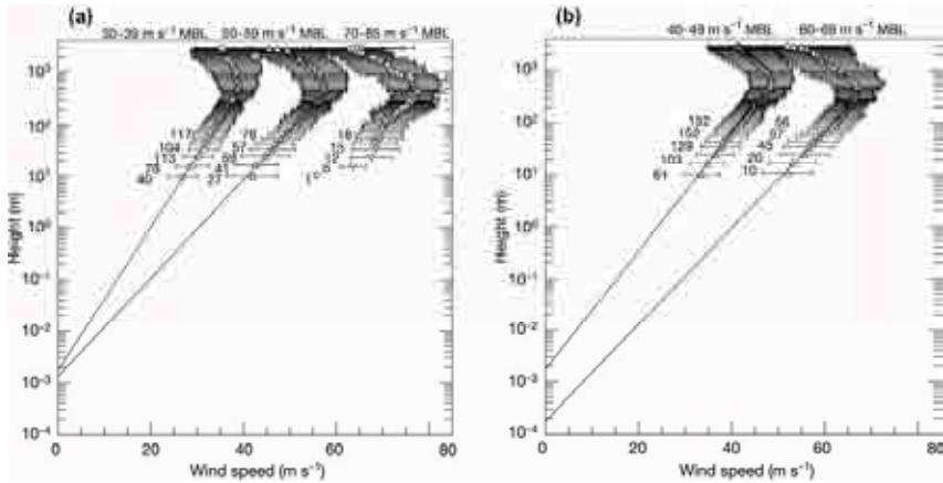
FIG. 3. Mean wind profiles by MBL group: (a) 30–39 m/s (72 profiles), 50–59 m/s (55 profiles) and 70–85 m/s (38 profiles) and (b) 40–49 m/s (105 profiles) and 60–69 m/s (61 profiles) MBL groups. Symbols and horizontal bars represent mean and standard deviation for each vertical bin. Numbers adjacent to each level represent the number of samples within each of the lowest five height bins. From Powell et al. (2003).
