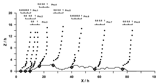
Figure 2: Mean wind velocity profiles for different downwind stations of sources for Easterly wind over the coastal complex terrain
