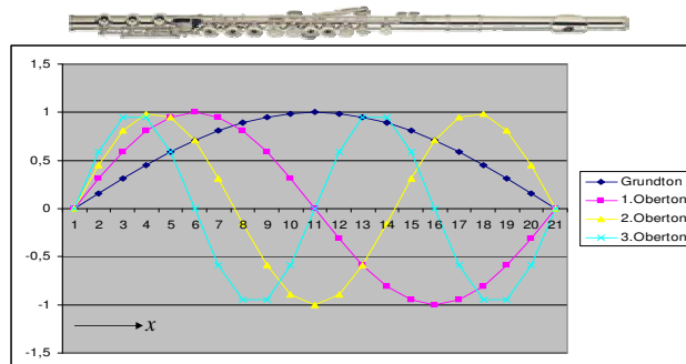
Figure 6: Harmonics of a flute
