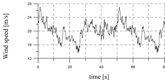
Figure 4: Exemplary wind speed (x component) simulated with WAWS method.
