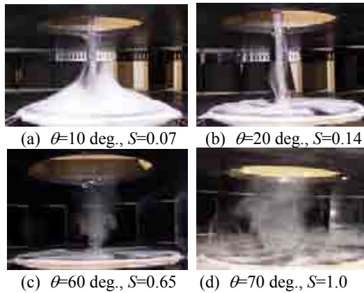
Figure 1: Flow visualization of tornado-like flow for various swirl ratios (without roughness block)
