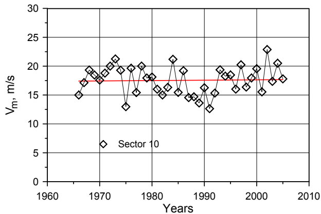
Figure 3. Annual maxima of the 10 min mean wind speed corrected for open terrain
