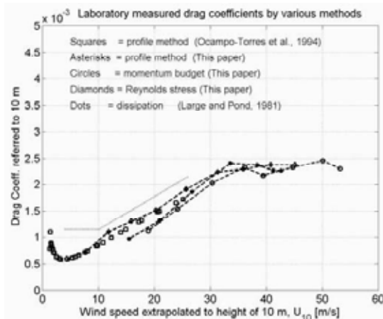
FIG. 6. Laboratory measurements of the neutral stability drag coefficient by profile, Reynolds Stress and momentum budget methods. The drag coefficient refers to the wind speed measured at the standard anemometer height of 10 m. The frequently cited drag coefficient formula derived from field measurements by Large and Pond (1981) is also shown. From Donelan et al. (2004).
