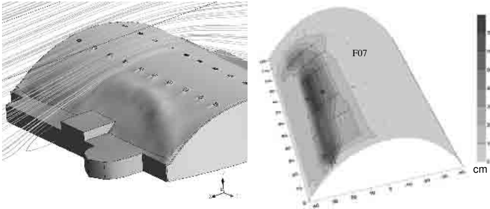
Figure 3: Snow depth measured at 27.02.07 (right). 3D simulation snow surface and wind stream lines (left).
