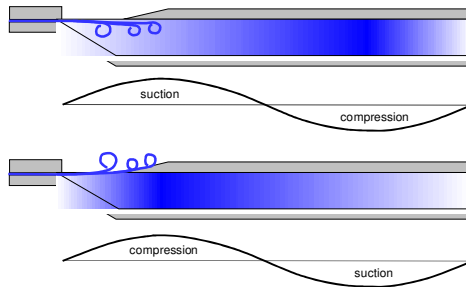
Figure 16: Schematic feedback mechanism for the synchronization of the air reed
