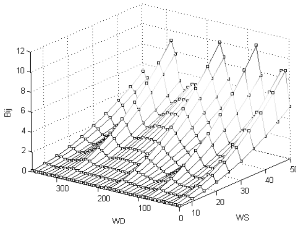
Figure 2. Response surface representing a member's demand-to-capacity index b_{ij} as a function of wind speed WS and direction WD (Spence, 2009).
