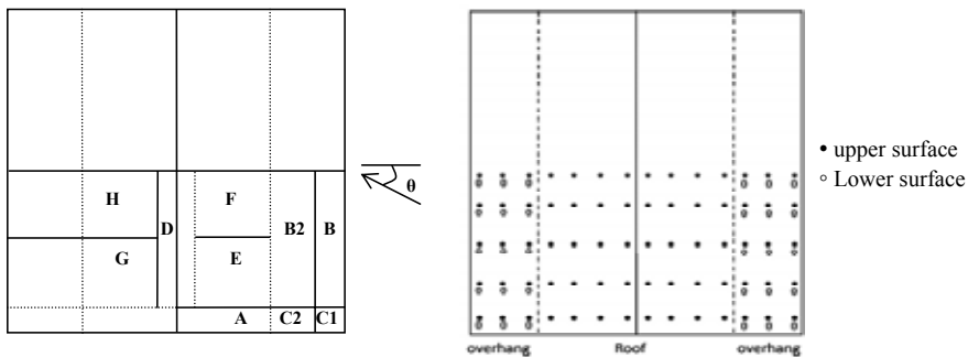
Figure 2. Different zones on roof and overhang of building and location of pressure taps
