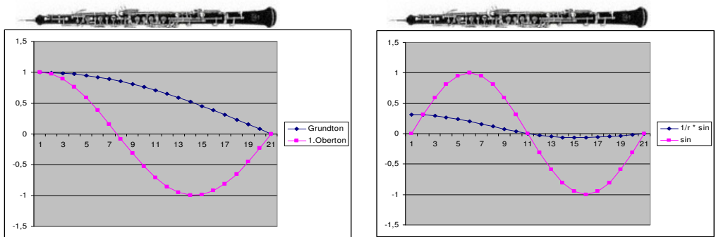
Figure 10: Influence of a conical bore on the action of even harmonics
