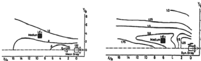
Figure 3: IF for mean and fluctuating forces parallel to wind.
