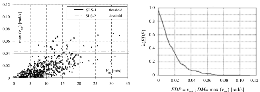
Figure 2. Structural response statistics: population (left), probability curves (right).
