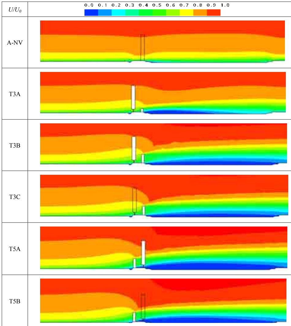
Figure 2: Predicted isolines of the wind velocity for several configurations of the shelterbelt.
