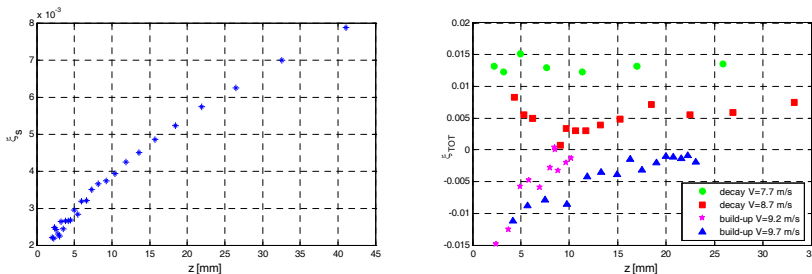
Figure 6: (a) structural non dimensional damping as a function of the oscillation amplitude (b) total damping (structural and aerodynamic) measured during wind free motion tests as a function of the oscillation amplitude.
