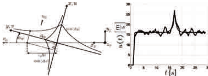
Figure 3: Sketch of exponential gust (left) and gust scenario with superposed turbulence (right)
