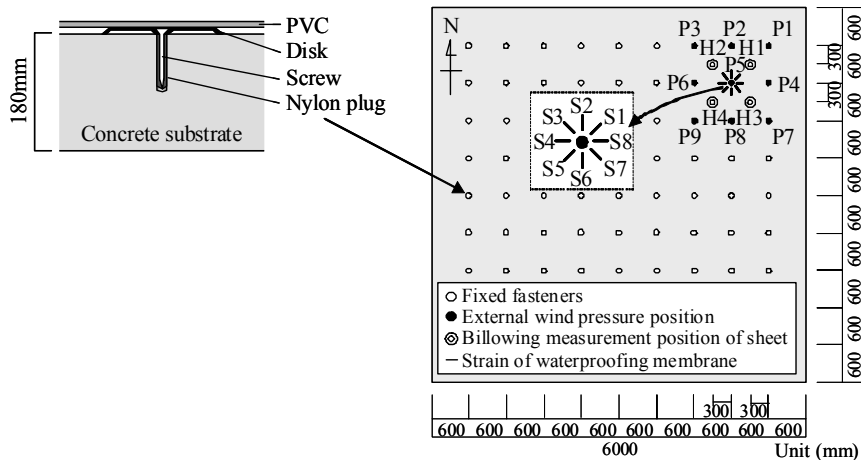
Figure 2: waterproofing membrane system and outline of the measurement
