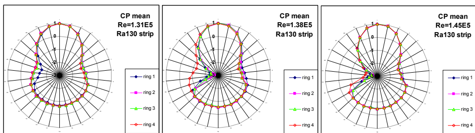
Figure 5: Mean pressure coefficients evolution with Re from the four pressure rings, denoted 1 to 4 from ground to ceiling, Ra130 stripped surface model.
