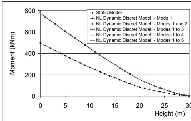
Figure 3: wind action.
