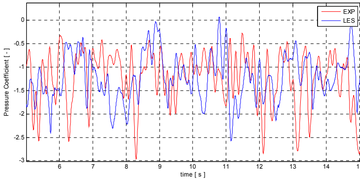
Figure 4: Wind tunnel vs CFD results comparison: time histories of the instantaneous values of the pressure coefficient.
