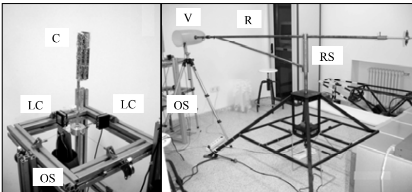
Figure 2: Sketch of the experimental set-up. V: vehicle. R: rotating arm. RS: rotating arm support. C: cylinder. LC: Load cell. OS: Object support structure.
