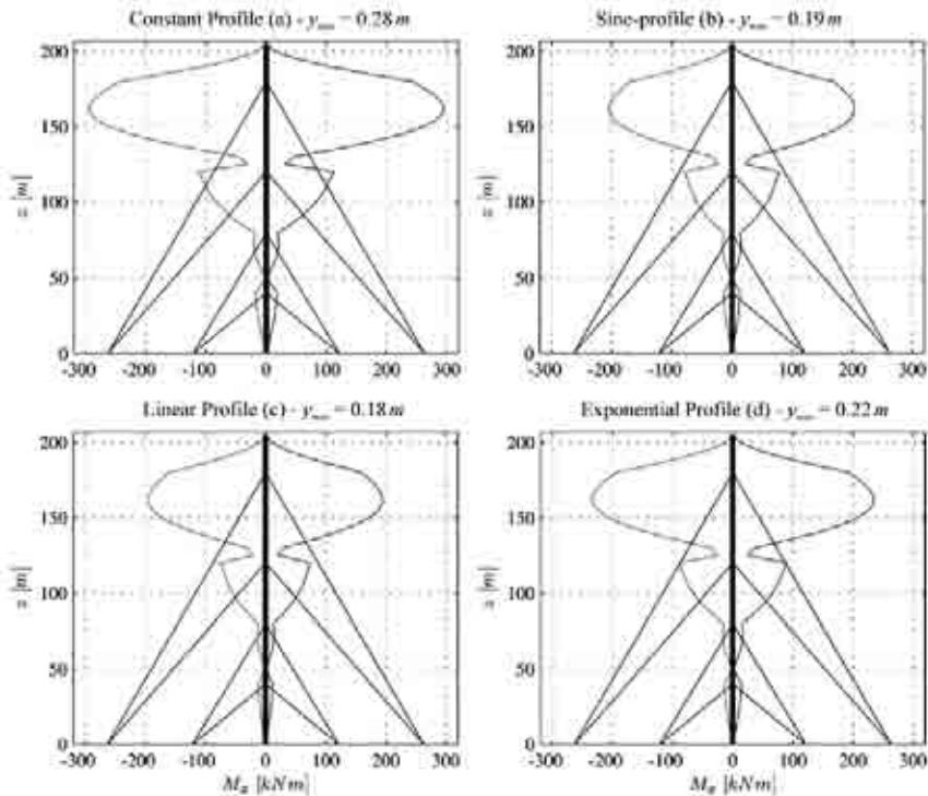
Figure 5: Lateral bending moments for different wind profiles.
