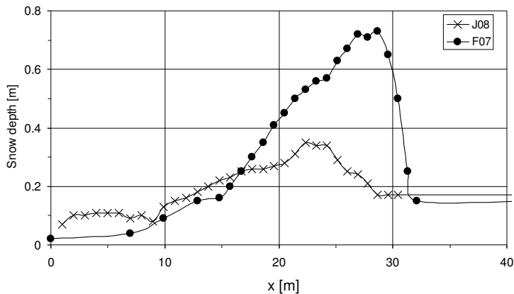
Figure 2: Snow depth on the roof of Vallhall arena measured at 27.02.07 (F07) and at 07.01.08 (J08).
