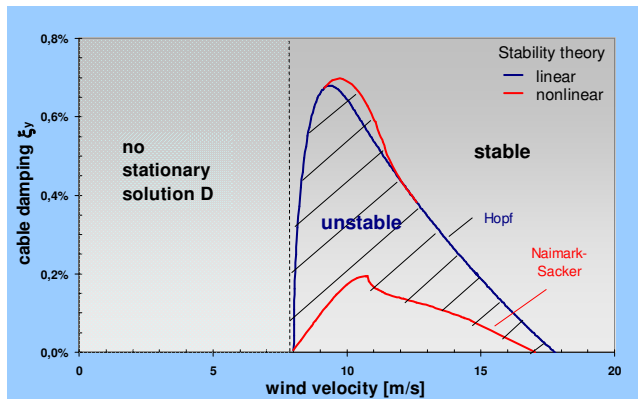
Figure 30: Stability chart of rain-wind induced vibrations of a cable
