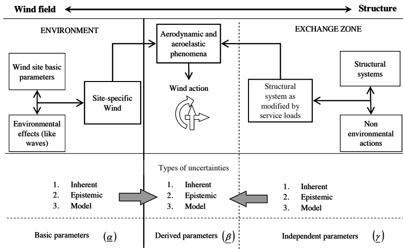
Figure 1: sources of uncertainty in wind engineering.
