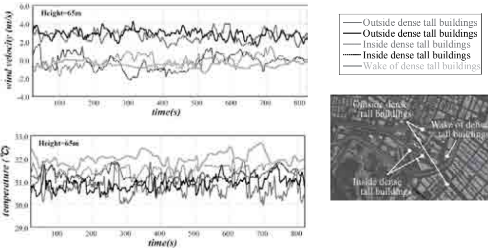
Figure 4: Time histories of the wind velocity and temperature in various local points at 65m height
