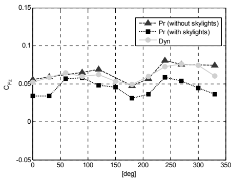
Figure 5: Mean lift force coefficient: force vs. pressure measurements.
