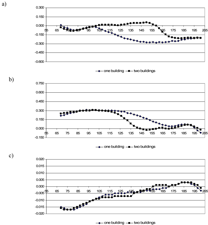
Figure 3: Functions of aerodynamic coefficients – a) drag coefficient C_x , b) lift coefficients C_y , c) moment coefficient C_m for the cross-section of the building on the level 134 m above ground (40 th floor) in the two considered situations (one building and two buildings) obtained from wind tunnel tests.
