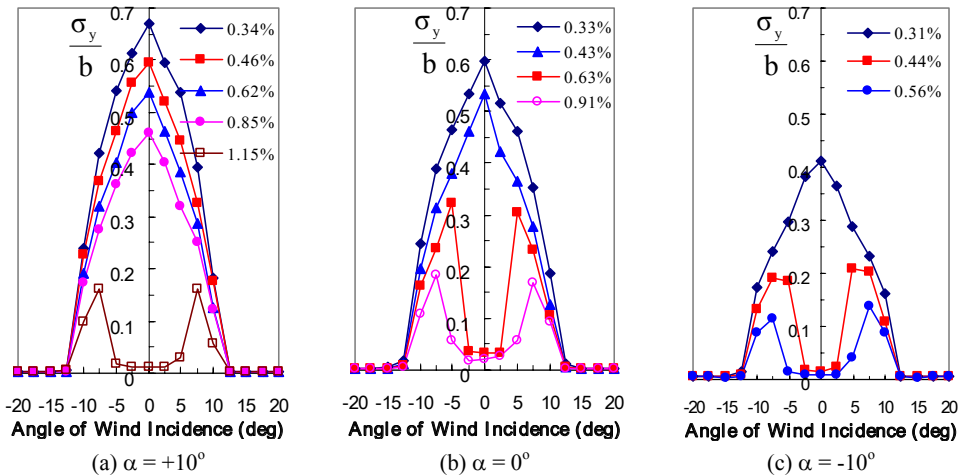
Figure 3: Normalized transverse response of the square tower model as a function of angle of incidence of mean wind for various levels of structural damping
