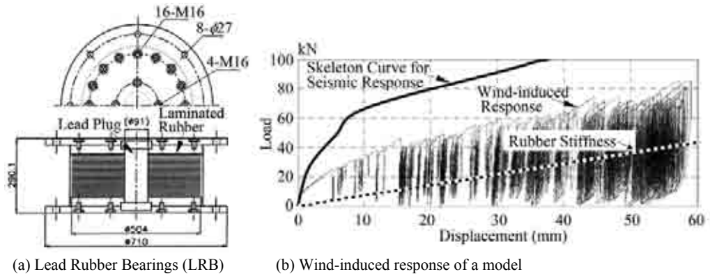
Figure 8: Base-isolation device (LRB) and experimental result of wind-induced response of a building model with LRB base-isolation system (Takenaka et al., 2004)
