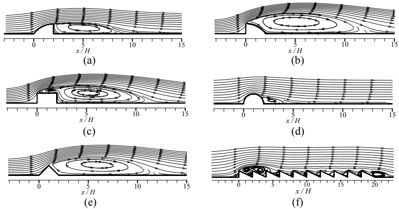
Figure 3: Streamlines distribution around the roofs of lower greenhouses
