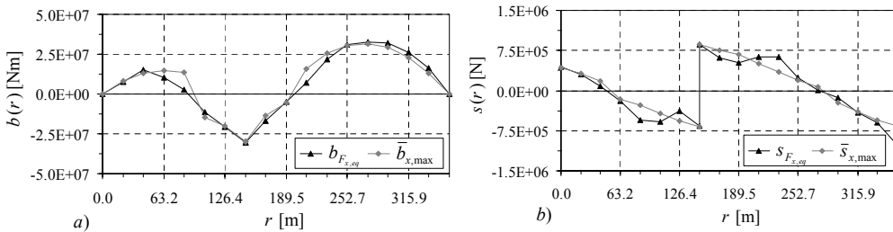
Figure 3: Diagrams of \bar{e}_{x,max}(r) and of the load effects e_{Fx,eq} generated by the ESF F_{x,eq}(z) obtained using spectral eigenfunctions and imposing 14 conditions: a) e=b ; b) e=s .
