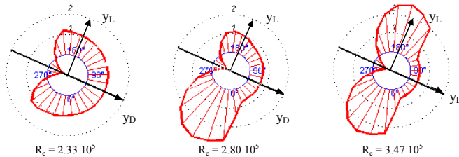
Figure 2: Evolution of the mean pressure distribution around the cylinder with Reynolds number for yaw angle \beta = -17.5^\circ (upper ring)
