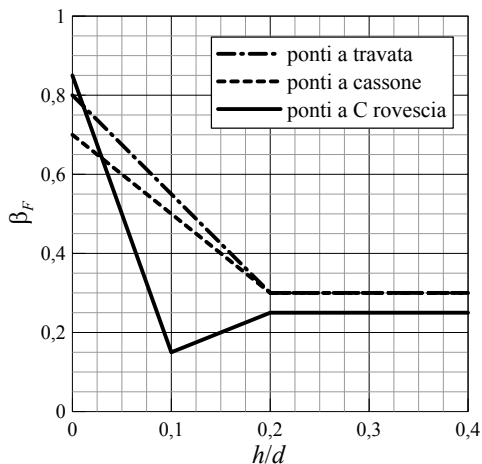
Figure 4: aerodynamic efficiency coefficient \beta_F as a function of the height/width deck ratio for evaluating the flutter susceptibility of bridge decks (Fig. P.6 from CNR-DT 207/2008)
