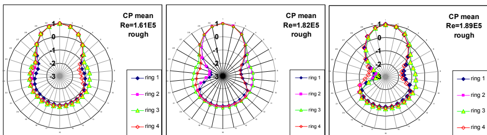
Figure 4: Mean pressure coefficients evolution with Re from the four pressure rings, denoted 1 to 4 from ground to ceiling, rough surface model.
