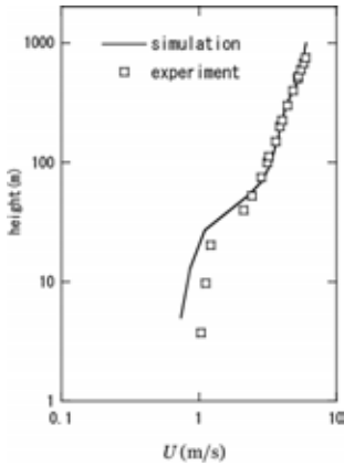
Figure 3: Mean velocity profiles at inlet.
