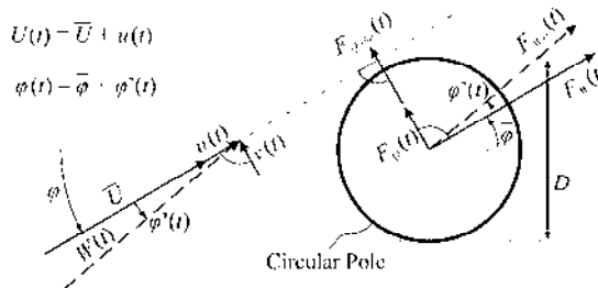
Figure 2: Wind velocities and forces on a circular cross section.
