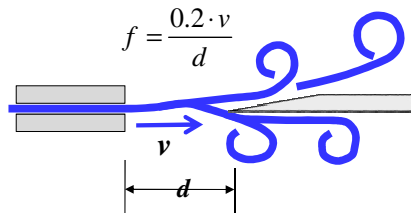
Figure 15: Edge tone excitation
