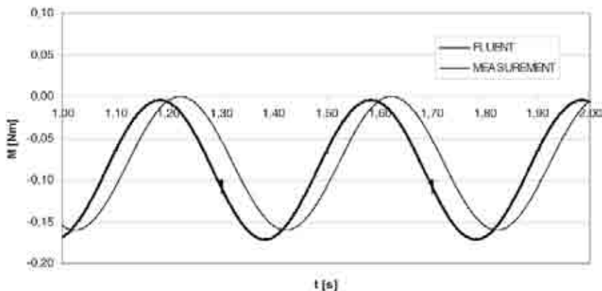
Figure 3: torsion moments as a function of time.
