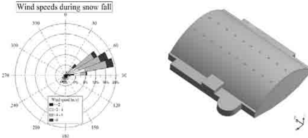
Figure 1: Wind direction and velocity during cold precipitation at the building site (left); 3D digital model of the building (right).
