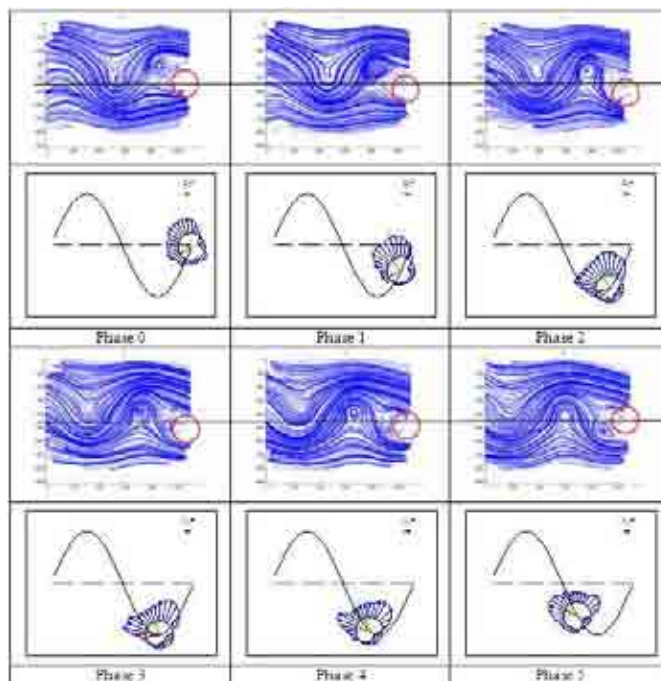
Figure 3: Comparison between flow maps and pressure distribution for different cylinder position at V/V_s=1.3
