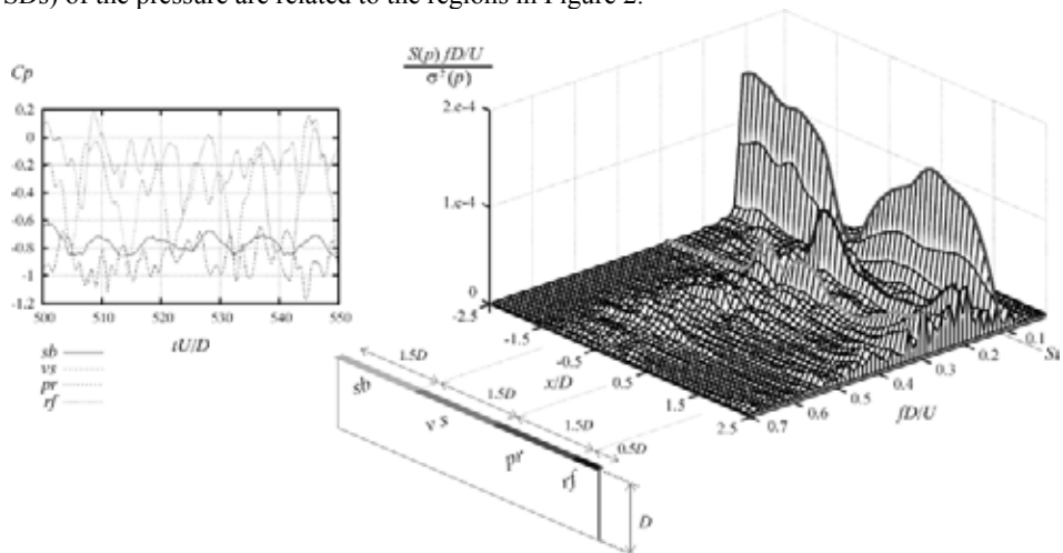
Figure 2: Pressure coefficient time histories and PSD along the upper side surface
