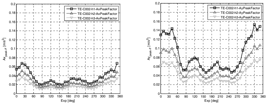
Figure 2: Point at the top-floor: peak-accelerations (3.5xRMS) in x and y direction in function of the exposure angle. Damping h=1\% , 2\% , 4\% .
