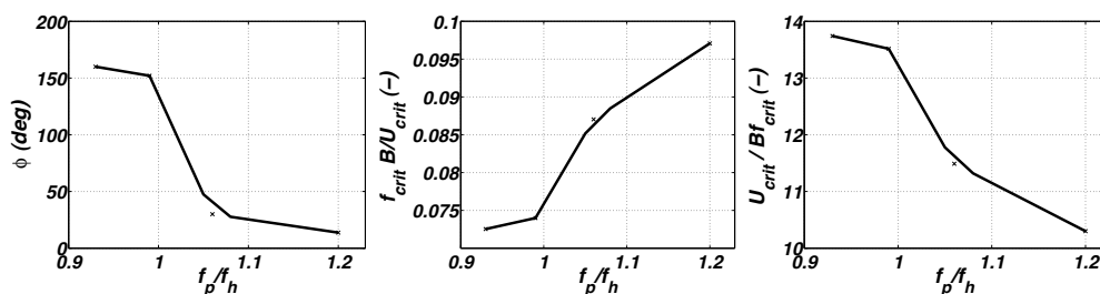
Figure 2: Influence of the eigen-frequency ratio on the the response of the rectangular deck: phase lag between the pitch and heave movements-left, flutter frequency-middle, critical velocity-right.
