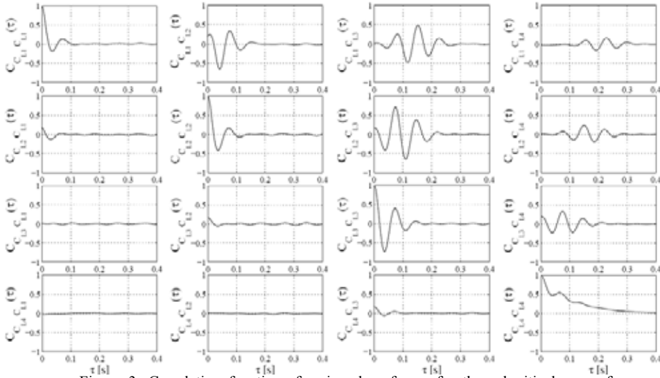
Figure 3: Correlation functions for ring drag forces for the subcritical case of U=12\text{m/sec} . Propagation is evidently one-sided. Model setup, \phi=60^\circ and \alpha=0^\circ .
