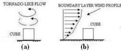
Figure 1: (a) Cube in tornado-like flow (b) Cube in boundary layer flow
