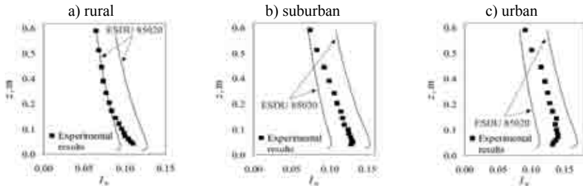
Figure 3: Turbulence intensity profiles I_u compared with ESDU 85020 (1985) data; a) rural, b) suburban, and c) urban ABL simulation
