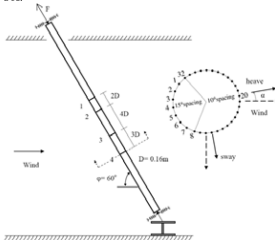
Figure 1: Illustration of the pressure tap arrangement. Cross-sectional arrangement refers to the case of zero rotation of the spring supports i.e. principal axes along and transverse to the flow.
