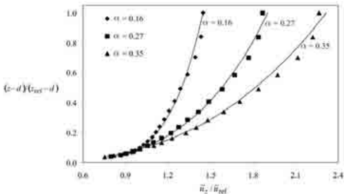
Figure 2: Mean velocity profiles in x -direction compared with the power law (linear presentation)
