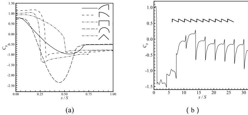
Figure 5: Variation of pressure coefficient C_p with curve length of periodically placed roofs of lower greenhouses
