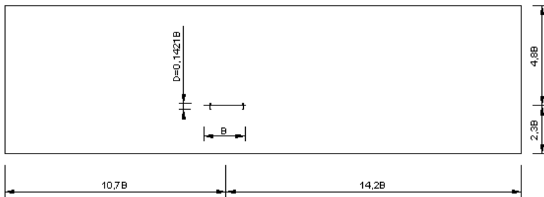
Figure 2: Computational domain.
