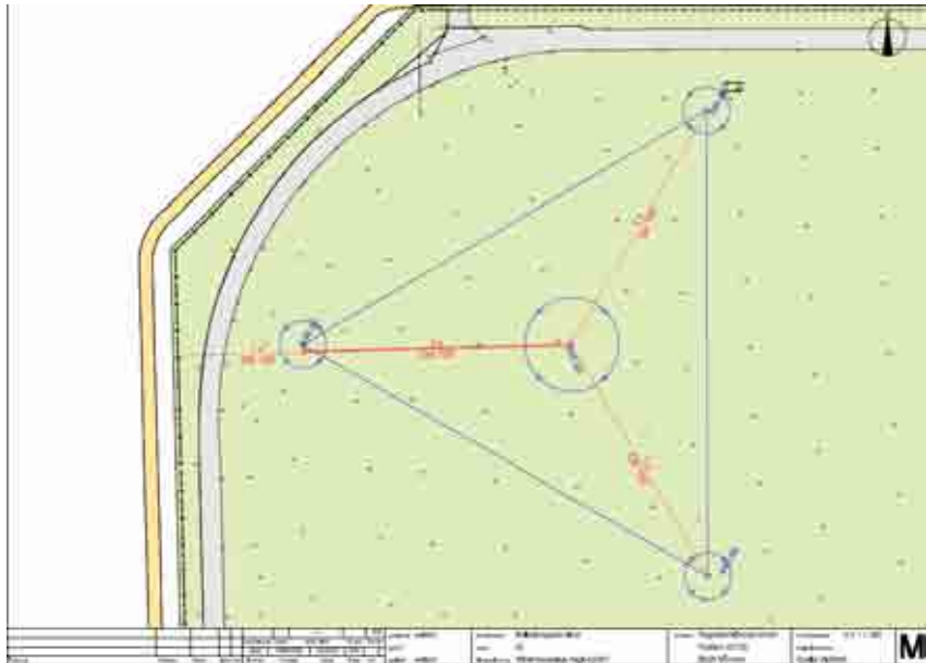
Figure 2: Basic layout of the storm trap at the Airport Munich
