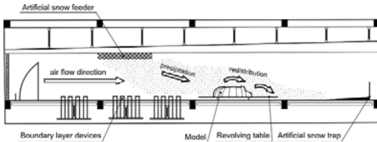
Figure 3: Arrangement of the experiment in the wind tunnel working section.
