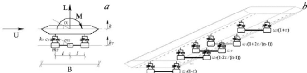
Figure 1: two-DOFs aeroelastic deck model equipped with two DOFs STMD device (a); sketch of the MTMD system.
