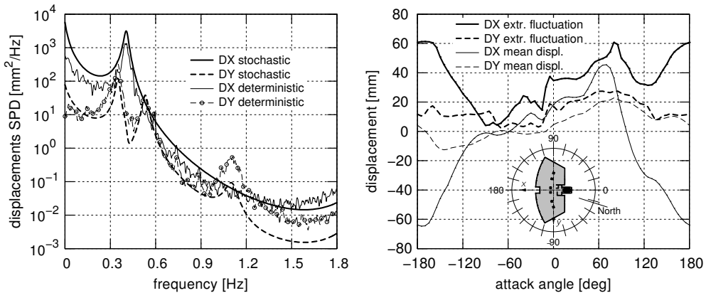
Figure 1: (left) – displacement SPDs for the central node of the highest floor, comparison between stochastic and deterministic analyses, angle of attack is 180^\circ ; (right) – extreme values of displacements fluctuations from the stochastic analysis, compared to static values.
