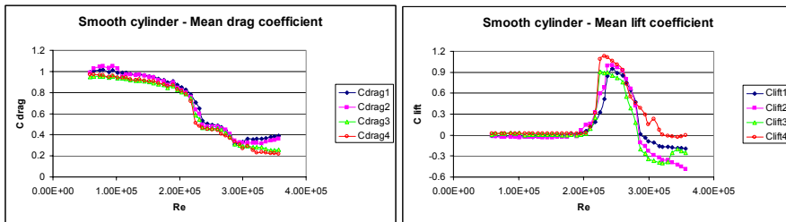
Figure 3: Mean drag and lift coefficients calculated by integration from the four pressure rings, denoted 1 to 4 from ground to ceiling, for a smooth surface cylinder.
