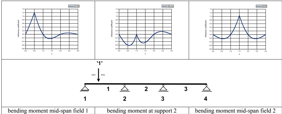
Figure 3: Influence lines for selected bending moments
