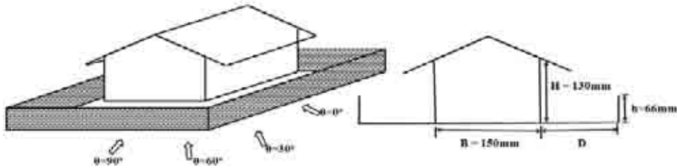
Figure 1. Building model with interfering boundary-wall
