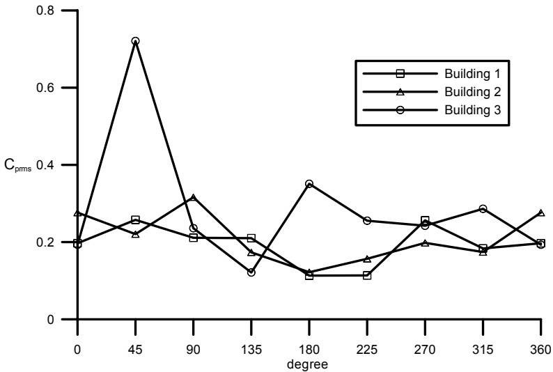
Fig.3 Root mean square of wind pressure coefficient as functions of wind attack angle for front faces of three buildings at location z/H=0.888 , and y/W=0.38 and -0.38
