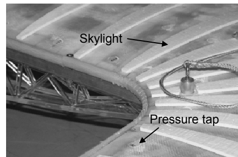
Figure 4: Model roof: skylights and pressure taps.
