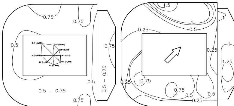
Figure 4: Exemplary results (roof shape factor \mu ); left: basic load scheme, right: a sample load scheme for wind induced redistribution.
