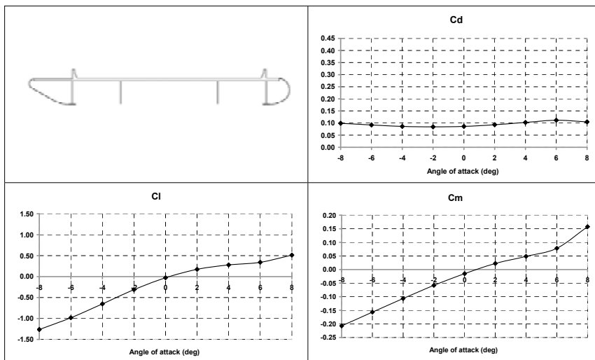
Figure 4: Aerodynamic coefficients for the modified design proposal.
