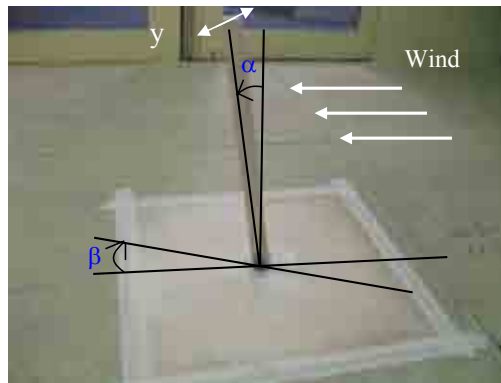
Figure 1: Orientation of square tower model
