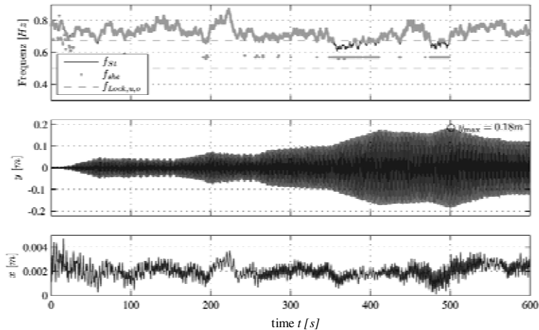
Figure 26: Time history of excitation frequency and corresponded deflection of the mast top
