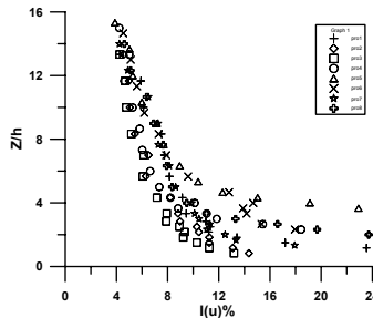
Figure 3: Longitudinal turbulence intensity profiles at various downwind stations of sources for easterly wind over the coastal complex terrain
