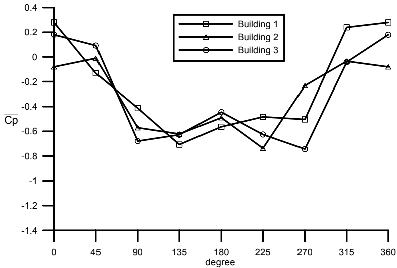
Fig.2 Mean wind pressure coefficient as functions of wind attack angle for front faces of three buildings at location z/H=0.888 , and y/W=0.38 and -0.38
