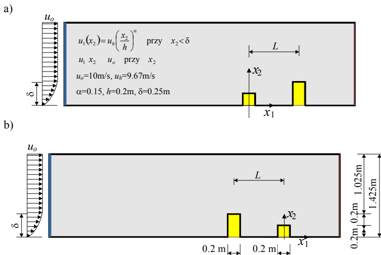
Figure 1: The arrangements of models: a) the set with square cylinder as the upstream model; b) the set with square cylinder as the downstream model.
