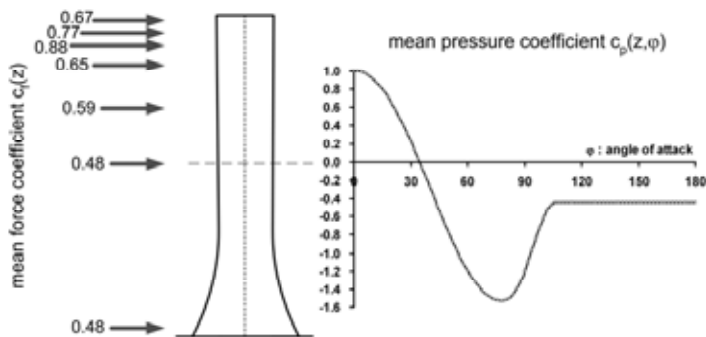
Figure 2: Distribution of wind force coefficients over the tower height
