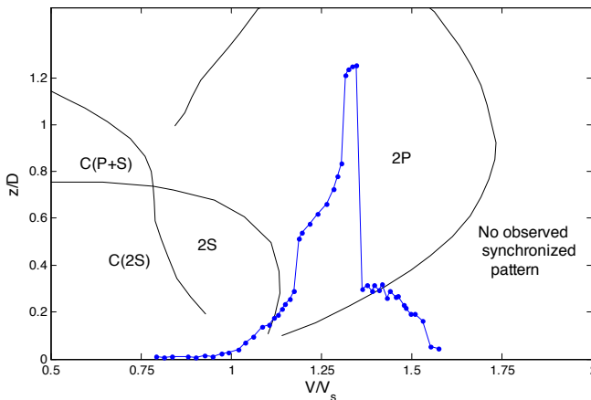
Figure 2: Williamson & Roshko (1988) map of wake modes with superimposed steady state oscillating response
