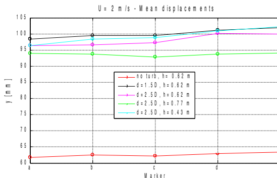
Fig.4 : Mean y displacement of the markers
