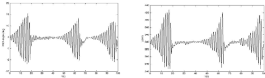
Fig.2: (a) pitch angle – (b) horizontal displacement
