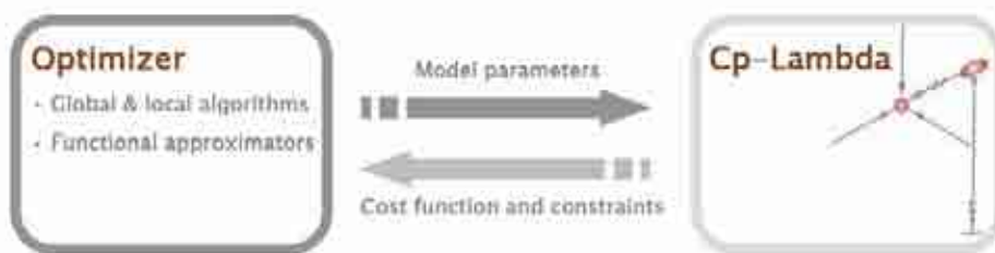
Figure 1: Coupling between optimizer and aero-servo-elastic solver for multi-disciplinary design optimization.
