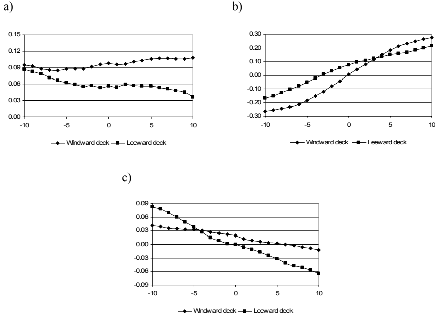
Figure 4: Functions of aerodynamic coefficients – a) drag coefficient C_x , b) lift coefficients C_y , c) momentum coefficient C_m for the windward and leeward decks of the Cracow cable-stayed bridge obtained from wind tunnel tests.
