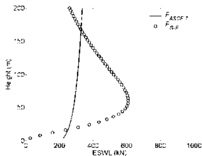
Figure 1: F_{ASCE7} and F_{G-F} in an example building
