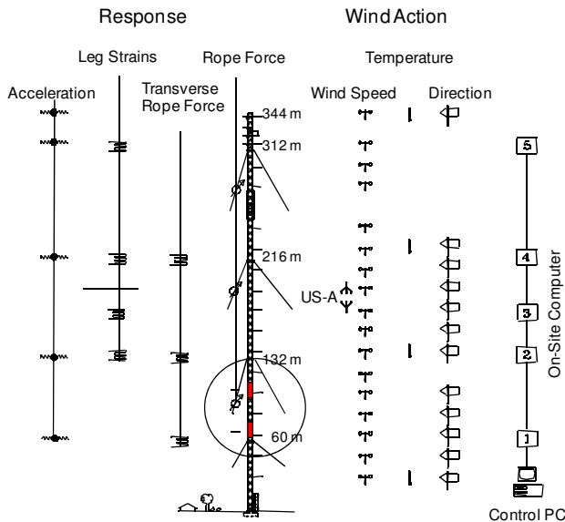
Figure 32: Wind and mast measurement equipment in Gartow
