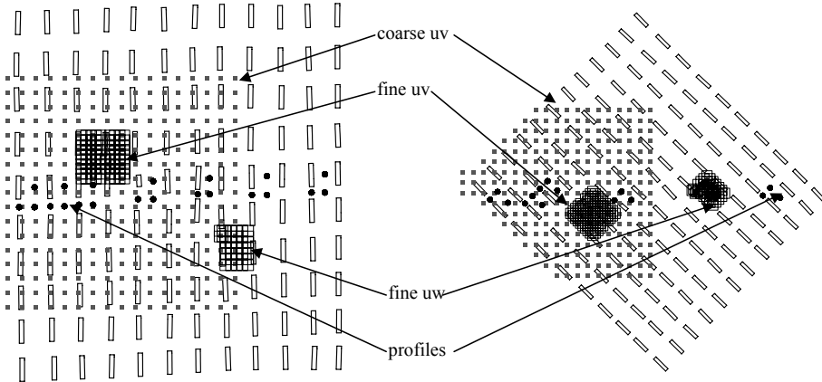
Figure 1: Obstacle arrangement and velocity measurement zones for the MUST wind tunnel case. Left: approach flow direction 0^\circ . Right: approach flow direction -45^\circ . Wind always from left.
