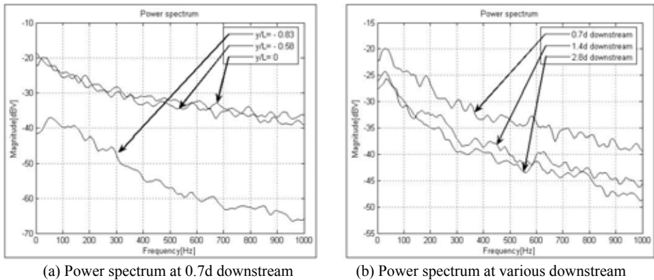
Figure 2: Power spectrum for both 0.7d downstream and various downstream
