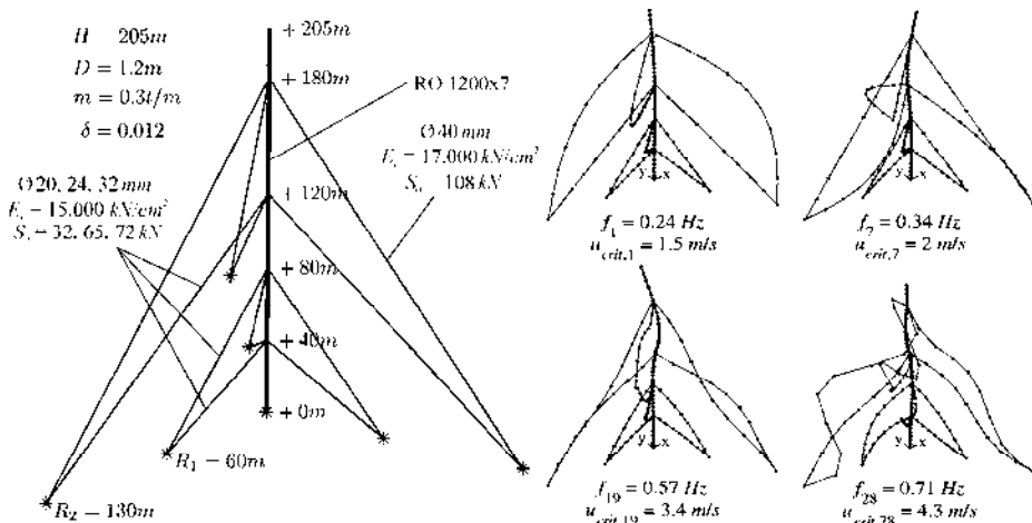
Figure 4: Structural properties and chosen mode shapes with the corresponding u_{crit} .
