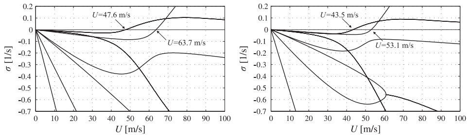
Figure 2: Real part \sigma of the system eigenvalues against the mean horizontal wind speed U . For a flap-free system on the left, for a system extended with unmoved flaps on the right.
