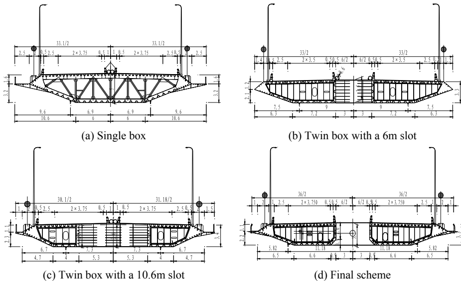
Figure 5: Proposed box girder sections for Xihoumen Bridge (Unit: m)
