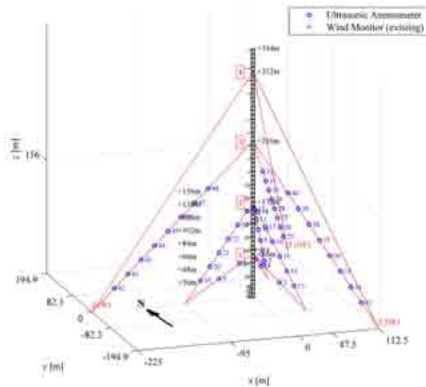
Figure 32: Additional sensor boxes placed on the cables
