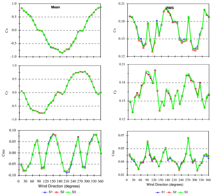
Figure 4: Effect of tap resolution – Typical balcony scenario shown in Figure 1.
