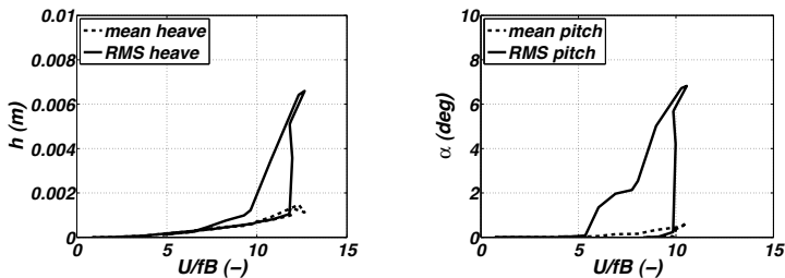
Figure 3: Heave (left) and pitch (right) amplitude rectangular deck characteristics as the functions of the wind velocity. The dashed line and solid line denotes the mean and root mean square value, respectively.
