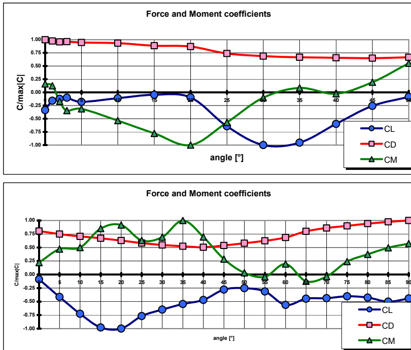
Figure 3: obtained results for two different tested configurations: angle of incidence = 0^\circ (above), angle of incidence = 45^\circ (below); coefficients are plotted as ratios with respect to their maximum absolute values
