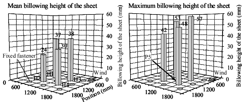
Figure 2: the result of billowing height of waterproofing membrane (Maximum wind speed :16.8m/s)
