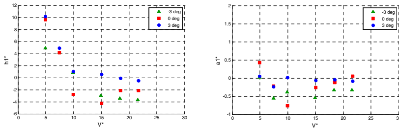
Figure 6: Flutter derivatives as a function of V^* measured on pedestrian deck, wind blowing from the sea, for different mean angle of attack : (a) h1^* (b) a1^* .
