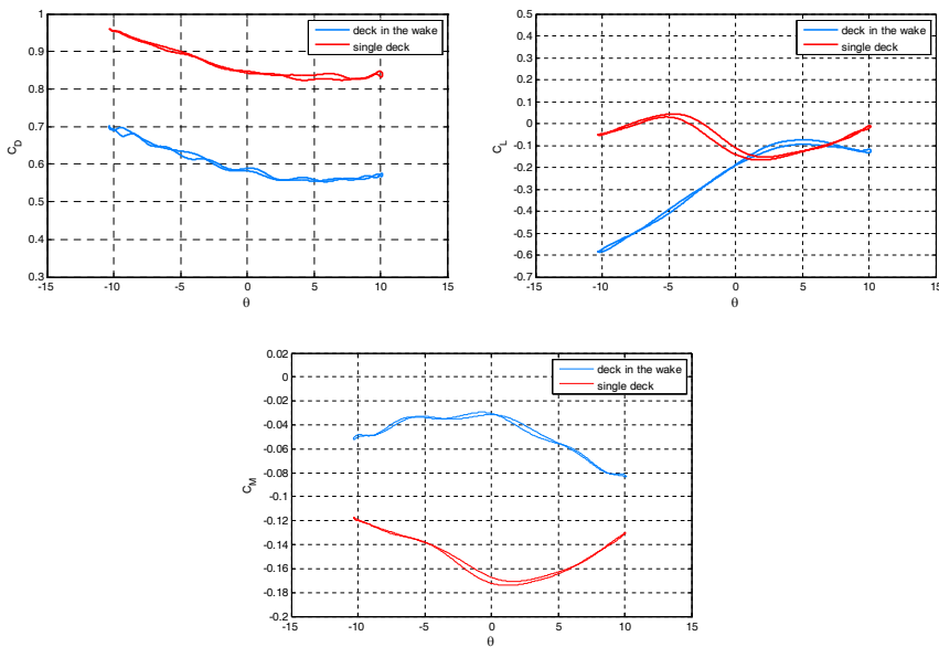
Figure 5: C_D , C_L , C_M measured on pedestrian deck, wind blowing from the land side, with and without wake effects.
