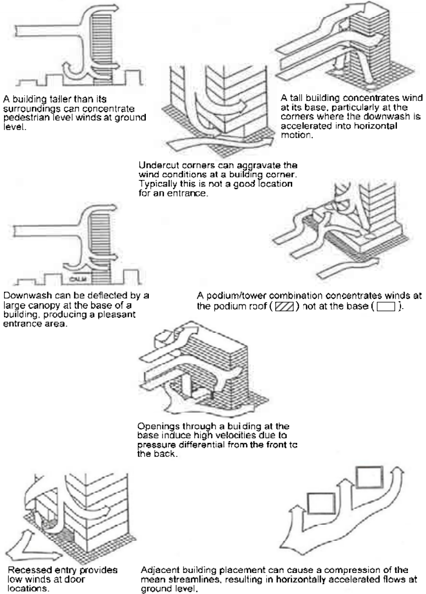
Figure 2: design features to change and/or ameliorate pedestrian wind conditions, after Cochran (2004).
