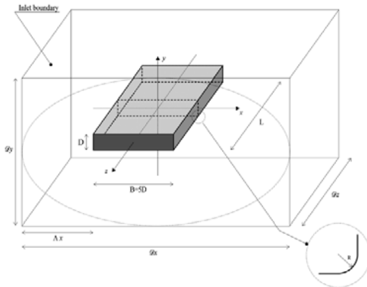
Figure 2: sketch of the computational domain
