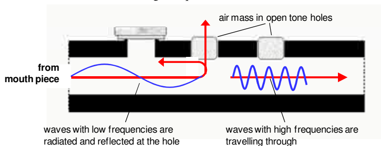
Figure 22: Behavior of tone holes as low pass filters
