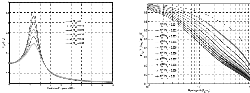
Figure 3: (a) Gain of internal pressure fluctuations over windward external pressure for a range of porosity ratios (b) Influence of background leakage and non-dimensional area-volume ratio on fluctuating internal pressure
