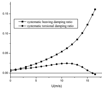
Figure 1: Damping ratios
