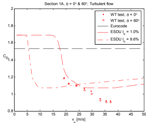
Figure 6: Velocity-dependant force coefficients in turbulent flow for configuration 1A, 0 and 60 degrees angle of attack.
