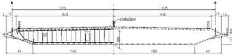
Figure 2: Deck cross-section of Runyang Bridge (Unit: m)
