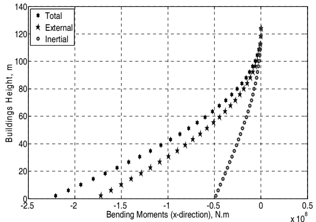
Figure 4: “Load case 28”: vertical distribution of total bending moment M_{xx} , moment associated only to the external pressure loads and moment associated only to the inertial loads.
