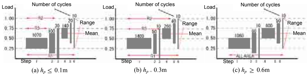
Figure 4: Pressure loading cycles for laboratory testing for a period of 10 min
