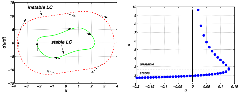
Figure 1: Attractive and repulsive limit cycles stemming from the solution of the basic Eq. (1) - left; The stability diagram for the parameter \vartheta - right.
