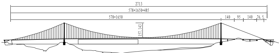
Figure 4: Elevation of Xihoumen Bridge (Unit: m)
