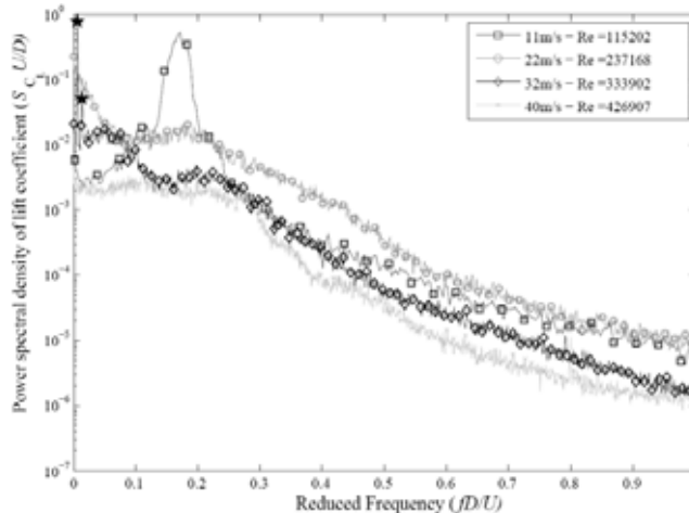
Figure 2: Spectra of the lift coefficient average from the four pressure rings. Star-marked points, 32m/s case, show the resonant peaks that correspond to the structural frequency of 1.4Hz and to twice this value. Model setup, \varphi=60^\circ and \alpha=0^\circ .
