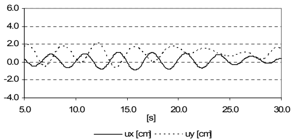
Figure 4: Time history of displacements- u_x , u_y (comp. Fig.2b) -of the middle point of the top floor of the building: a) one building experimental situation- angle of wind attack equal to 135^\circ , b) two buildings experimental situation- angle of wind attack equal to 135^\circ .
