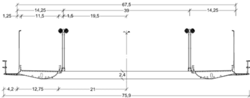
Figure 2: Cross-section of the deck with main suspension cables spaced apart of 39 m.
