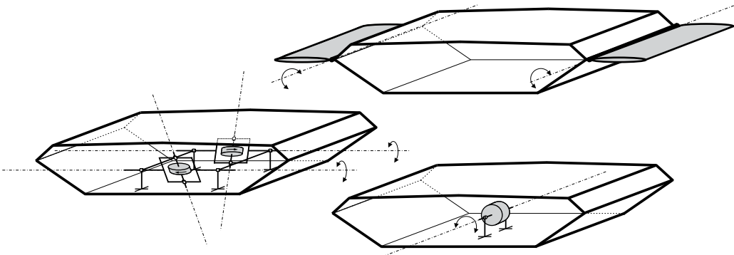
Figure 27: Actuators for stabilising bridges under wind action: aerodynamically effective control shields, twin control moment gyroscope and reaction wheel.
