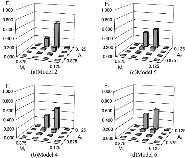
Figure 3: Three-dimensional cycle histogram that shows load cycle distribution over both cycle ranges A and cycle mean levels M ( h_p = 0.1\text{ m} , \theta = 30^\circ , Zone 1)
