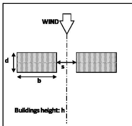
Figure 2: Plan view of the building models
