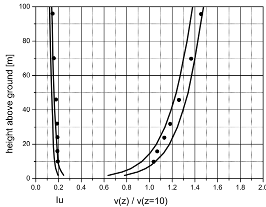
Figure 1: Comparison of the boundary layer flow in the wind tunnel experiment to the ESDU-model for flat, open country
