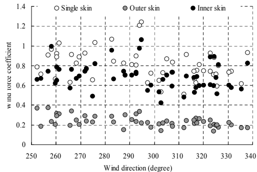
Fig.8 Peak wind force coefficients on the single skin and the outer skin and the inner skin.
