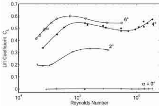
Figure 1: Lift coefficient upon the Reynolds number for different angles of incidence \alpha
