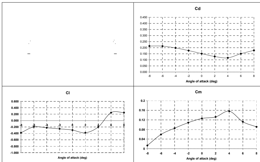
Figure 3: Aerodynamic coefficients for the preliminary design proposal.
