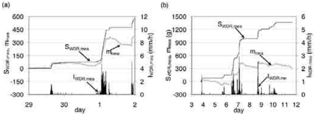
Figure 2: Measurement results of (a) November 29 - December 2, 2007 and (b) December 3 -12, 2007. m_{mea} : weight change of the specimen; S_{WDR,mea} : cumulative amount; I_{WDR,mea} : intensity of wind-driven rain.
