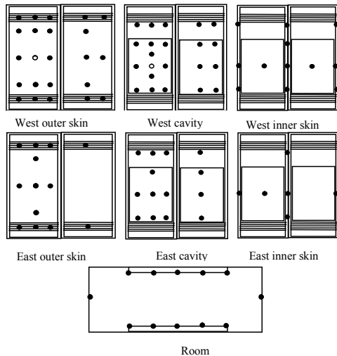
Fig.3 Pressure measurement points
