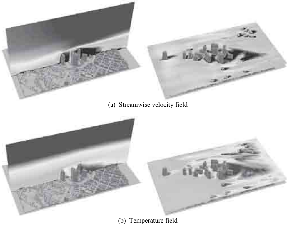
Figure 3: Time-averaged streamwise velocity field and temperature field in vertical section and horizontal section at 60m height.
