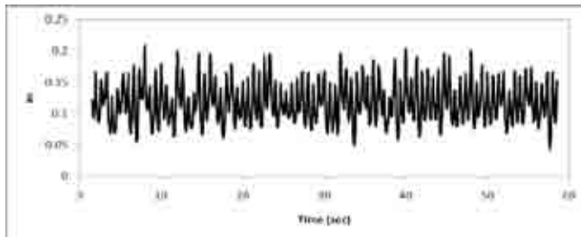
Figure 4 Calculated value of relative displacement of pantograph and overhead contact wire
