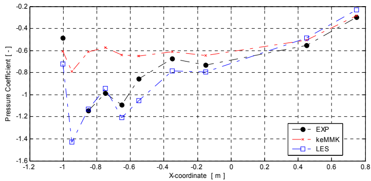
Figure 3: Wind tunnel vs CFD results comparison: pressure coefficient mean values for different simulations compared with experimental results.
