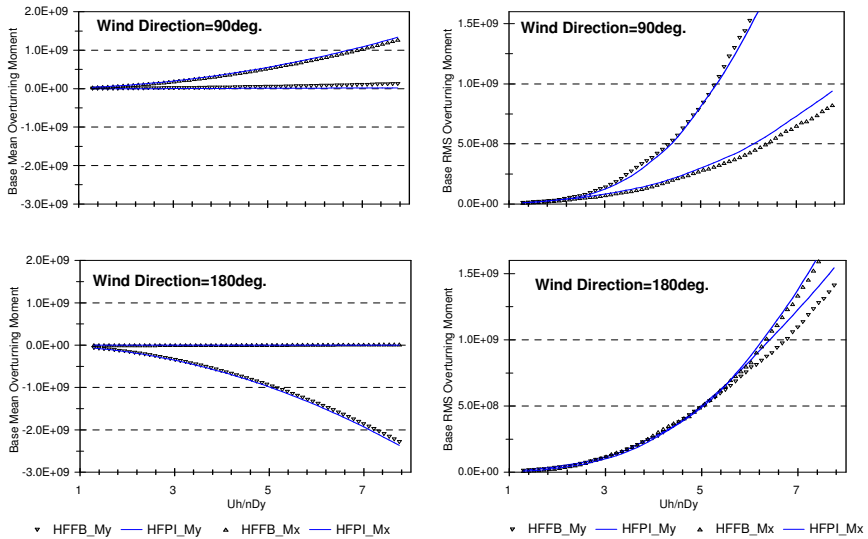
Figure 3: Comparison of base moments predicted by HFFB and HFPI methods as a function of reduced velocity
