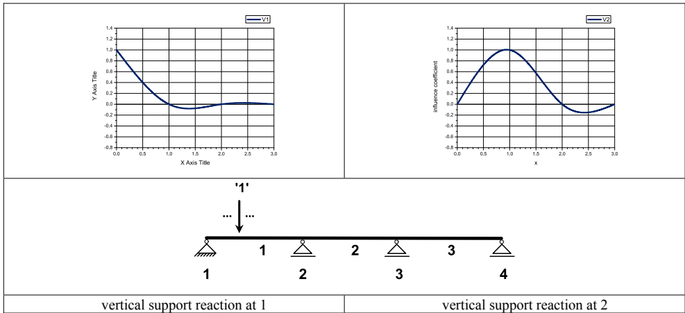
Figure 4: Influence lines for selected support reactions
