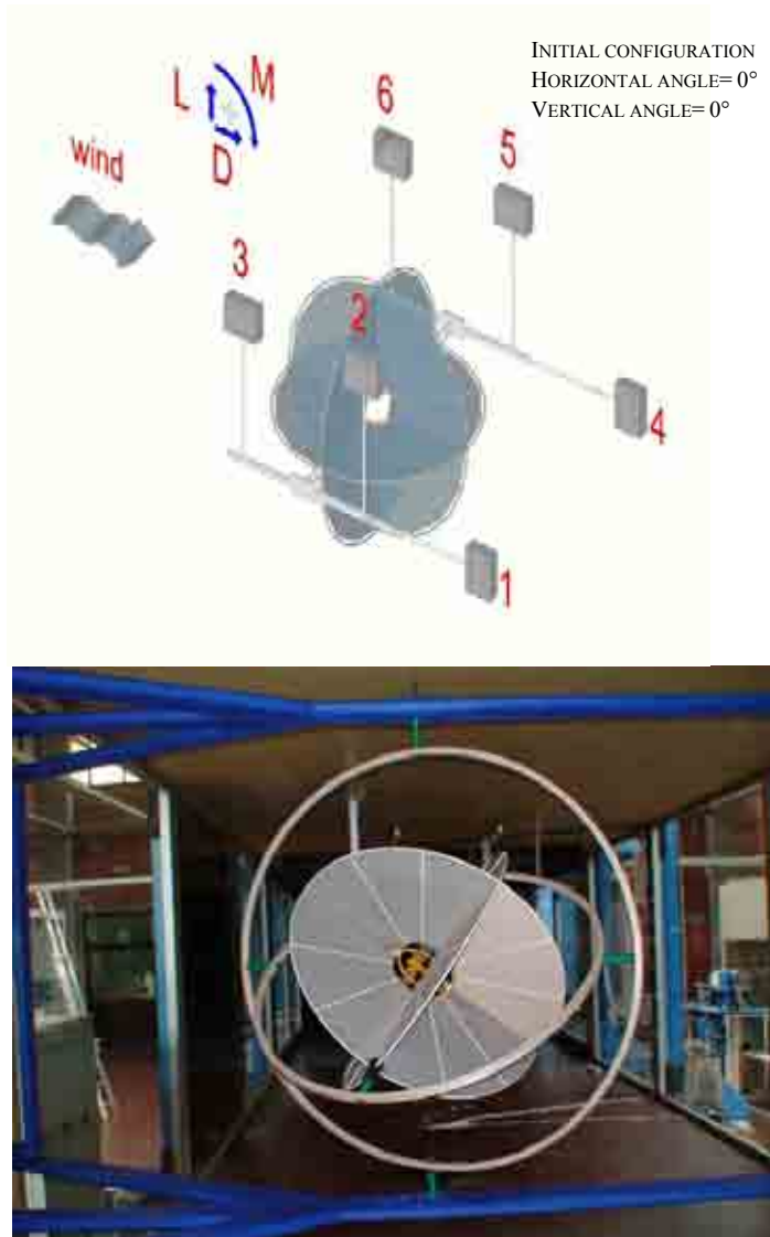
Figure 2: above: experimental setup (6 force measurement points) and sign convention; below: a view of the model in the CRIACIV wind tunnel
