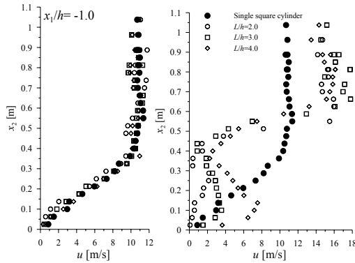
Figure 3: The graphs of velocities in vertical cross-section in front of square cylinder which is: a) the upstream model; b) the downstream model.
