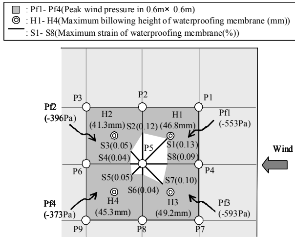
Figure 3: relationship between peak wind pressure, maximum billowing height-strain of waterproofing membrane
