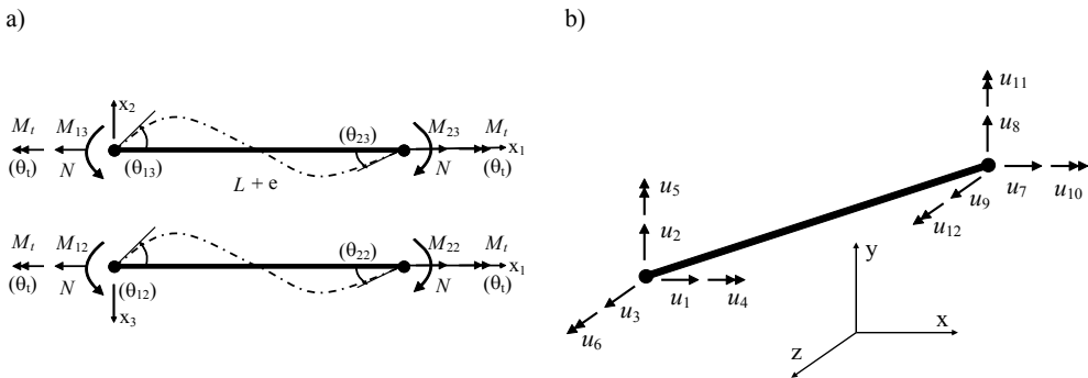
Figure 1. (a) Member basic displacements and forces (principal system); (b) Global reference system displacements.
