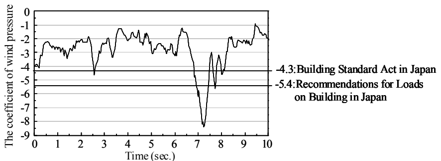
Figure 5: the coefficient of wind pressure for 10 minutes at P7 point
