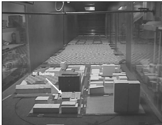
Figure 9: typical wind tunnel set-up for a pedestrian wind assessment study.
