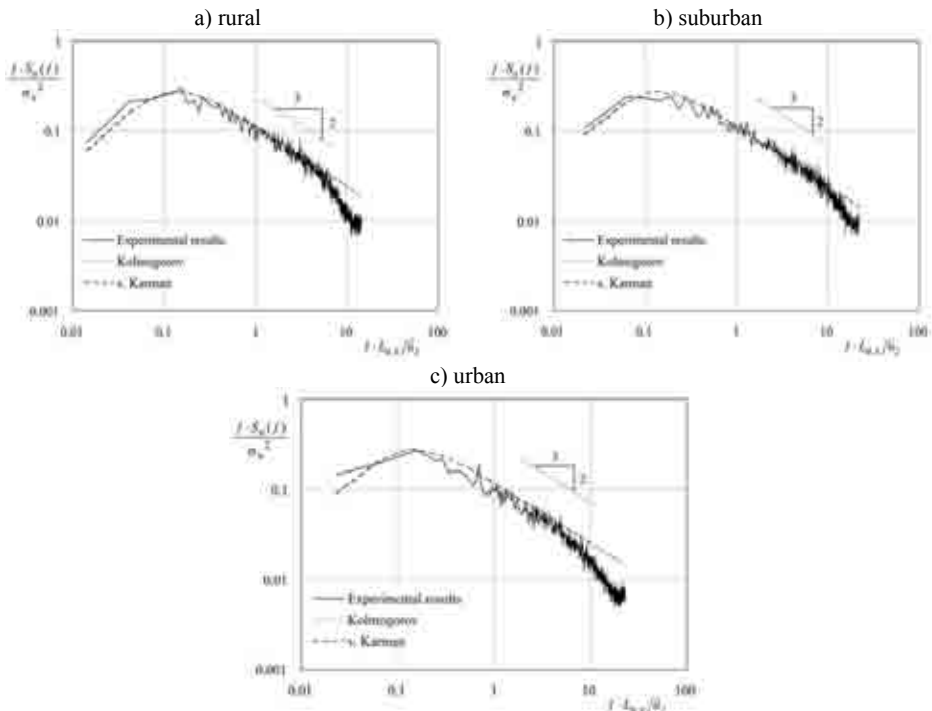
Figure 4: Power spectral density of longitudinal velocity fluctuations at z = 0.2 m; a) rural, b) suburban, and c) urban ABL simulation
