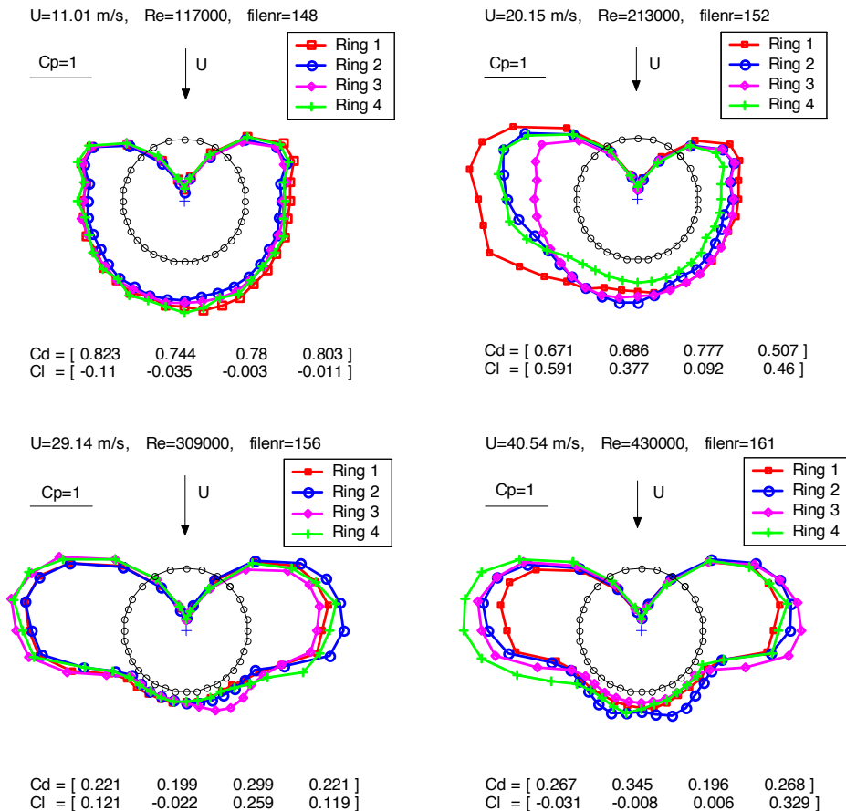
Figure 1: Mean pressure coefficients around cylinder at different Reynolds numbers, fixed cylinder inclined at 59.3^\circ to the approaching flow
