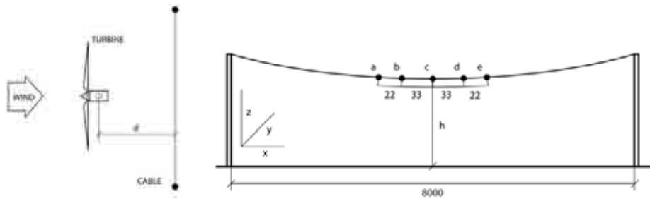
Fig.3: (a) Wind turbine and aeroelastic cable model relative position - (b) Marker position and reference frame.
