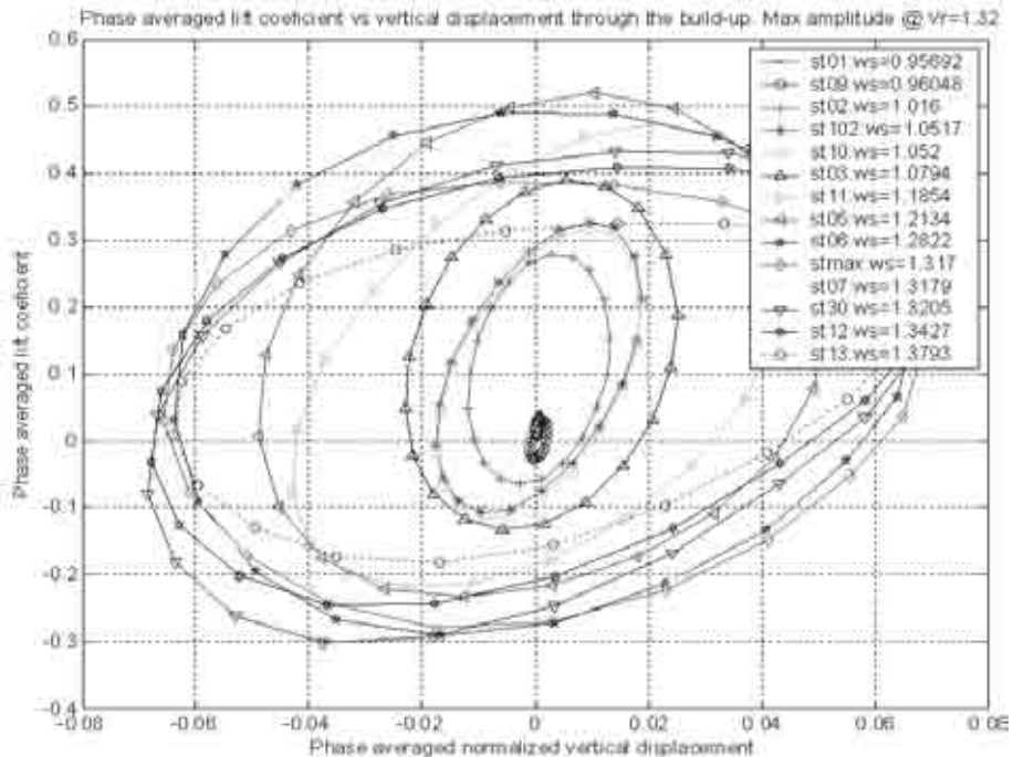
Figure 3: Phase plan diagrams for the simultaneously measured lift force and response for the different phases of the response.
