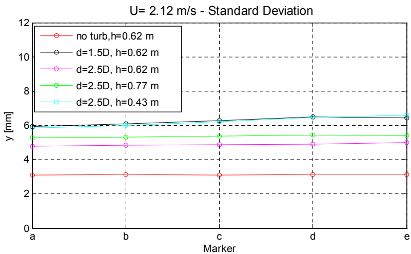
Figure 3: y standard deviation of the 5 monitored points of the aeroelastic cable model.
