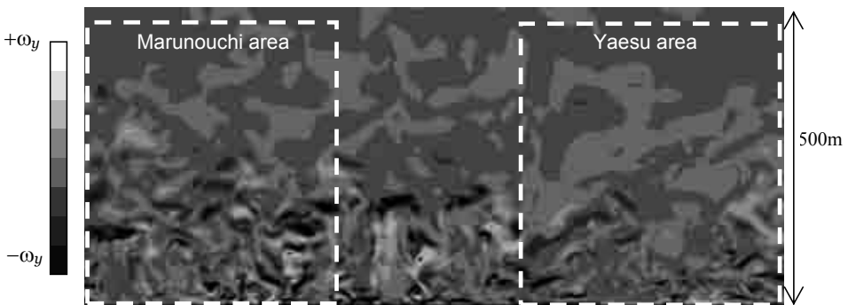
Figure 6: Instantaneous spanwise vorticity contour in mid section of the Marunouchi and Yaesu area.
