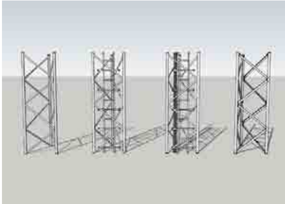
Figure 1: Lattice mast configurations used for full-scale section model testing. From left to right: 1A, 1B, 1C, 2A.
