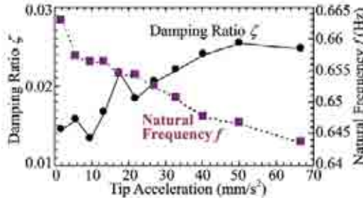
Figure 6: Variation of dynamic characteristics of a 99m-high steel-framed building (Tamura and Suganuma, 1996)
