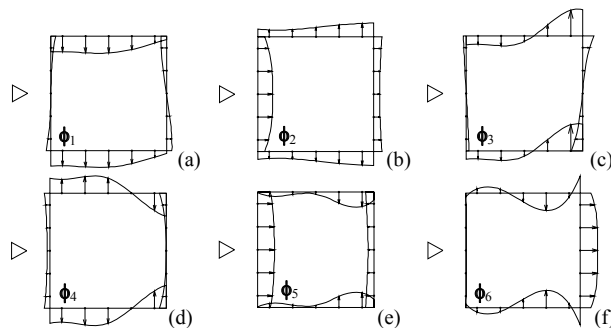
Figure 1: first six PCA modes of pressure field along a high-rise building cross-section.
