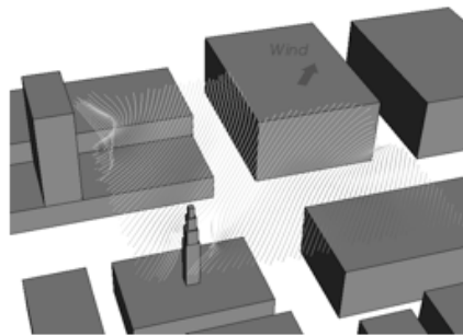
Figure 4: Stream traces for the flow field at the highest horizontal levels (the starting points for the stream traces, forward and backward, are along a diagonal line across the intersection directed from NW to SE at z = 150 mm; where the traces are not visible they are outside of the measurement domain 300 \text{ mm} < x, y < 300 \text{ mm} , 25 \text{ mm} < z < 150 \text{ mm} ).
