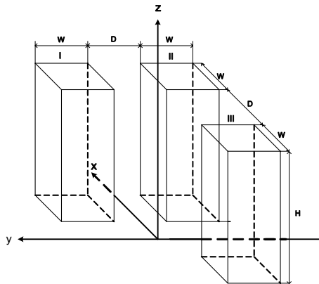
Fig. 1 Schematic diagram of building models arrangement and coordinate system
