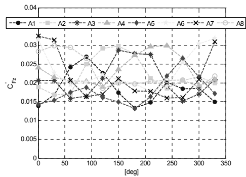
Figure 6: Mean lift force coefficient of each section of the roof.
