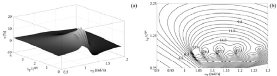
Figure 2: Control effectiveness of IMTMDs ( \varepsilon=0.15 and \delta=0.50 ) as a function of the damping ratio and of the frequency tuning: tridimensional view of the objective function \eta (a); contour plot of the objective function \eta in the region of the optimal solution (values in percentage) (b).
