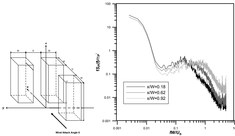
Fig.4 Wind pressure spectrum variations along downstream distance for inner face of building 1 at z/H=0.888
