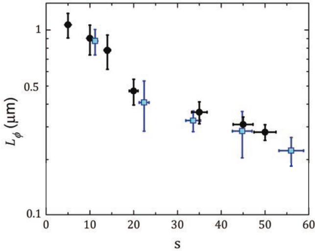
Figure 4.6: L_{\phi} of an array of 1D gases, reported as a function of the transverse confinement which squeezes the gas in 1D micro-tubes. Blue squared and black dots denote the data corresponding to two different values of the momentum of the excitation ( q_{B,1} = 16.0(2) \mu\text{m}^{-1} and q_{B,2} = 7.3(2) \mu\text{m}^{-1} , respectively).
