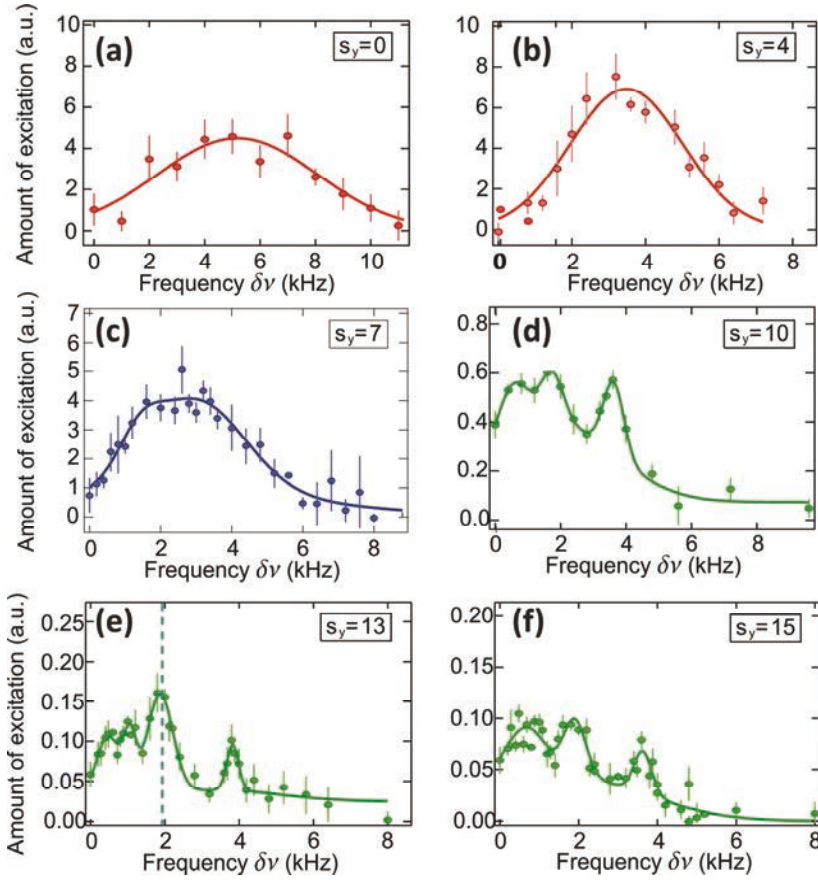
Figure 5.2: Spectra in the lowest energy band measured across the transition from superfluid to Mott insulator. Solid lines are guides to the eye. The vertical dashed line in (e) marks the particle-hole excitation energy \Delta_{ph}(q_B) (see text). Note the reduction in the amplitude of the response (vertical scale).
