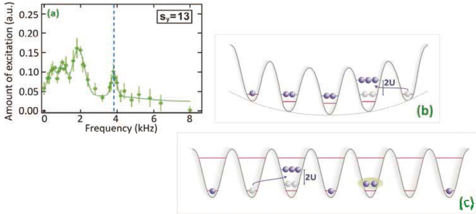
Figure 5.11: (a) Spectrum as in Fig. 5.9. The blue dashed line points out the resonance at \sim 4 kHz, corresponding to an excitation at frequency twice \Delta_{ph}(q_B) . This is the energy required for a particle to hop into a lattice site already occupied by two other particles. Some doubly-occupied (or even multi-occupied) lattice-site can be present in the initial many-body state: Two possible mechanisms at its basis are the slow-varying confinement due to the Gaussian laser-beam profile and the magnetic trapping potential along the axis of the gas (b) and the presence of defects on the lattice filling, induced by a non-perfectly adiabatic loading of the gas in the lattice.
