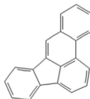
benzo(b)fluoranthene
