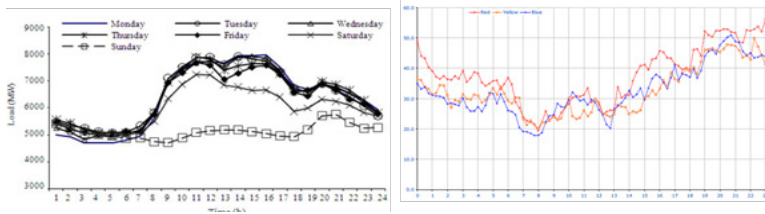
Fig. 2 Typical week load pattern across different sectors (Ismail et al., 2008) and residential aggregate load (Busrah et al., 2011).
