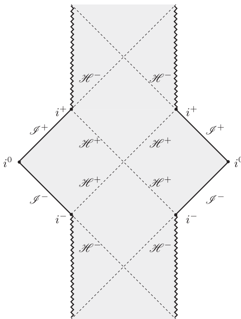
Figure 6.14 Penrose diagram of the Reissner-Nordström spacetime in the non-extremal ( q^2 < m^2 ) case. The points i^0 correspond to the various spatial infinities, the points i^\pm to future and past timelike infinity, respectively, and the lines \mathcal{S}^\pm to the various components of null infinity. The dashed lines \mathcal{H}^\pm correspond to the various horizons. Finally, the serrated lines denote the singularities.
