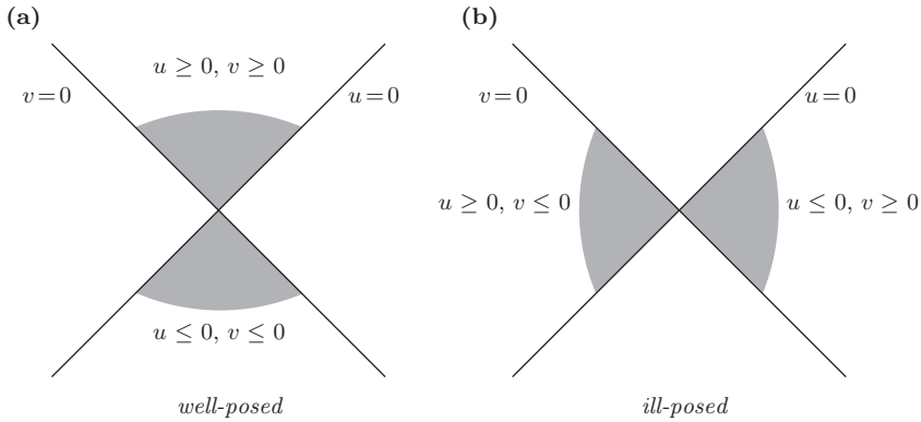
Figure 12.9 Schematic representation of well-posed (a) and ill-posed (b) characteristic initial value problems.
