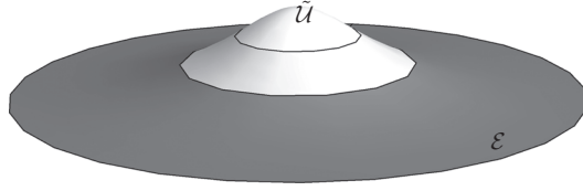
Figure 11.2 Schematic depiction of the exterior gluing construction given by Theorem 11.3. It contains an inner region \tilde{\mathcal{U}} where the 3-metric has a fixed arbitrary value \tilde{\mathbf{h}} , an annular transition region between \mathcal{E}_{r_*} and \mathcal{E}_{2r_*} and an exterior region \mathcal{E} where it is equal to data for a member of the Schwarzschild family of solutions.
