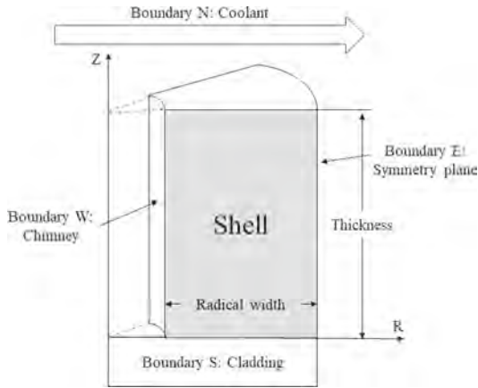
Fig. 2. Schematic diagram of coordinates and boundary conditions
