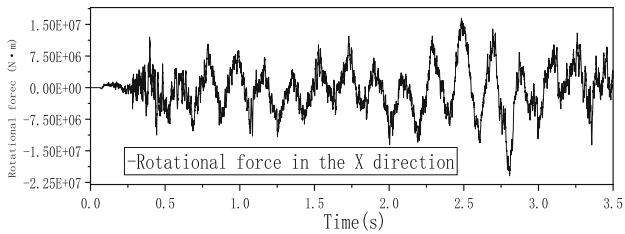
Fig. 21. The time history curve of the rotating force on the bearing in the X direction
