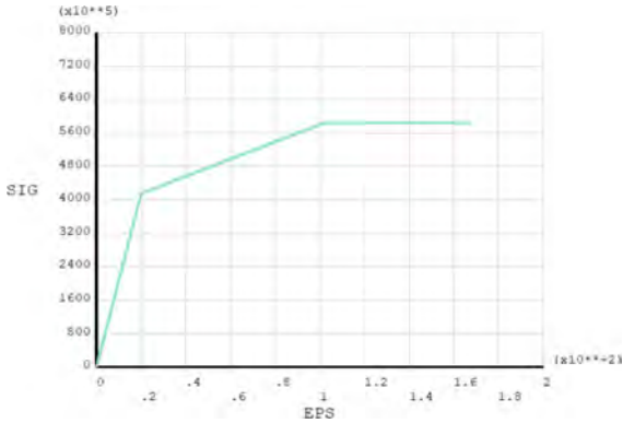
Fig. 4. Constitutive relation of material model
