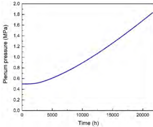
Fig. 5. Evolution of the plenum pressure.
