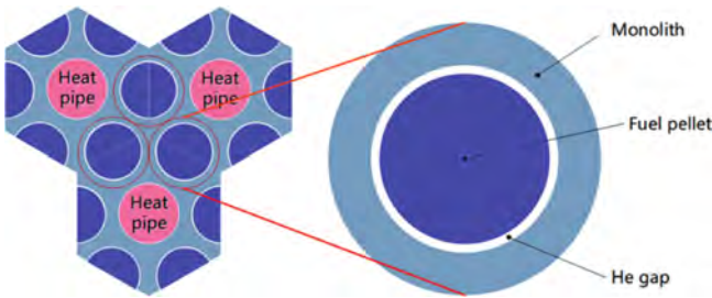
Fig. 3. Mechanical model
