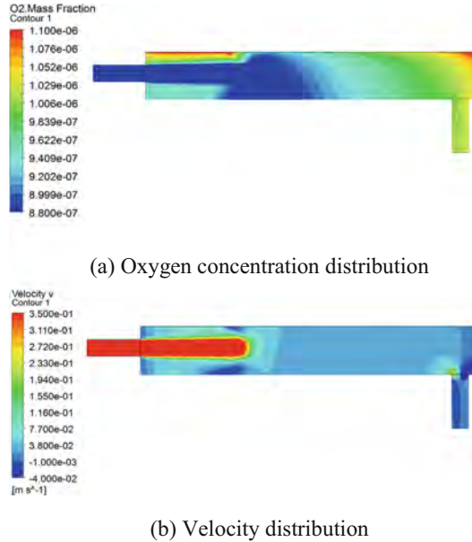
Fig. 3. The distribution of oxygen concentration and velocity under the typical working condition ( T_{\text{lbe}} = 550 \text{ }^\circ\text{C} , u_{\text{lbe}} = 0.5 \text{ m/s} , C_{\text{in}} = 8 \times 10^{-7} \text{ wt\%} , C_{\text{g/l}} = 1 \times 10^{-5} \text{ wt\%} )
