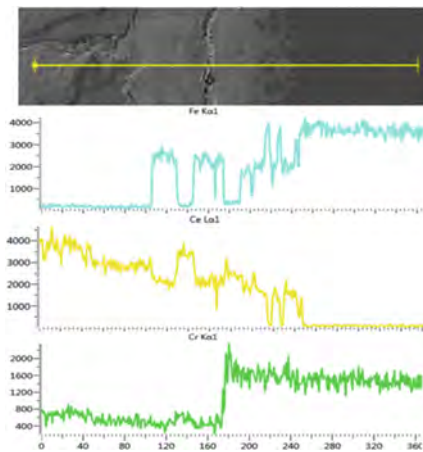
Fig. 8. Element line scan analysis at interface
