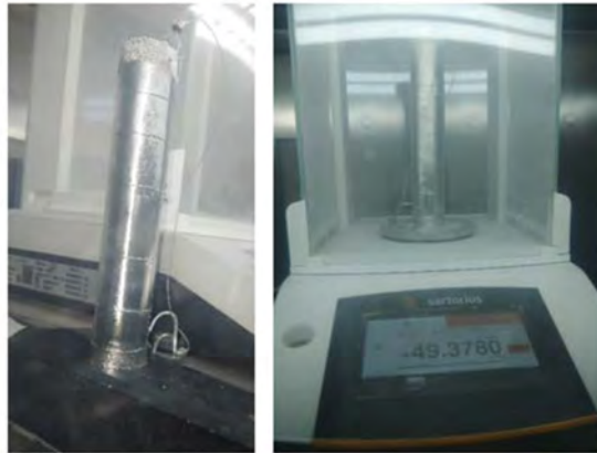
Fig. 5. wire mesh wick sodium aspiration experimental result diagram.
