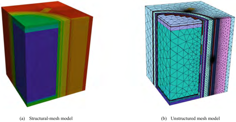
Fig. 5. Structural-mesh and unstructured-mesh models for HBR-2 benchmark
