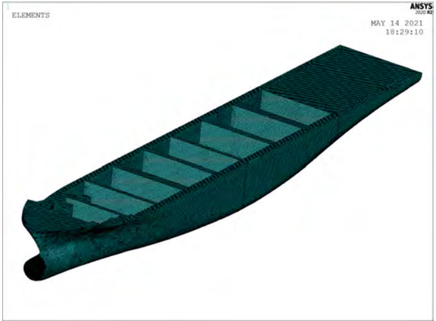
Fig. 1. Finite element model of container ship.
