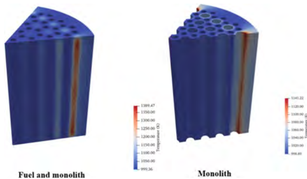
Fig. 7. Temperature distribution
