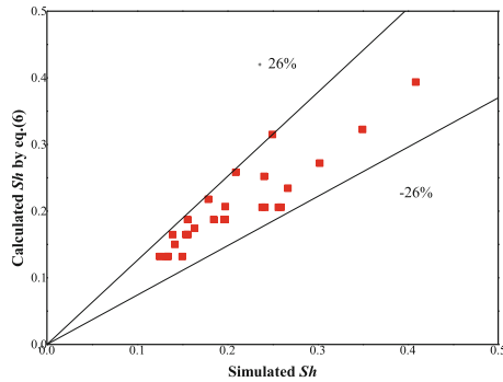
Fig. 6. The deviations between simulated results and calculated results by (6)
