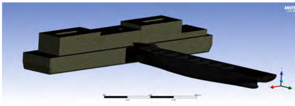
Fig. 5. Finite element model of two ship impact.
