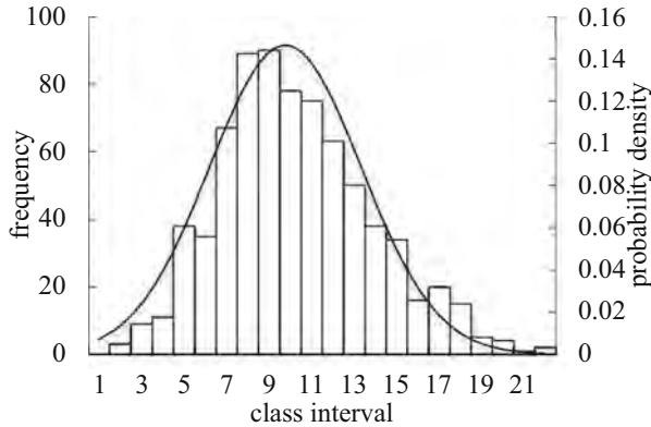
Fig. 6. Normal distribution curve of compressive strength
