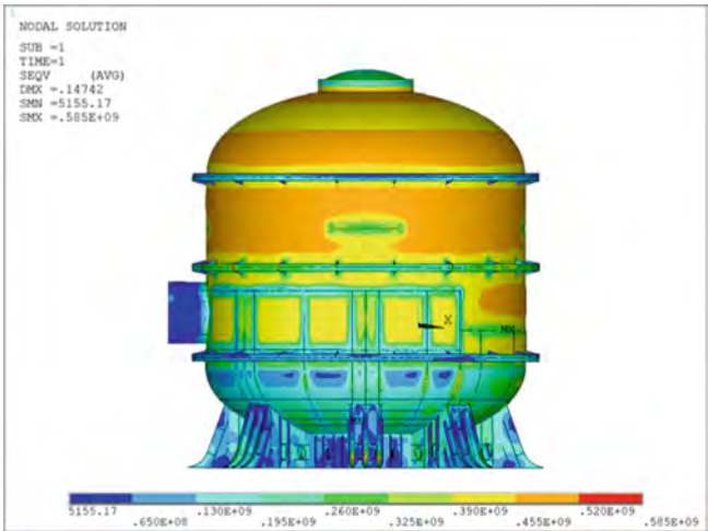
Fig. 11. Stress nephogram of steel containment in case of strength failure
