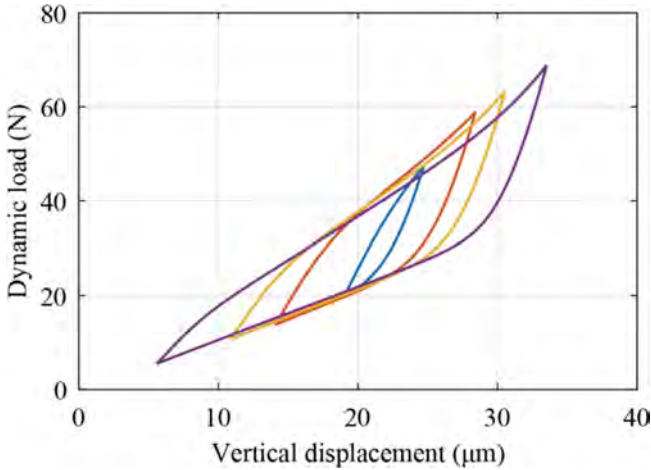
Fig. 6. Influence of the Stribeck effect on the hysteresis curves with different excitation amplitudes.
