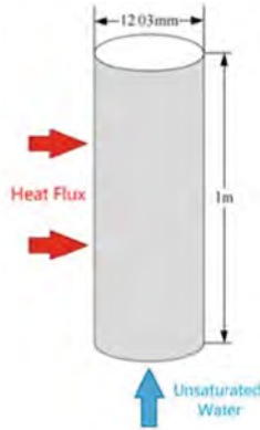
Fig. 2. Schematic Diagram of Test Piece Geometry
