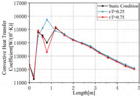
Fig. 6. Convective Heat Transfer Coefficient Curves at Different Times
