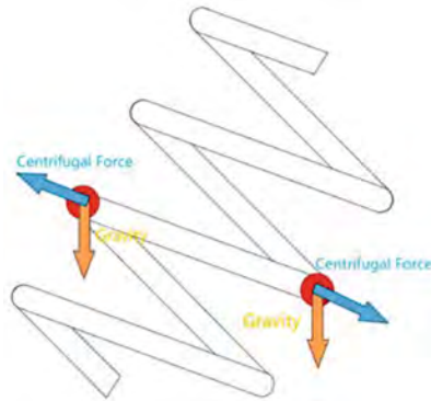
Fig. 12. Force Analysis of Fluid in Spiral Tube in Inclined State
