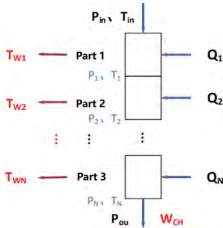
Fig. 5. Single channel boundary conditions and control volume partition schematics
