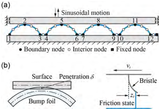
Fig. 2. Modeling of the system: (a) the schematic of the system and the reduction scheme of the bump foil and (b) the diagram of the frictional contact.
