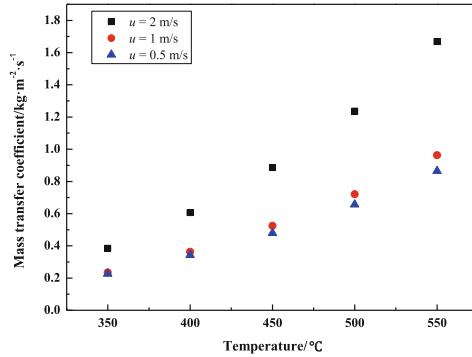
Fig. 4. The effects of the temperature and the velocity of LBE on the average oxygen mass transfer coefficient
