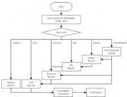
Fig. 2. Flowchart of CSG-CAD conversion
