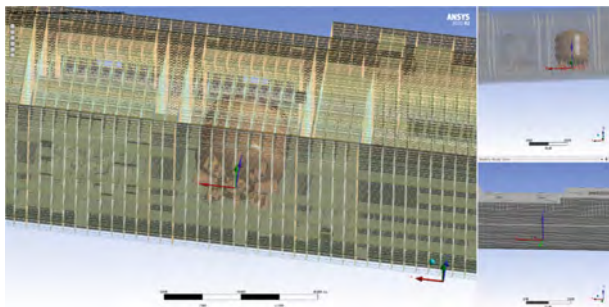
Fig. 7. Connection between containment and floating nuclear power plant.
