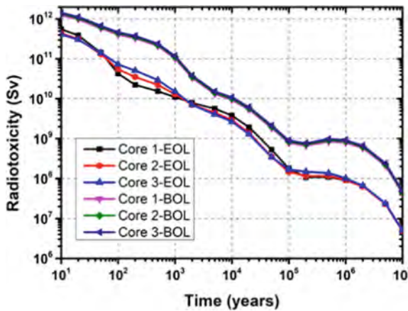
Fig. 7. Evolutions of the total radiotoxicity with Flibe and Flinak salts in the three MSR cores
