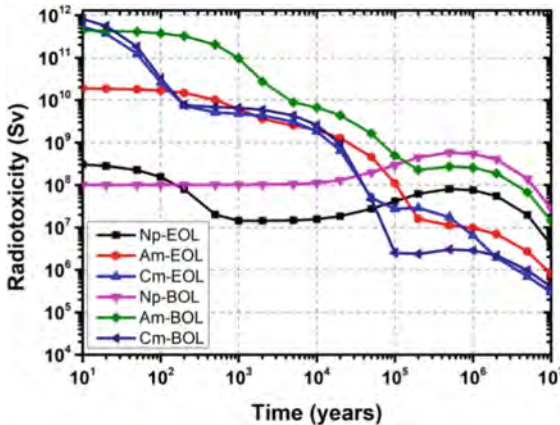
Fig. 8. Evolutions of the MA radiotoxicity with Flibe salt in the thermal MSR core
