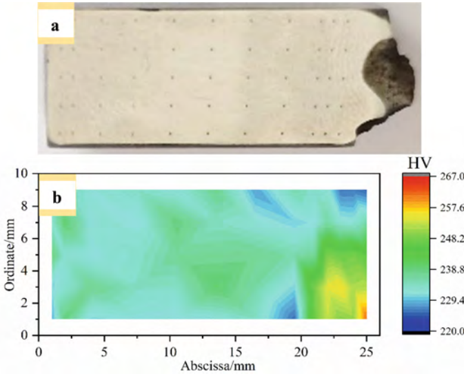
Fig. 7. The hardness distribution of the impact fracture at the upper shelf. a) impact fracture, b) The hardness distribution graph.
