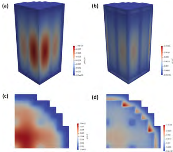
Fig. 5. (a) (c) Fast flux and (b) (d) Thermal flux distribution of 3D-IAEA problem
