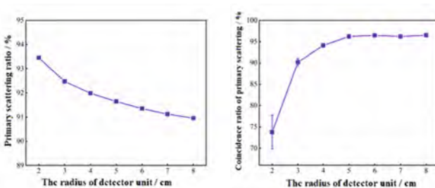
Fig. 7. The radius of detector unit Vs. Primary scattering ratio and coincidence ratio of primary scattering
