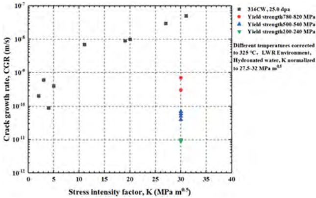
Fig. 9. CGR and K of 316CW material irradiated at 25.0 dpa, CGR of the material at different yield strengths when K is 30 \text{ MPa m}^{0.5} [14–18].
