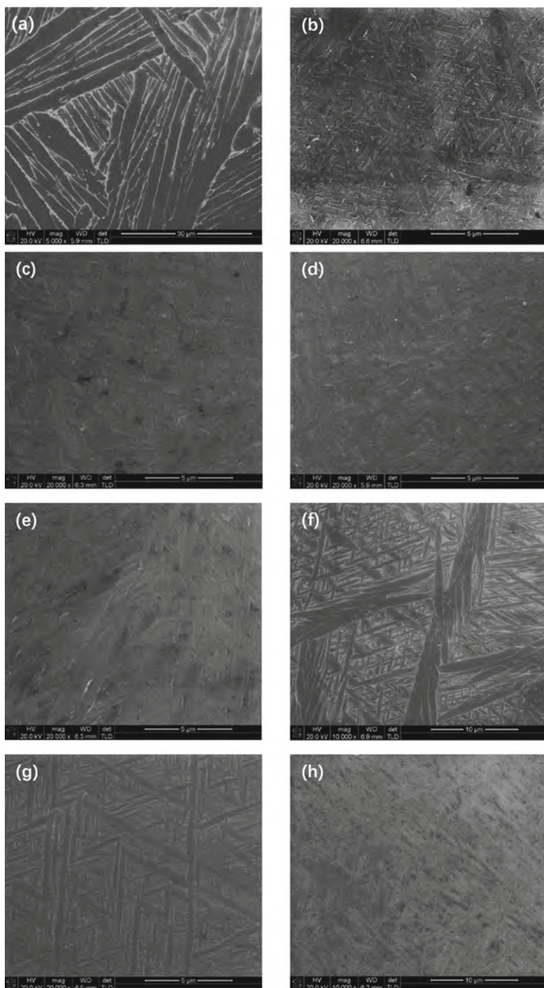
Fig. 3. RD-ND surface SEM images of Zr-Sn-Nb-Fe billet sheet specimens under different quenching processes (a) as forged (b) 950 °C/0.5 h (c) 1050 °C/0.25 h (d) 1050 °C/0.5 h (e) 1050 °C/1 h (f) 1050 °C/2 h (g) 1150 °C/0.25 h (h) 1150 °C/1 h
