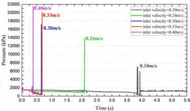
Fig. 8. Effect of subcooled water inlet velocity on CIWH
