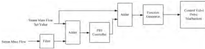
Fig. 2. The Control Schematic Diagram of the Steam Mass Flow
