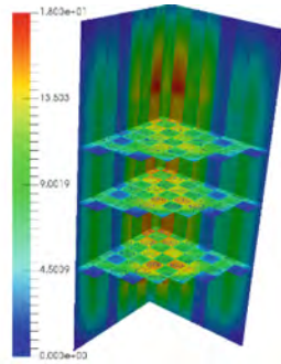
(b) power distribution at the end
