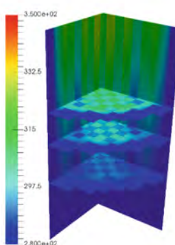
(f) the temperature of coolant at the end
