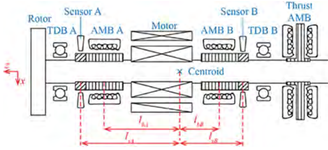
Fig. 1. AMB-rotor system
