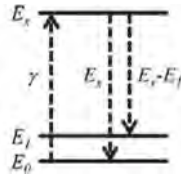
Fig. 1. NRF excitation-de-excitation process
