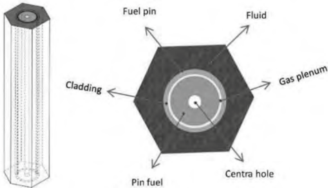
Fig. 6. Model of fuel pin channel [6]
