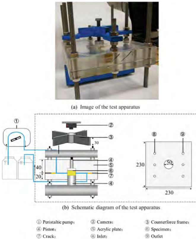
Fig. 1. Setup for conducting the intrusion/erosion test
