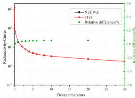
Fig. 1. Comparison of the radioactivity between TIST and NECP-X
