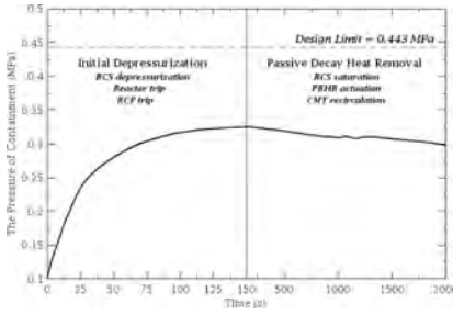
Fig. 7. Containment Pressure
