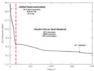
Fig. 3. RCS Pressure
