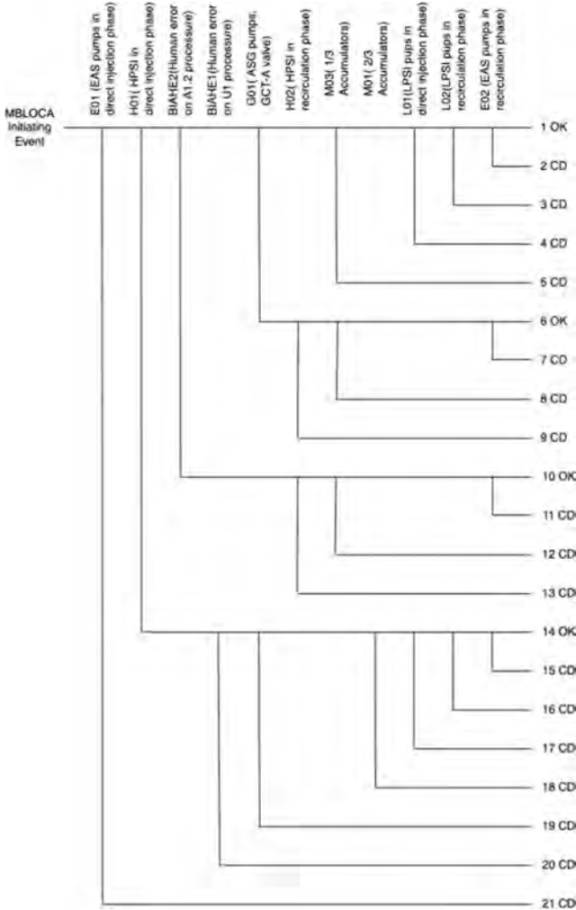
Fig. 3. MBLOCA Event Trees
