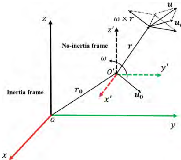
Fig. 1. Relationship between the non-inertial frame and the inertial frame.
