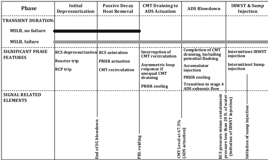
Fig. 9. MSLB Transient Scenario (Wilson et al. 1997)
