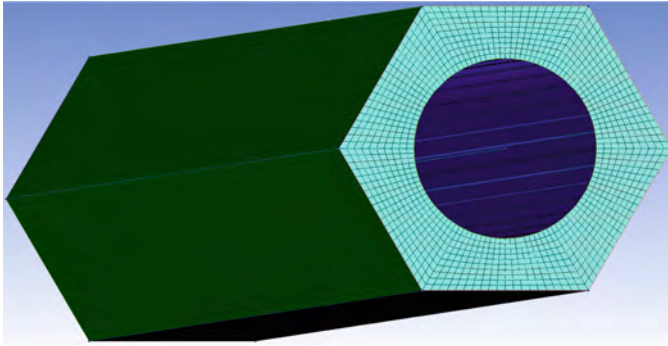
Fig. 7. Mesh generation of coolant channel
