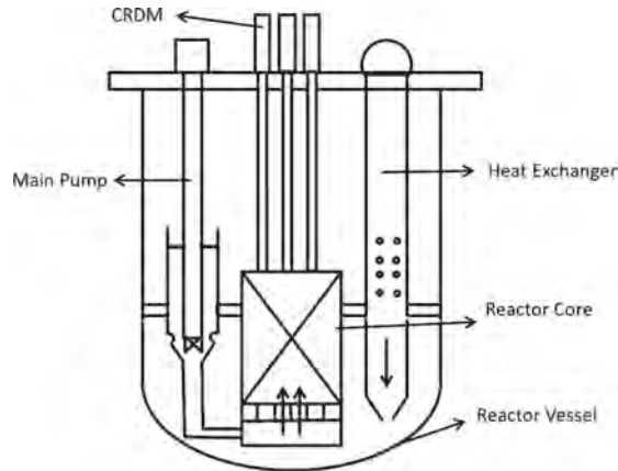
Fig. 1. Schematic Diagram of Pool-type Structure of Lead-bismuth Fast Reactor
