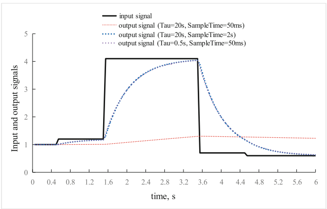
Fig. 4. Output of filter with different \text{Tau} and \text{SampleTime}
