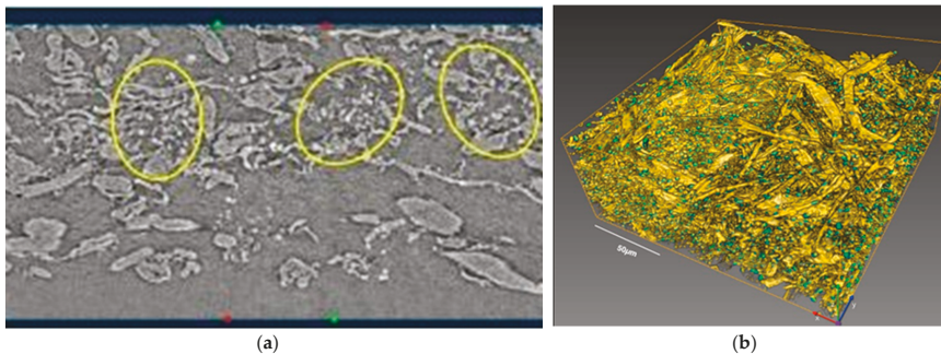
Figure 6.17. (a) X-ray microtomography of Stain A. One of the ‘slices’ from approximately 1500 X-ray micro-tomographs ( \mu CT) generated at ESRF shows a cross-section of stain type A. (b) The 3D visualization of a black stain type A derived by compiling and processing X-ray micro-tomography data, on beam ID19 at synchrotron ESRF. The green particles are spores dispersed in the paper matrix. Source: Reprinted from (Szczepanowska et al. 2015).
