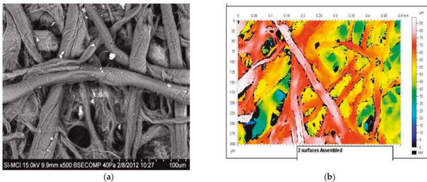
Figure 5.15. (a) The surface morphology captured on SEM-VP micrograph shows well-preserved fibers. There is no evidence of any additives, which was confirmed with EDS analysis. SEM-VP, scale bar 100 \mu\text{m} . (b) The 3D surface topography of an area 500 \mu\text{m} x, 300 \mu\text{m} y, 85 \mu\text{m} h, show well-defined individual fibers, loosely interconnected and well-articulated. Surface morphology was generated based on data collected by white-light profilometer (WLP). Source: Figure by author.
