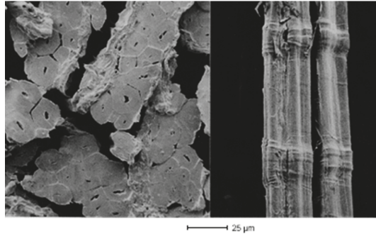
Figure 2.17. Flax (linen) fibers, often used in artist's paper, are seen here in an SEM micrograph. The morphological features of their surface (prominent nodules) and their cross-sections are used as diagnostic features in the comparative analysis of paper fiber content. Source: Reprinted from http://www.freewebs.com/textile-technology/fibrescience.htm (accessed on 13 April 2012).
