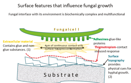
Figure 4.8. Visualization of fungal interactions with the substrate's surface (not to scale). The typical size of fungal spores ranges from 5 to 9 \mu\text{m} . Spores flatten upon contact with the surface to enlarge the area of attachment. Source: © Szczepanowska 2011; drawings based on description in article by (Nicholson et al. 1988; Pascholati et al. 1993; Hoch et al. 1987).
