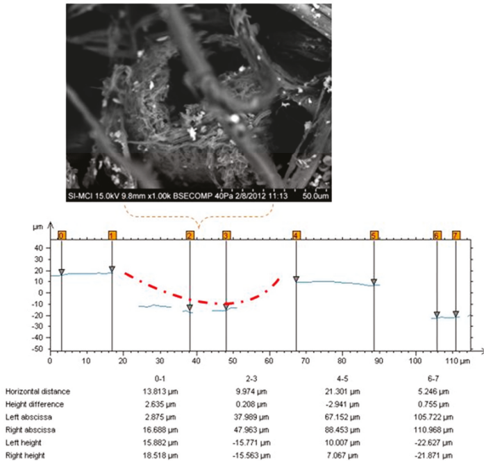
Figure 6.16. A fungal inclusion in stain type B. The SEM-VP micrograph is aligned with a profile generated by non-contact, white-light profilometer; it corresponds with the shape and size of the fruiting structure. The diameter of the embedded part of the fruiting body was 50–60 µm, and the ‘void area’ indicated by lack of data was near 50 µm. The depth of fruiting body ‘immersion’ in the paper matrix is ca 25 µm. Source: Reprinted from (Szczepanowska et al. 2013).
