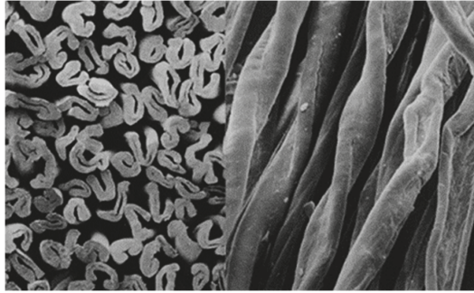
Figure 2.16. Longitudinal study and cross-sections of cotton fibers. The characteristic, ribbon-like twist is one of the identifying features of cotton fibers. The cross-section of cotton fibers shows the water entry areas. SEM micrograph. Source: Reprinted from http://www.freewebs.com/textile-technology/fibrescience.htm (accessed on 13 April 2012).
