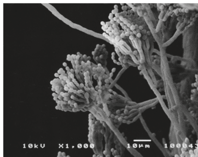
Figure 2.6. Chains of conidiospores of Penicillium chrysogenum . SEM micrograph, scale bar: 50 \mu\text{m} . Source: Reprinted from (Szczepanowska and Cavaliere 2003, Figure 8b, p. 141).
