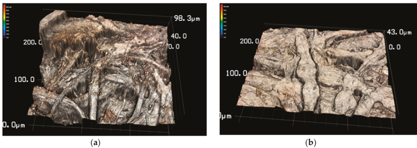
Figure 2.21. (a) Three-dimensional topography captured with confocal laser scanning microscope shows rough surface with well-pronounced fibers, and numerous fungal cells. (b) Confocal laser scanning micrograph, 3D topography of the reverse side of the same paper, smoother than recto, seen in Figure 2.21, on which no fungal cells were detected. Source: Figure by author.
