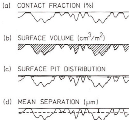
Figure 2.19. The diagram shows various ways in which the surface topography of paper can be defined and measured. Source: Reprinted from (Bristow 1986a, p. 172), used with permission.
