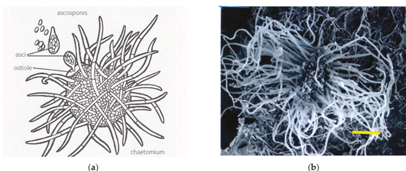
Figure 2.10. (a) A schematic drawing of an ascocarp (perithecium) of Chaetomium , showing seta (perithecial hairs) and asci being released via the ostiolo. Each ascus contains eight ascospores. Source: Reprinted from (Szczepanowska 1986, p. 34). (b) Chaetomium globosum , perithecium with seta, perithecial hairs, growing in all directions. The species was growing on deteriorated paper pamphlets. Scale 20 \mu\text{m} . Source: Reprinted from (Szczepanowska and Cavaliere 2000, p. 248).
