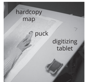
Figure 1.2: Digitizing tablet for manual map digitization
