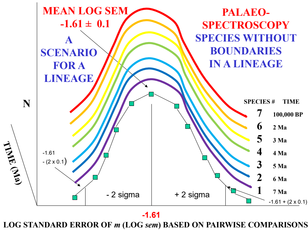
Figure 4. A scenario in which log sem values for seven species within a lineage spanning 7 million years (Fig. 3) are distributed. In each case they are associated with a mean log sem value of -1.61 \pm 0.1 for conspecifics (see Fig. 2 and Table 1).
