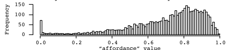
Histogram of finds "affordance" - early medieval
