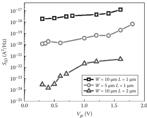
FIGURE 6.21 Variation of drain current noise power spectral density for three devices with W/L = 10 \mu\text{m}/1 \mu\text{m} , W/L = 5 \mu\text{m}/1 \mu\text{m} , and W/L = 10 \mu\text{m}/2 \mu\text{m} at V_{ds} = 0.05 \text{ V} and f = 150 \text{ Hz} .
