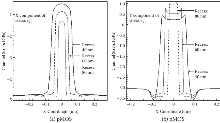
FIGURE 7.2 Profiles of the (a) lateral stress component \epsilon_{xx} and (b) vertical stress component \epsilon_{yy} in a transistor structure for different stressor depths where the gate length L is 45 nm.
