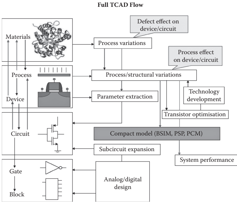
FIGURE 1.4 Compact multilevel technology/device/subsystem modelling flow. (After Maiti, T. K., Process-Induced Stress Engineering in Silicon CMOS Technology, PhD thesis, Jadavpur University, 2009.)
