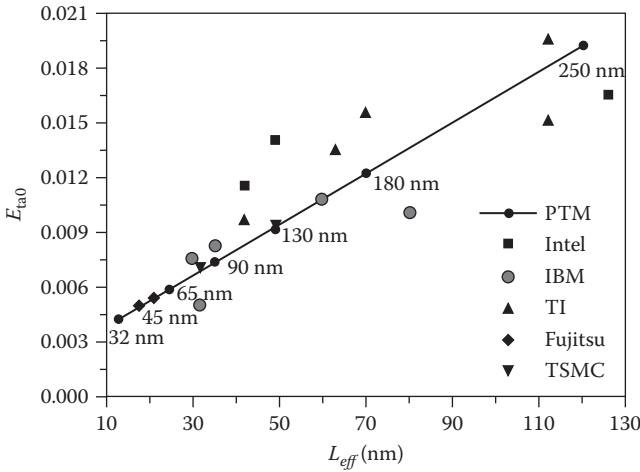
FIGURE 9.6 Trend of DIBL coefficient E_{tao0} scaling from the 250 nm to 32 nm nodes. (After Zhao, W., Predictive Technology Modelling for Scaled CMOS, PhD thesis, Arizona State University, 2009.)
