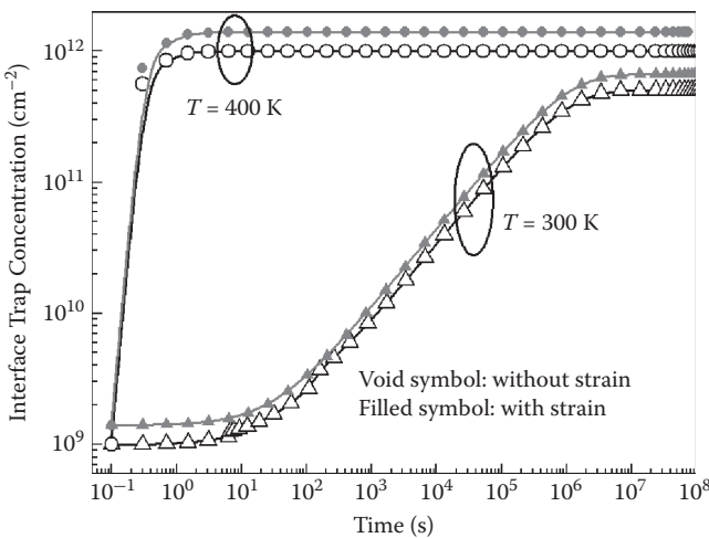
FIGURE 8.1 Temperature dependence of interface state degradation with the change in drain stress bias.
