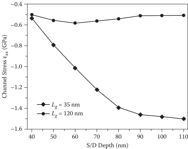
FIGURE 7.3 Stress boosting in p-MOSFETs by increasing SiGe depth for 35 and 120 nm gate length devices.
