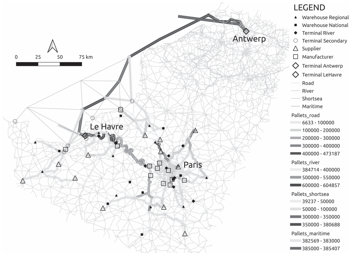
Figure 14.5 Scenario 1 (Run 1) flow of goods (in pallets). All ports are active. These values are taken at the 86,400th time step (equivalent to 60 days or 2 months of simulated time).
