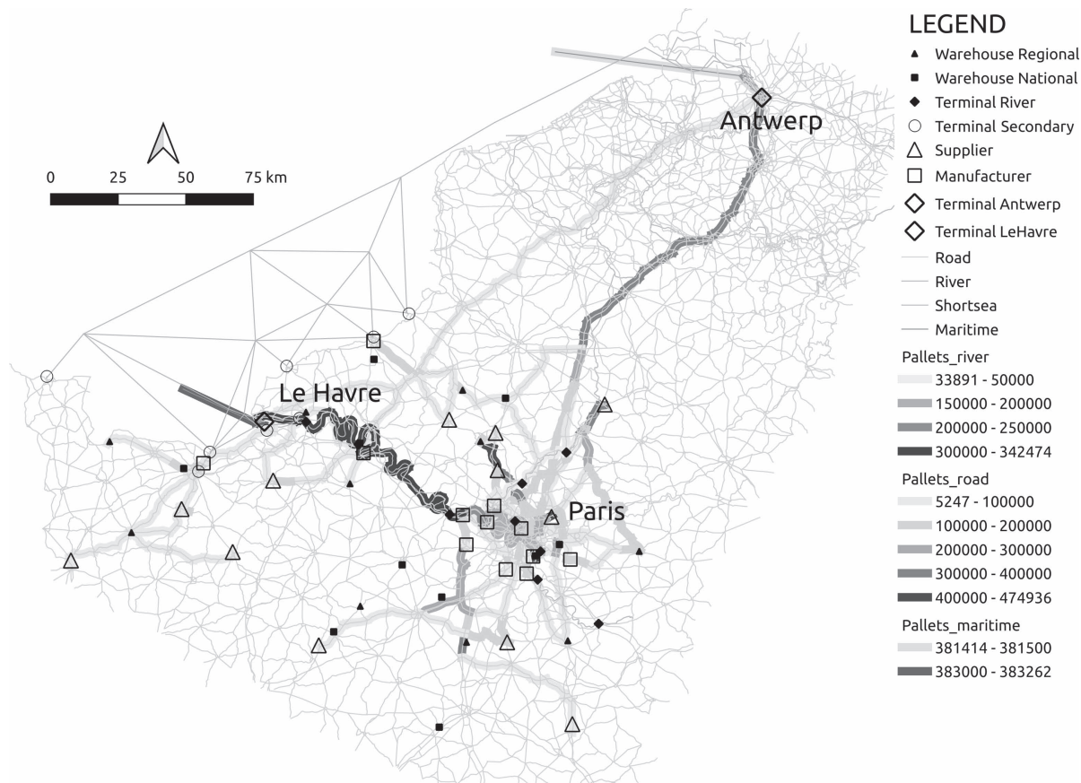
Figure 14.6 Scenario 4 (Run 1) flow of goods (in pallets). There is no short sea traffic (short sea ports are not active). The stocks from the port of Antwerp are transported to national warehouses via trucks. These values are taken at the 86,400th time step (equivalent to 60 days or two months of simulated time).
