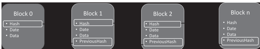
Figure 12.1 Chaining mechanisms in blockchains.
