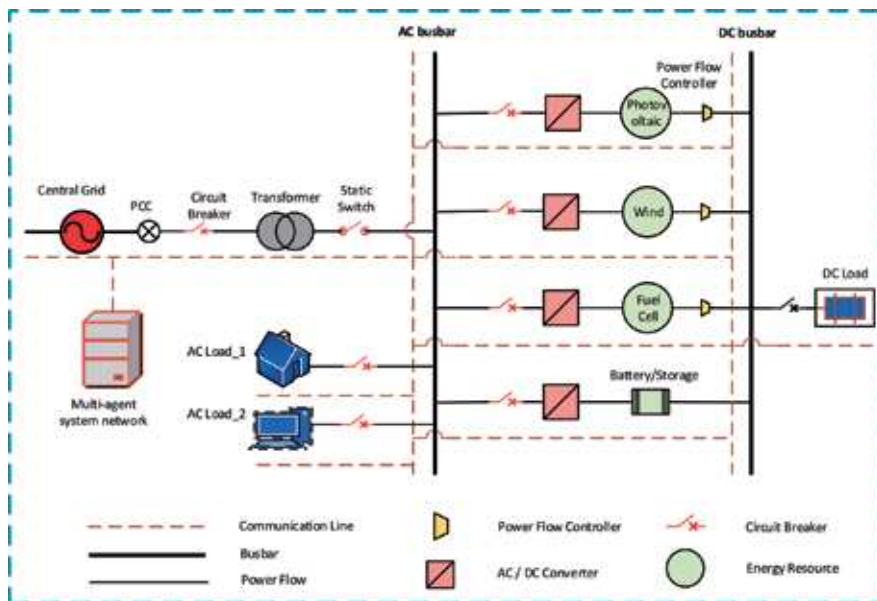
Figure 3. Structure of the proposed supervision system at the DMG level.
