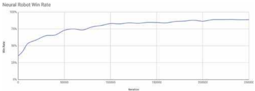
Figure 9. Winning percentage of AUNNRobot within rounds.
