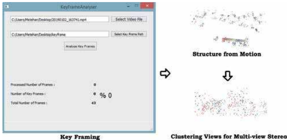
Figure 2. Overview of the pipeline.
