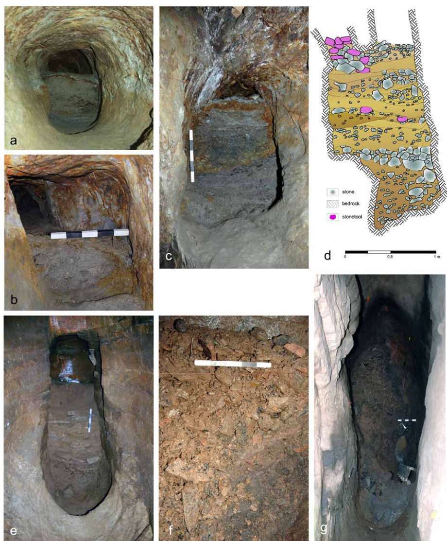
Figure 8: Refilled Bronze Age mining galleries: Arthurstollen, Austria, copper ore mining, search galleries (a) North gallery, (b) Cierny gallery, (c) profiles; Sakdrisi, Georgia, mine 1/2 North extension, western extraction gallery, gold mining (d); Askaraly II, Kazakhstan, tin ore mining, extraction galleries: East gallery (e), west gallery, detail of debris refilled upper part (f), and top view of refilled mining debris (g) (courtesy: DBM/RUB, J. Cierny, Th. Rabsilber, Th. Stöllner, P. Thomas).
