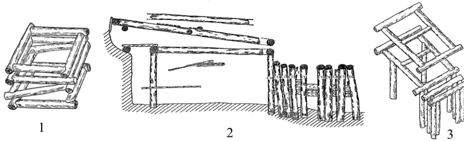
Figure 6: Timbering structures at Gangxia. 1: shaft (from: Gangxia, 1988, p.34); 2: gallery (from: Gangxia, 1988, p.40); 3: junctions between the shaft and gallery (from: Gangxia, 1988, p.40).
