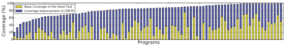
Fig. 5. Coverage improvement over seed test case by CRETE on GNU COREUTILS
