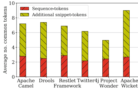
Fig. 8. Additional information revealed when mining snippets instead of sequences.
