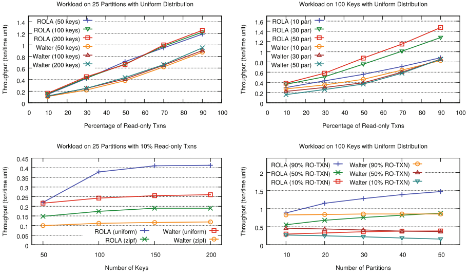
Fig. 1. Throughput comparison under different workload conditions.
