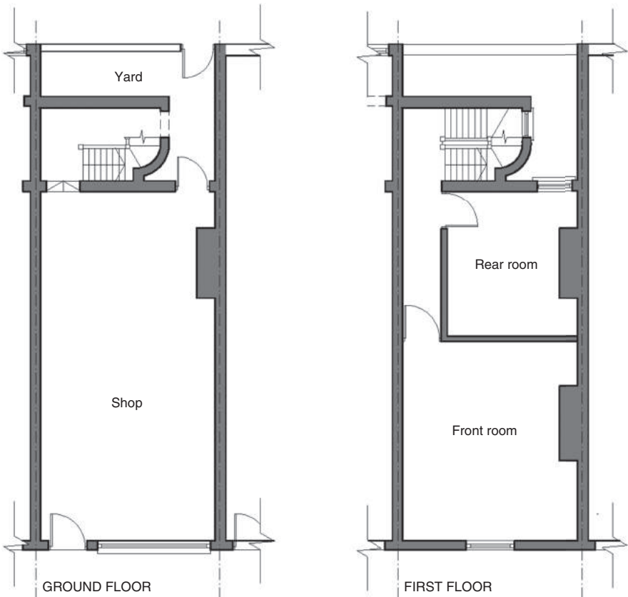
Figure 5.10. Plan of original layout of 89 (41) Dale Street, Liverpool. Drawing by Stephen Leighton, based on a survey by Stephen Corbett.
