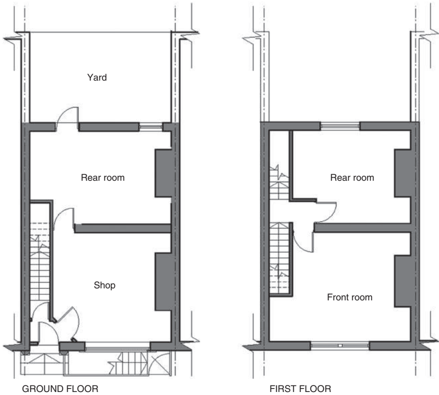
Figure 5.6. Plan of original layout of 33 Thomas Street, Manchester. Drawing by Stephen Leighton based upon a survey by the Manchester Regional Industrial Archaeology Society.
