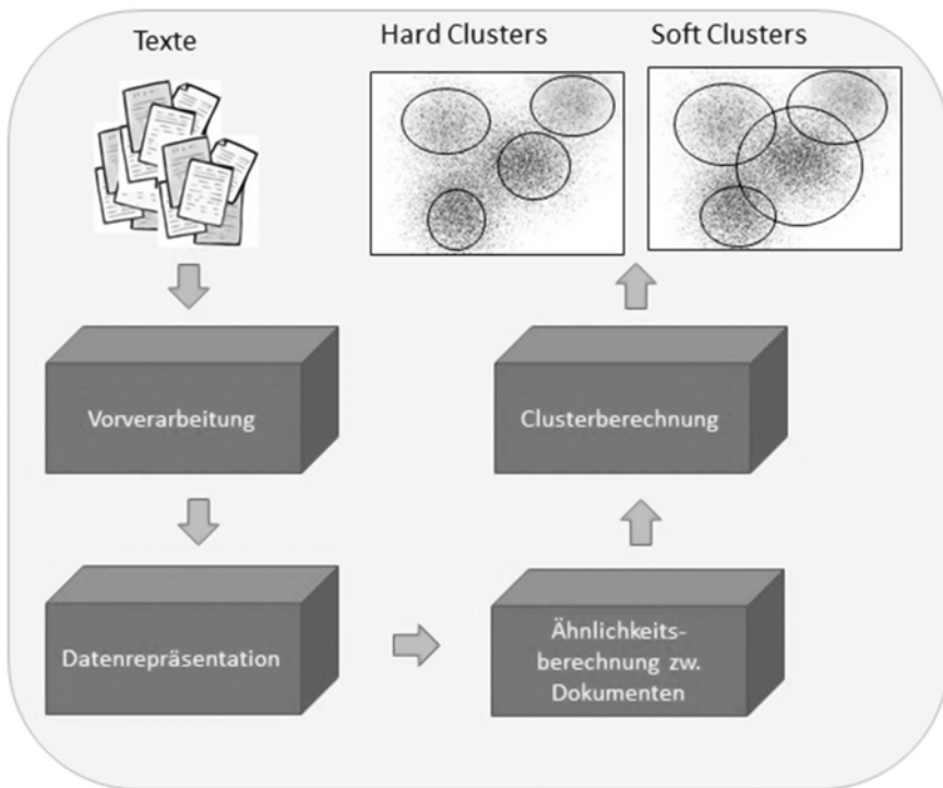
Abb. 4: Document Clustering (Brigitte Krenn).
