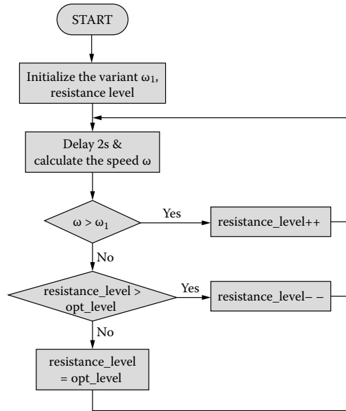
FIGURE 3.13 Flowchart of the automatic control of the resistance system.
