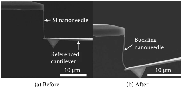
FIGURE 9.15 Calibration of the Si nanoprobe (a) before buckling and (b) after buckling.
