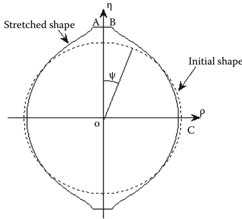
FIGURE 8.1 Coordinates definition before and after optical stretching. Image courtesy of Y. Tan, used with permission from IEEE (Tan et al. 2009).
