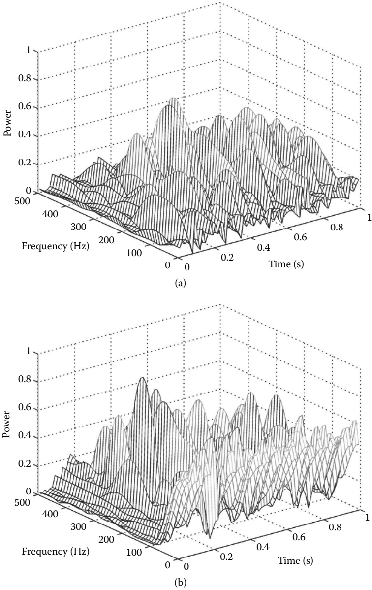
FIGURE 12.9 STFT results at different speeds: (a) low speed and (b) high speed.
