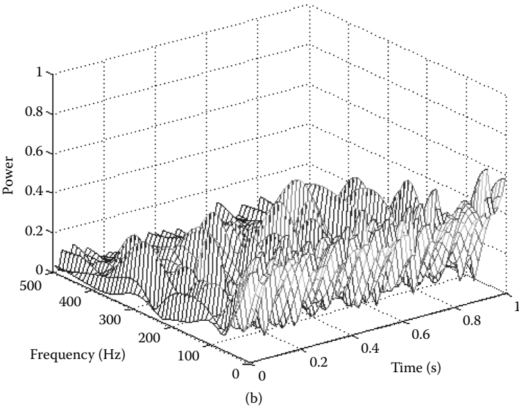
FIGURE 12.8 STFT results at different forces: (a) high force and (b) low force.
