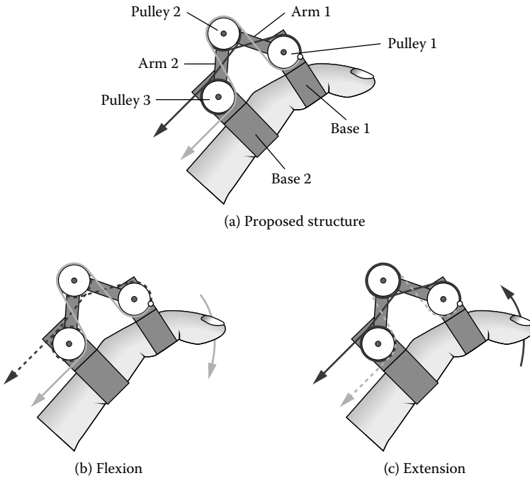
FIGURE 15.3 Proposed design.
