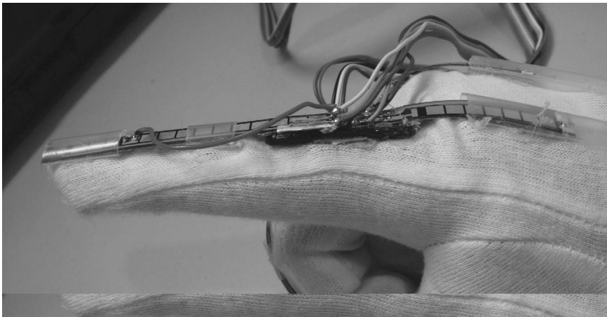
FIGURE 15.12 Data glove used for measurement of DIP and PIP joint angles.
