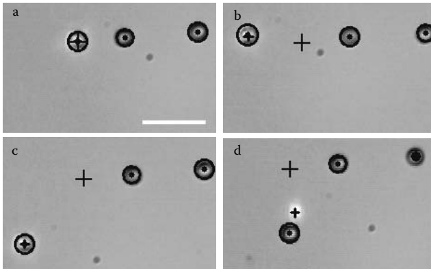
FIGURE 8.5 Robotic manipulation process of microbeads by optical tweezers: the large cross denotes the initial position of the manipulated bead, while the small cross denotes the position of the optical trap. The black circle and dot indicate the contour and the center of the microbeads, respectively. Scale bar is 10 \mu\text{m} . Reprinted with permission from IEEE (Tan et al. 2009).
