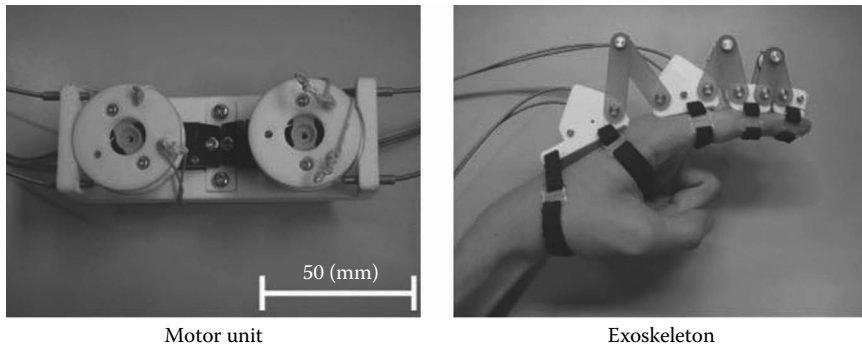
FIGURE 15.9 Prototype of the exoskeleton for one finger.
