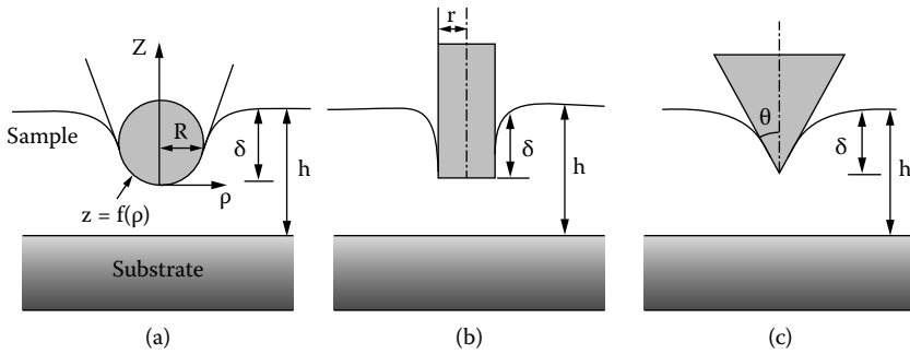
FIGURE 9.5 Schematics of the tip–sample contact for (a) spherical, (b) cylindrical, and (c) conical tips.
