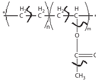
FIGURE 2.36 Chemical structure of ethylene vinyl acetate (EVA) copolymer with the structural groups isolated.
