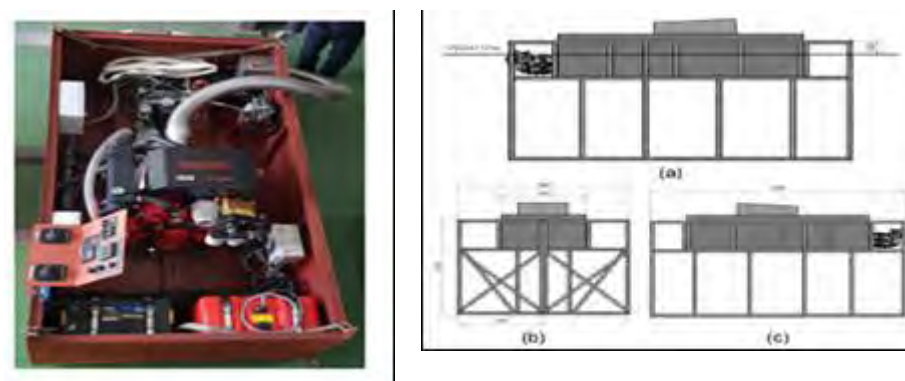
Figure 10: Test Bed for the USV Platform and Frame for the Test Bed
