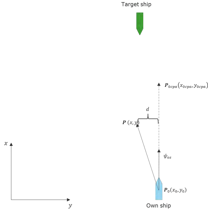
Figure 7: Head-on situation
