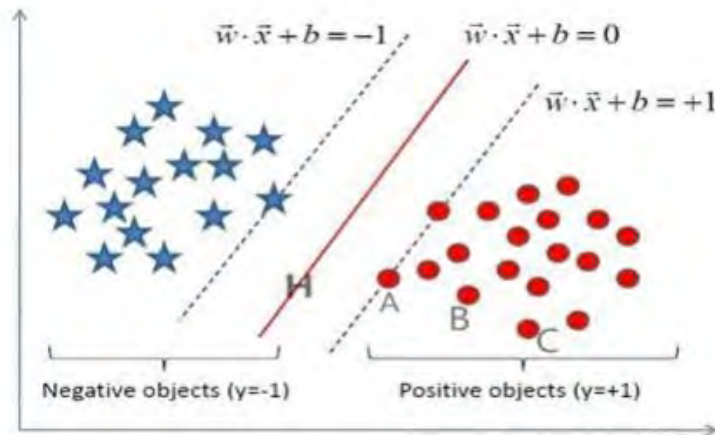
Figure 4: Schematic diagram of SVM
