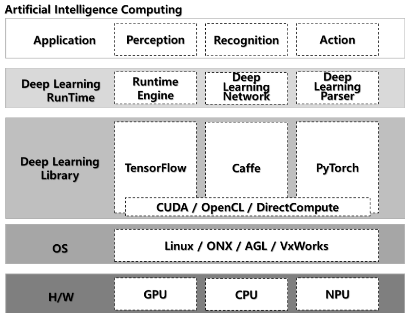
Figure 6: Structure of Computing Module for Autonomous Vehicle
