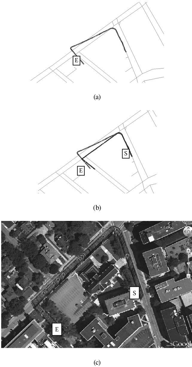
FIGURE 9.15 (See color insert.) Position estimations and map matching results. (a) Monocular visual odometry results in one route before map matching. (b) Estimated locations on one route before map matching and after map matching. (c) Map matching results overlaid on Google Maps.
