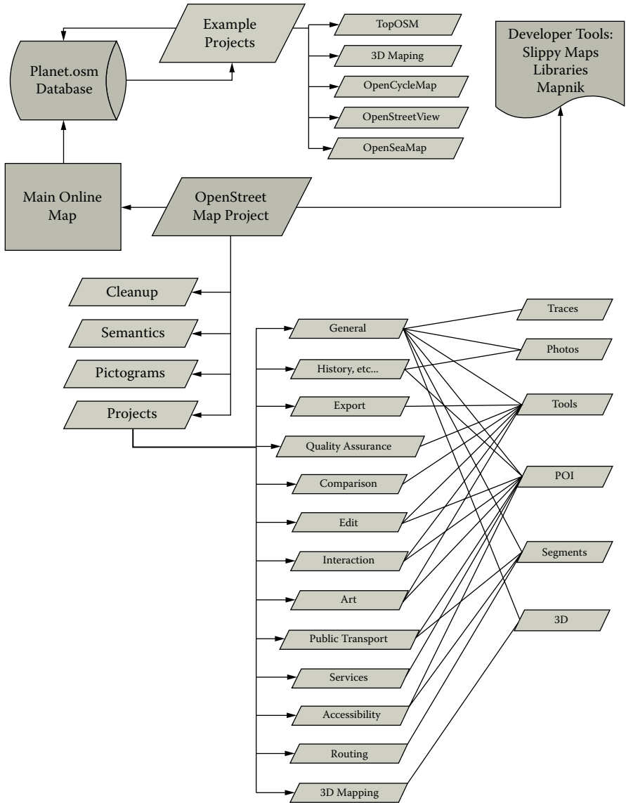
FIGURE 6.9 OSM Landscape.
