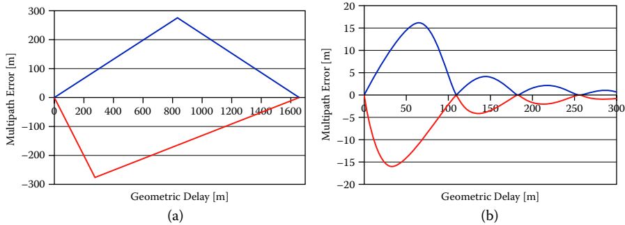
FIGURE 1.14 Multipath error envelopes for (a) GSM and (b) UMTS. (From Hein, G., 2001, On the Integration of Satellite Navigation and UMTS, CASAN-1 International Congress, Munich, Germany.)
