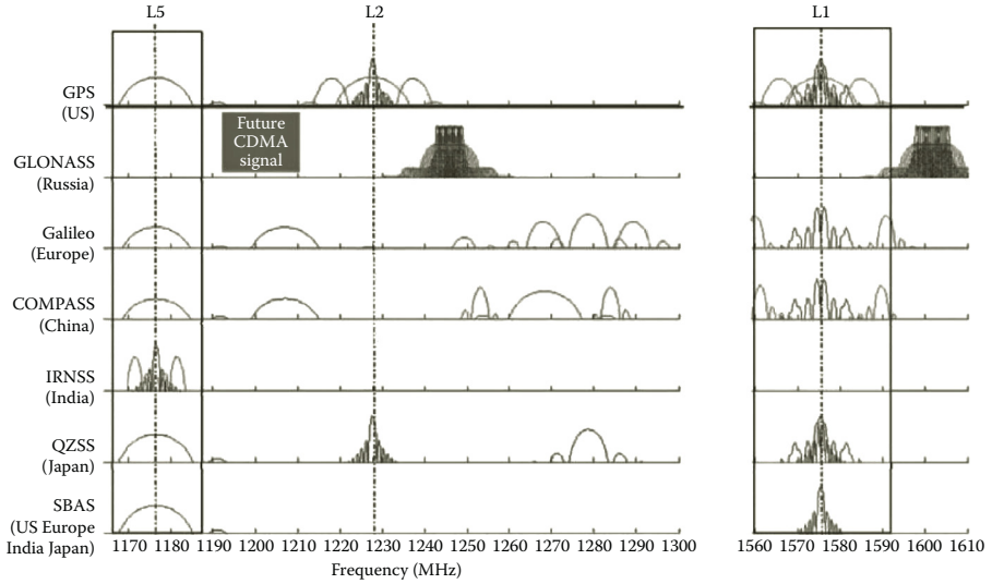
FIGURE 1.9 (See color insert.) Proposed Signal Overlay for all available GNSS, RNSS and SBAS (Turner, 2010). With Permission.
