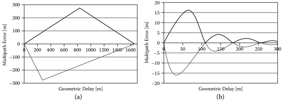
FIGURE 1.14 (See color insert.) Multipath error envelopes for (a) GSM and (b) UMTS. (From Hein, G., 2001, On the Integration of Satellite Navigation and UMTS, CASAN-1 International Congress, Munich, Germany.)
