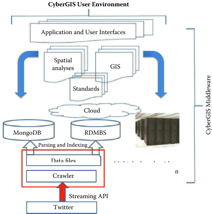
FIGURE 8.1 CyberGIS architecture.
