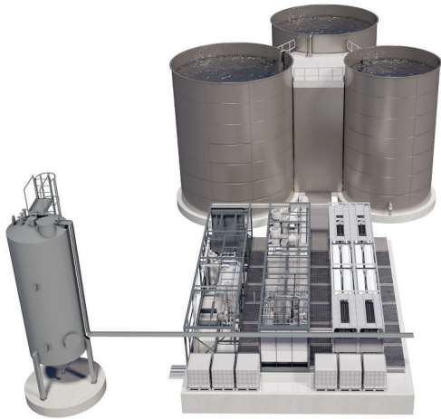
Figure 6.16: Arla-Vimmerby MBR WWTP in Sweden based on the Grundfos BioBooster modular concept. The concept of a Biobooster system and similar concepts, which have emerged in recent years, is a modular decentralised wastewater plant that is pre-assembled and can be delivered on trucks on site. The modularity allows for easy extending of the plant in case of increased load and vice versa.
