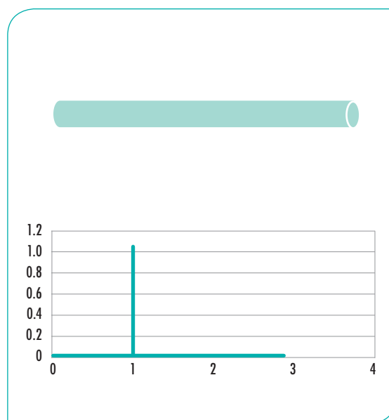
Figure 4.20: Not mixed reactor, i.e. similar to a piece of pipeline. The curve shows how the concentration in the tank at position “1” develops as function of time when a pulse disturbance has been injected at time 0 in the inlet of the pipeline. This type of flow pattern shows the same kind of concentration out of the reactor as the pattern flowing in.
