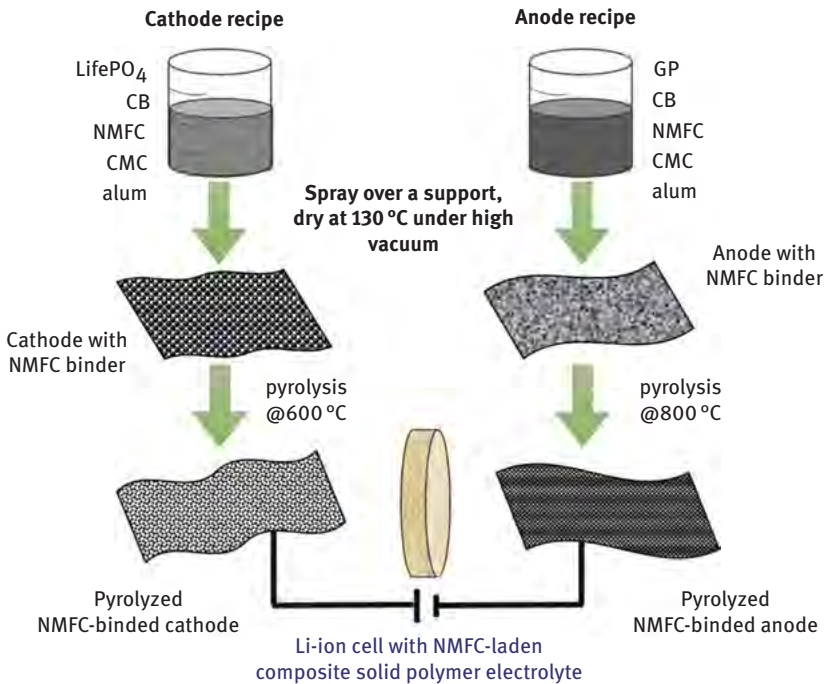
Figure 6.5: Different phases of the process involved in obtaining pyrolyzed nanocellulose-bound electrodes, which are then used to assemble the solid polymeric \text{Li}^+ -ion cell. (Image courtesy by Carbon (Elsevier) to reuse in a book under the copyright license number 4454160899455)
