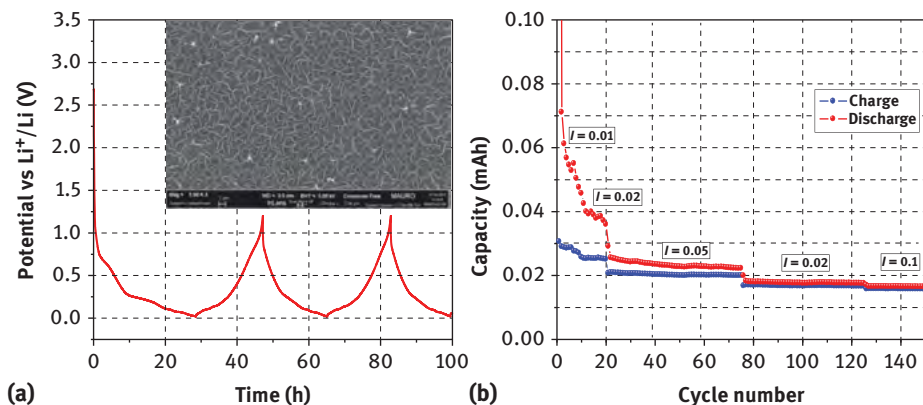
Figure 6.4: (a) Graph showing the galvanostatic charge/discharge curves of CNWs deposited on Cu: inset – morphological characterization of the nanostructured carbons deposited on Cu by FESEM ( ZEISS Supra 40 ); (b) capacity versus number of cycles in a cell Li/electrolyte/CNW-Cu at room temperature. (Image courtesy by Electrochimica Acta (Elsevier) to reuse in a book under the copyright license number 4454750182186)
