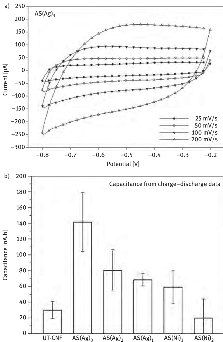
Figure 2.5: Cyclic voltammetry of carbon nanofibers functionalized with silver (a) and capacitance (b) calculated from charge-discharge experiments. Reprinted with permission from [25] Copyright (2017) American Chemical Society.
