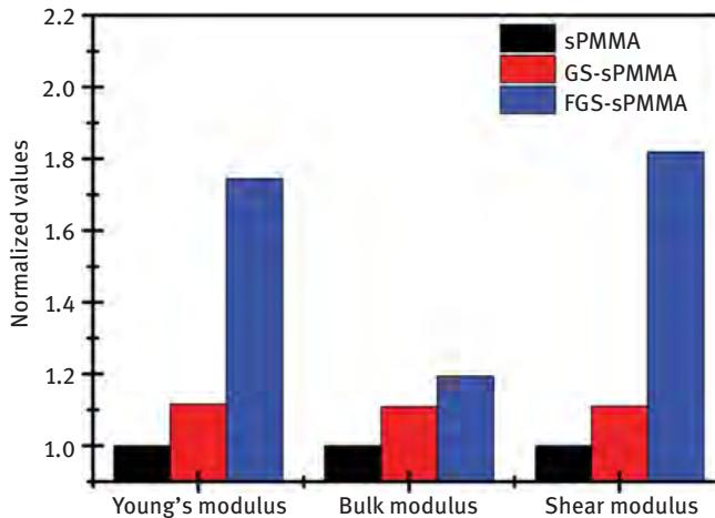
Figure 5.9: Summary of property improvement for the elastic constants of GS-sPMMA and FGS-sPMMA nanocomposites ( T = 300 K, P = 1 atm). Numerical values have been normalized with the corresponding value of the neat PMMA matrix at the same conditions ( E = 3.4 GPa, B = 4.2 GPa, G = 1.3 GPa and \nu = 0.36 ).
